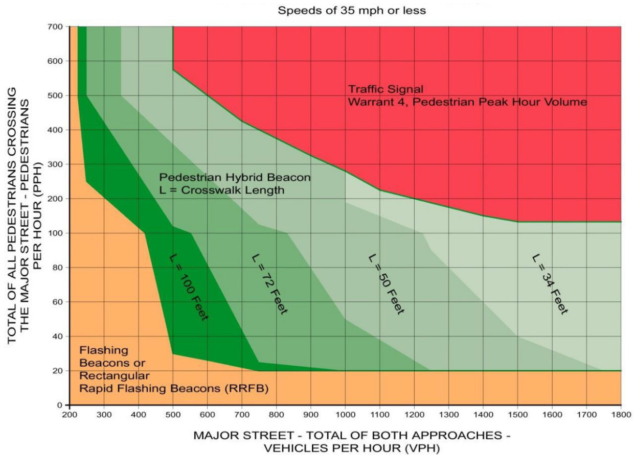
Figure 3.8-1. Guidelines for the Installation of Pedestrian Treatments on Low-Speed Roadways
