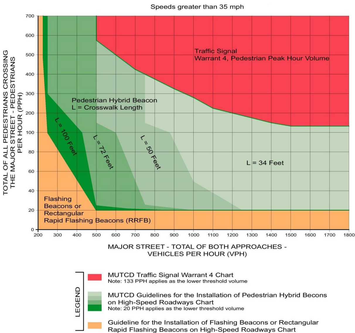
Figure 3.8-4. Guidelines for the Installation of Pedestrian Treatments on High-Speed Roadways
