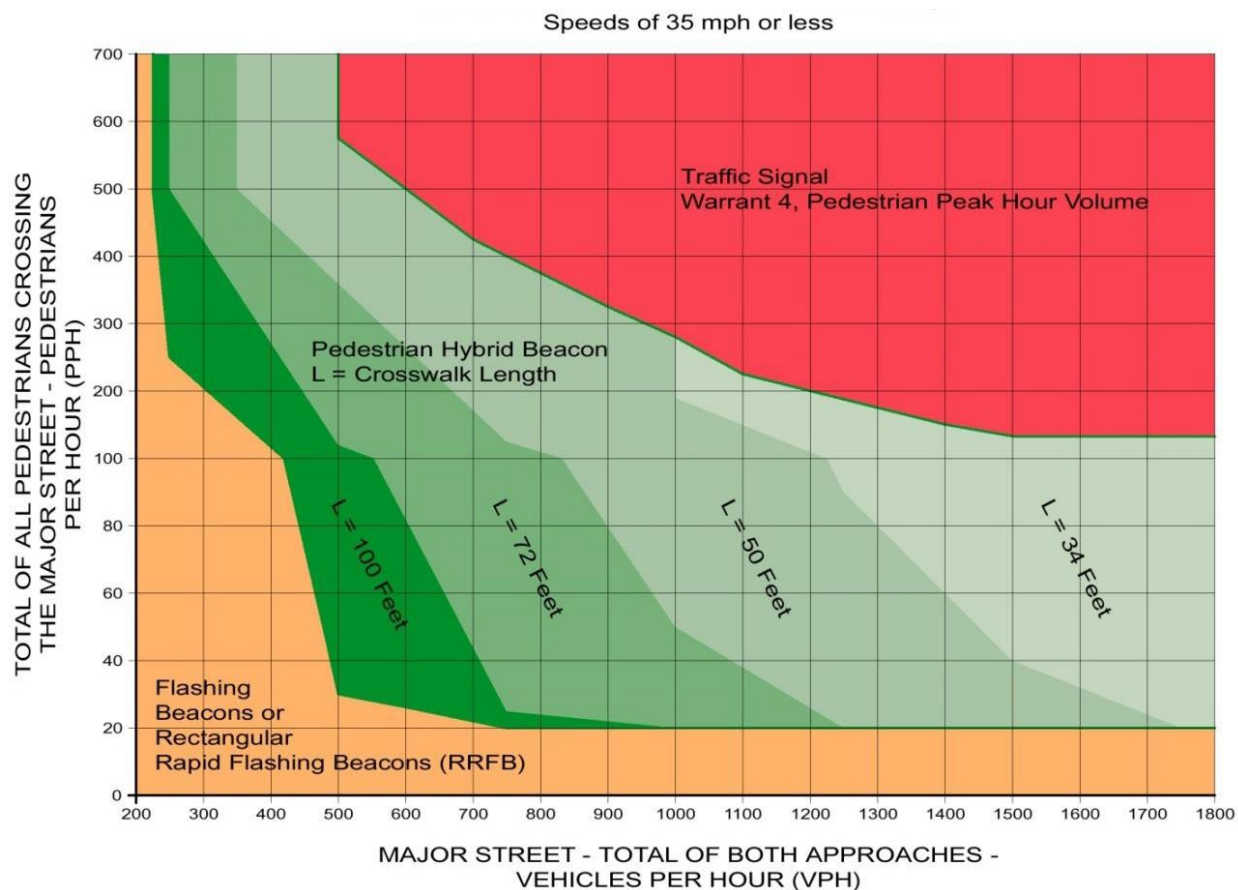
Figure 3.8-3. Guidelines for the Installation of Pedestrian Treatments on Low-Speed Roadways
