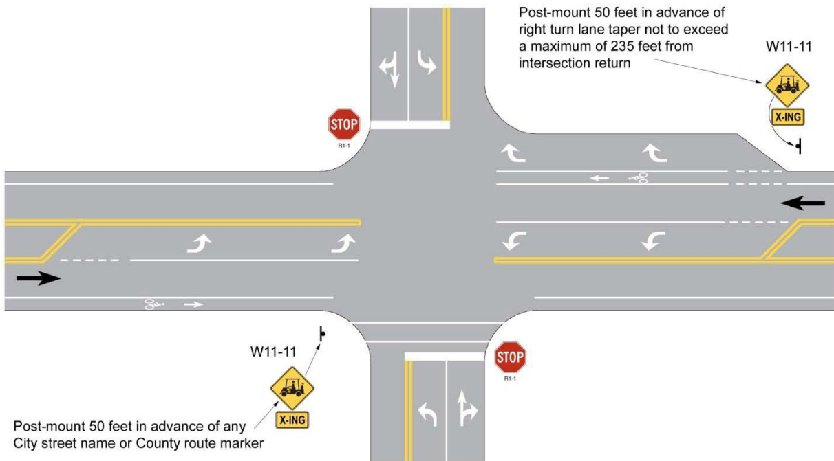
Figure 5.1-3. Stop-Controlled Crossing
