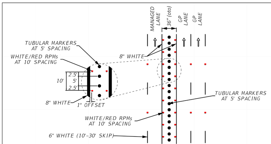
Figure 4.5-1. Separation Detail
