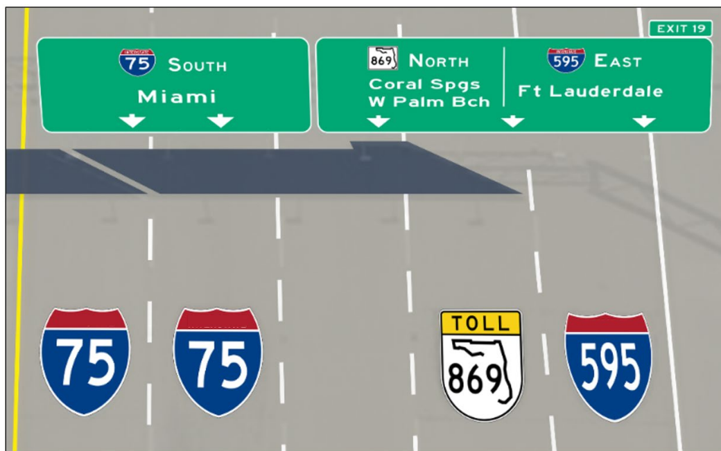
Figure 4.2-3. Route Shield Pavement Markings for Mainline
