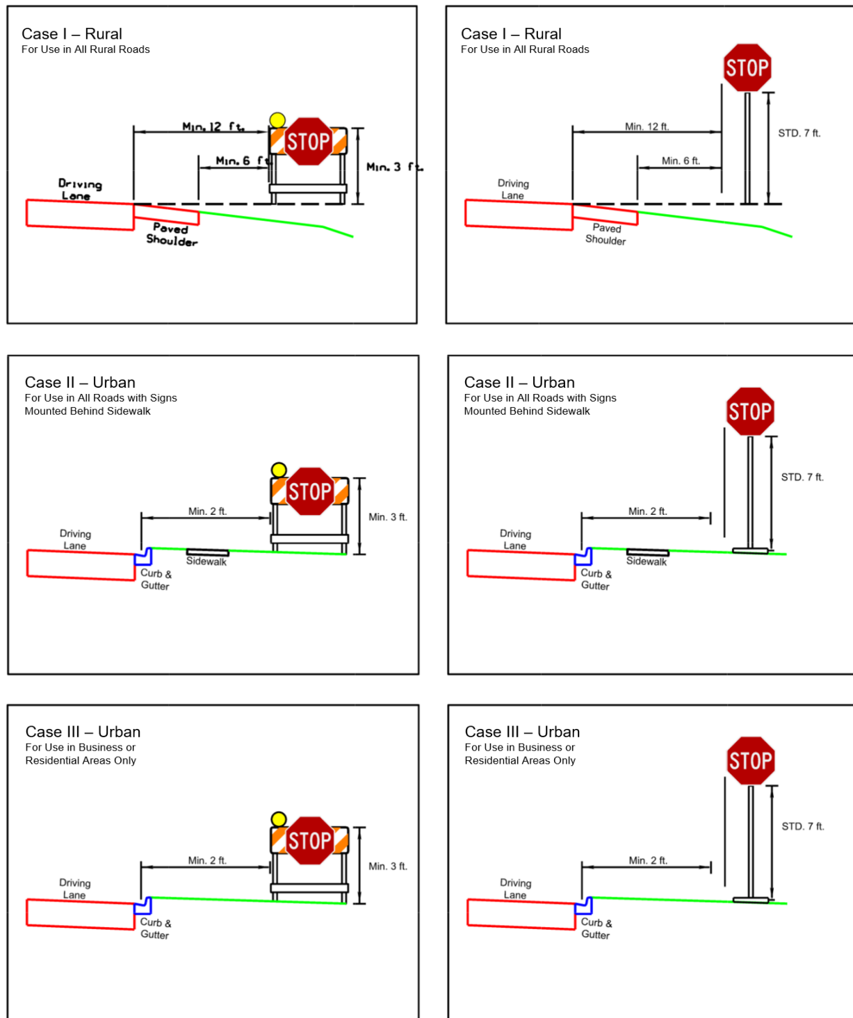
Figure 2.38-6. Temporary Signing for Power Outage—Sign Dimensions
