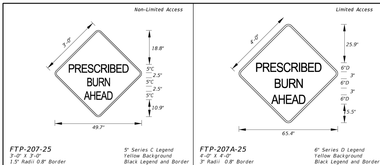
Figure 2.15-1. PRESCRIBED BURN AHEAD Signs
