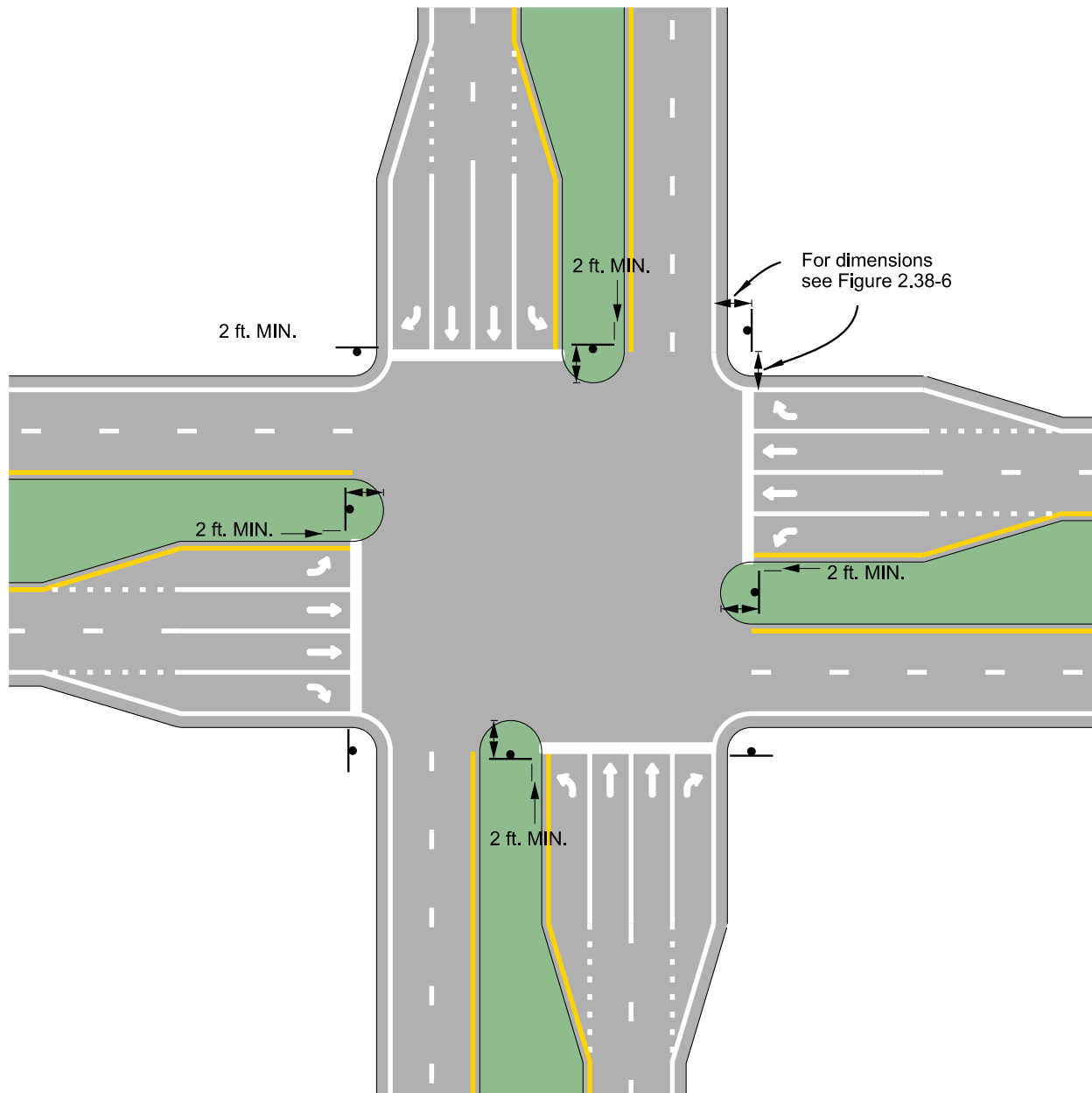
Figure 2.38-1. Temporary Signing for Power Outage—Left and Right Turn Lanes Intersection
