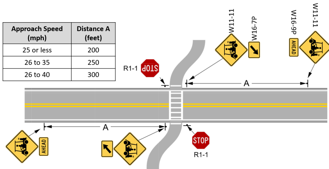
Figure 5.1-2. Midblock Crosswalk
