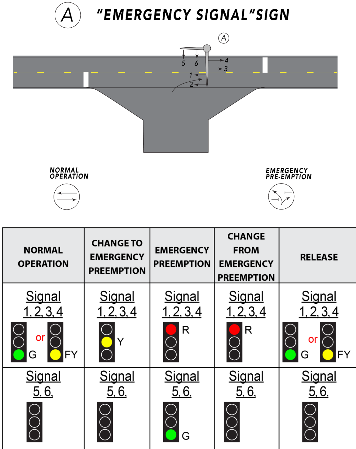
Figure 3.4-1. Mid-Block Emergency Signal Operation
