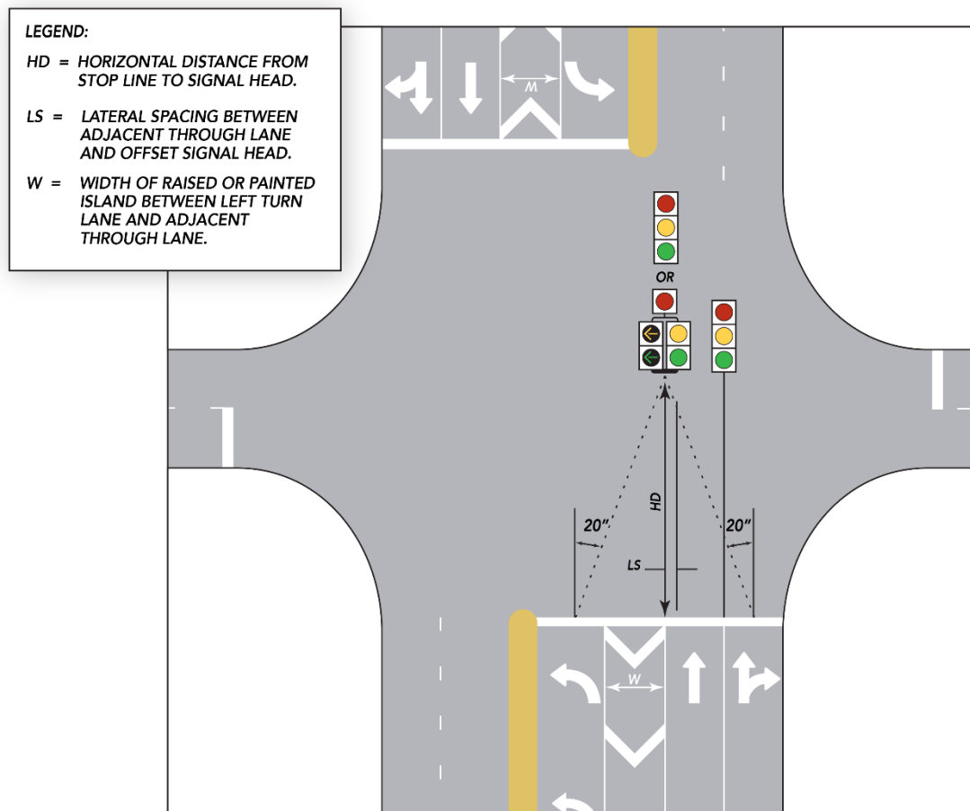
Figure 3.2-2. Left Turn Lane Signal Head Shift
