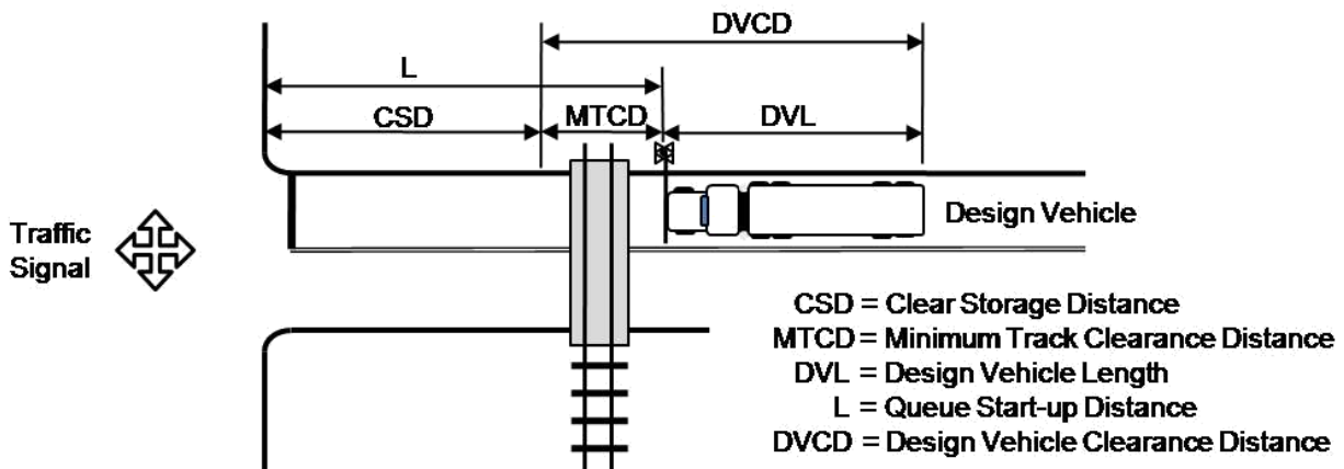
Figure 3.8-1. Geometric Data at the Highway-Rail Grade Crossing
