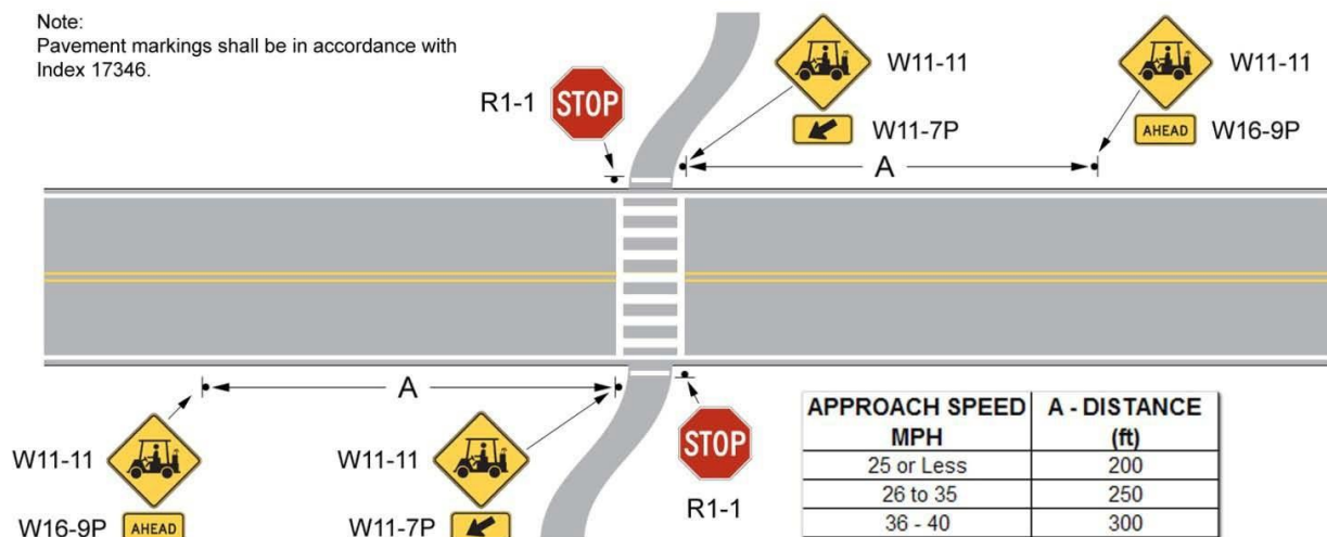
Figure 5.1-2. Mid-Block Crossing
