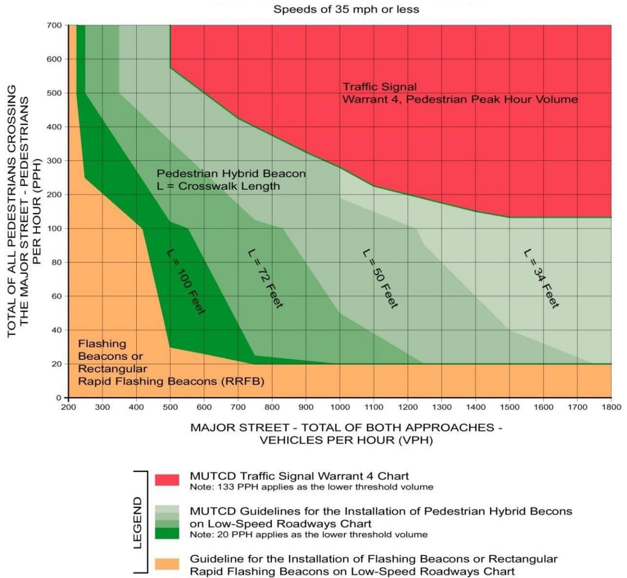
Figure 3.8-1. Guidelines for the Installation of Pedestrian Treatments on Low-Speed Roadways
