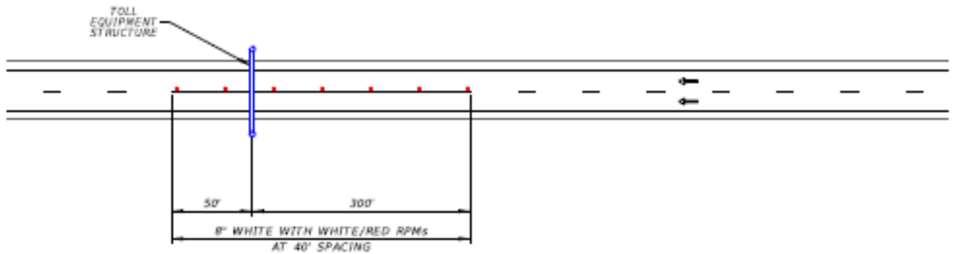
Figure 4.5-2. Striping Under Toll Gantry
