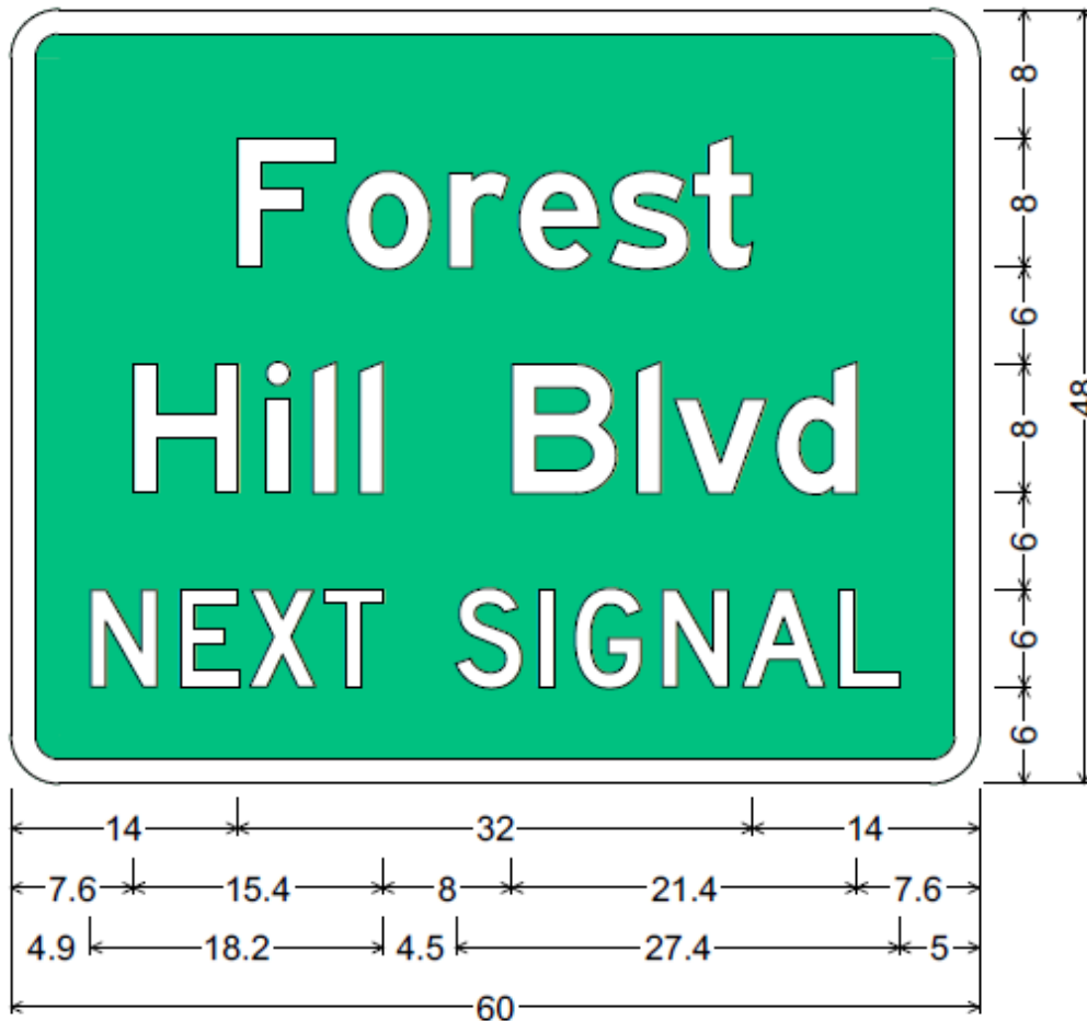
Figure 2.37-2. Advance Street Name Sign Design (Single Post)
