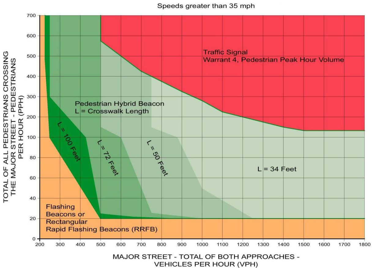
Figure 3.8-4. Guidelines for the Installation of Pedestrian Treatments on High-Speed Roadways
