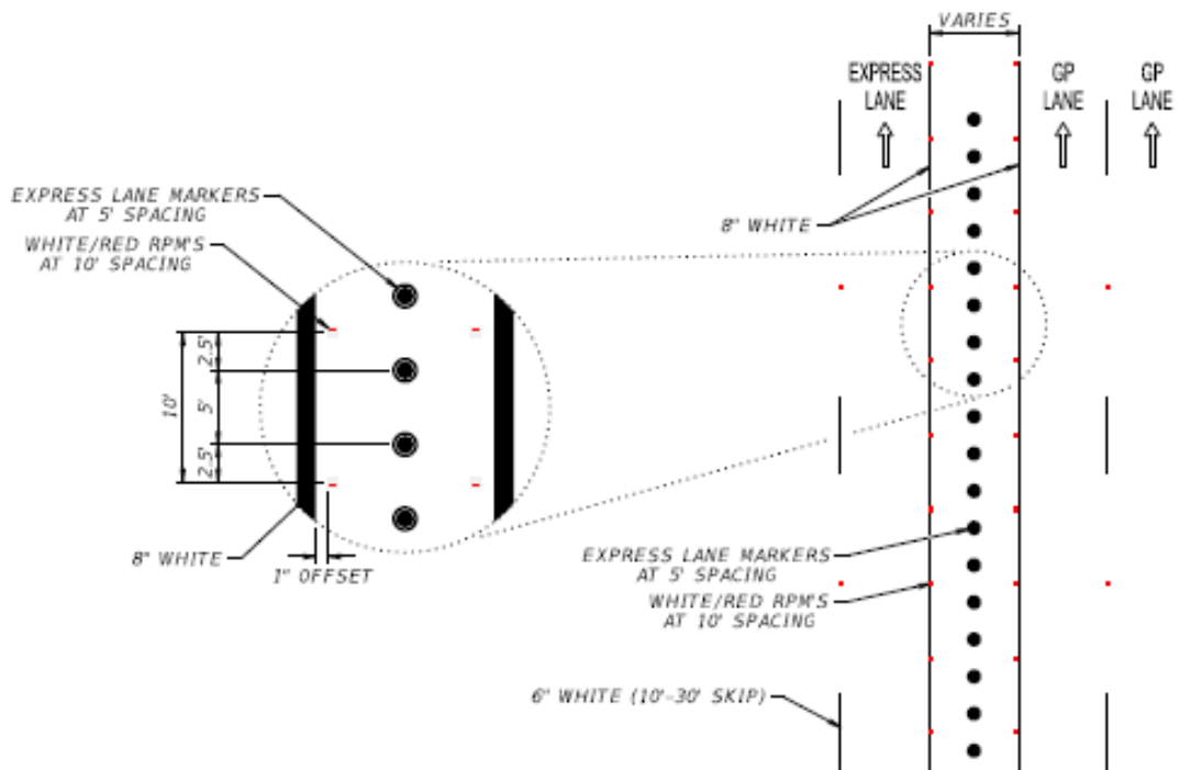
Figure 4.5.2. Striping under Toll Gantry
