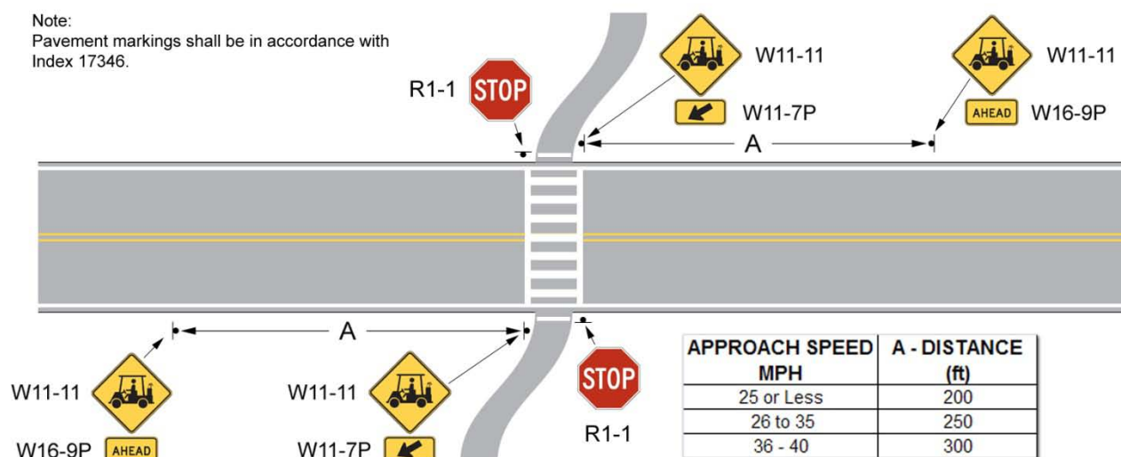
Figure 5.1-1. Mid-Block Crossing
