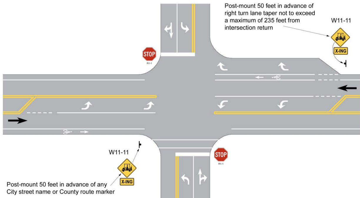
Figure 5.1-2. Stop-Controlled Crossing
