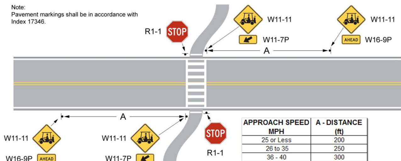
Figure 5.1-1. Mid-Block Crossing
