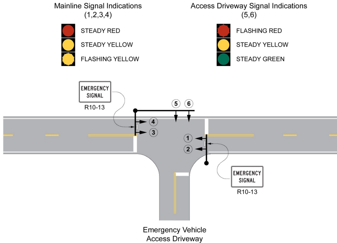
Figure 3.4-2. Mid-Block Emergency Signal Operation
