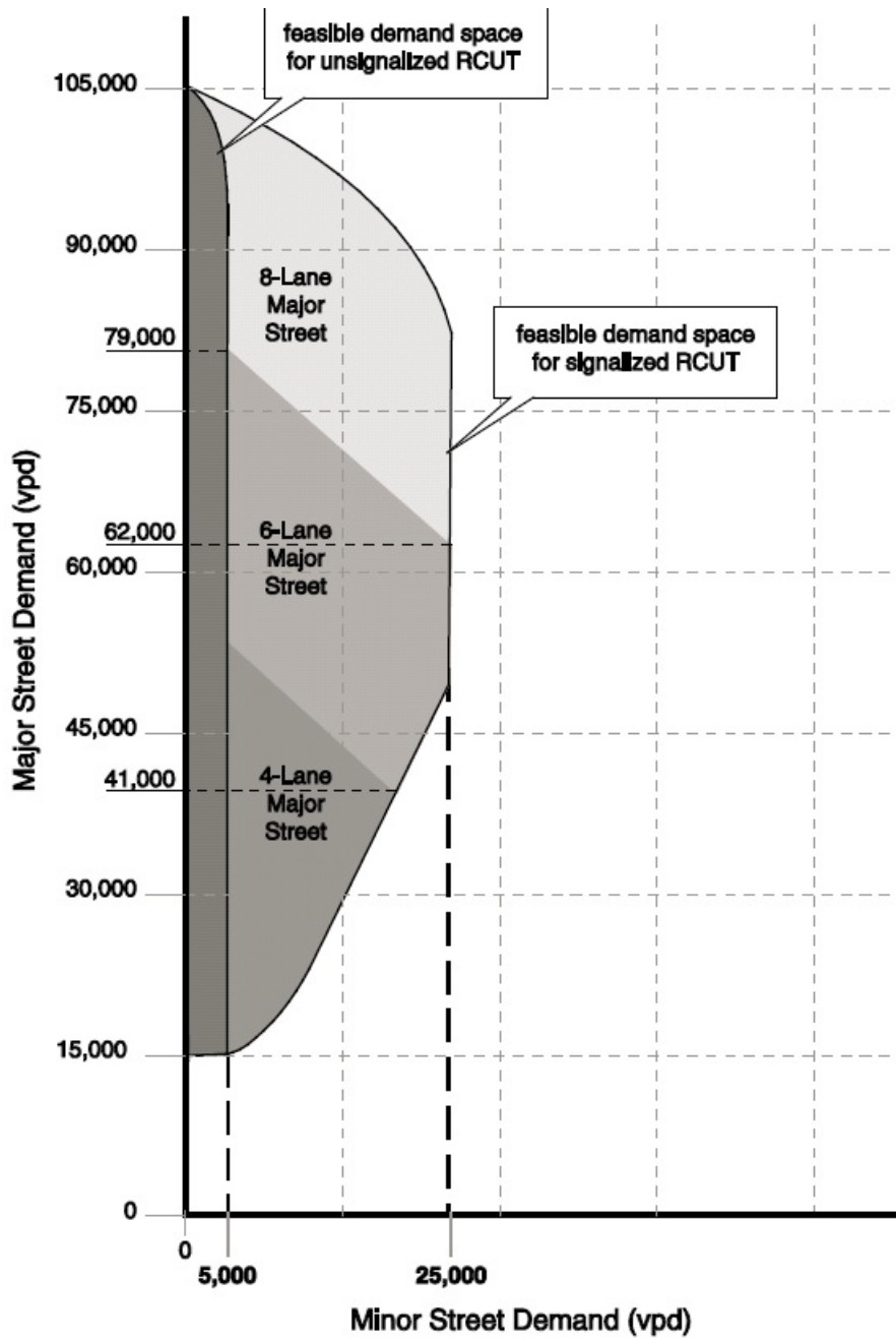
Figure A3: Feasible Demand Space for Signalized RCUT 10
