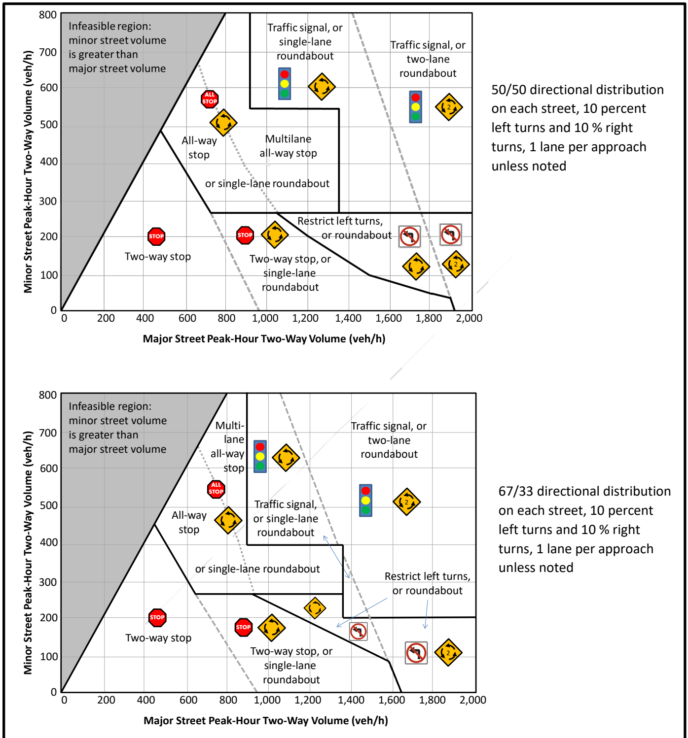
Figure A1: Intersection Control Type by Peak Hour Volume Thresholds 7
