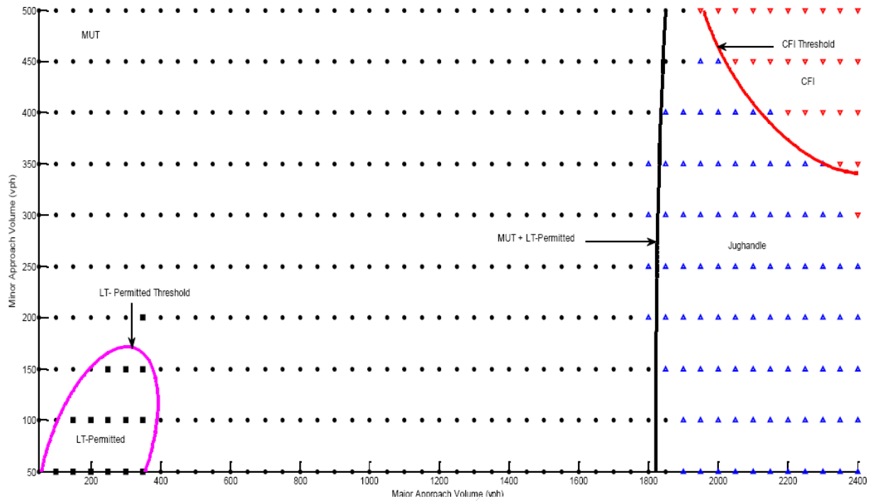
Figure A2: Decision Assistance Curves for Optimal Performance of Unconventional Intersections 9
