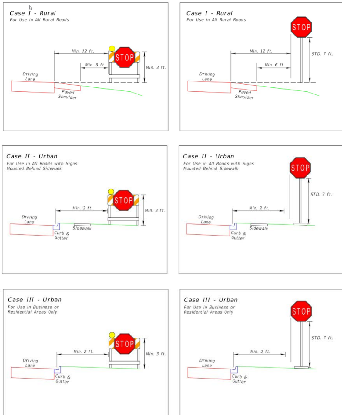
Figure 2.38-6. Temporary Signage for Power Outage – Sign Dimensions
