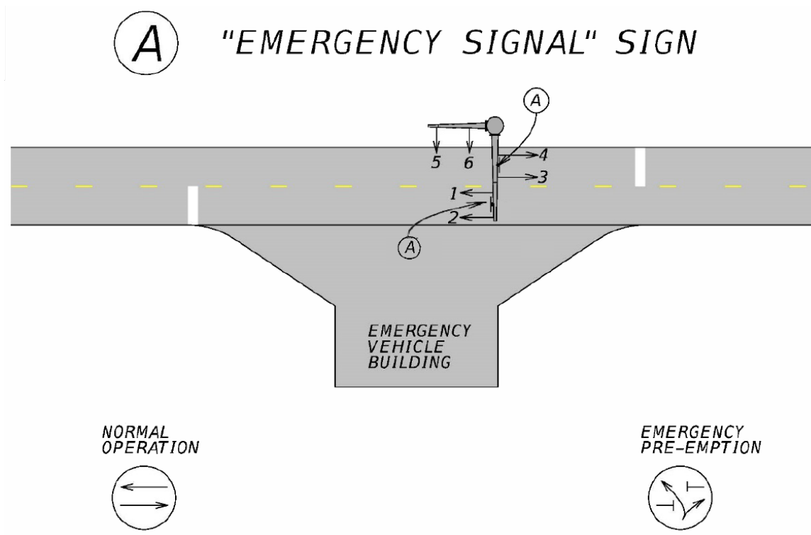
Figure 3.4-1. Mid-Block Emergency Signal Operation
