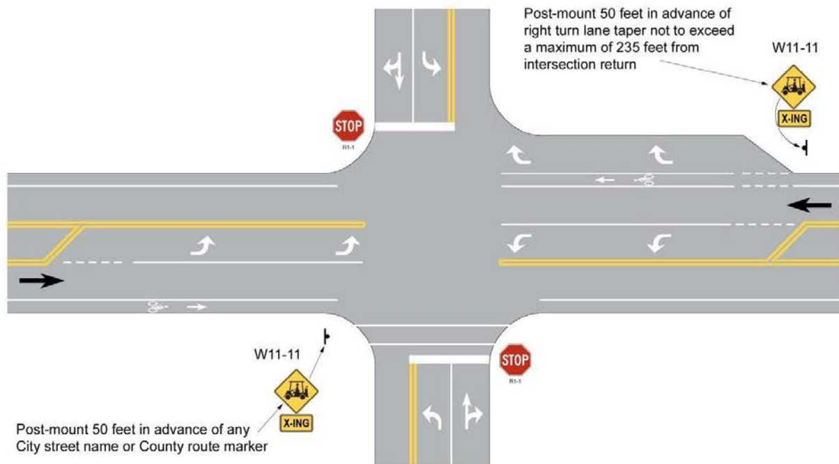
Figure 5.1-3. Stop-Controlled Crossing
