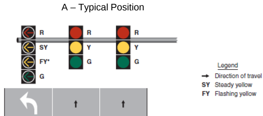
Figure 3.10-1. Four-Section Signal Protected-Permissive Left Turn Mode
