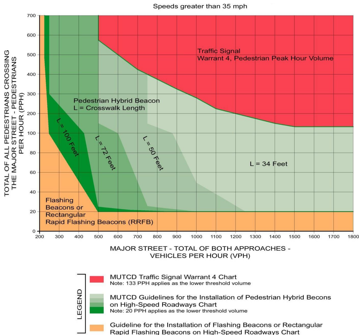
Figure 3.8-2. Guidelines for the Installation of Pedestrian Treatments on High-Speed Roadways
