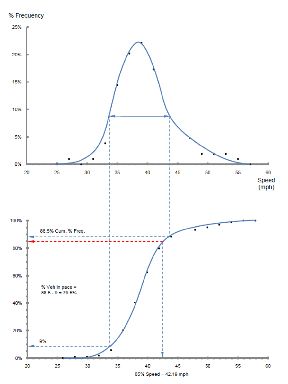
Figure 4-1. Speed Frequency and Cumulative Frequency Distribution Curves
