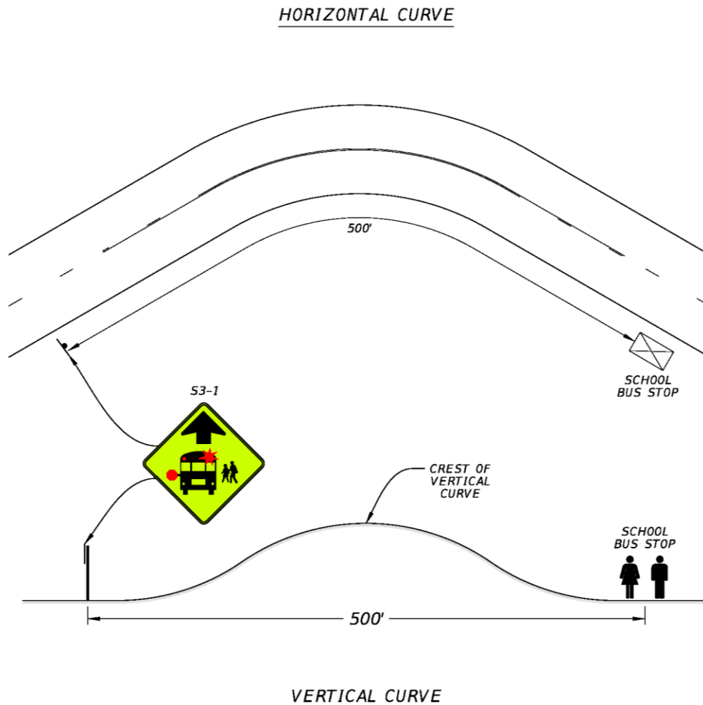
Figure 15-5 Traffic Control Devices at Typical School Bus Stop Locations
