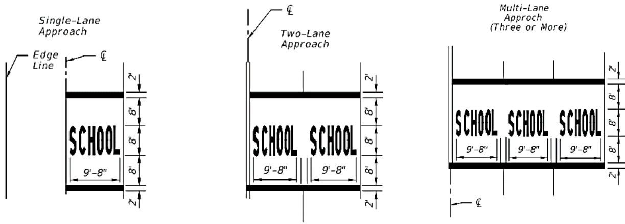
Figure 15-17B School Pavement Message Layouts for Single and Multi-Lane Approaches
