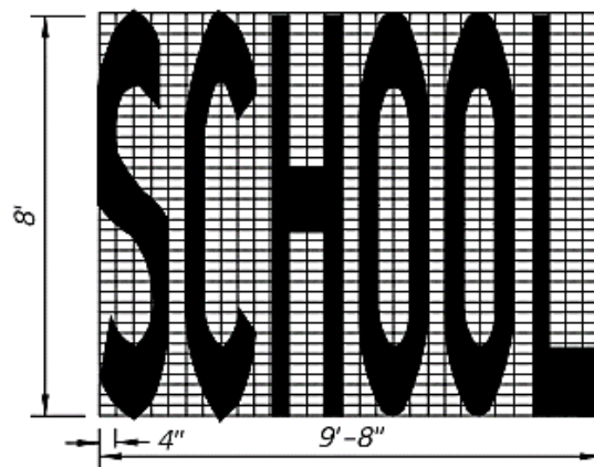
Figure 15-17A School Pavement Message Details
