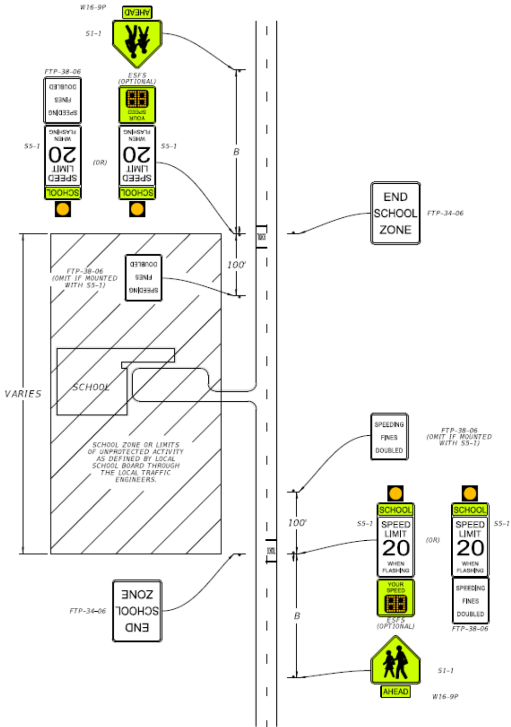
Figure 15-14 Typical School Zone Fronting the School Property Without a School Crossing
