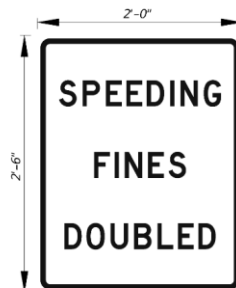
Figure 15-6A Speeding Fines Doubled Sign (Ground-Mounted Option – FTP 38-06)
