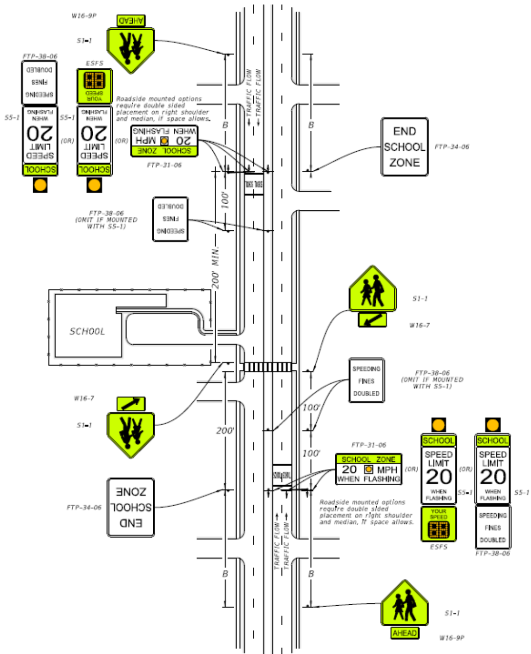
Figure 15-16 Typical School Zone With School Crossing (Multilane Divided) (45 mph or less) Mid-block or on Thru Street at an Intersection
