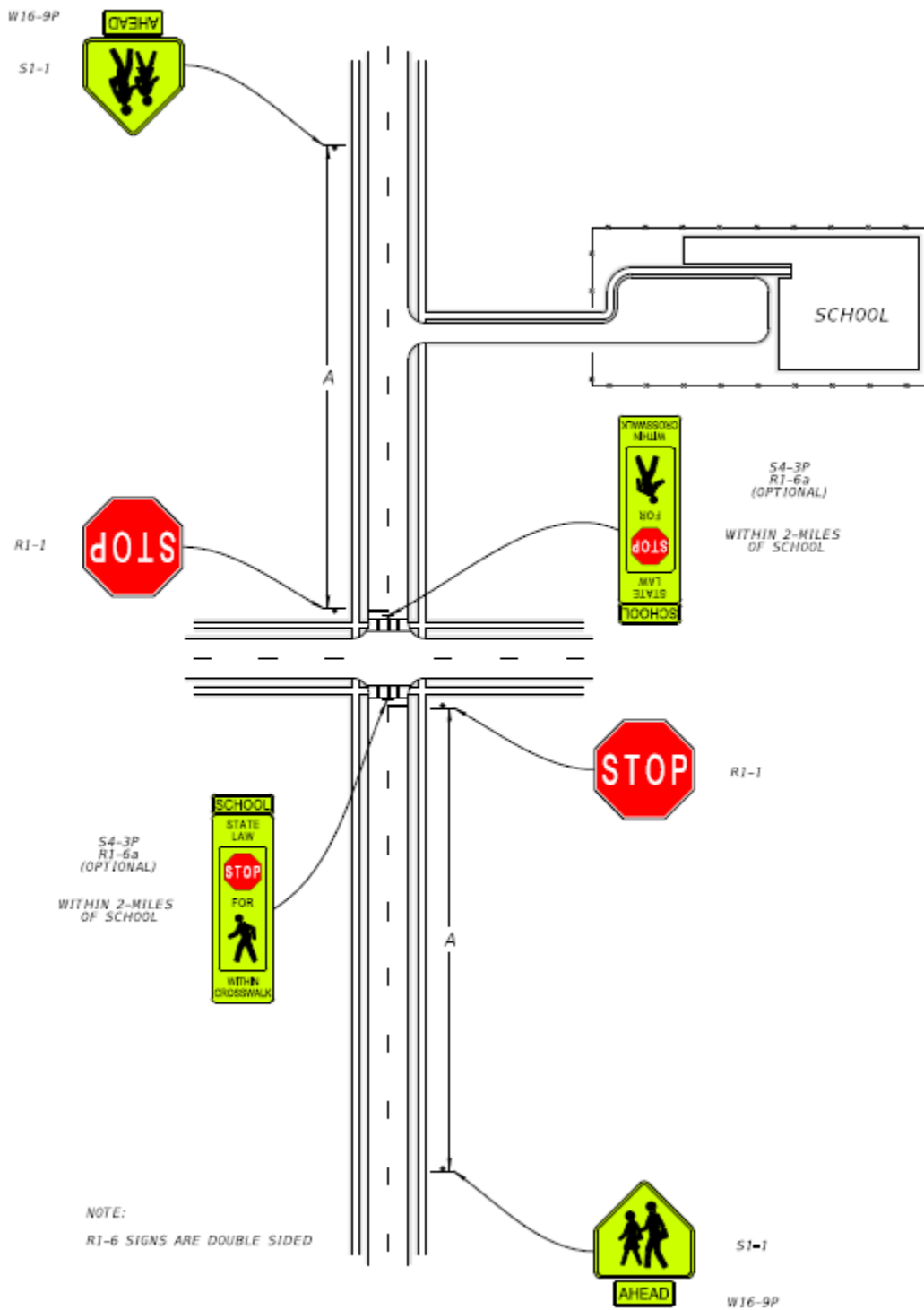
Figure 15-3 School Crosswalks at a Stop Controlled Intersection Without a School Zone
