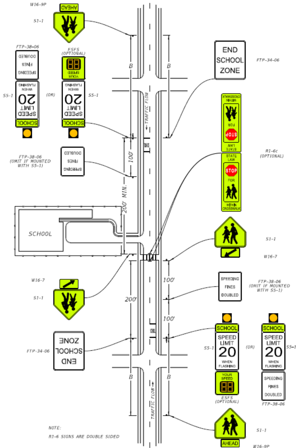
Figure 15-13 Typical School Zone With School Crossing (2- or 3-Lane, 2-Way) (45 mph or less) Mid-block or on Thru Street at an Intersection
