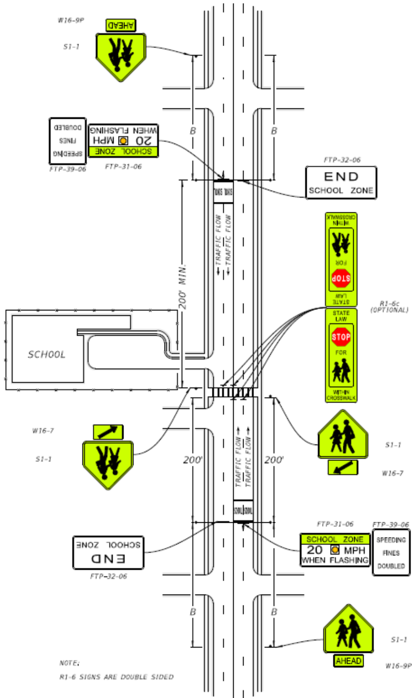
Figure 15-15 Typical School Zone With School Crossing (Multilane Undivided) (45 mph or less) Mid-block or on Thru Street at an Intersection
