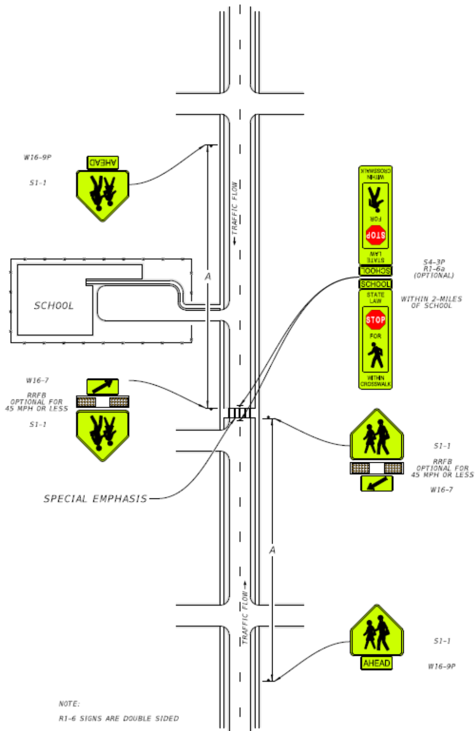
Figure 15-4 Midblock School Crosswalks Without a School Zone
