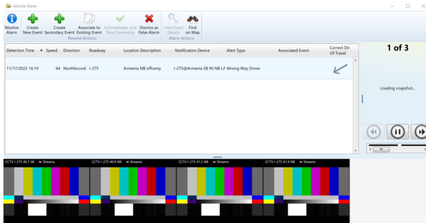
Figure 33: SunGuide Software System Alerts Window
