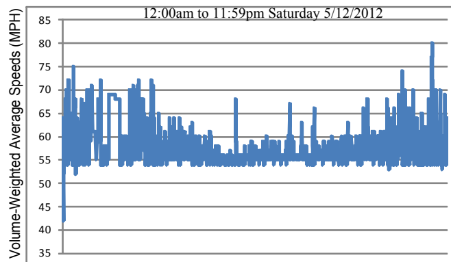
Figure 3: Volume-Weighted Speed Averages for “SR 528 @ I-95”
