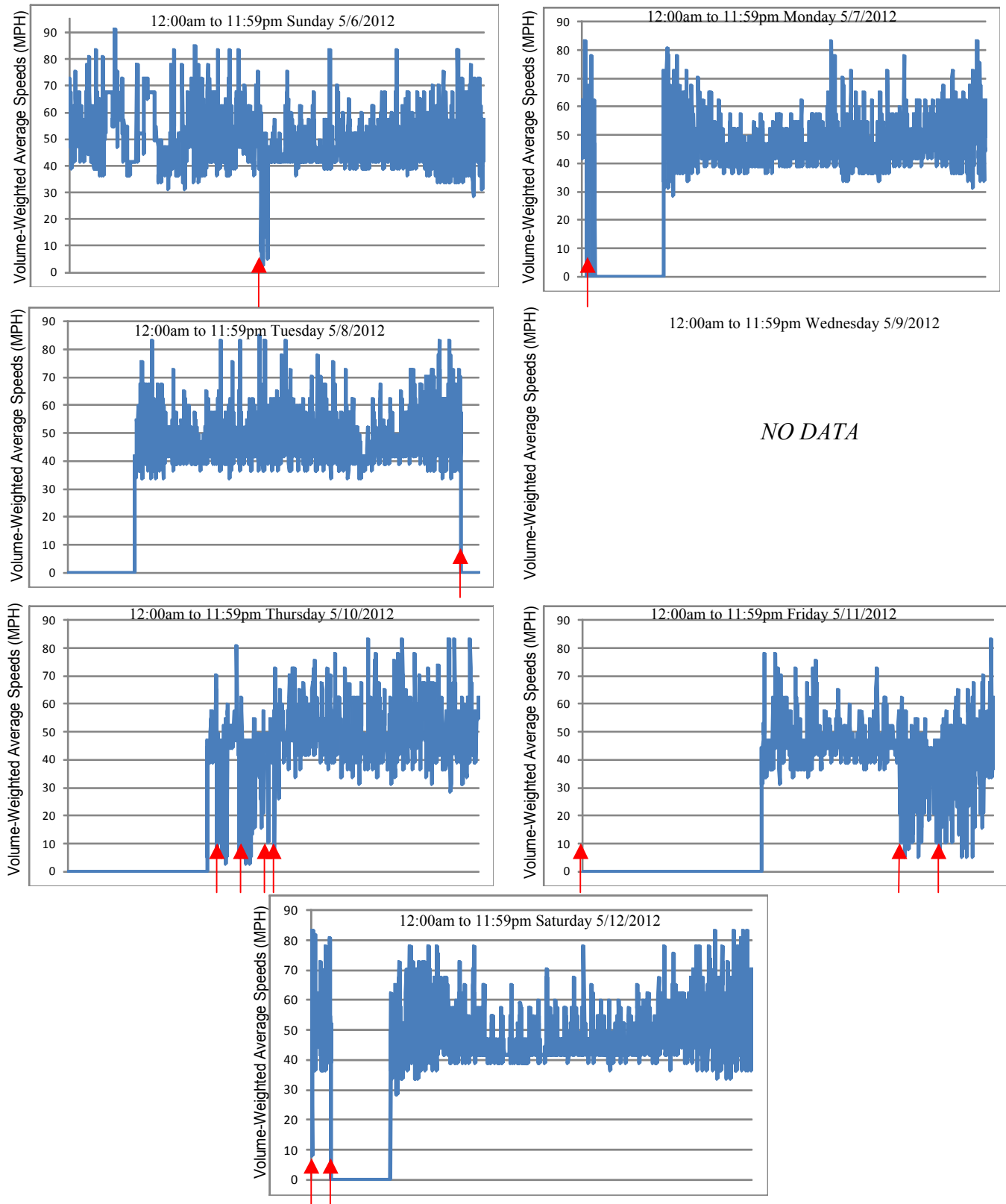
Figure 4: Volume-Weighted Speed Averages for “SR 528 @ Friday Rd”
