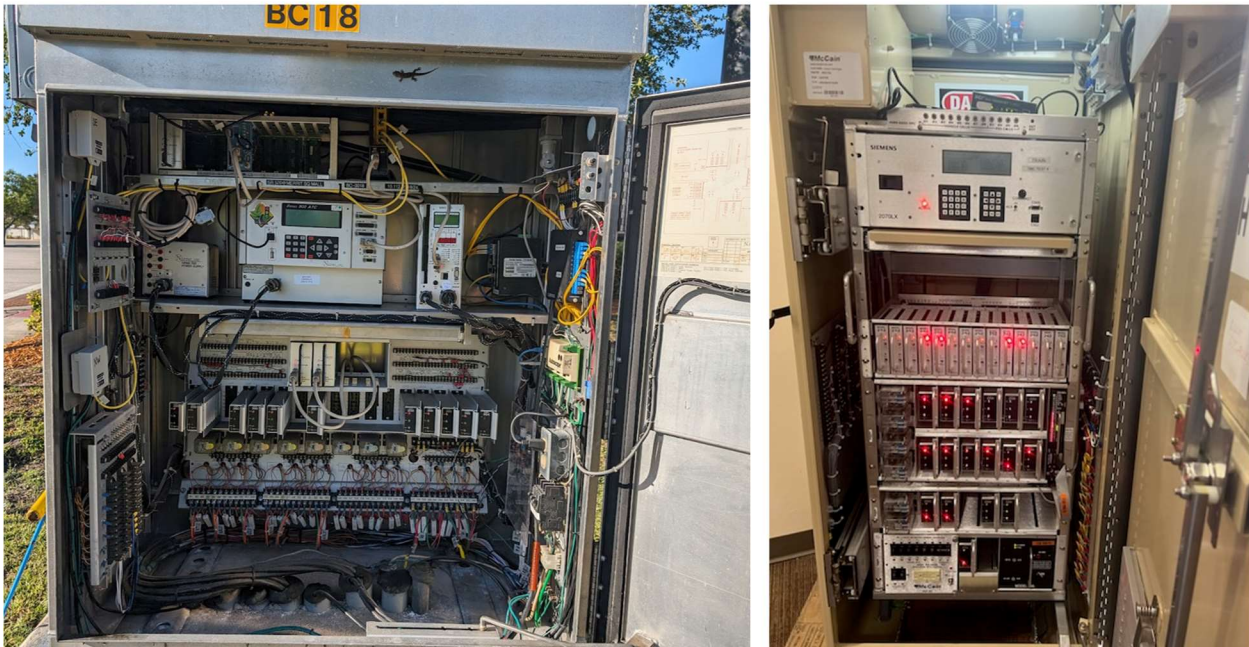
Figure 3-15: Examples of signal controller cabinet assembly interiors
