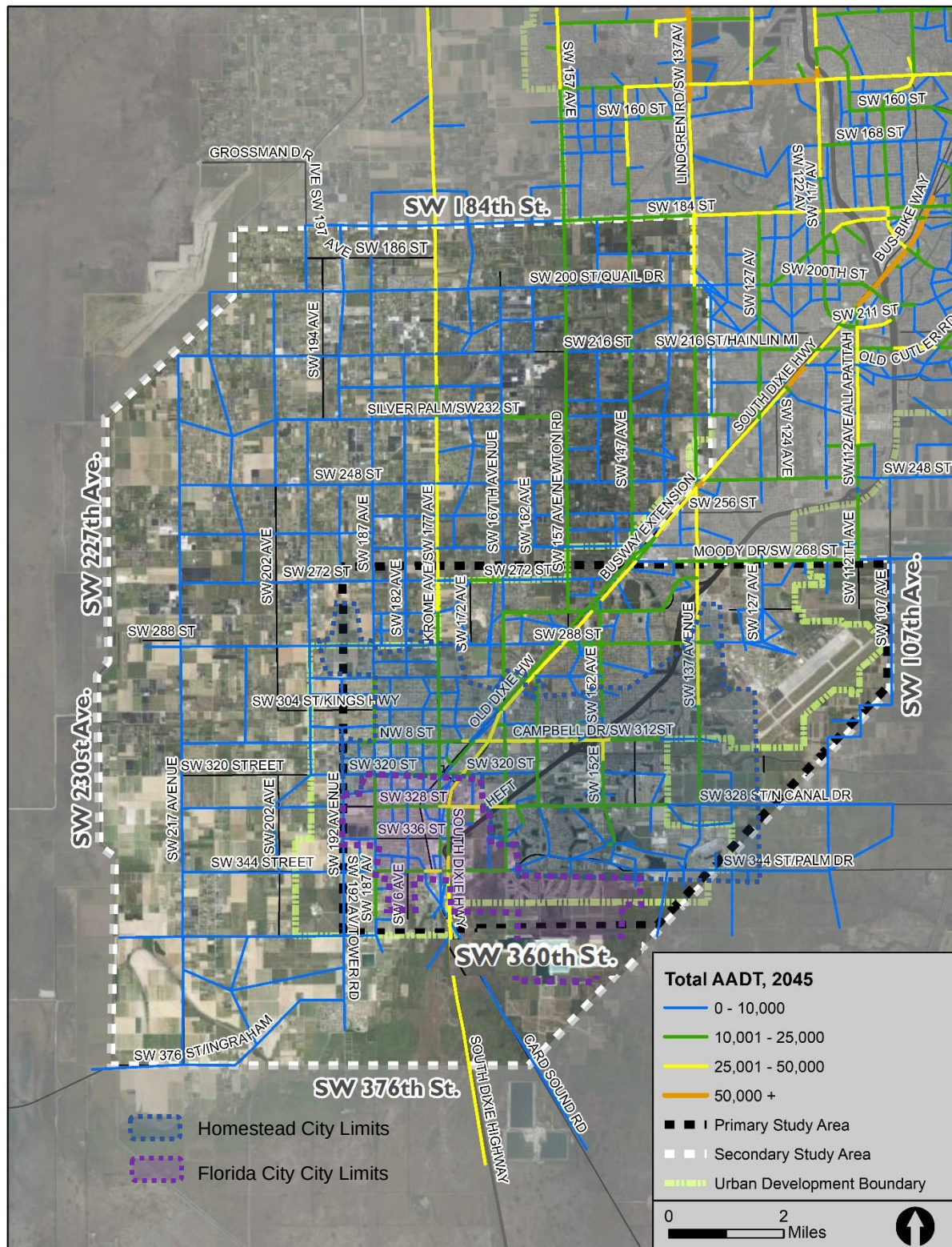
Figure 4-4 Total AADT, 2045
