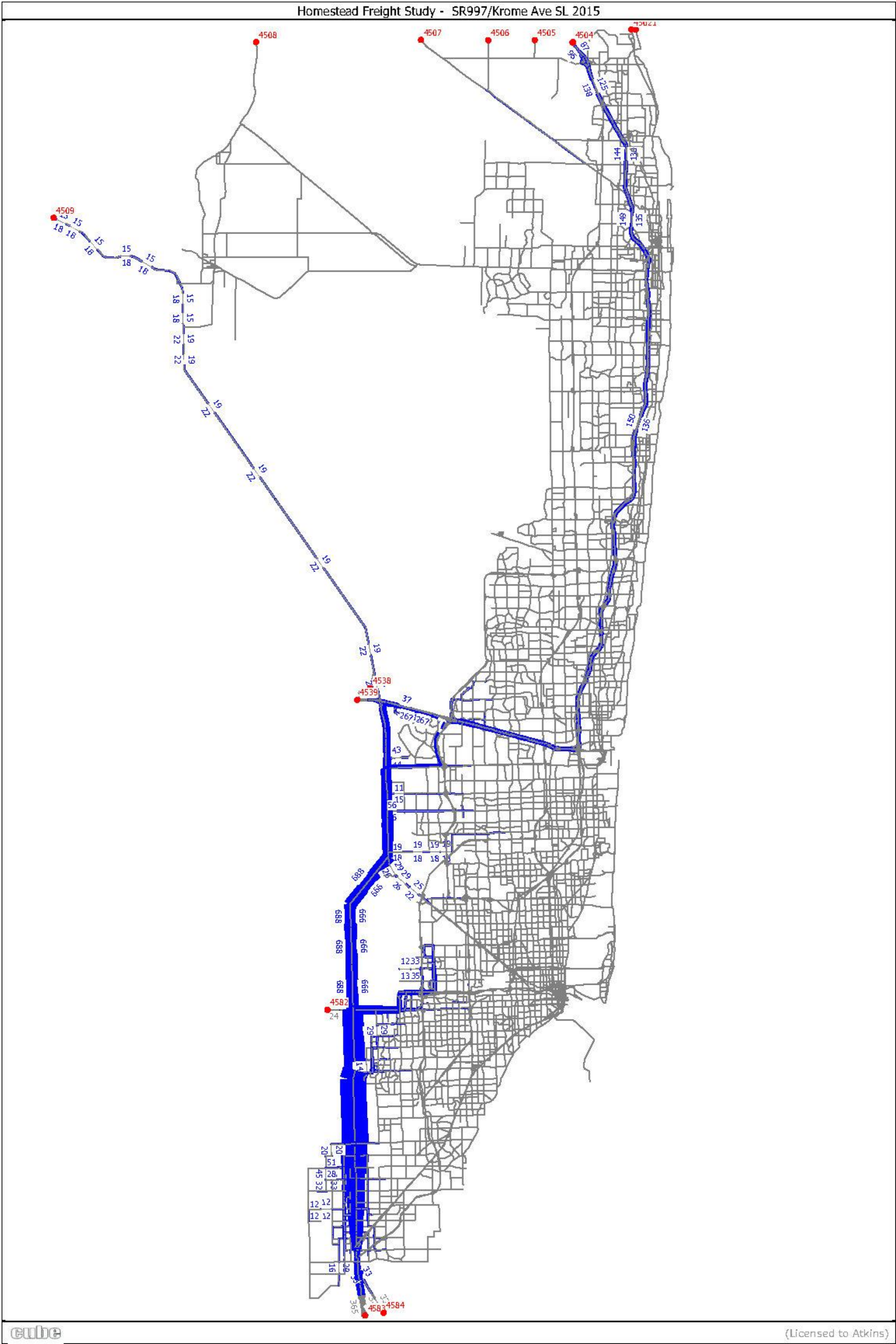
Figure 4-22 SR 997/Krome Avenue at Select Link, 2015
