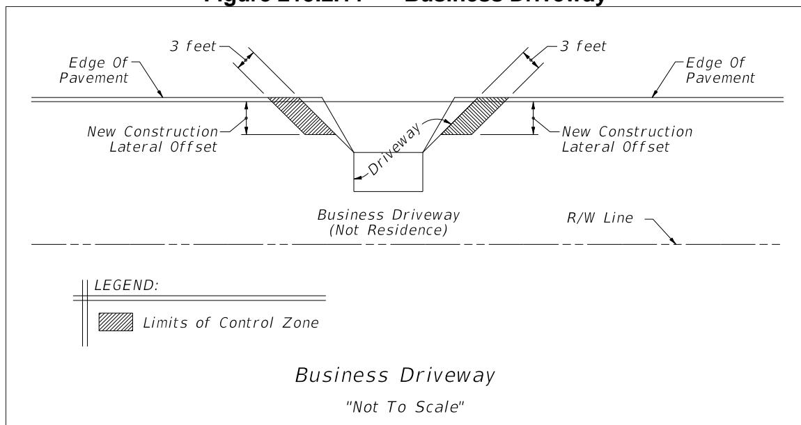
Figure 215.2.11 Business Driveway
