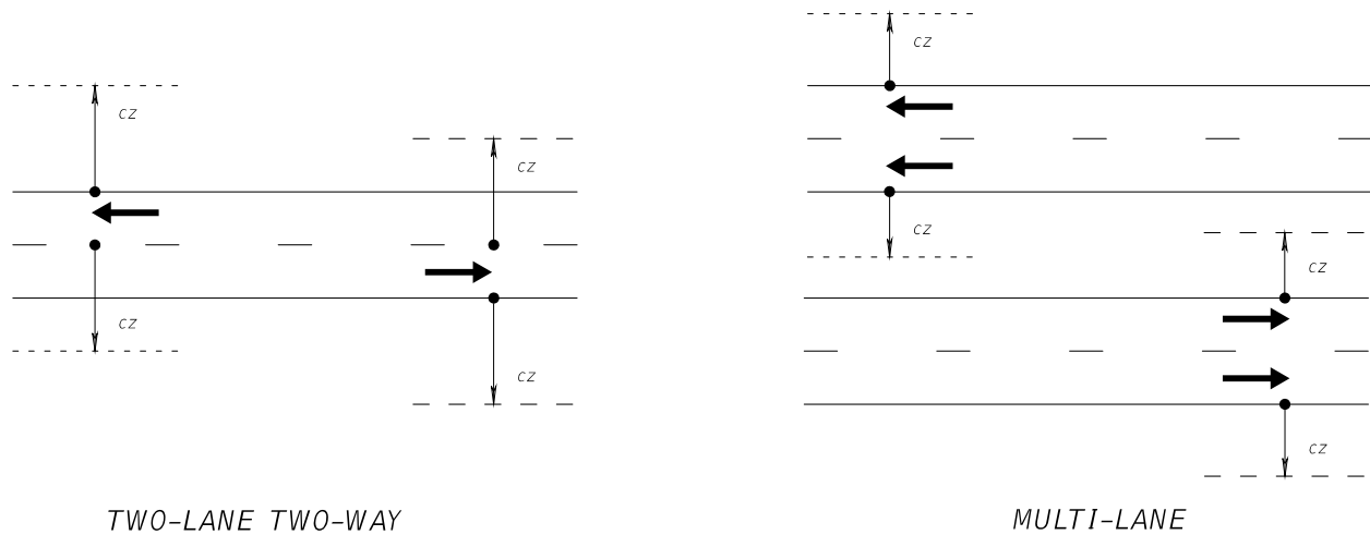
Figure 215.2.2 Clear Zone Concept
