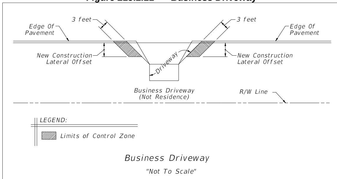
Figure 215.2.11 Business Driveway
