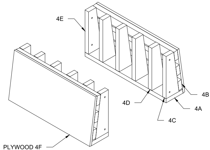
PANEL 4 ISOMETRIC VIEW
