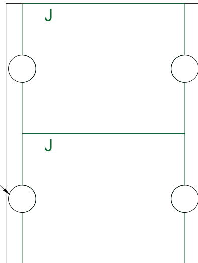
FRP PLATE CUTTING PLAN PLATES D-J, t = \frac{1}{4} "
