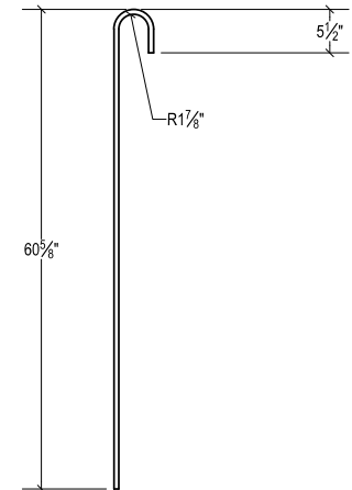
BAR J501 NO. 5 GR. 60 QTY. 4
