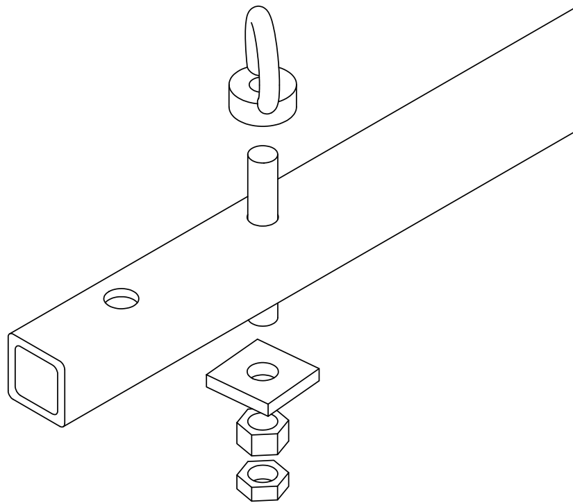
LIFTING EYE NUT ASSEMBLY
