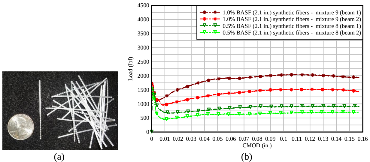
Figure 3.9 BASF synthetic fibers: (a) Fiber photograph; (b) CMOD flexural test results using BASF synthetic fibers at 1.0% and 0.5% fiber volumes (trial mixtures 8 and 9)
