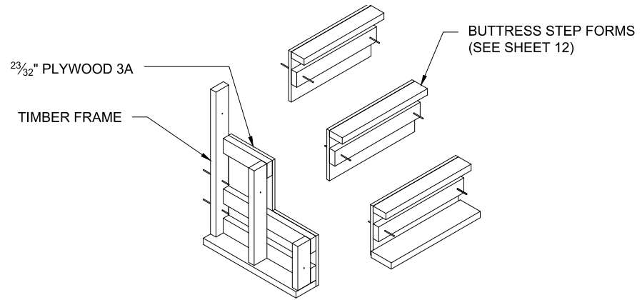
PANEL 3 ISOMETRIC VIEW OF COMPONENTS (RIGHT SIDE)
