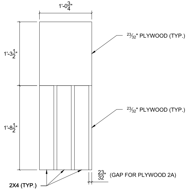
PANEL 2 BACK SEGMENT BACK ELEVATION VIEW
