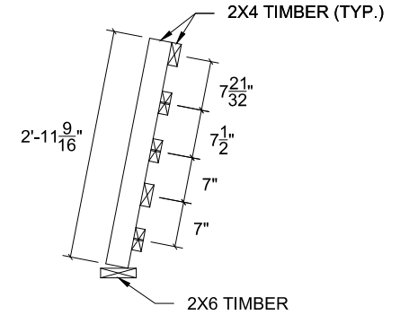
PLYWOOD 5A SIDE ELEVATION VIEW (t = 23/32")
