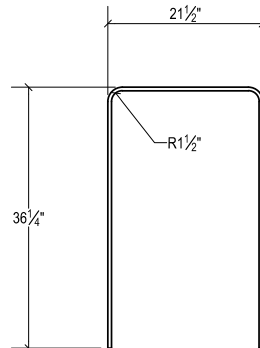
BAR U402 NO. 4 GR. 60 QTY. 2
