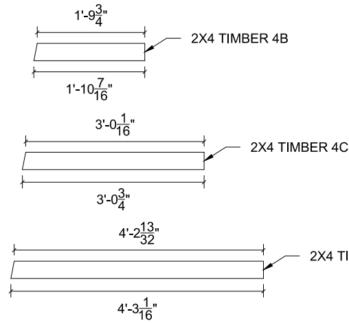
HORIZONTAL 2X4 MEMBERS (4B THROUGH 4D)
