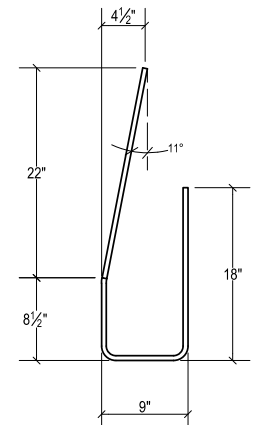
BAR 4V NO.4 QTY. 26
