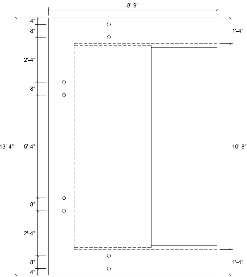
DECK PORTION OF IMPACT SPECIMEN PLAN VIEW
