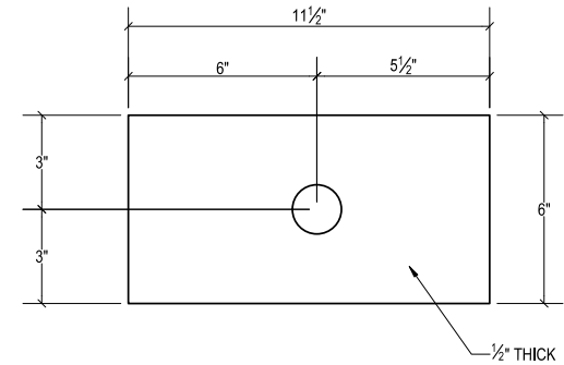
PLATE B BEARING PLATE A572 GR.50 QTY. 2
