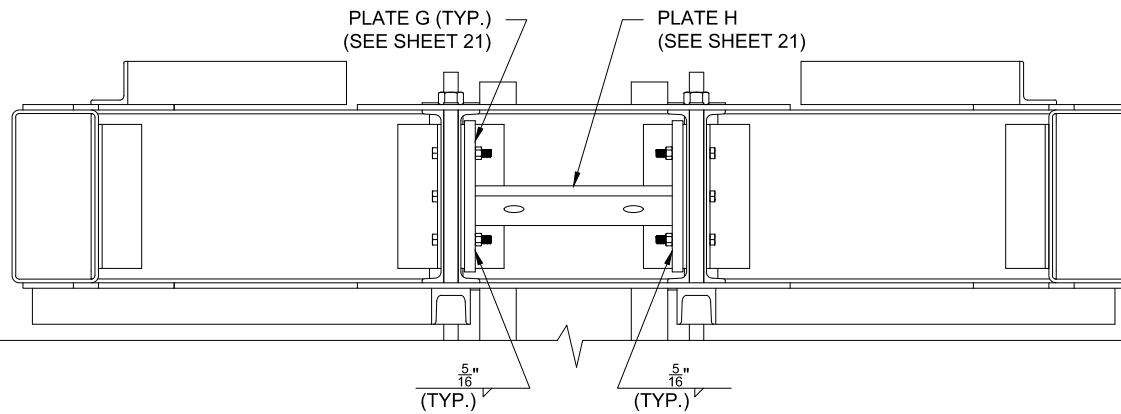
C-17: BACK ELEVATION VIEW OF PULL-BACK CONNECTION
