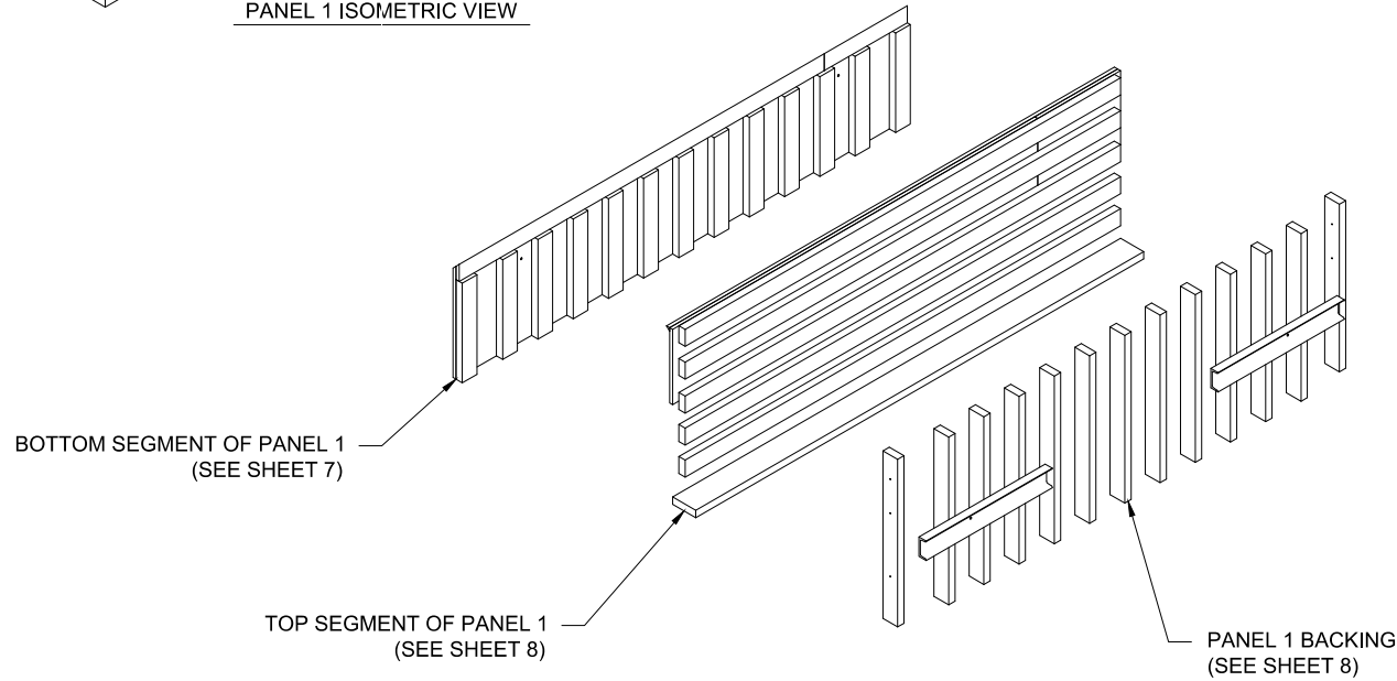
PANEL 1 ISOMETRIC VIEW
