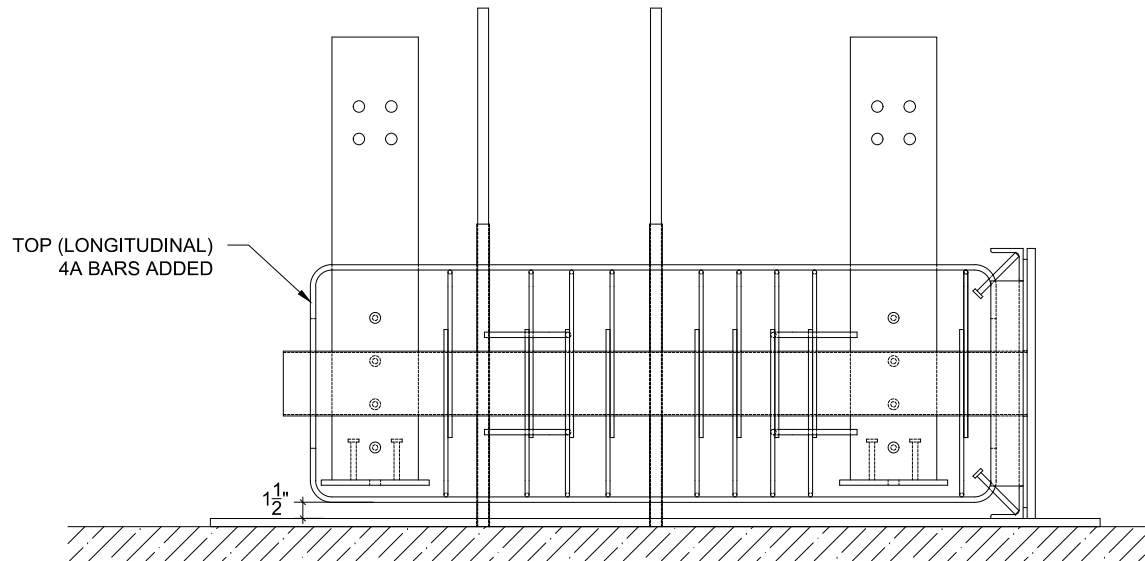
SIDE ELEVATION VIEW (FABRICATION SEQUENCE)
