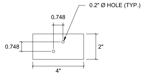
AP4 t = 1/2", ALUMINUM 6061 T6, QTY:2
