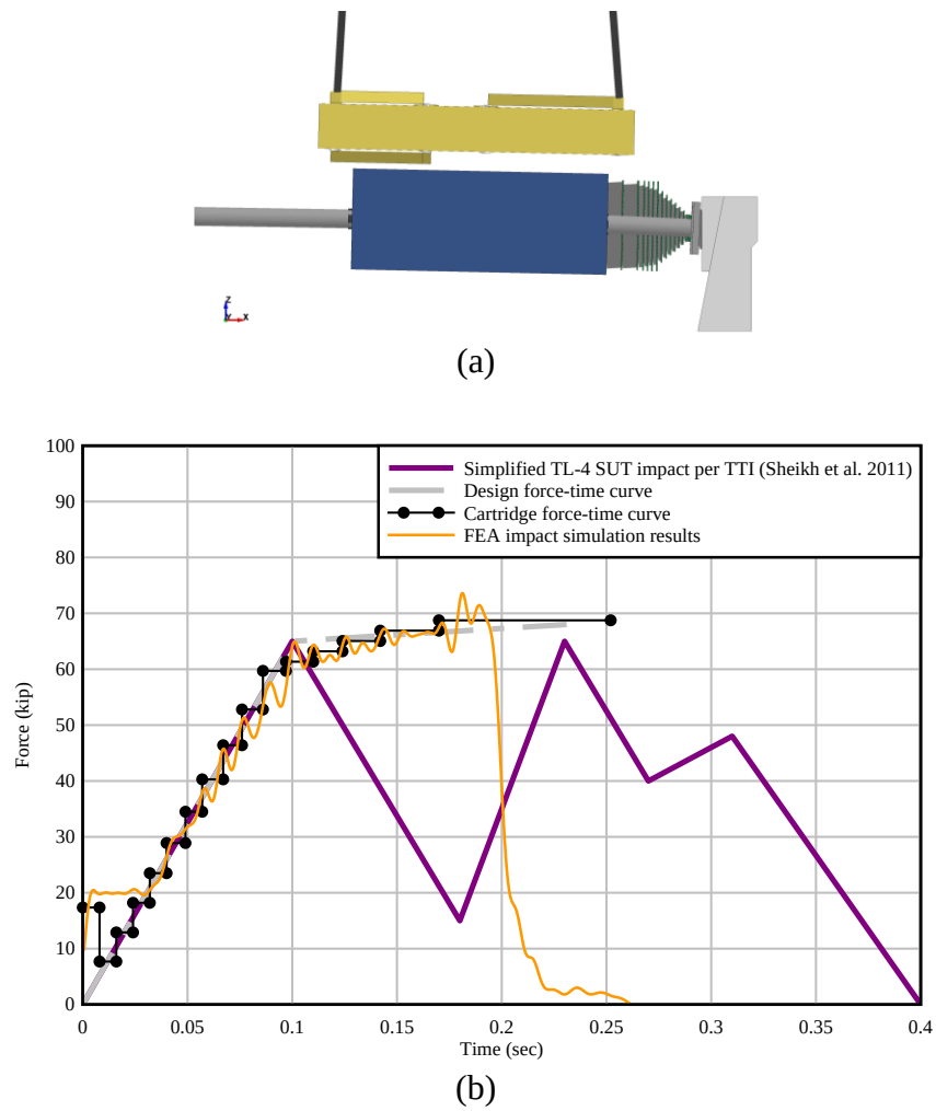
Figure 4.9 FEA impact simulation: (a) Side elevation view at end of impact; (b) Force-time results from FEA impact simulation compared to the (anticipated) force-time curve design
