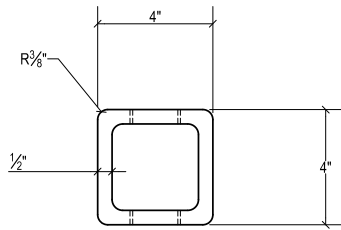
HSS 4X4X1/2 A500 GR.B
