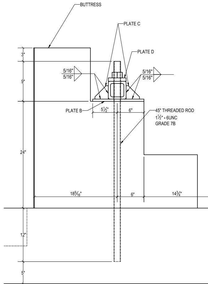
THREADED ROD ANCHOR CONNECTION
