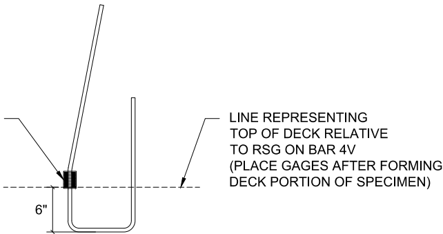
BAR 4V: CONNECTION BAR BETWEEN DECK AND RAIL QTY: 4 BARS EACH WITH 2 RSG (8 TOTAL)
