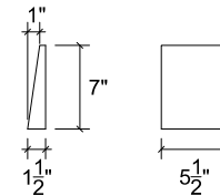
PANEL 3 PLAN VIEW
