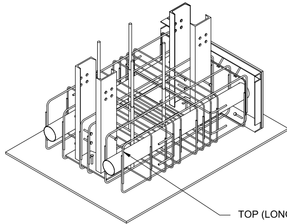
BACK ISOMETRIC VIEW (FABRICATION SEQUENCE)
