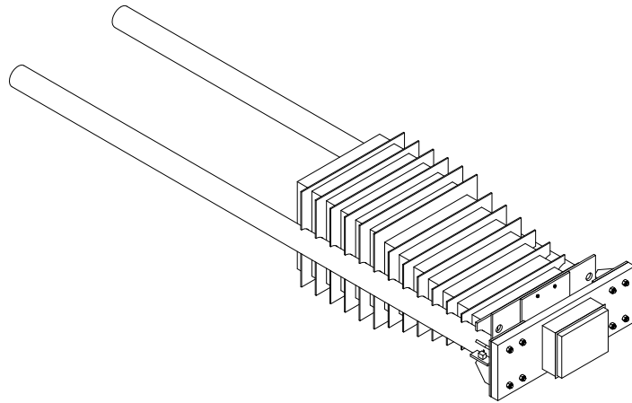
FRONT ISOMETRIC VIEW (FRONT NOSE COMPONENTS)
