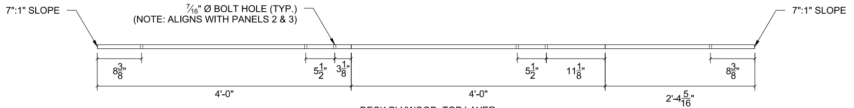
DECK PLYWOOD: TOP LAYER ELEVATION VIEW
