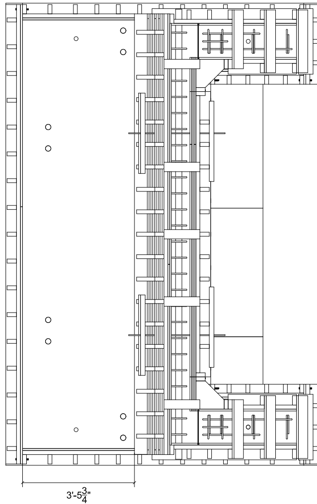
PLAN VIEW RAILING FORMWORK POSITIONED ON DECK
