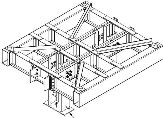
PLATE B WELDED TO C-1 CHANNELS
