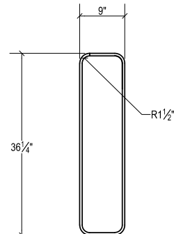
BAR H402 NO. 4 QTY. 4
