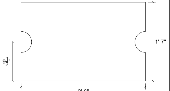
FRP PLATE I t = 1/4", QTY: 1
