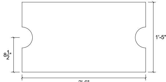
FRP PLATE H t = 1/4", QTY: 1
