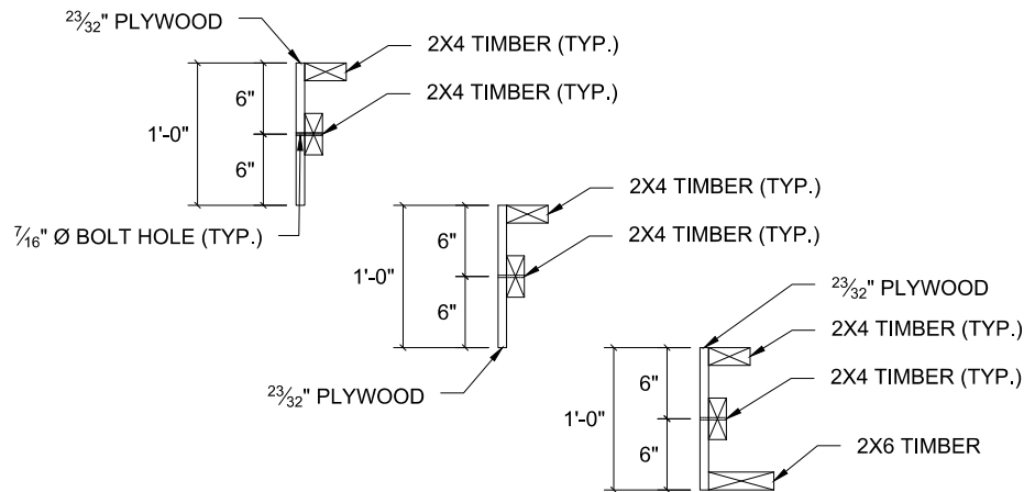
BUTTRESS STEP FORMS SIDE ELEVATION VIEW
