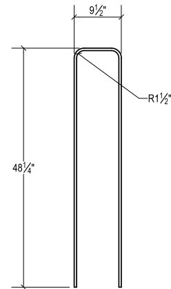
BAR U403 NO. 4 QTY. 2
