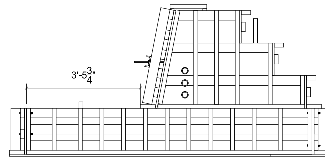
SIDE ELEVATION VIEW RAILING FORMWORK POSITIONED ON DECK
