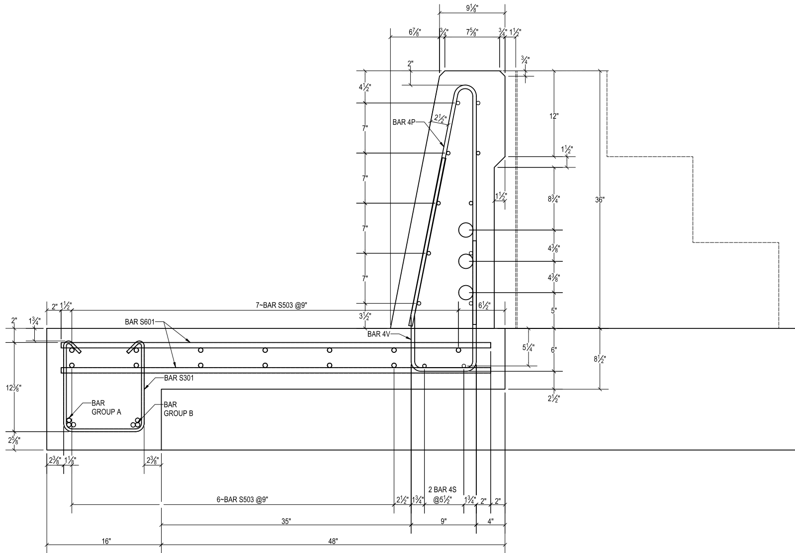
RAIL AND SLAB REINFORCEMENT DETAIL - SECTION B-B
