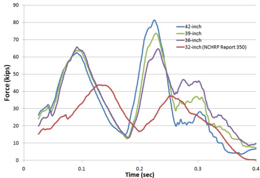
Figure 4.3 FEA impact force-time curves for single-slope traffic railings for various railing heights (after Sheikh et al. 2011)
