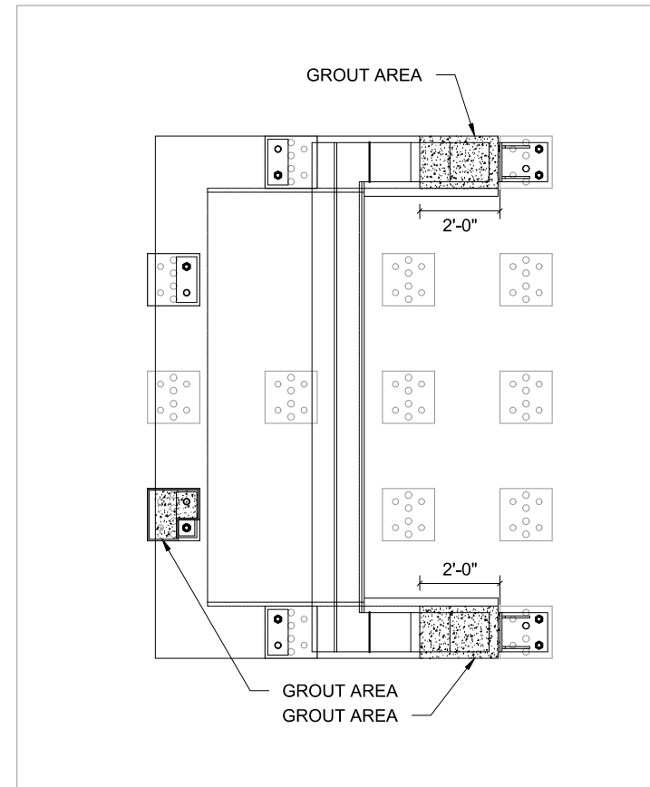
SPECIMEN INSTALLED ONTO FOUNDATION PLAN VIEW
