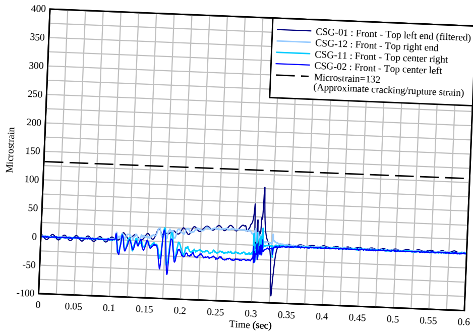
Figure 6.25 External concrete strain gage data for locations on the top front face of the railing during FRC COR test 2
