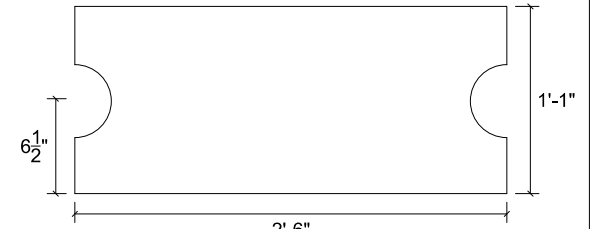
FRP PLATE F t = 1/4", QTY: 1
