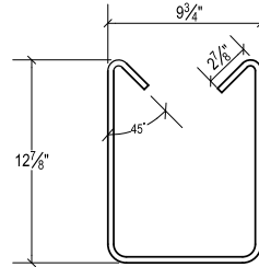
BAR S302 NO.3 QTY. 6
