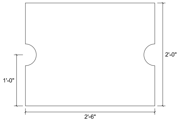
FRP PLATE J t = 1/4", QTY: 6
