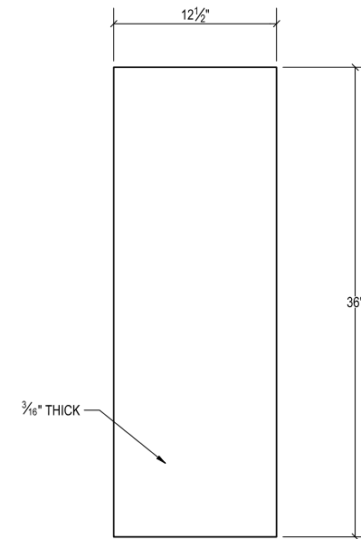
PLATE E STEEL SEPARATION PLATE A36 QTY. 2
