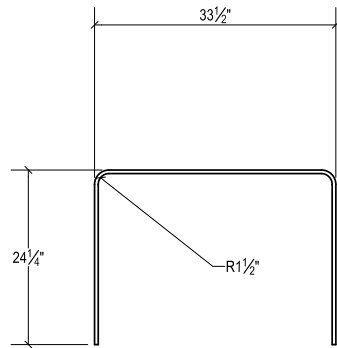
BAR U401 NO. 4 QTY. 2
