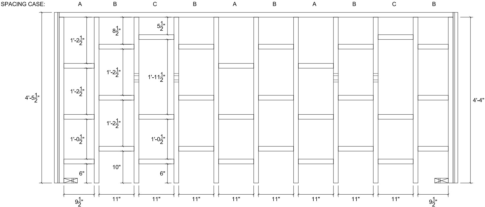
PANEL 1 SPACING PLAN VIEW
