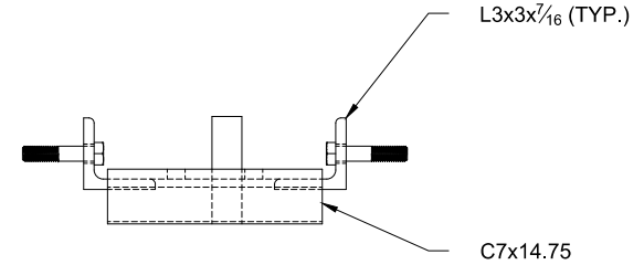
FLOOR CONNECTION HARDWARE ELEVATION VIEW
