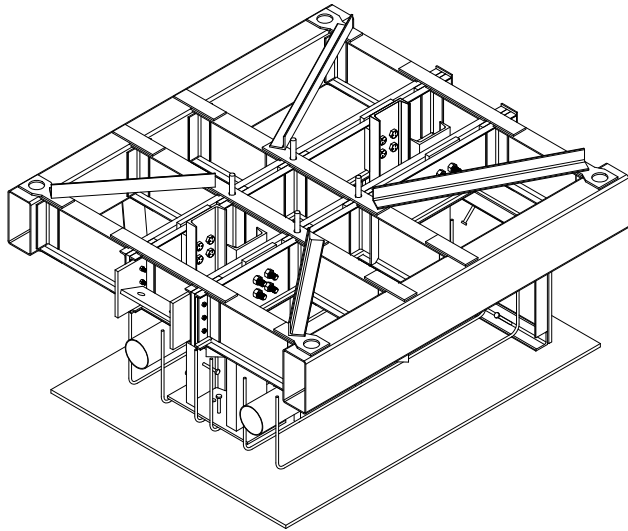
BACK ISOMETRIC VIEW (FABRICATION SEQUENCE)
