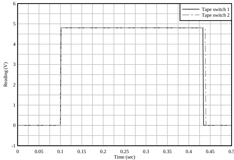
Figure 7.27 Tape switch data for R/C EOR test 1
