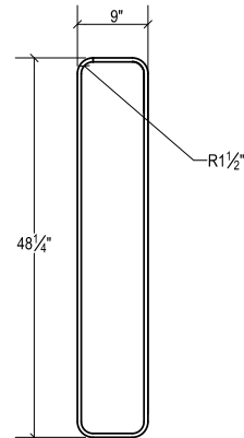
BAR H403 NO. 4 GR. 60 QTY. 4
