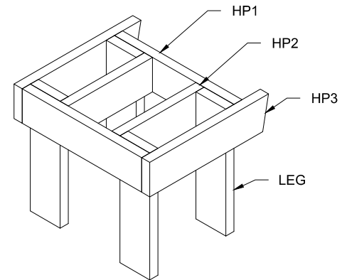
TEMPORARY LOADING WEDGE TABLE ISOMETRIC VIEW: PLYWOOD REMOVED
