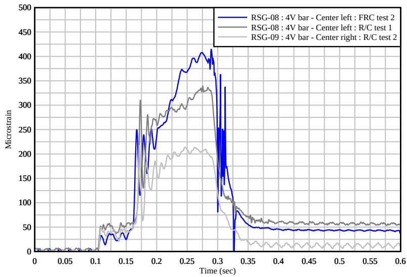
Figure 6.70 Comparison of internal strain gauges located on the railing connection rebar
