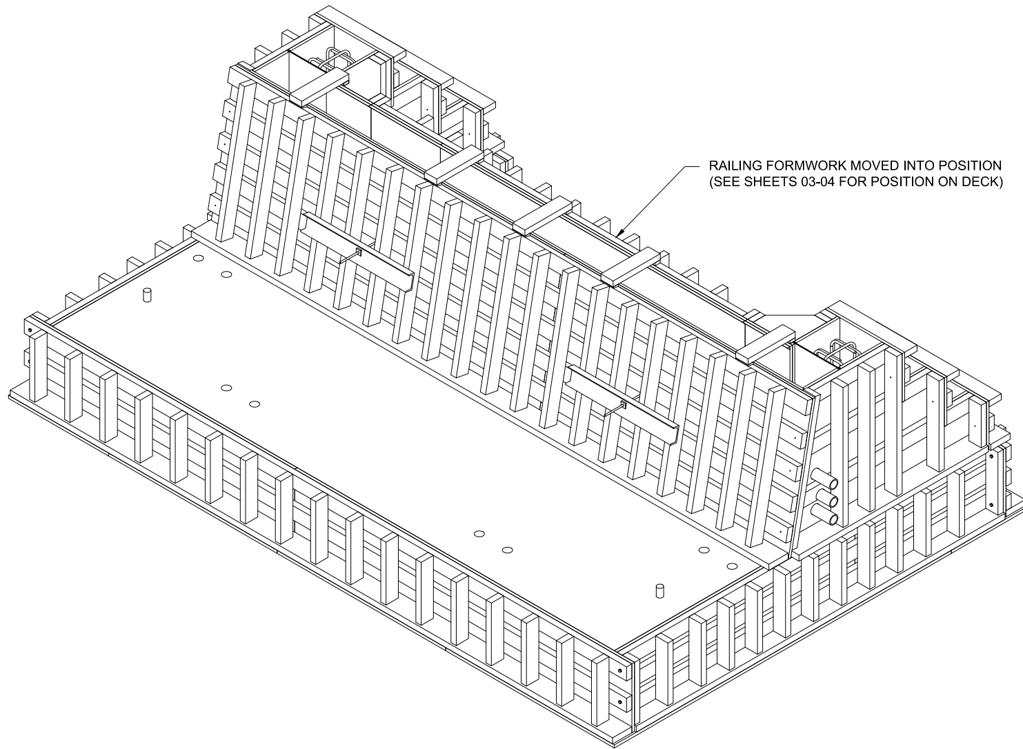
ISOMETRIC VIEW AFTER DECK CONCRETE PLACEMENT
