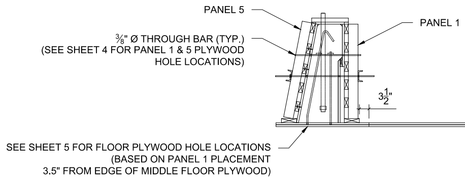
SIDE ELEVATION VIEW (ONLY PANELS 1 & 5 SHOWN FOR CLARITY)
