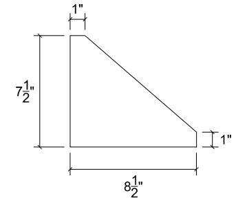
SSP-3 t = \frac{5}{8} ", A572-50, QTY: 4
