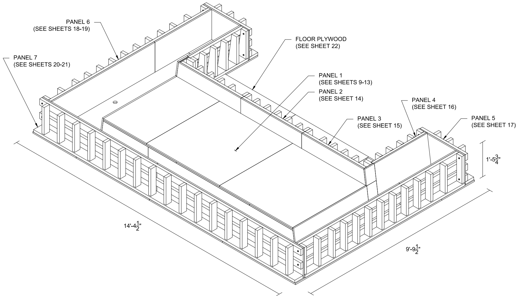
DECK FORMWORK FRONT ISOMETRIC VIEW
