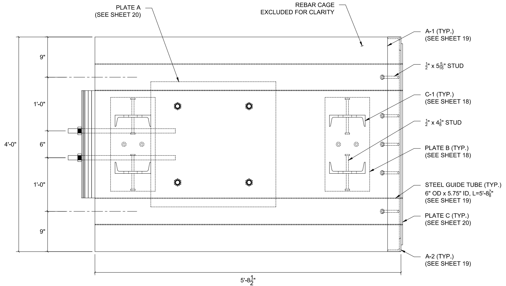
PLAN VIEW (BACK BLOCK COMPONENTS, REBAR CAGE EXCLUDED)
