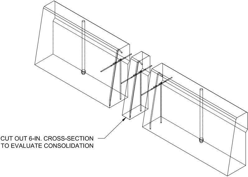
ISOMETRIC VIEW (WITH EMBEDDED BARS SHOWN)
