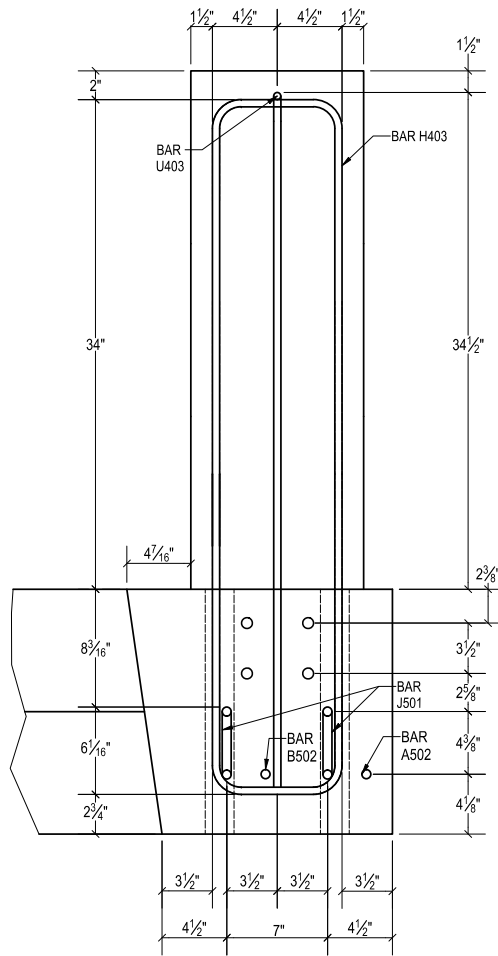
BUTTRESS REINFORCEMENT SECTION D-D
