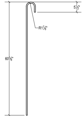
BAR J501 NO. 5 GR. 60 QTY. 4
