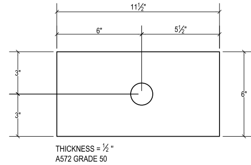
PLATE B BEARING PLATE QTY. 2
