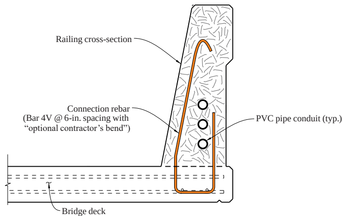
Figure 5.5 FRC 36-in. single-slope traffic railing
