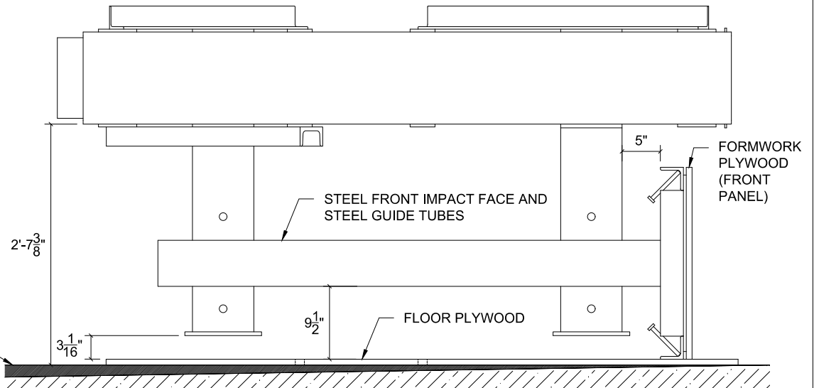
SIDE ELEVATION VIEW (FABRICATION SEQUENCE)
