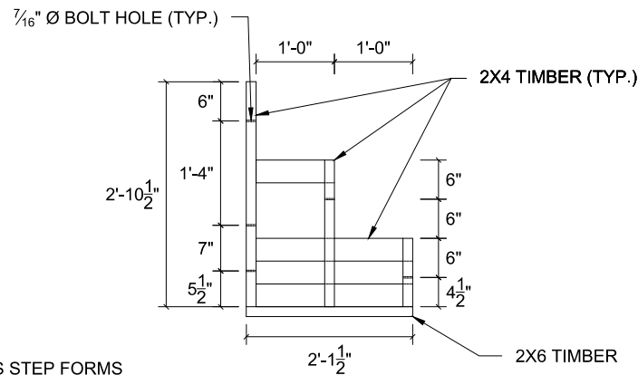
TIMBER FRAME SIDE ELEVATION VIEW
