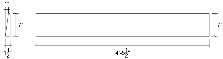
1B: SLOPED 2x8 QTY: 2
