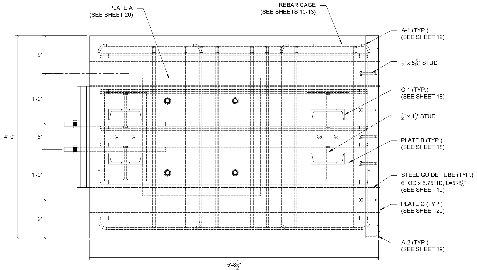
PLAN VIEW (BACK BLOCK COMPONENTS)
