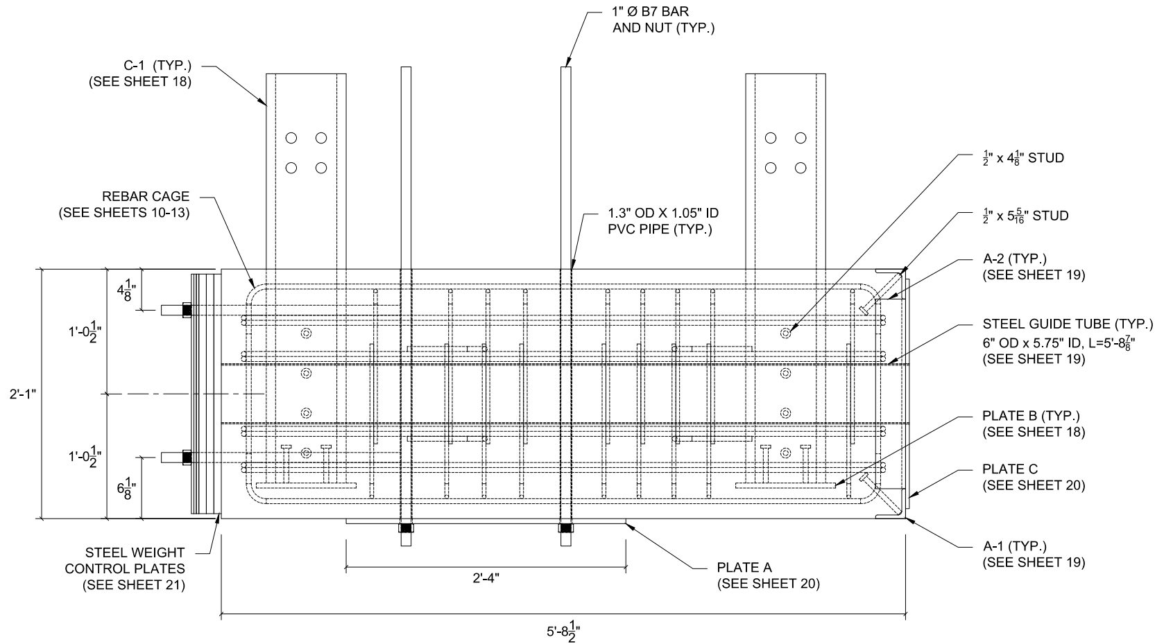
SIDE ELEVATION VIEW (BACK BLOCK COMPONENTS)
