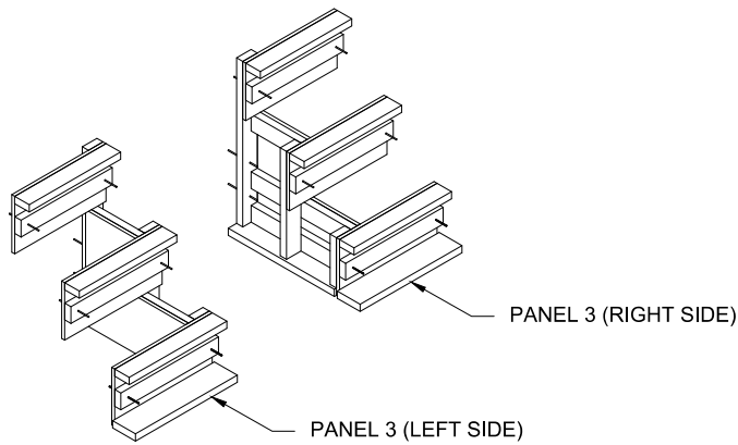
PANEL 3 ISOMETRIC VIEW
