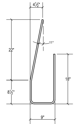
BAR 4V NO.4 GR.60 QTY. 16
