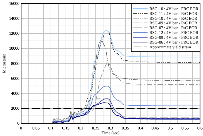
Figure 7.45 Comparison of internal strain gauges located on the railing connection rebar
