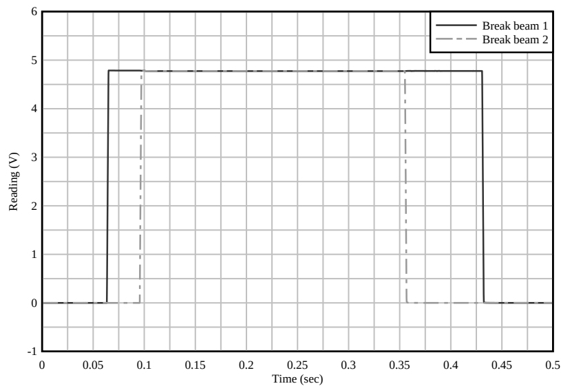
Figure 6.34 Break beam data for R/C COR test 1
