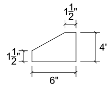
AP3 t = 1/2", ALUMINUM 6061 T6, QTY:4
