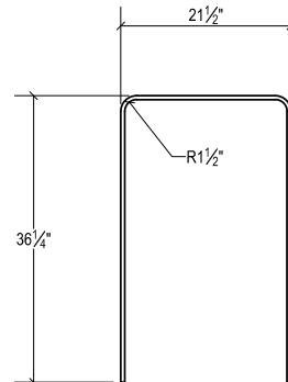
BAR U402 NO. 4 QTY. 2
