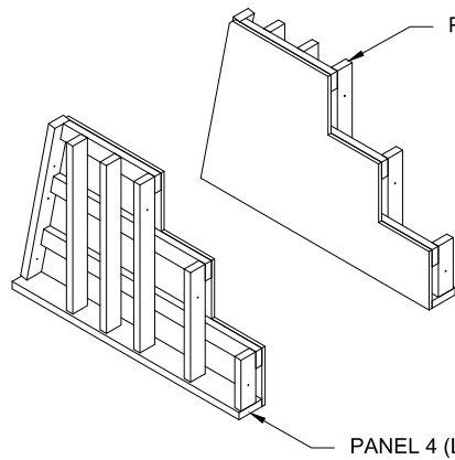
PANEL 4 ISOMETRIC VIEW
