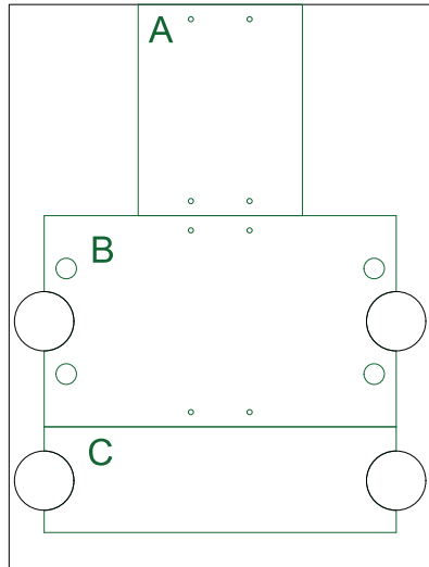
FRP PLATE CUTTING PLAN PLATES A-C, t = \frac{1}{2} "
