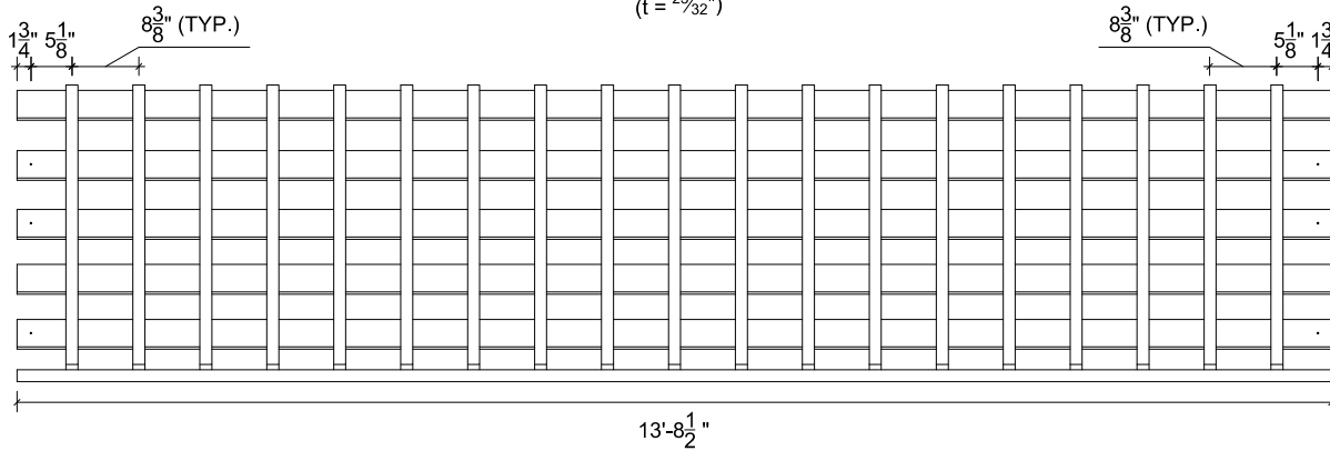
TIMBER FRAME FRONT ELEVATION VIEW
