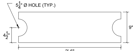
FRP PLATE D t = 1/4", QTY: 1
