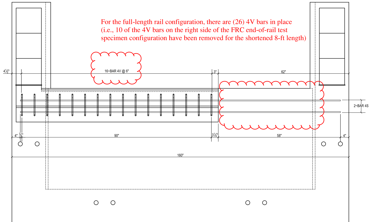
RAIL REINFORCEMENT (PLAN VIEW)
