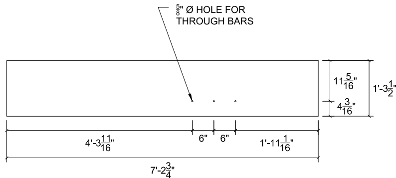
PANEL 1 TOP SEGMENT PLYWOOD BACK ELEVATION VIEW (t = 23/32")
