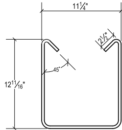
BAR S301 NO.3 QTY. 24
