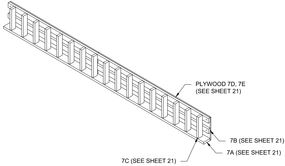
PANEL 7 ISOMETRIC VIEW
