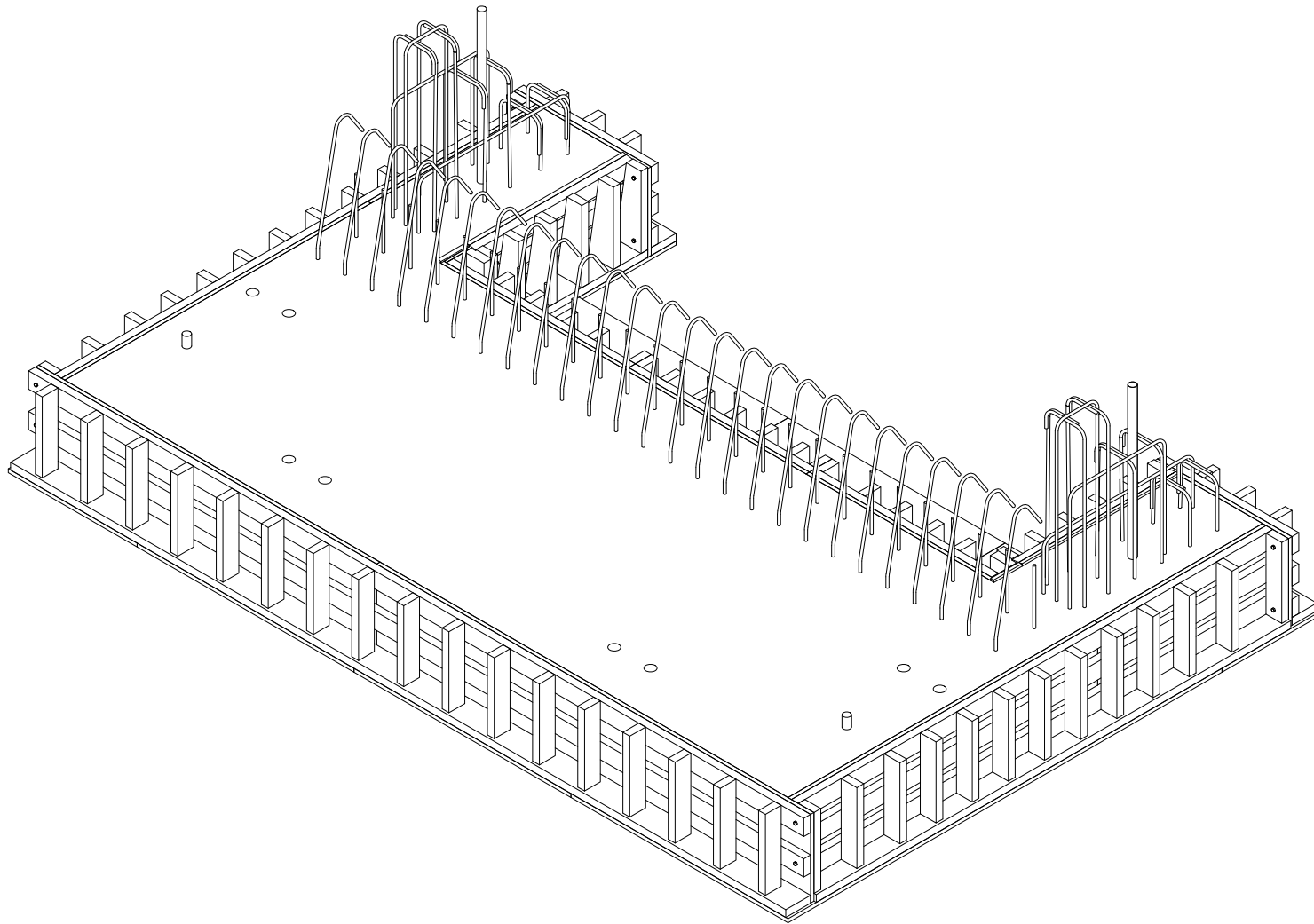
ISOMETRIC VIEW AFTER DECK CONCRETE PLACEMENT
