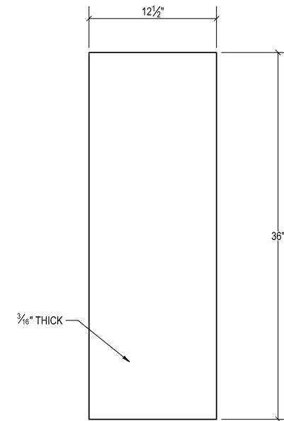
PLATE E STEEL SEPARATION PLATE QTY. 2
