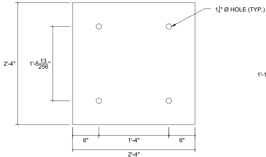
PLATE A t = 1/2", A572-50, QTY: 1
