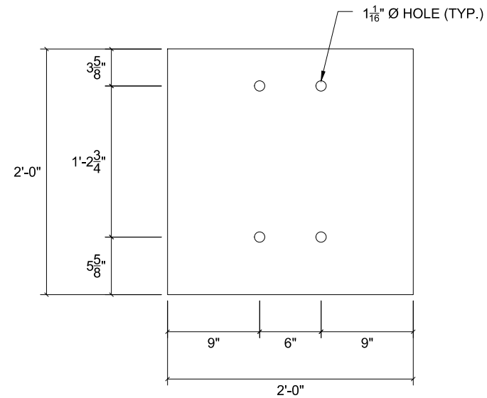
STEEL WEIGHT CONTROL PLATES
