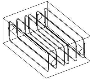
ISOMETRIC VIEW: 4A BARS
