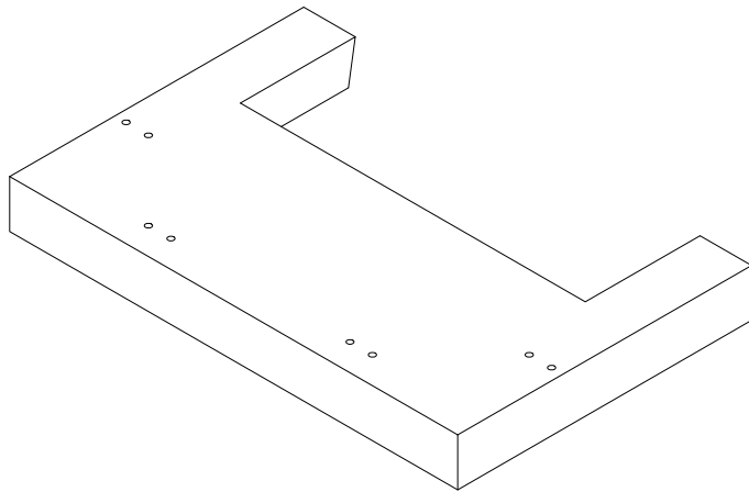
DECK PORTION OF IMPACT SPECIMEN FRONT ISOMETRIC VIEW
