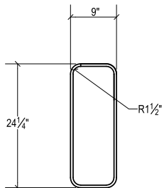
BAR H401 NO. 4 QTY. 4
