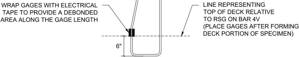
BAR 4V: CONNECTION BAR BEWTEEN DECK AND RAIL QTY: 4 BARS EACH WITH 2 RSG (8 TOTAL)
