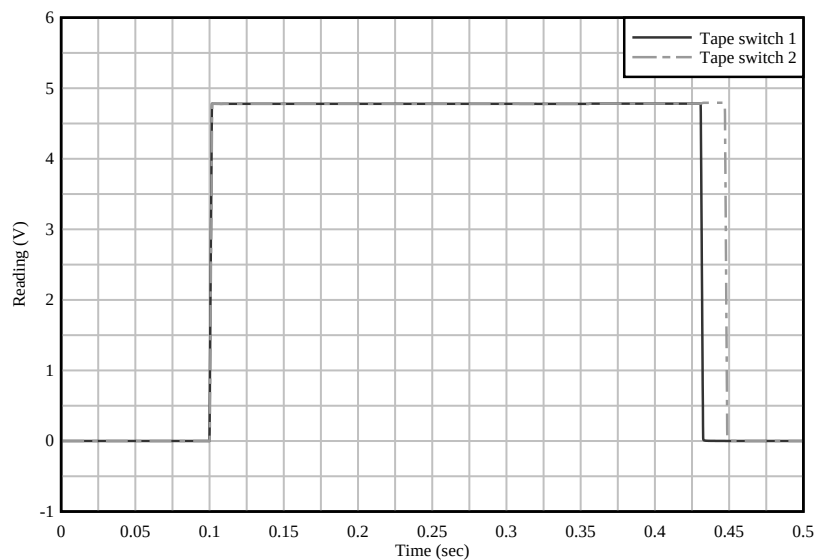
Figure 6.35 Tape switch data for R/C COR test 1
