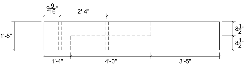
DECK PORTION OF IMPACT SPECIMEN SIDE ELEVATION VIEW
