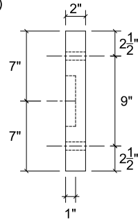
AP1: SIDE ELEVATION VIEW t = 2", ALUMINUM 6061 T6, QTY:1
