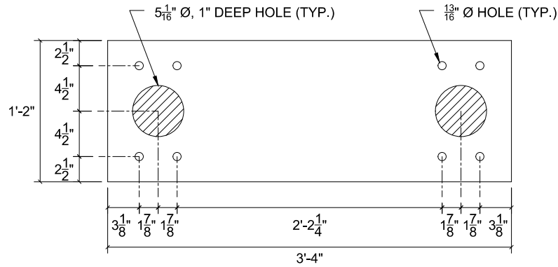
AP1: BACK ELEVATION VIEW t = 2", ALUMINUM 6061 T6, QTY:1
