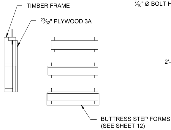
PANEL 3 TOP VIEW OF COMPONENTS (RIGHT SIDE)
