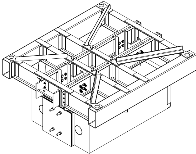
BACK ISOMETRIC VIEW (FABRICATION SEQUENCE)
