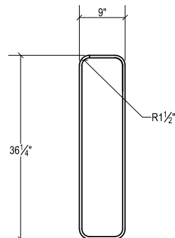
BAR H402 NO. 4 GR. 60 QTY. 4
