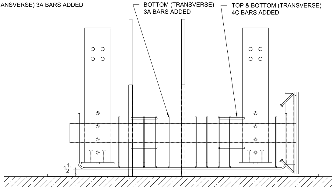
SIDE ELEVATION VIEW (FABRICATION SEQUENCE)
