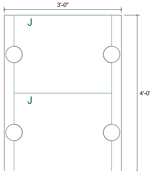
FRP PLATE CUTTING PLAN PLATES D-J, t = \frac{1}{4} "
