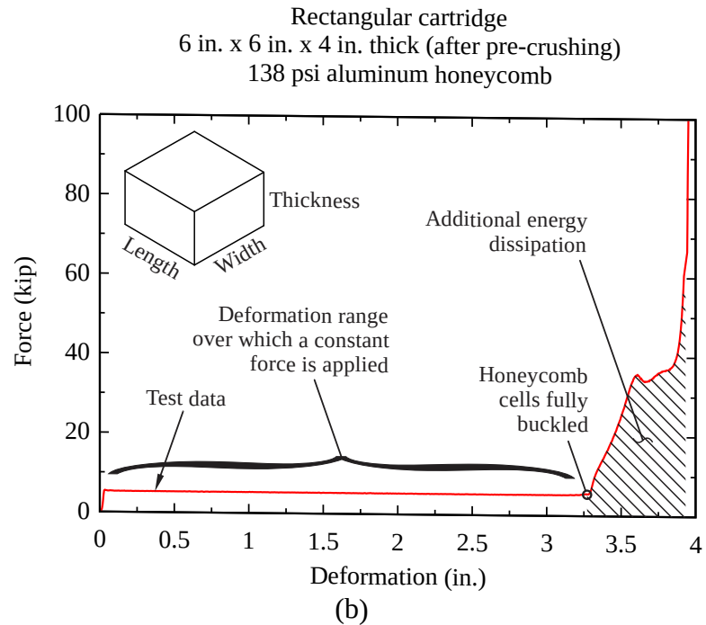
Figure 4.4 Aluminum honeycomb: (a) Cell structure and crush sequence of rectangular cartridge; (b) Force-deformation curve for an individual rectangular aluminum honeycomb cartridge (after Groetaers et al. 2016)
