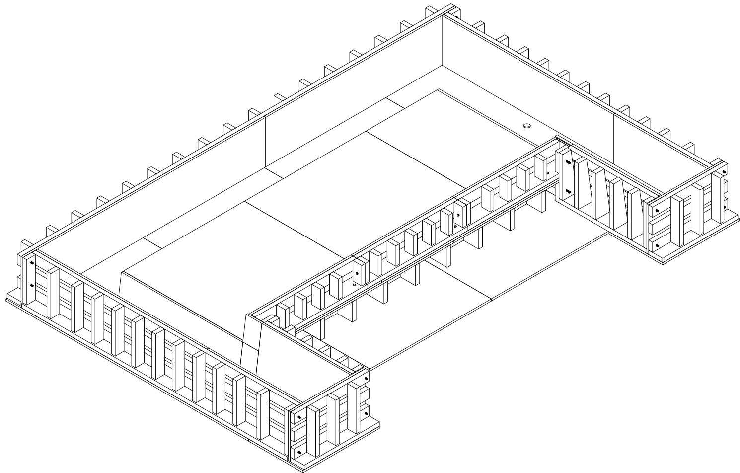
DECK FORMWORK BACK ISOMETRIC VIEW
