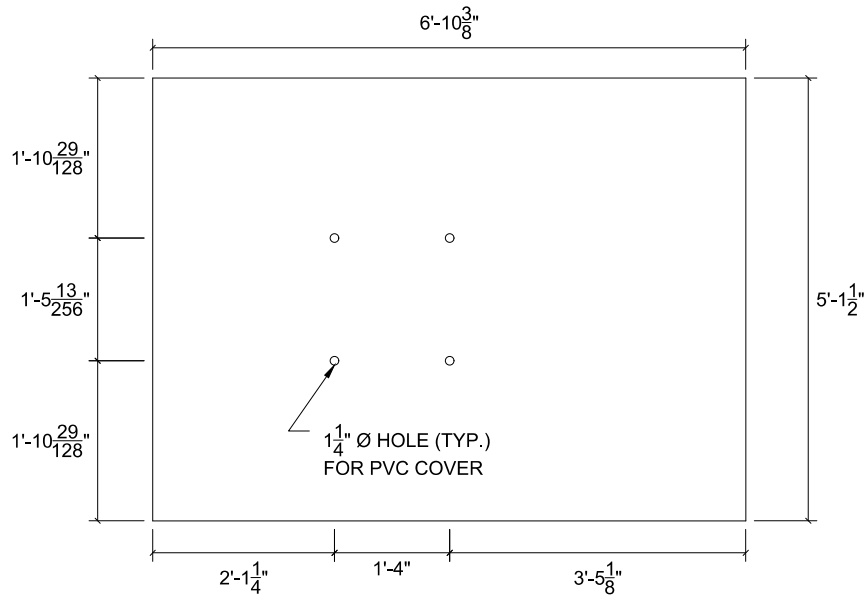
FLOOR PLYWOOD t = 3/4", QTY: 1
