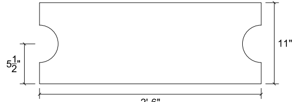
FRP PLATE E t = 1/4", QTY: 1
