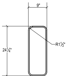
BAR H401 NO. 4 GR. 60 QTY. 4
