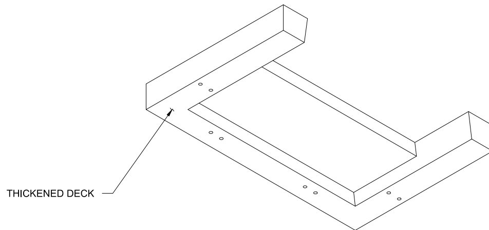
DECK PORTION OF IMPACT SPECIMEN BOTTOM ISOMETRIC VIEW
