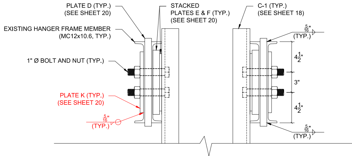
B-16: FRONT ELEVATION VIEW OF CONNECTION (BACK BLOCK CONNECTION TO HANGER FRAME)
