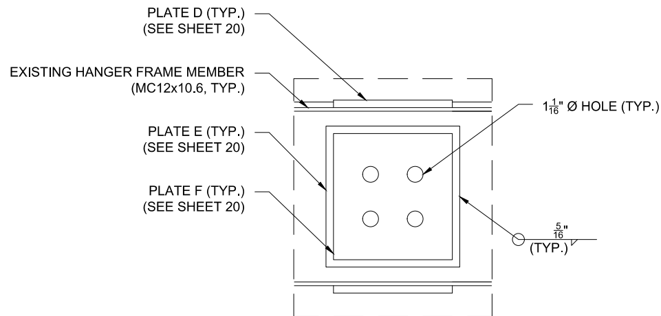
B-16: FRONT ELEVATION VIEW OF CONNECTION (BACK BLOCK CONNECTION TO HANGER FRAME)
