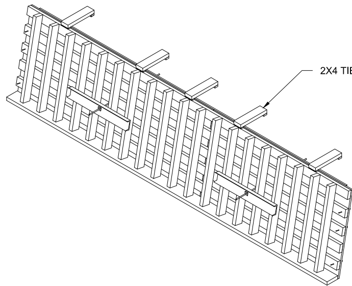
PANEL 5 ISOMETRIC VIEW
