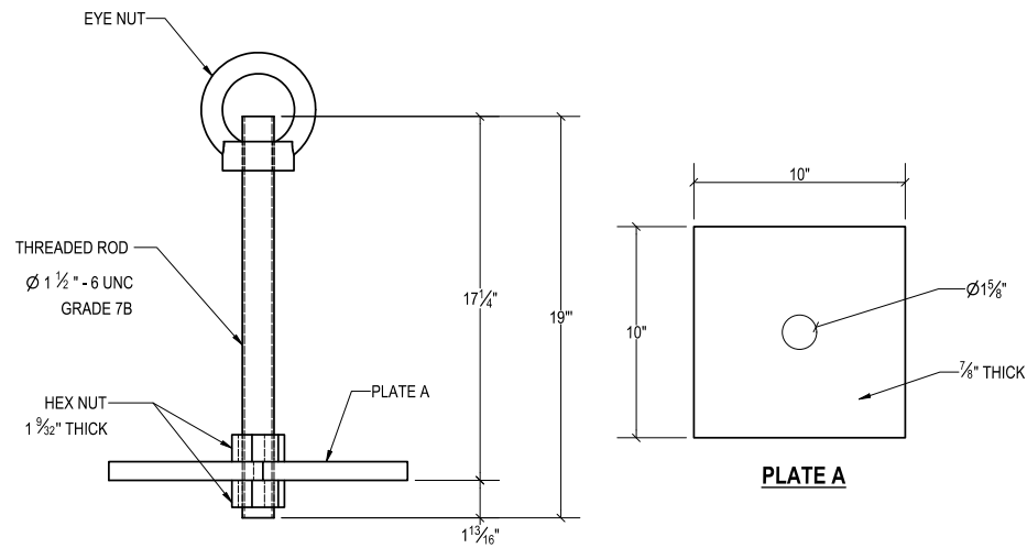
ANCHOR AND PLATE CONNECTION
