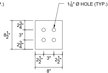
PLATE F t = 5/16", A572-50, QTY: 4
