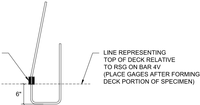
BAR 4V: CONNECTION BAR BEWTEEN DECK AND RAIL QTY: 4 BARS EACH WITH 2 RSG (8 TOTAL)
