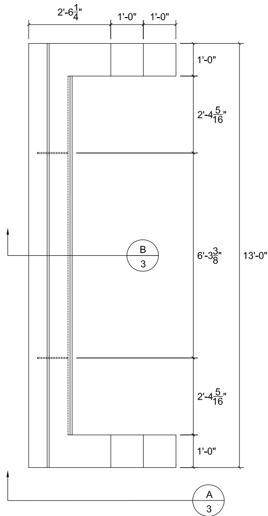
PLAN VIEW OF CONCRETE RAILING SPECIMEN
