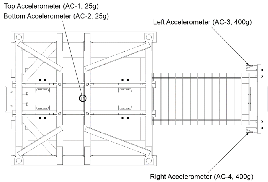
Figure 5.26 Accelerometers installed on pendulum impactor (top view)
