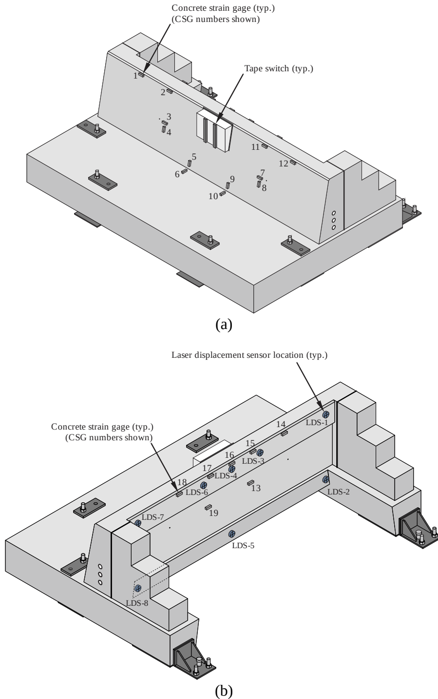
Figure 5.23 External instrumentation: (a) Front concrete strain gage and tape switch sensor locations; (b) Back concrete strain gage and laser displacement sensor locations
