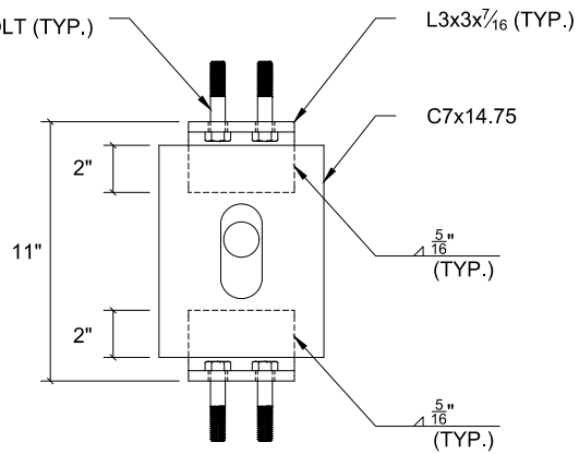
FLOOR CONNECTION HARDWARE PLAN VIEW
