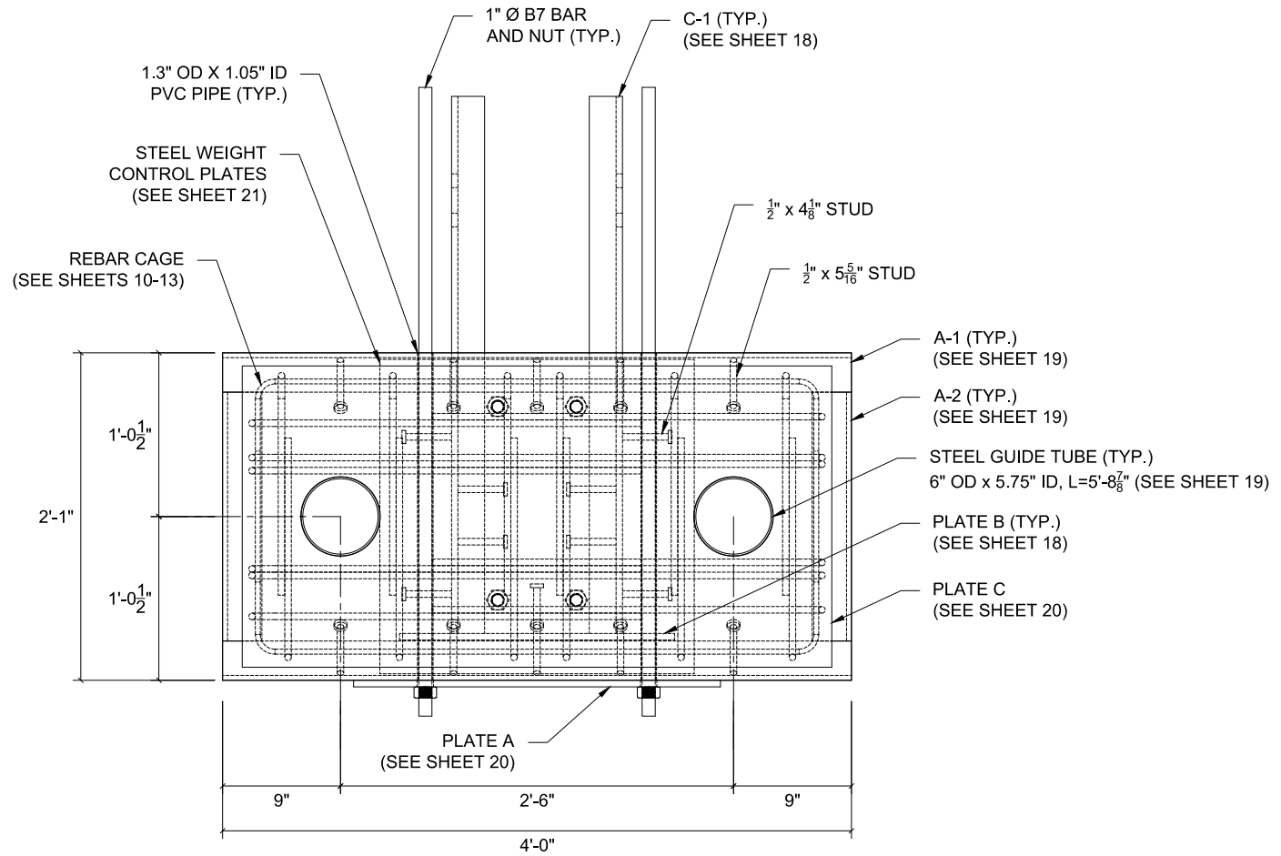
FRONT ELEVATION VIEW (BACK BLOCK COMPONENTS)
