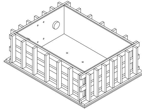
FRONT ISOMETRIC VIEW (BACK BLOCK FORMWORK)
