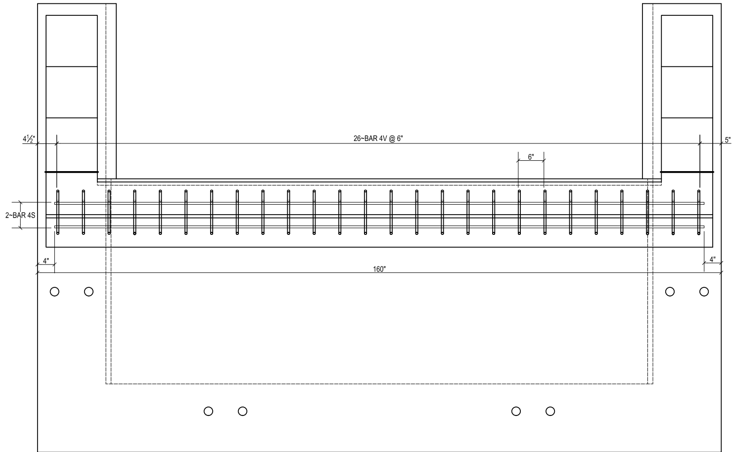
RAIL REINFORCEMENT (PLAN VIEW)
