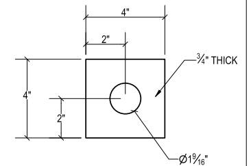
PLATE D SQUARE PLATE A572 GR.50 QTY. 4
