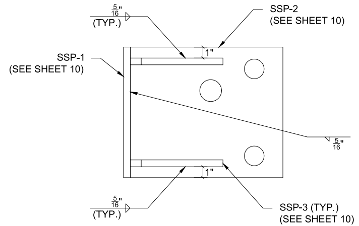
SLIDE STOPPER PLAN VIEW
