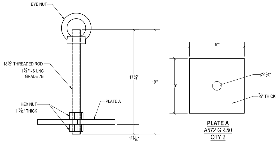
ANCHOR AND PLATE CONNECTION
