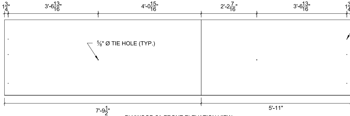
PLYWOOD 5A FRONT ELEVATION VIEW (t = 23/32")
