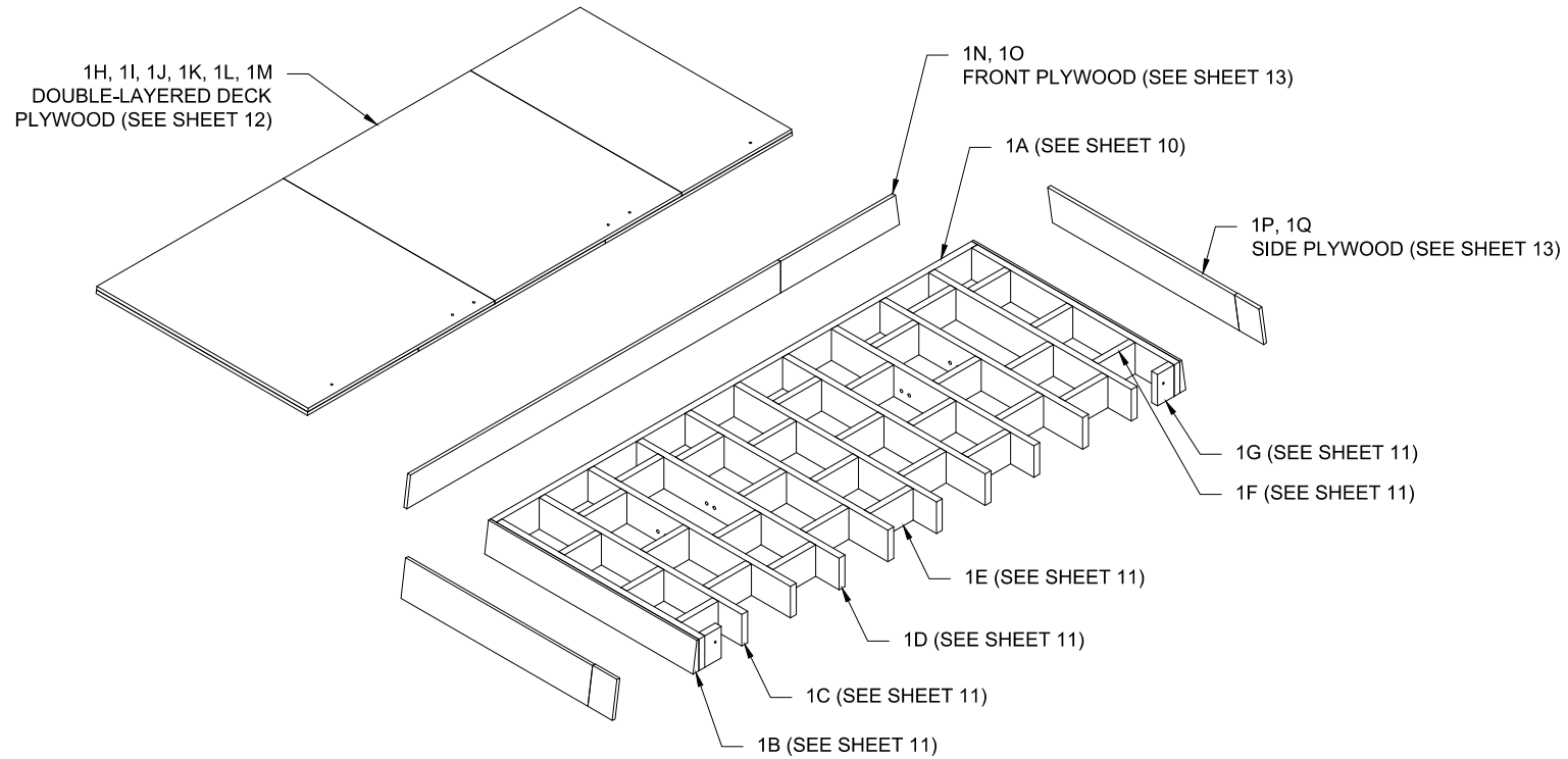
PANEL 1 BACK ISOMETRIC VIEW OF COMPONENTS
