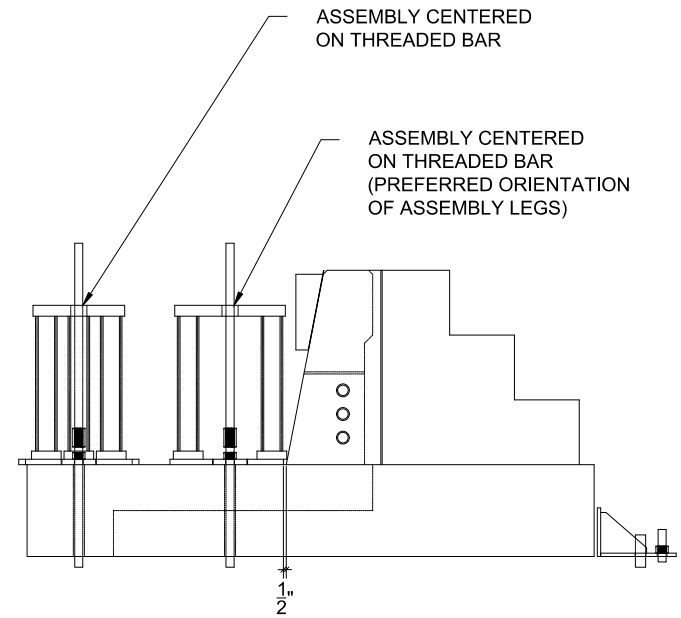
ANCHORED IMPACT SPECIMEN SIDE ELEVATION VIEW
