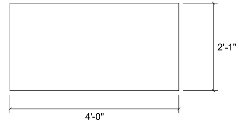
FRONT PANEL PLYWOOD t = 3/4", QTY: 1
