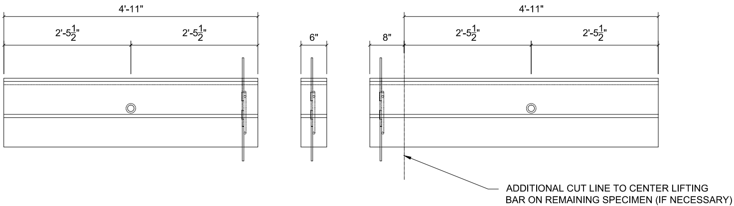
TOP VIEW (WITH EMBEDDED BARS SHOWN)
