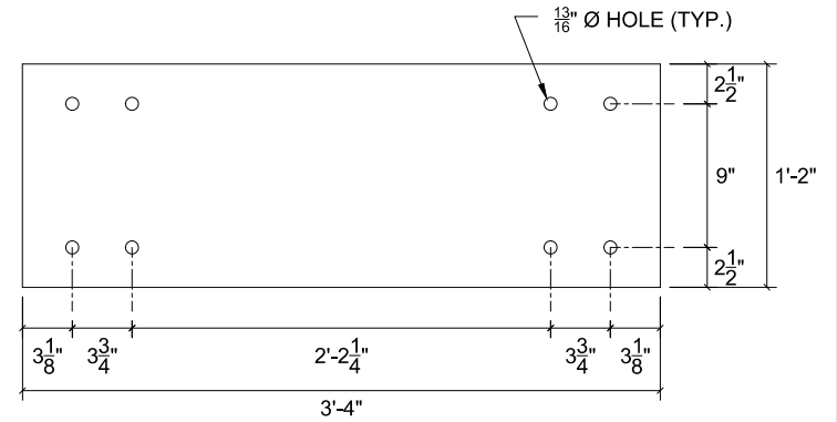
AP1: FRONT ELEVATION VIEW t = 2", ALUMINUM 6061 T6, QTY:1
