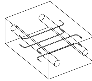
ISOMETRIC VIEW: 4C BARS
