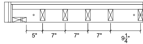
PANEL 3 PLAN VIEW
