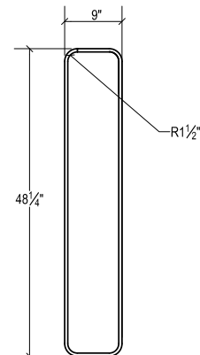
BAR H403 NO. 4 GR. 60 QTY. 4
