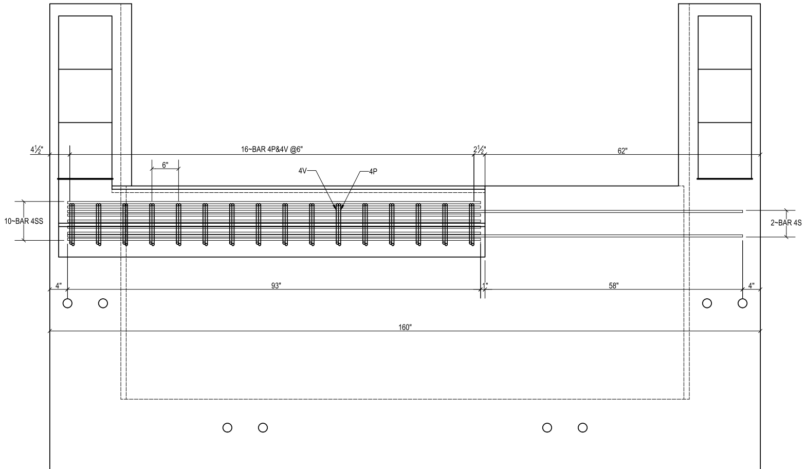
RAIL REINFORCEMENT (PLAN VIEW)
