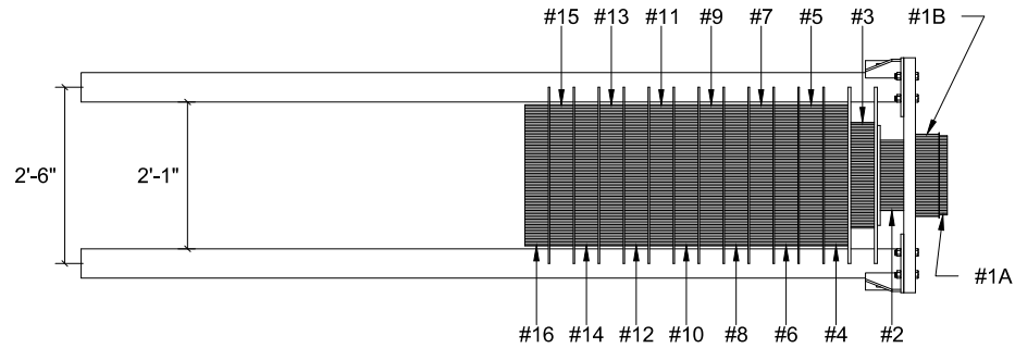
PLAN VIEW (CARTRIDGE NUMBERING)
