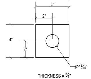
PLATE D SQUARE PLATE QTY. 4
