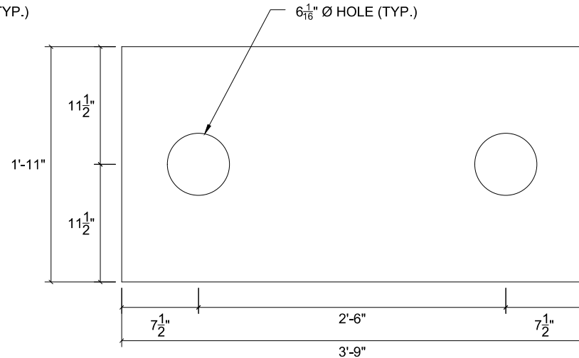
PLATE C t = 3/8", A572-50, QTY: 1
