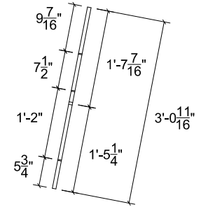
PLYWOOD 5A SIDE ELEVATION VIEW (t = 23/32")
