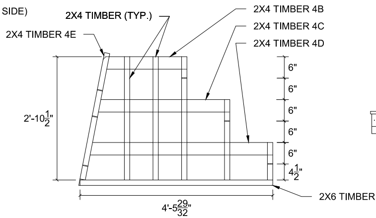
PANEL 4 SIDE ELEVATION VIEW (LEFT SIDE)
