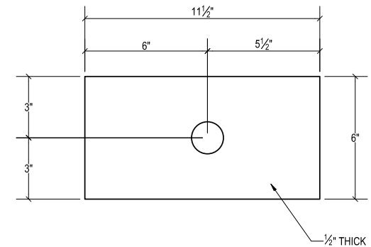
PLATE B BEARING PLATE A572 GR.50 QTY. 2
