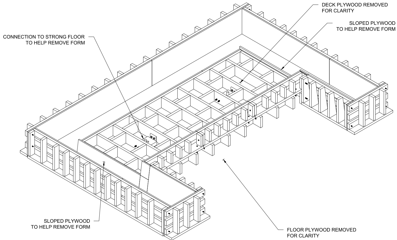
DECK FORMWORK BACK ISOMETRIC VIEW
