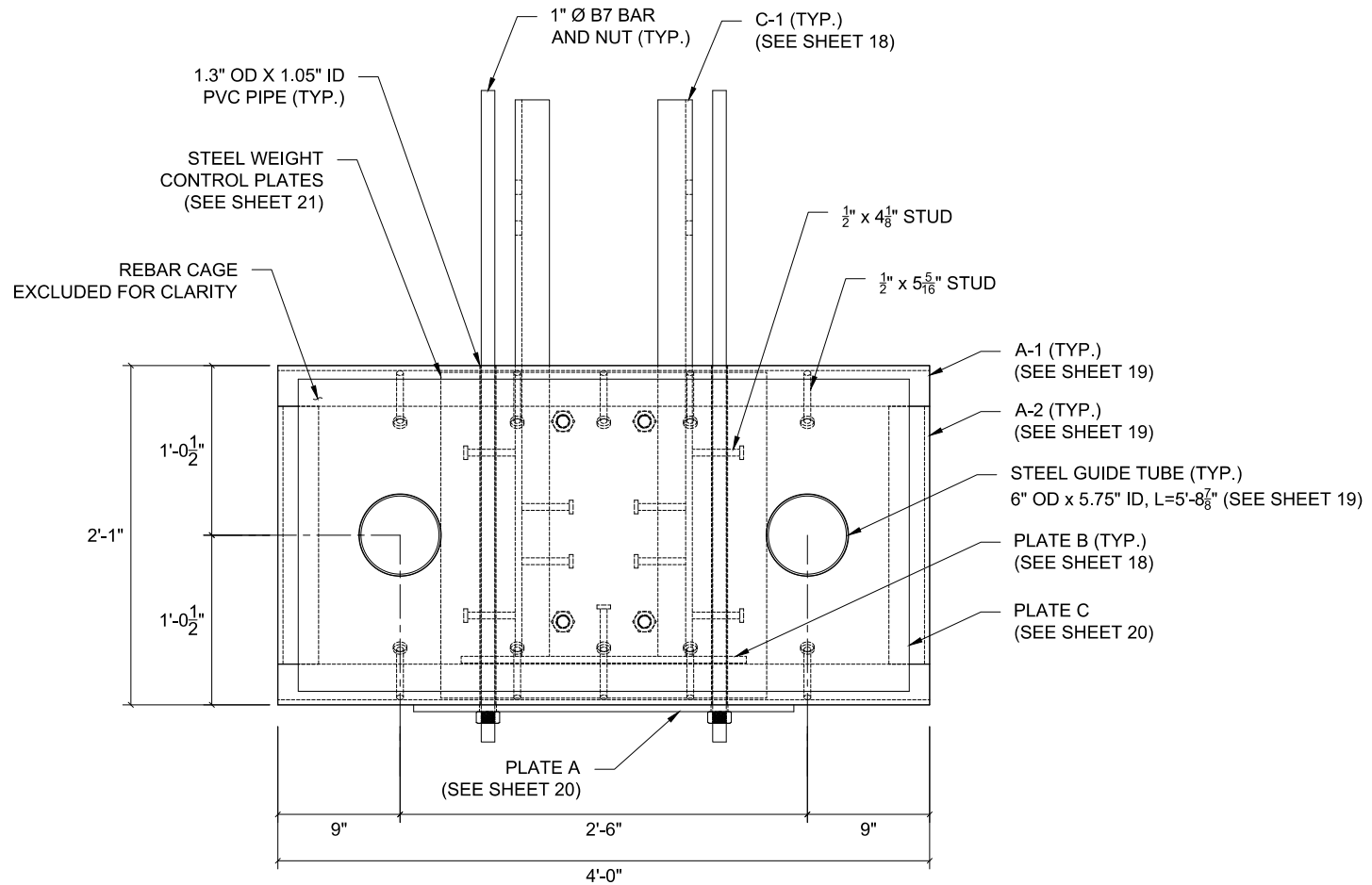
FRONT ELEVATION VIEW (BACK BLOCK COMPONENTS, REBAR CAGE EXCLUDED)
