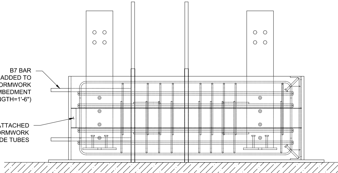
SIDE ELEVATION VIEW (FABRICATION SEQUENCE)
