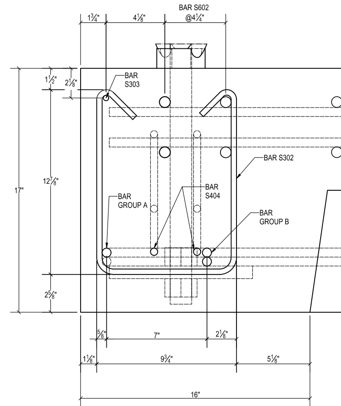
THICKENED EDGE SECTION C-C
