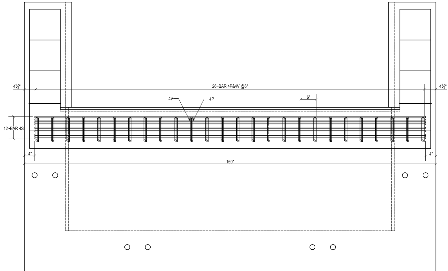
RAIL REINFORCEMENT (PLAN VIEW)
