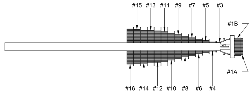
SIDE ELEVATION VIEW (CARTRIDGE NUMBERING)
