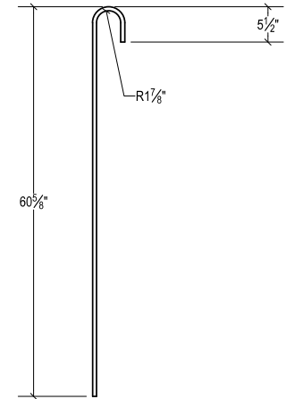
BAR J501 NO. 5 QTY. 4
