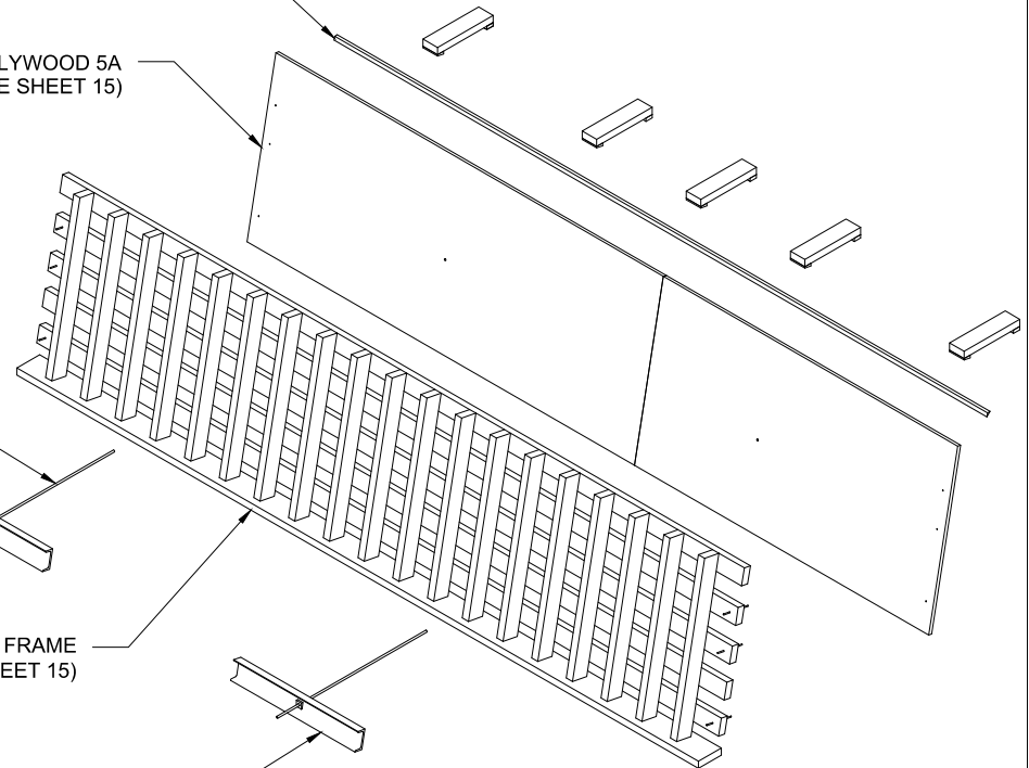
PANEL 5 ISOMETRIC VIEW OF COMPONENTS
