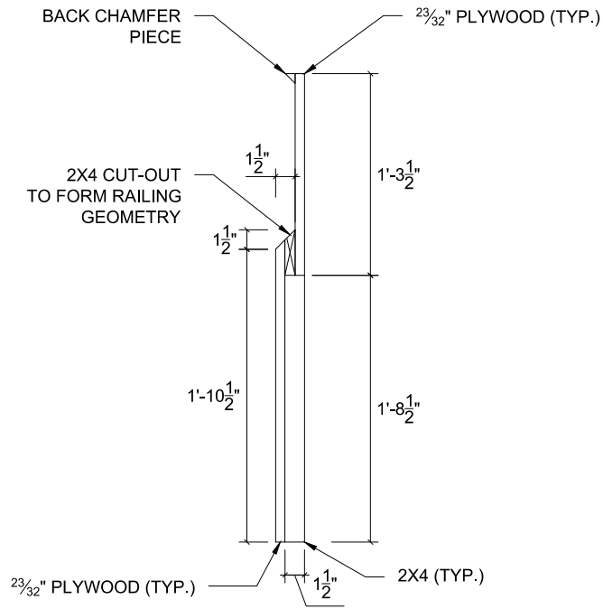
PANEL 2 BACK SEGMENT SIDE ELEVATION VIEW
