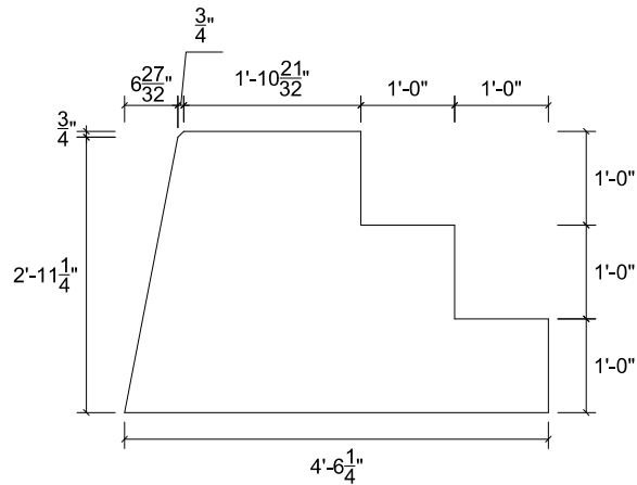
PLYWOOD 4A (t = 2 3/32")
