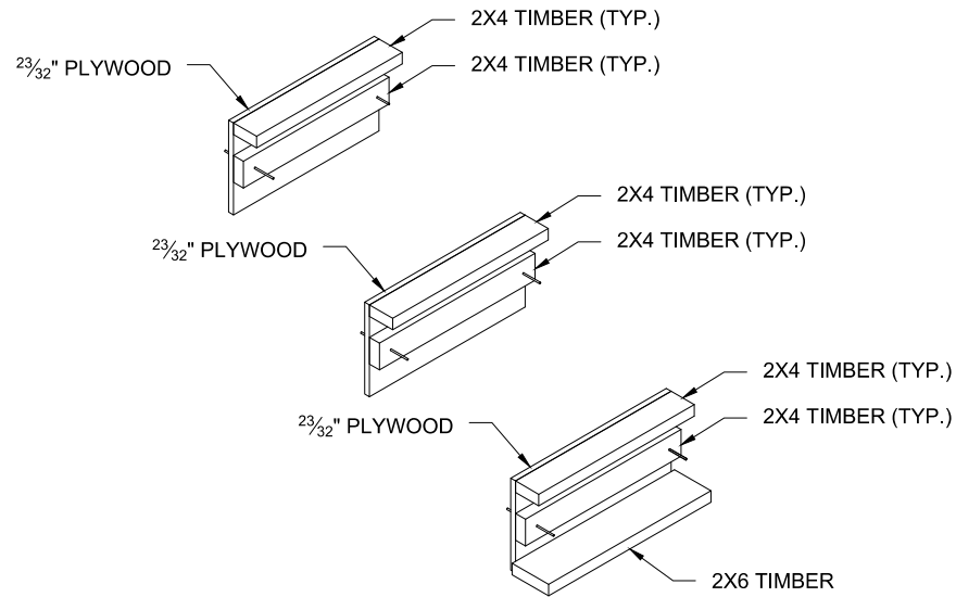
BUTTRESS STEP FORMS ISOMETRIC VIEW
