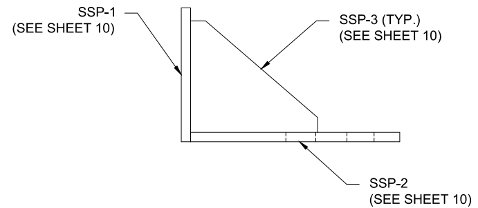
SLIDE STOPPER SIDE ELEVATION VIEW
