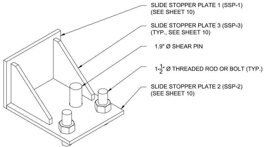
SLIDE STOPPER (QTY: 2) BACK ISOMETRIC VIEW
