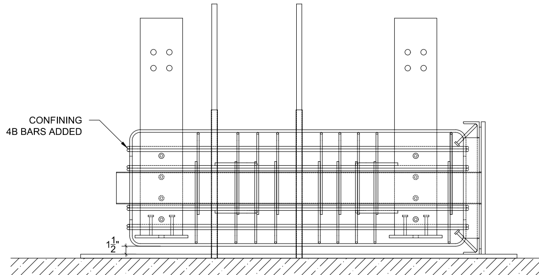
SIDE ELEVATION VIEW (FABRICATION SEQUENCE)
