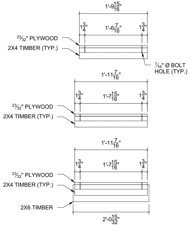
BUTTRESS STEP FORMS TOP VIEW
