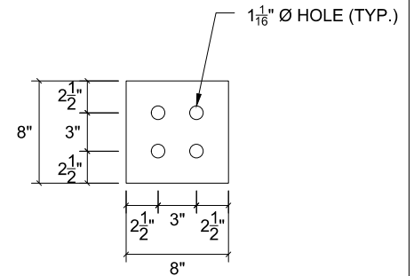
PLATE K t = 1/2", A572-50, QTY: 4
