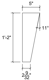
ALUMINUM LOADING WEDGE: SIDE ELEVATION VIEW t = 5", ALUMINUM 6061 T6, QTY:1
