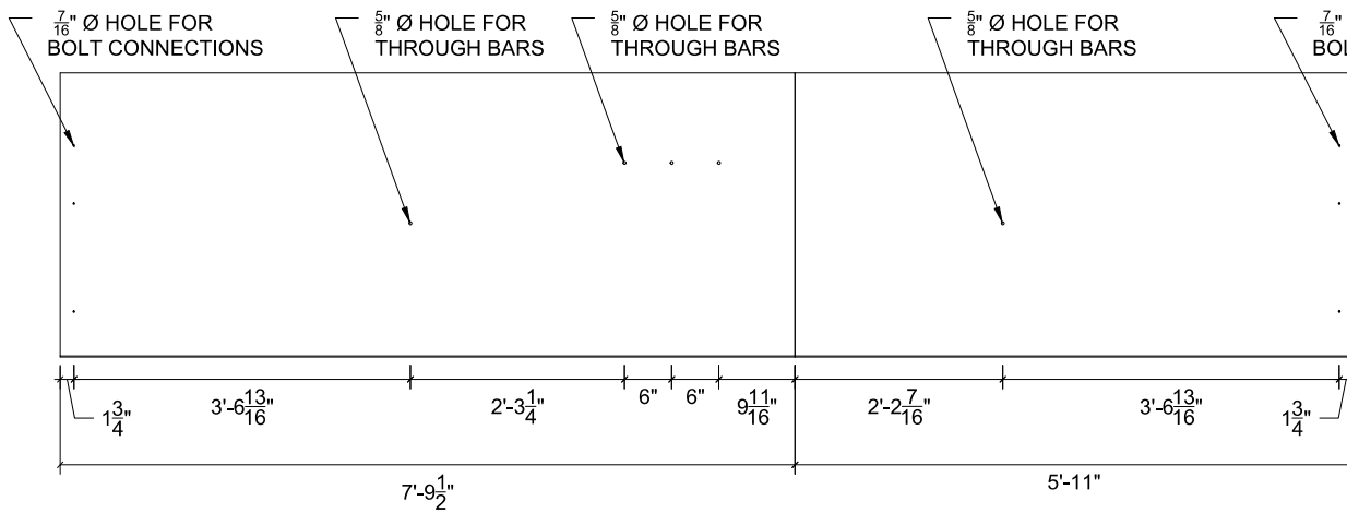
PLYWOOD 5A FRONT ELEVATION VIEW (t = 23/32")
