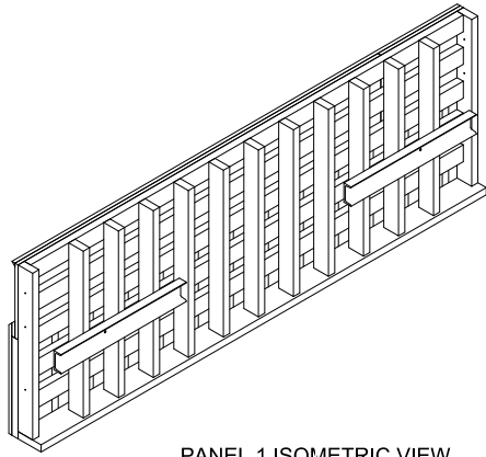
PANEL 1 ISOMETRIC VIEW
