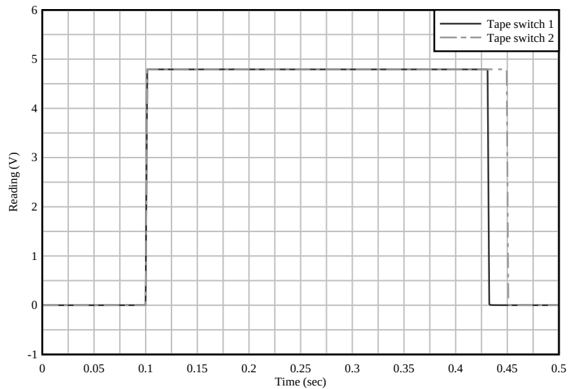
Figure 7.9 Tape switch data for FRC EOR test 1
