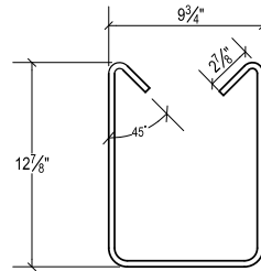
BAR S302 NO.3 GR. 60 QTY. 6
