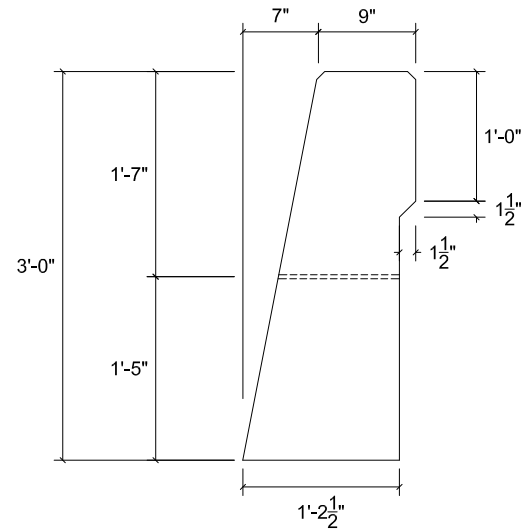
B-3 SIDE ELEVATION VIEW
