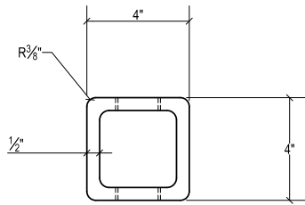
HSS 4X4X \frac{1}{2} A1058
