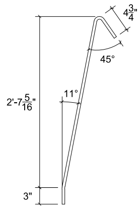
BAR 4V-A BAR SIZE: #4, LENGTH=3'-3 13 / 16 " , QTY:3
