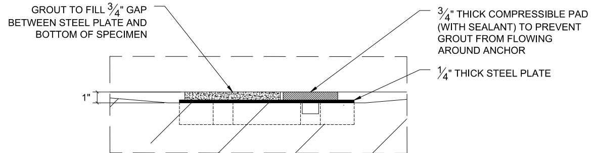
ANCHORED IMPACT SPECIMEN FRONT ELEVATION VIEW
