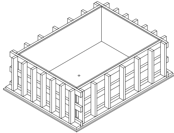
BACK ISOMETRIC VIEW (BACK BLOCK FORMWORK)
