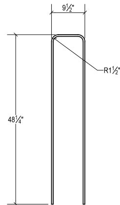
BAR U403 NO. 4 GR. 60 QTY. 2
