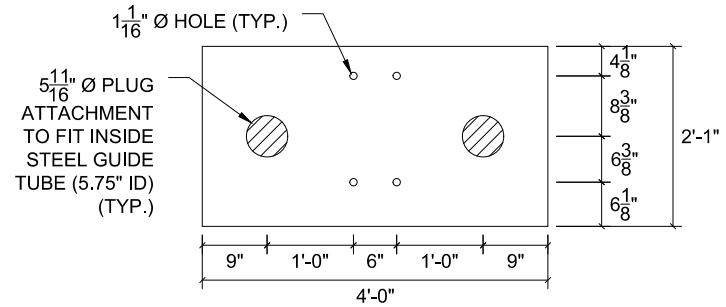
BACK PANEL PLYWOOD t = 3/4", QTY: 1
