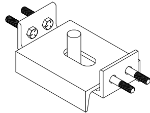
FLOOR CONNECTION HARDWARE ISOMETRIC VIEW
