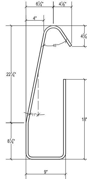
BAR 4V NO.4 GR.60 QTY. 26
