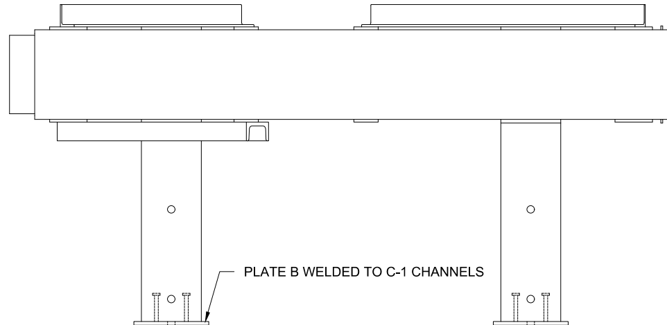
SIDE ELEVATION VIEW (FABRICATION SEQUENCE)
