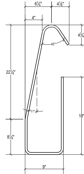
BAR 4V NO.4 GR.60 QTY. 16
