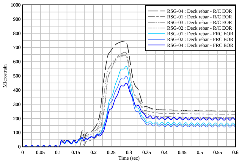
Figure 7.44 Comparison of internal strain gauges located on the top deck rebar
