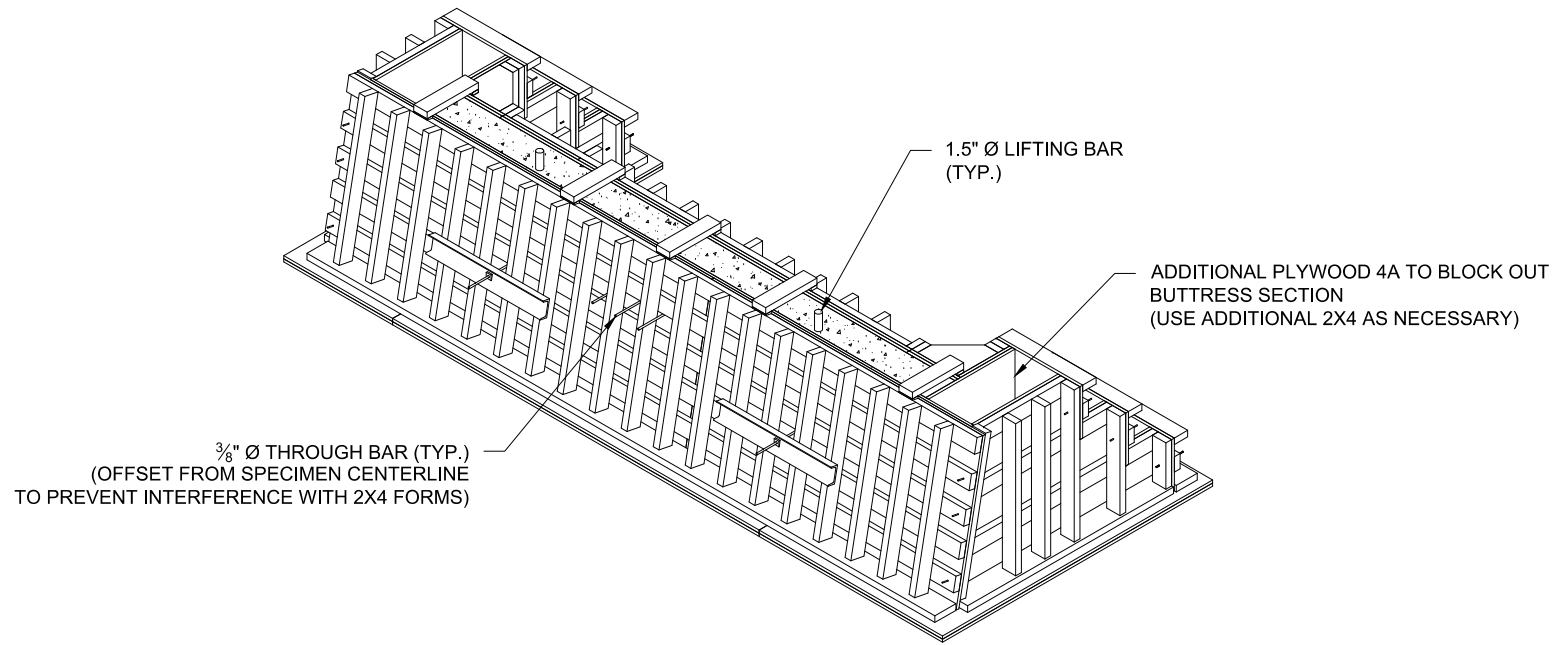
ISOMETRIC VIEW
