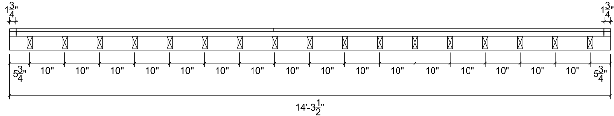
PANEL 7 PLAN VIEW
