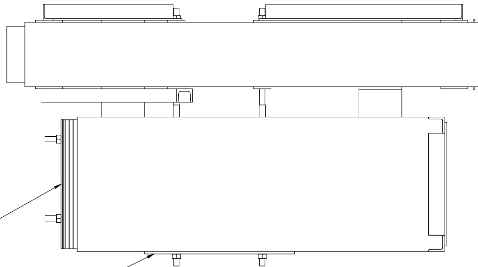
SIDE ELEVATION VIEW (FABRICATION SEQUENCE)
