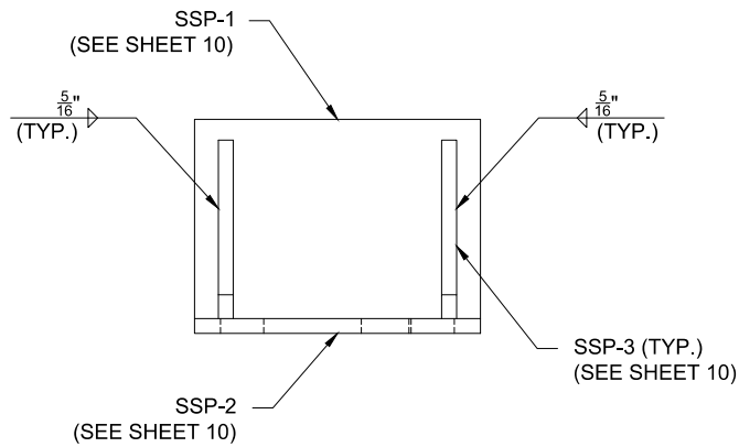
SLIDE STOPPER BACK ELEVATION VIEW
