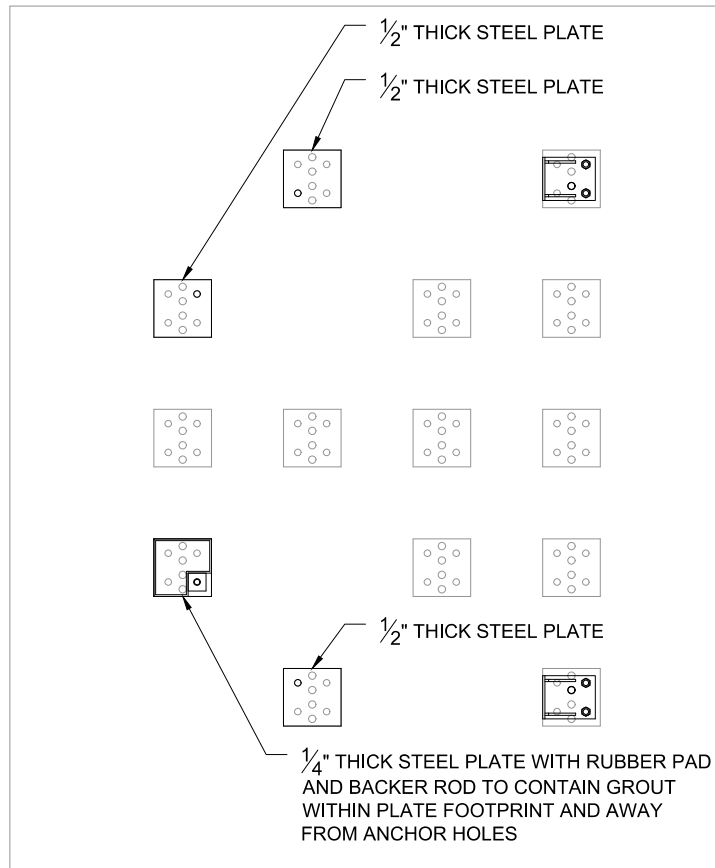
PLATES INSTALLED ONTO FOUNDATION PLAN VIEW
