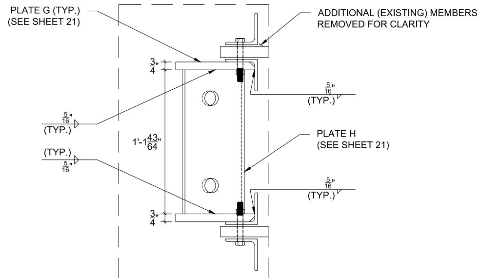
D-17: PLAN VIEW OF PULL-BACK CONNECTION
