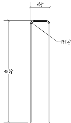
BAR U403 NO. 4 GR. 60 QTY. 2
