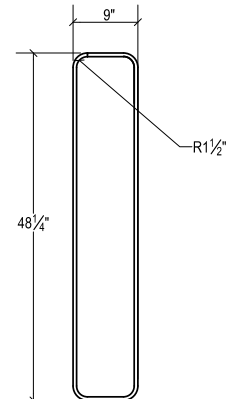
BAR H403 NO. 4 QTY. 4
