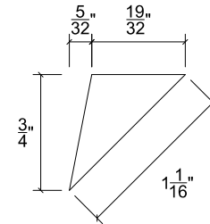
FRONT CHAMFER PIECE SIDE ELEVATION VIEW
