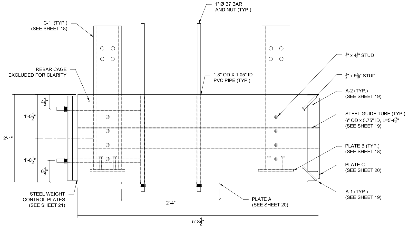
SIDE ELEVATION VIEW (BACK BLOCK COMPONENTS, REBAR CAGE EXCLUDED)
