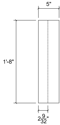
ALUMINUM LOADING WEDGE: PLAN VIEW t = 5", ALUMINUM 6061 T6, QTY:1
