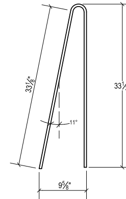
BAR 4P NO.4 GR.60 QTY. 16
