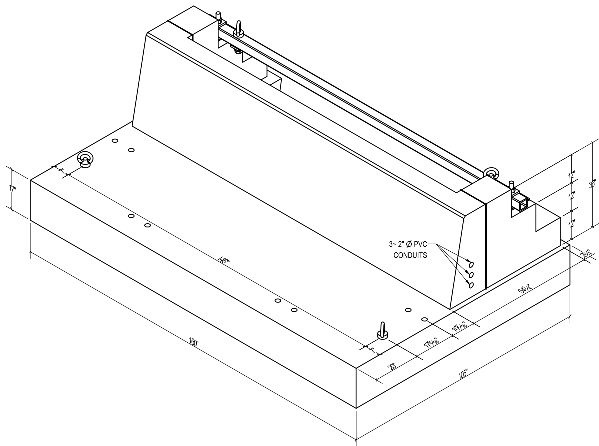
TEST SPECIMEN FRONT ISOMETRIC VIEW
