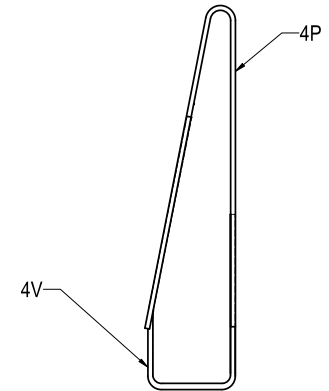
BARRIER STIRRUP 4P&4V (FDOT STANDARD PLANS 521-427)
