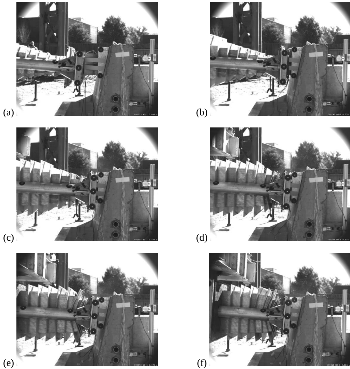
Figure 7.4 High-speed video frames from HSC-1 (FRC EOR test 1) showing crush deformation of aluminum honeycomb: (a) At initial impact; (b) – (e) Intermediate frames; (f) At peak impact force
