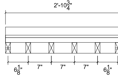
PANEL 4 PLAN VIEW
