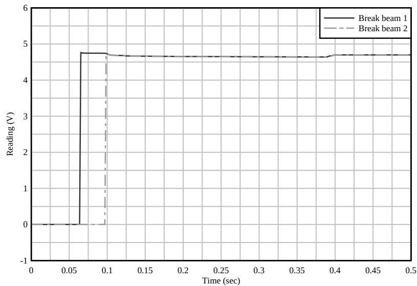
Figure 6.51 Break beam data for R/C COR test 2
