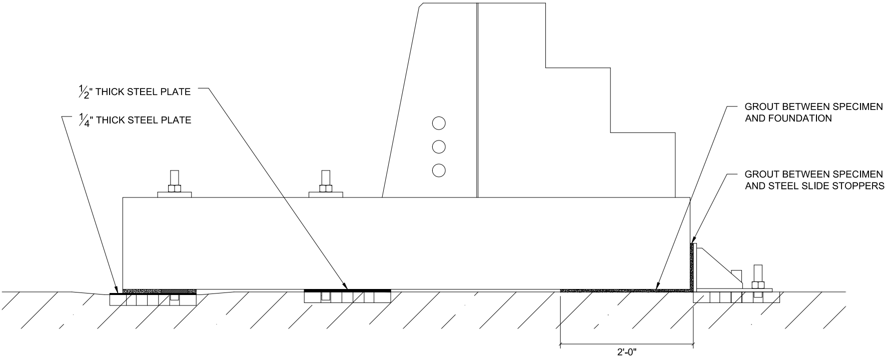
ANCHORED IMPACT SPECIMEN SIDE ELEVATION VIEW
