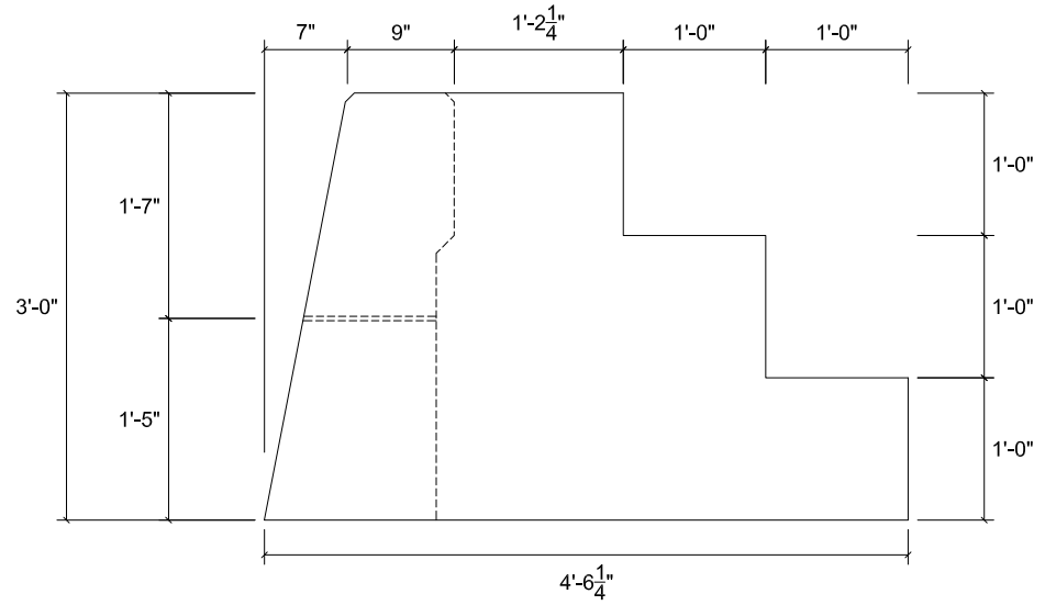
A-3 SIDE ELEVATION VIEW
