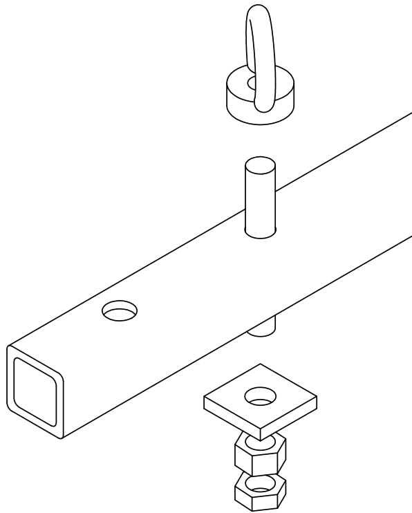
LIFTING EYE NUT ASSEMBLY
