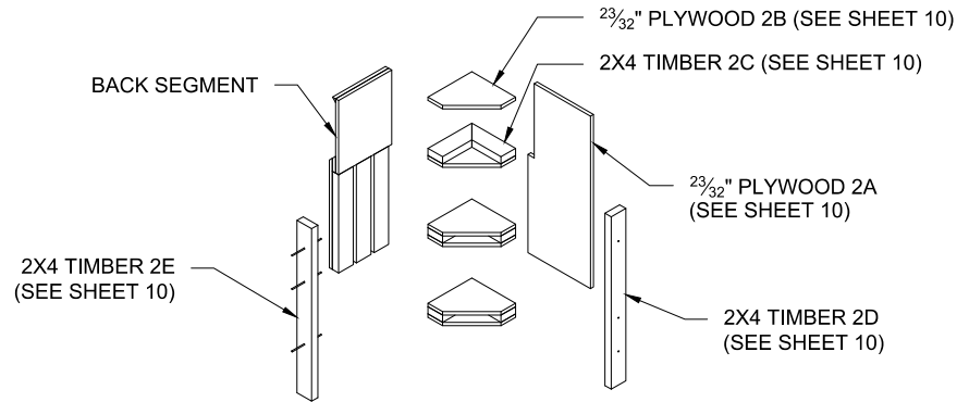
PANEL 2 (RIGHT CORNER FORM) ISOMETRIC VIEW OF COMPONENTS
