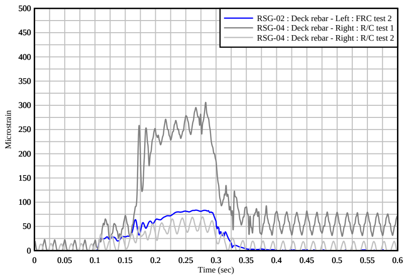
Figure 6.69 Comparison of internal strain gauges located on the top deck rebar
