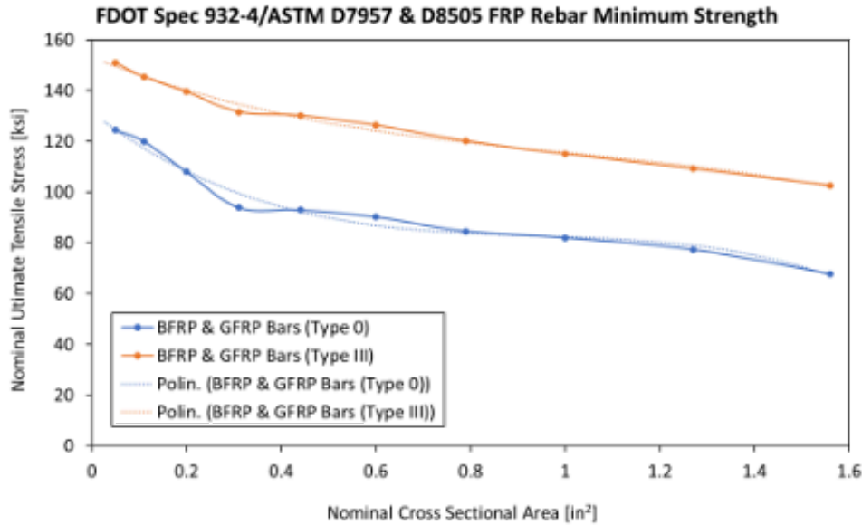
Figure 65. Ultimate stress trend vs. FRP bars area
