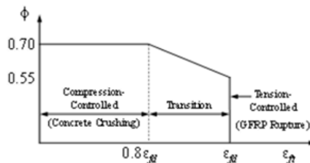
Figure 71. Figure C2.5.5.2-1—Variation of \phi_f with tensile strain at failure \epsilon_{ft} in GFRP Reinforcement
