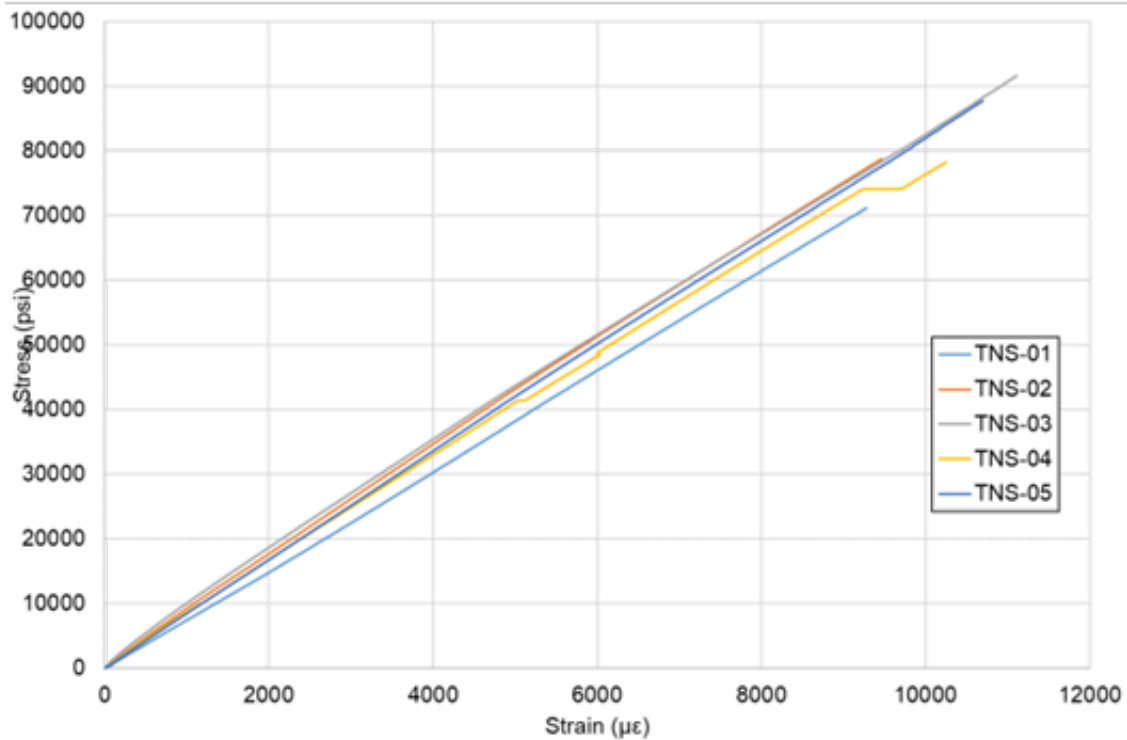
Figure 17. Stress vs. strain of #11 FRP bars at both gauge lengths (extensometer removed halfway during the test)
