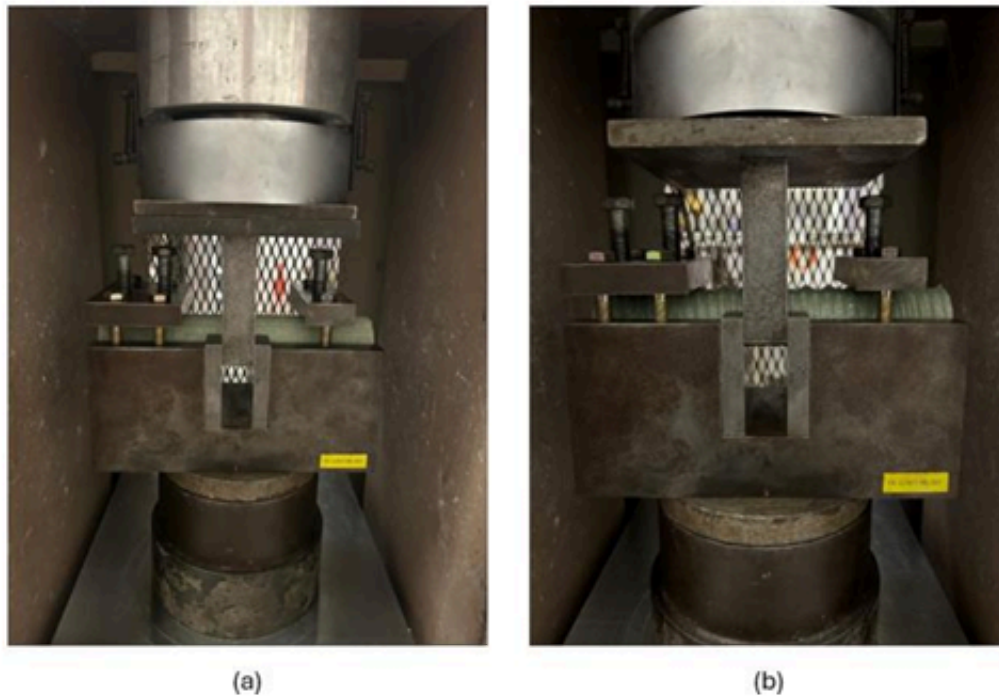
Figure 34. Transverse shear strength test setup (a) Pultrall and (b) MST-Bar
