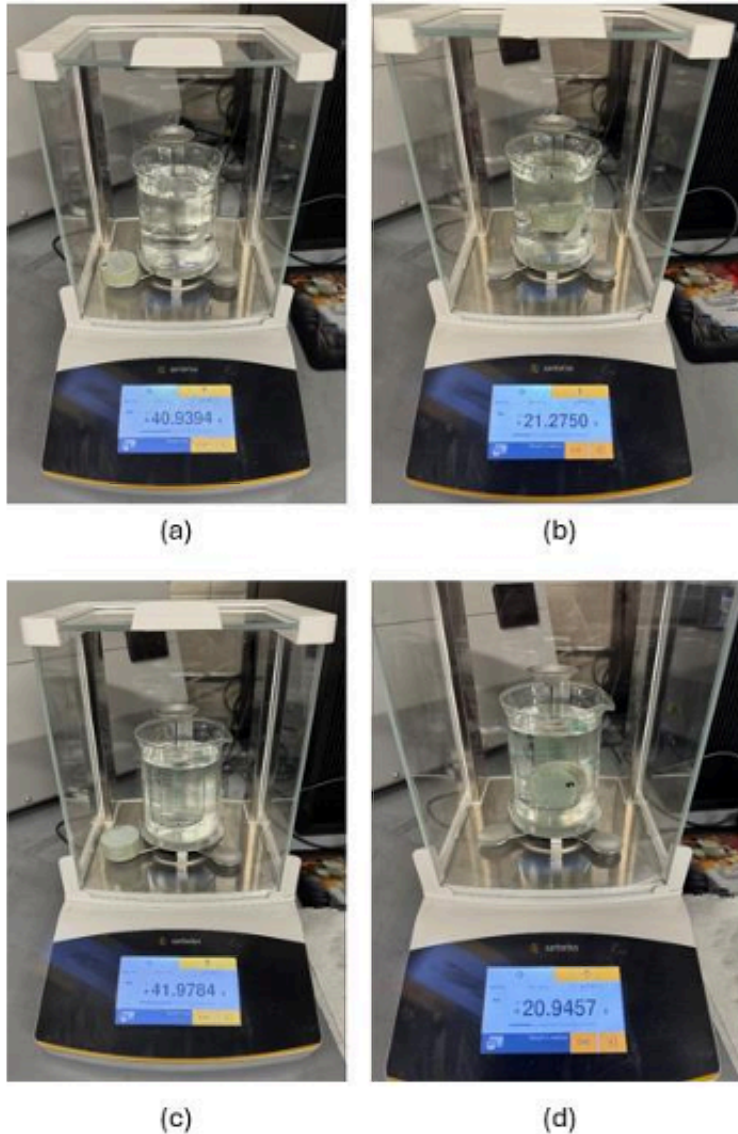
Figure 30. Test setup for measurement of cross-sectional area; (a) specimen weight and (b) immersed specimen for Pultrall; (c) Specimen weight and (b) immersed specimen for MST-Bar
