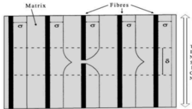
Figure 4. Illustration of load-sharing fiber rupture [6]
