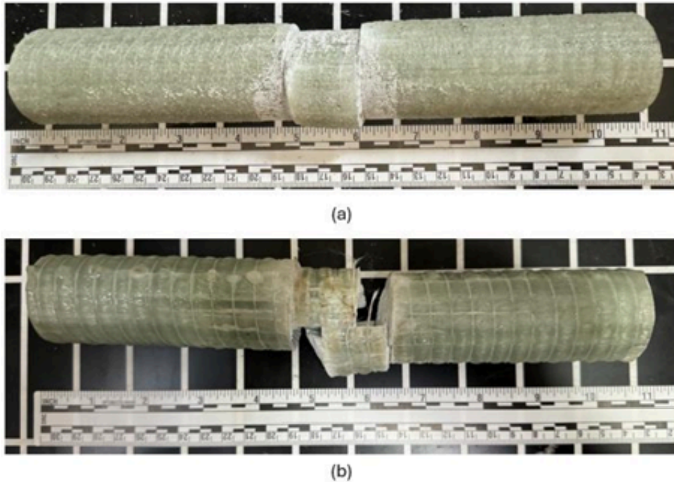
Figure 35. Transverse shear strength representative double shear failure mode; (a) Pultrall and (b) MST-Bar
