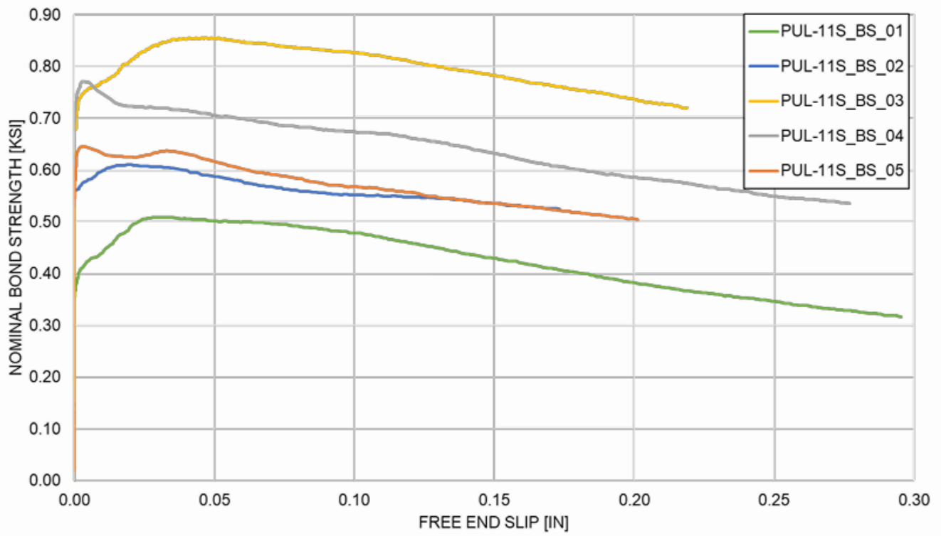
Figure 75. Nominal bond strength vs. free-end slip for Pultrall #11 bars
