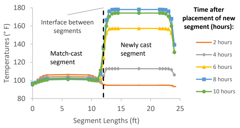
Figure B-156: Simulation 52 - Internal temperatures along the wing of segments
