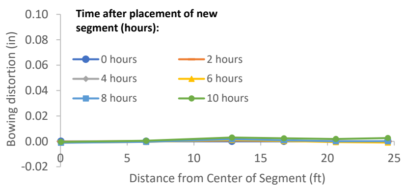
Figure B-19: Simulation 7 - Bowing distortion of match-cast segment after placement of the new segment
