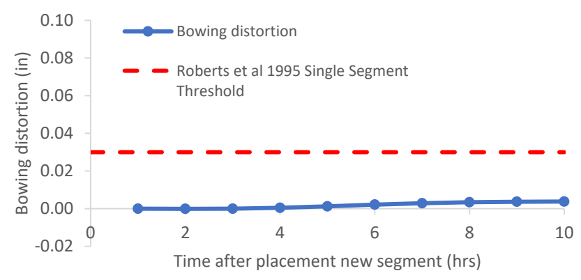
Figure B-362: Simulation 121 - Bowing distortion progression of match-cast segment from time of placement of new segment to 10 hours
