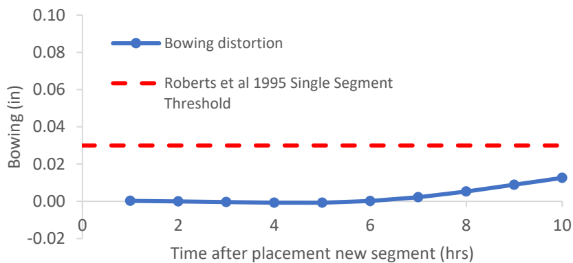
Figure B-143: Simulation 48 - Bowing distortion progression of match-cast segment from time of placement of new segment to 10 hours
