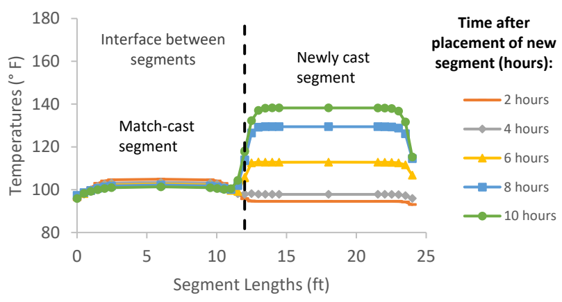
Figure B-147: Simulation 49 - Internal temperatures along the wing of segments
