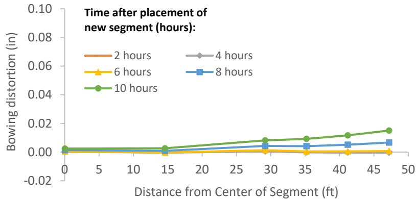
Figure B-142: Simulation 48 - Bowing distortion of match-cast segment after placement of the new segment
