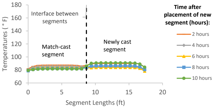
Figure B-171: Simulation 57 - Internal temperatures along the wing of segments
