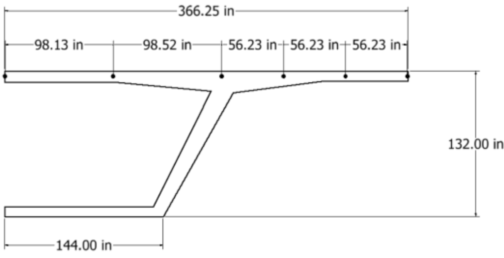
Figure A-8: Locations where deformations were examined for Bridge D
