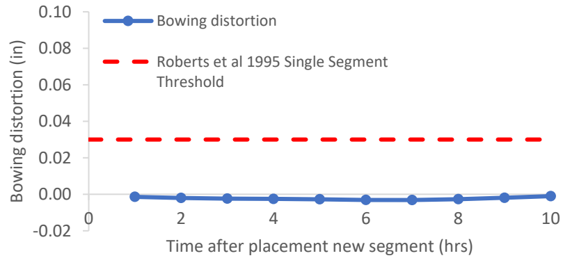
Figure B-308: Simulation 103 - Bowing distortion progression of match-cast segment from time of placement of new segment to 10 hours
