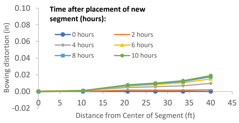
Figure B-31: Simulation 11 - Bowing distortion of match-cast segment after placement of the new segment
