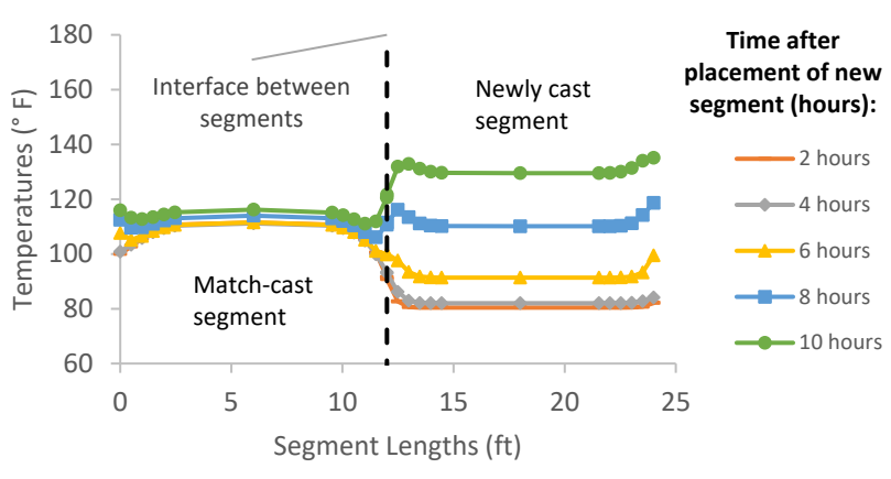
Figure B-282: Simulation 94 - Internal temperatures along the wing of segments
