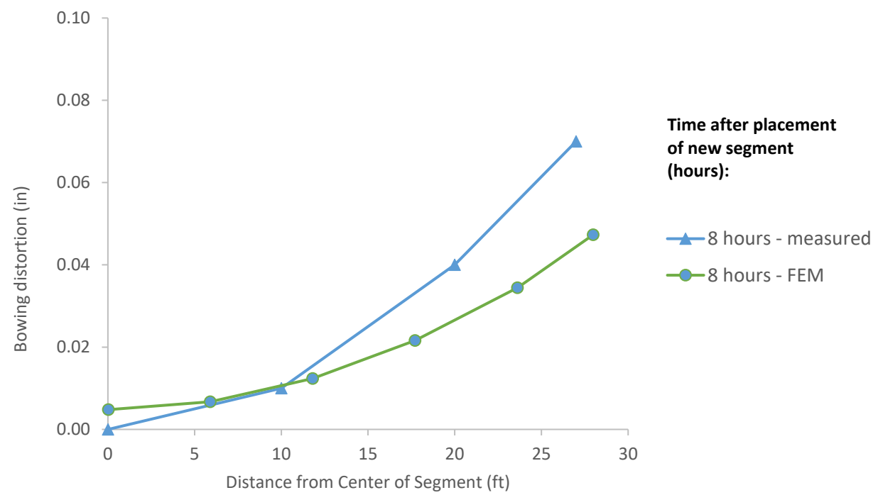
Figure 31: Measured and FEM simulated distortion for San Antonio “Y” type III segment at 8 hours after new concrete placement
