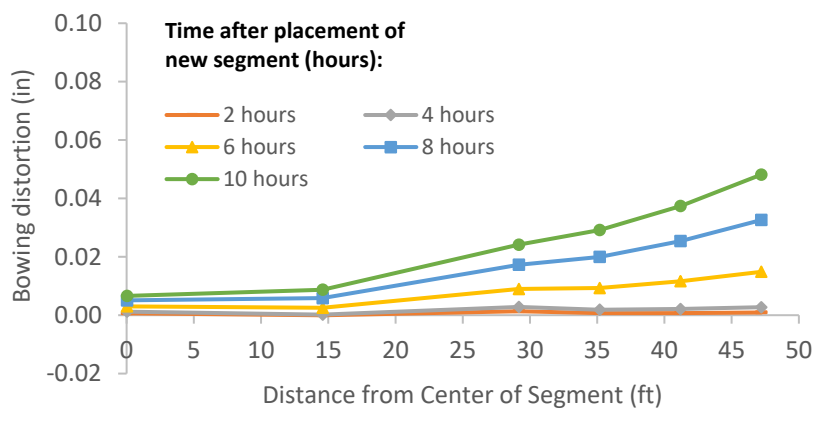
Figure B-124: Simulation 42 - Bowing distortion of match-cast segment after placement of the new segment
