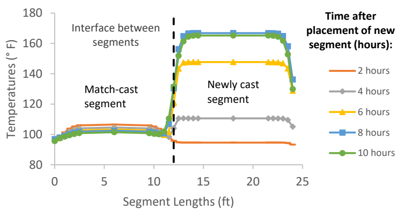
Figure B-129: Simulation 43 - Internal temperatures along the wing of segments
