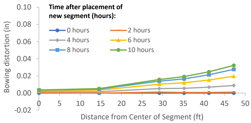
Figure B-7: Simulation 3 - Bowing distortion of match-cast segment after placement of the new segment
