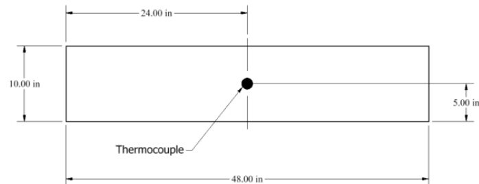
Figure 54: Elevation view of thermocouple setup
