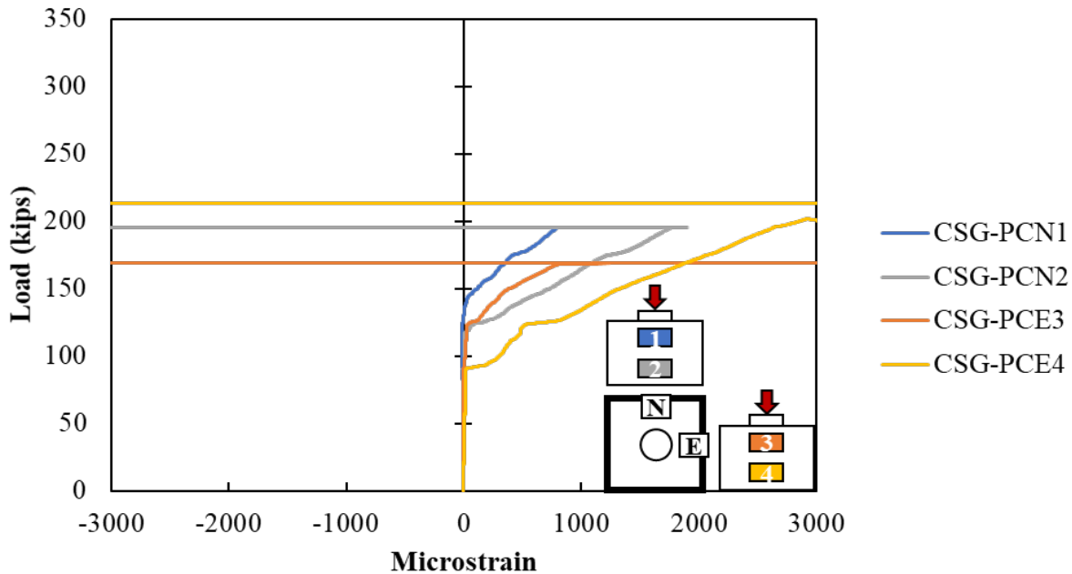
Figure A.203: Concrete strain gauges in the surface of Specimen S3-10
