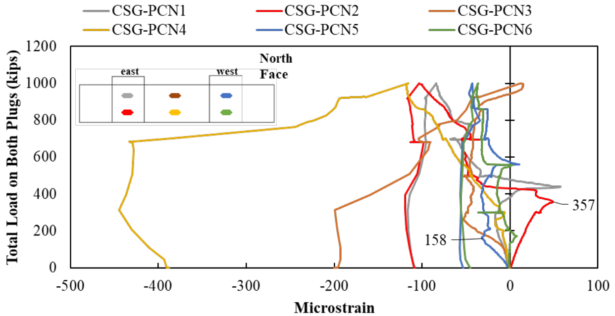
Figure B.39: Concrete strain gauges on the concrete surface of Specimen MP-2
