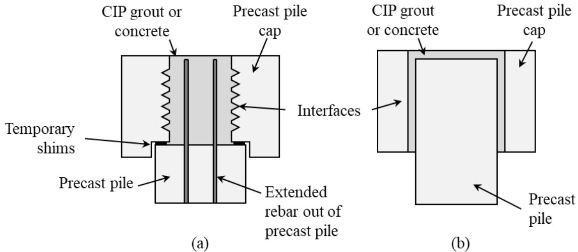
Figure 6.1: Example connection between pre-cast pile and pile: (a) pocket connection, and (b) socket connection
