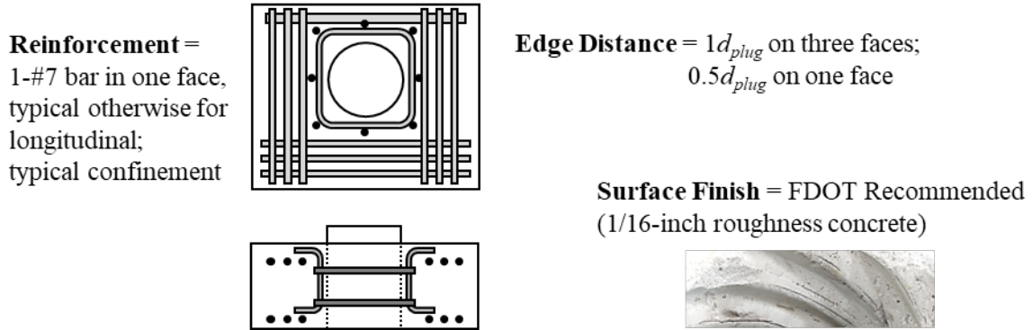
Figure A.193: Details for S3-9
