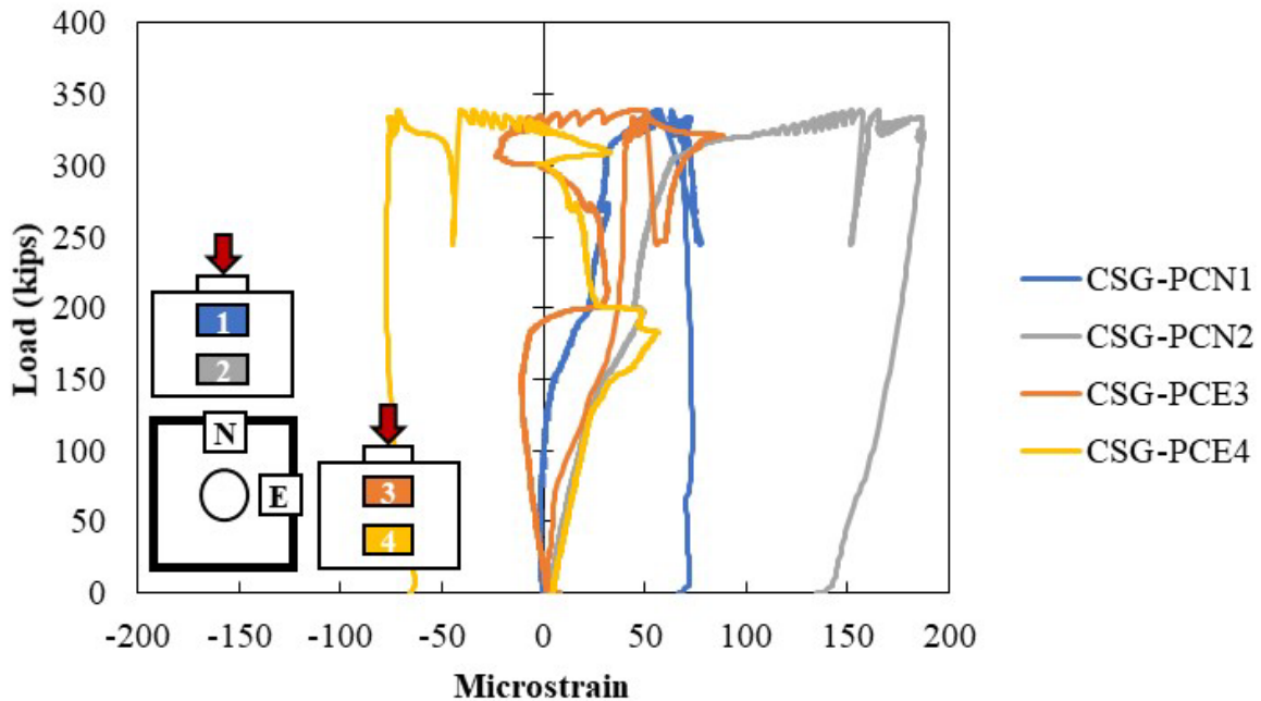
Figure A.23: Concrete strain gauge on the concrete surface of Specimen S2-1
