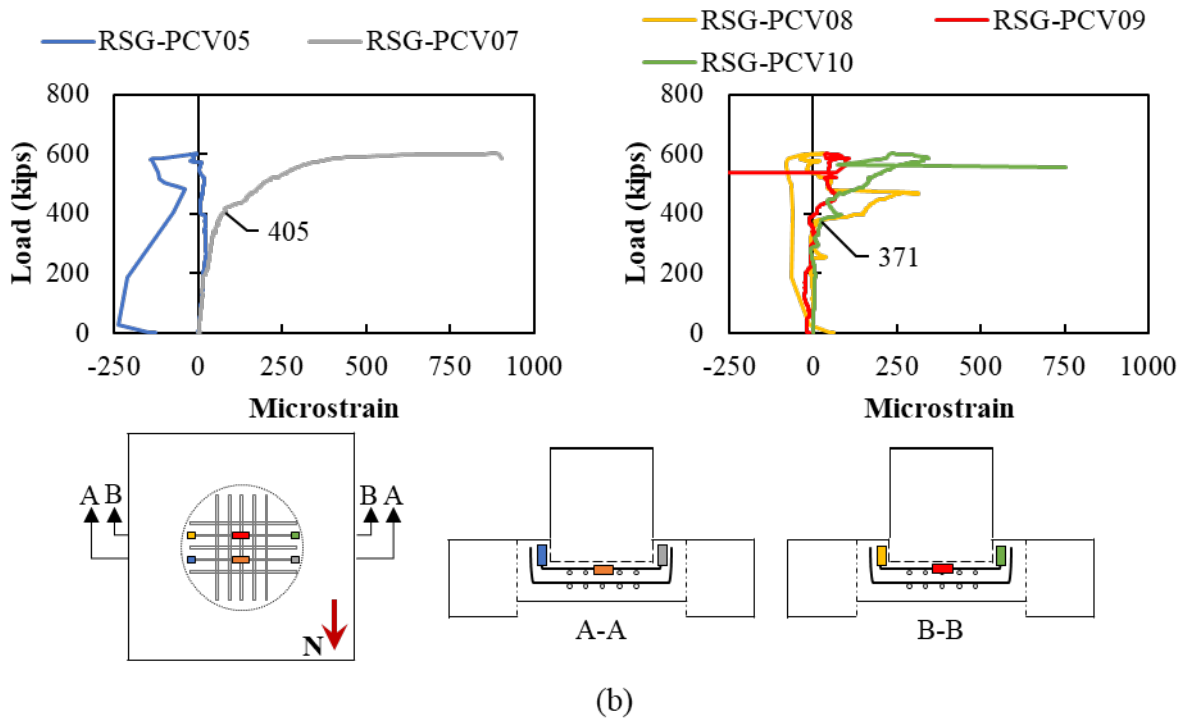
Figure B.56: Load versus strain measured using RSG for (a) bottom layer and (b) top layer of void reinforcement in Specimen SC-2 in the east-west direction
