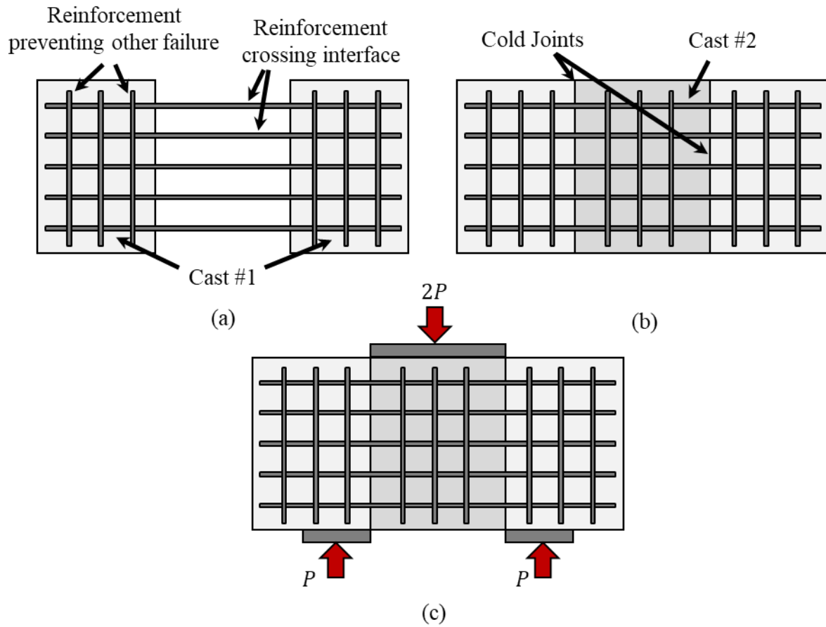
Figure 2.15: Typical casting and testing procedure for push-through tests: (a) casting of first component, (b) casting of second component, and (c) testing of push-through specimen
