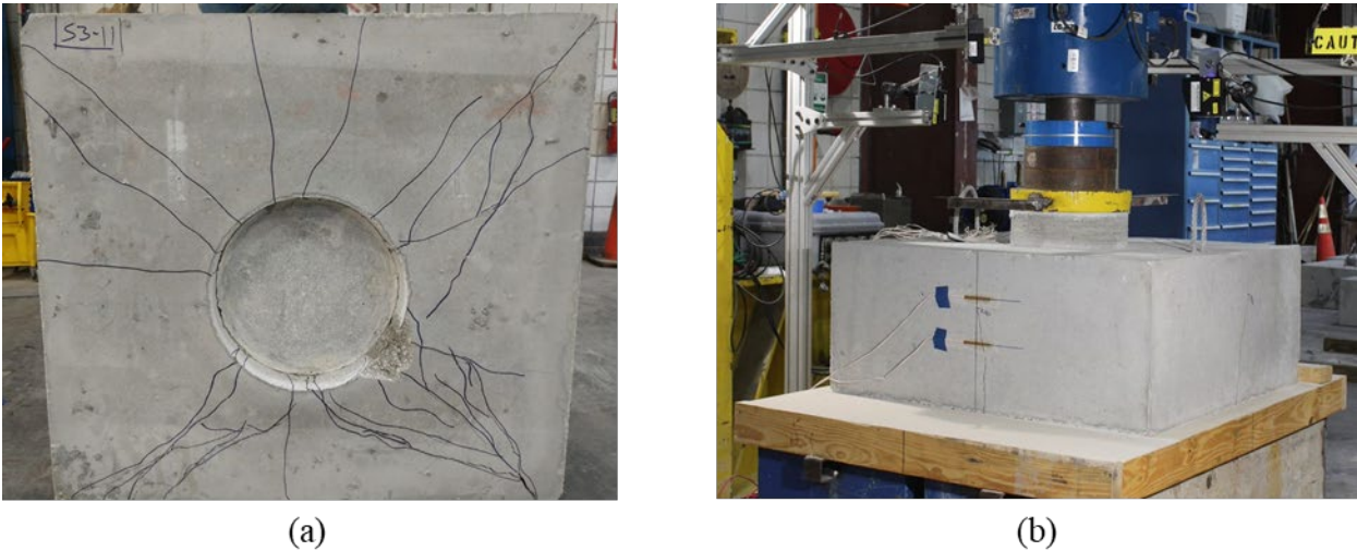
Figure A.211: Cracking on (a) bottom after testing and (b) cap during testing of Specimen S3-11
