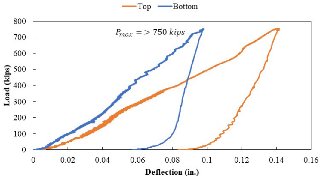
Figure A.28: Load versus deflection curve for Specimen S2-2
