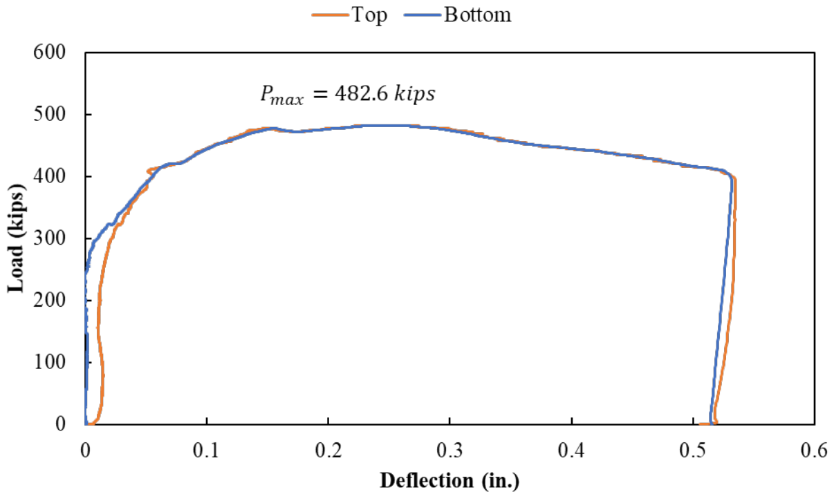
Figure A.132: Load deflection curve for Specimen S2-19
