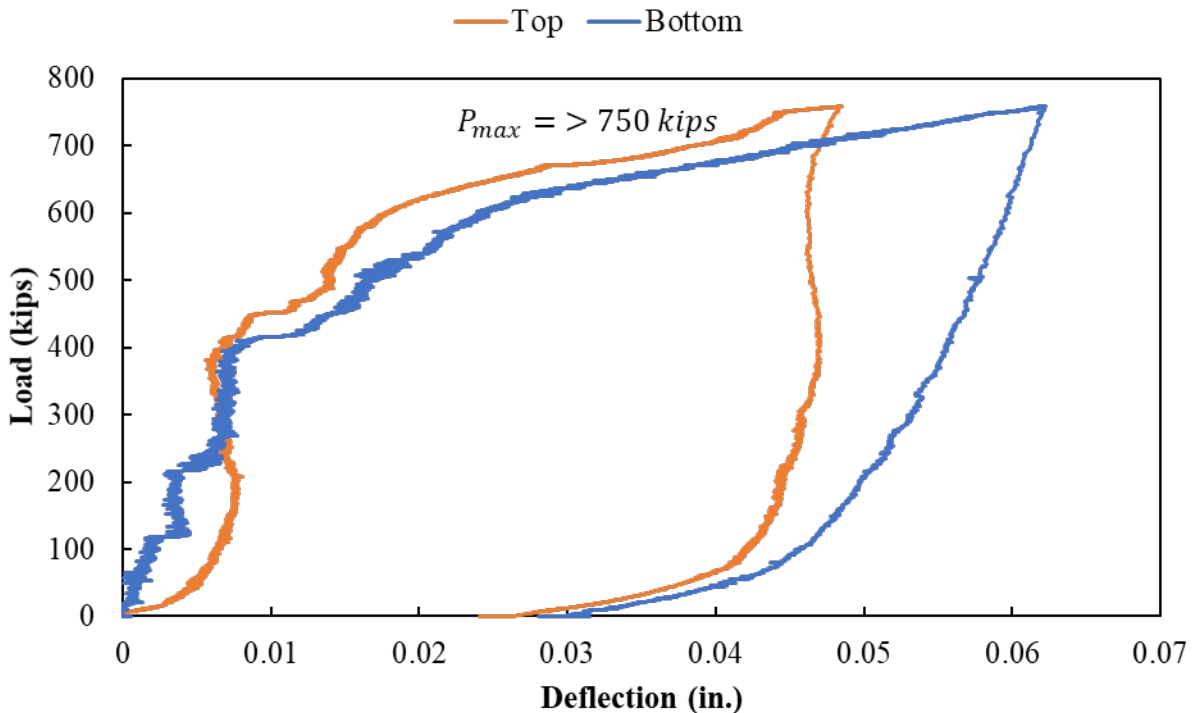
Figure A.120: Load versus displacement curve for Specimen S2-16
