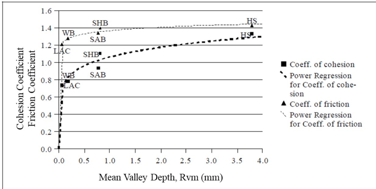
Figure 2.5: Correlation between the Mean Valley Depth ( R_{vm} ) and the cohesion and friction coefficient [22]
