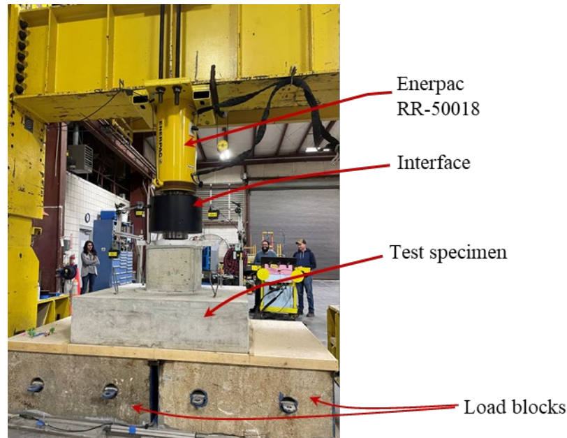
Figure 4.22: Photograph of test setup for socket connection specimens
