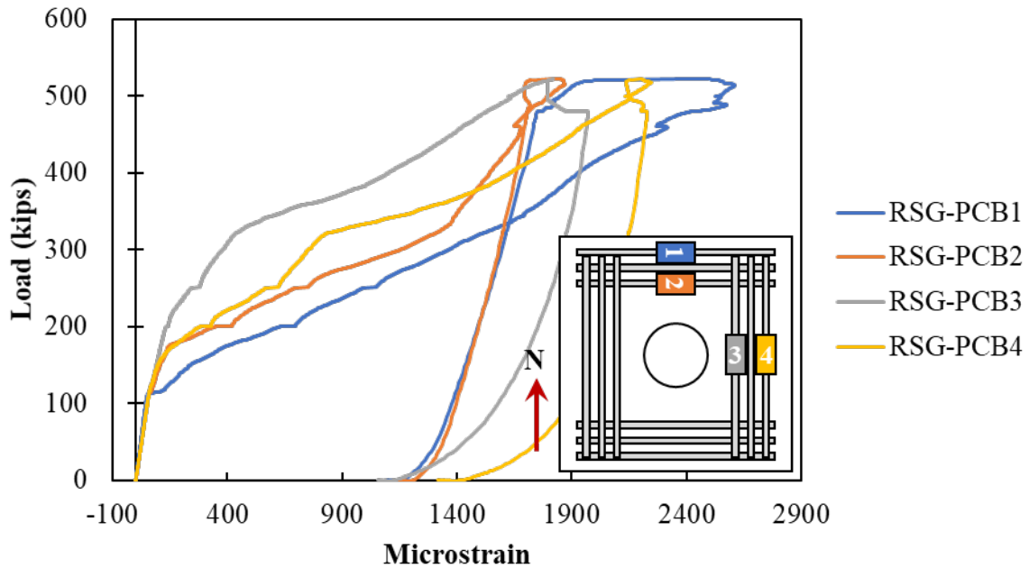
Figure A.100: Rebar strain gauges in the longitudinal reinforcement on bottom of Specimen S2-12
