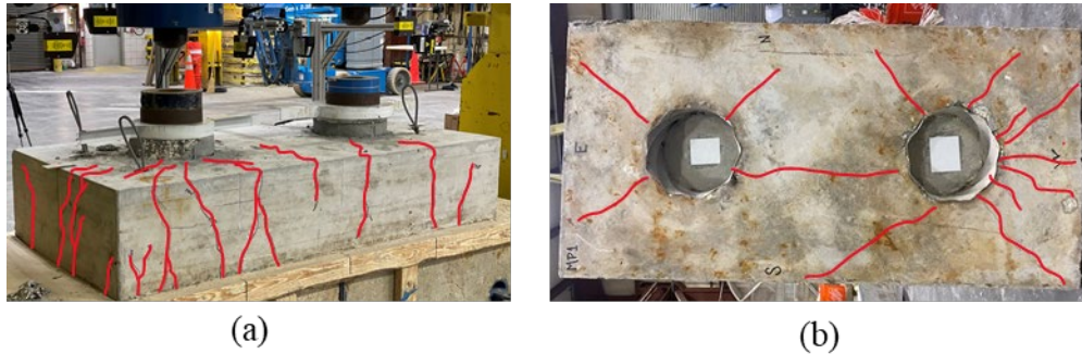
Figure B.35: Cracking after testing on (a) south-west view and (b) bottom of specimen MP-1
