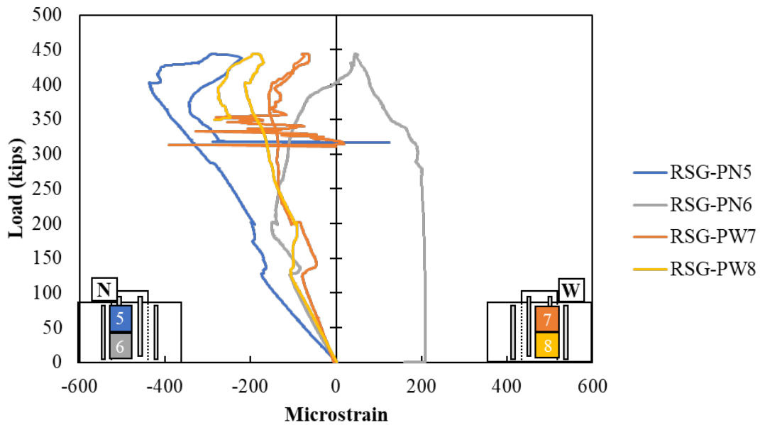
Figure A.151: Rebar strain gauges in vertical reinforcement on plug of Specimen S3-2
