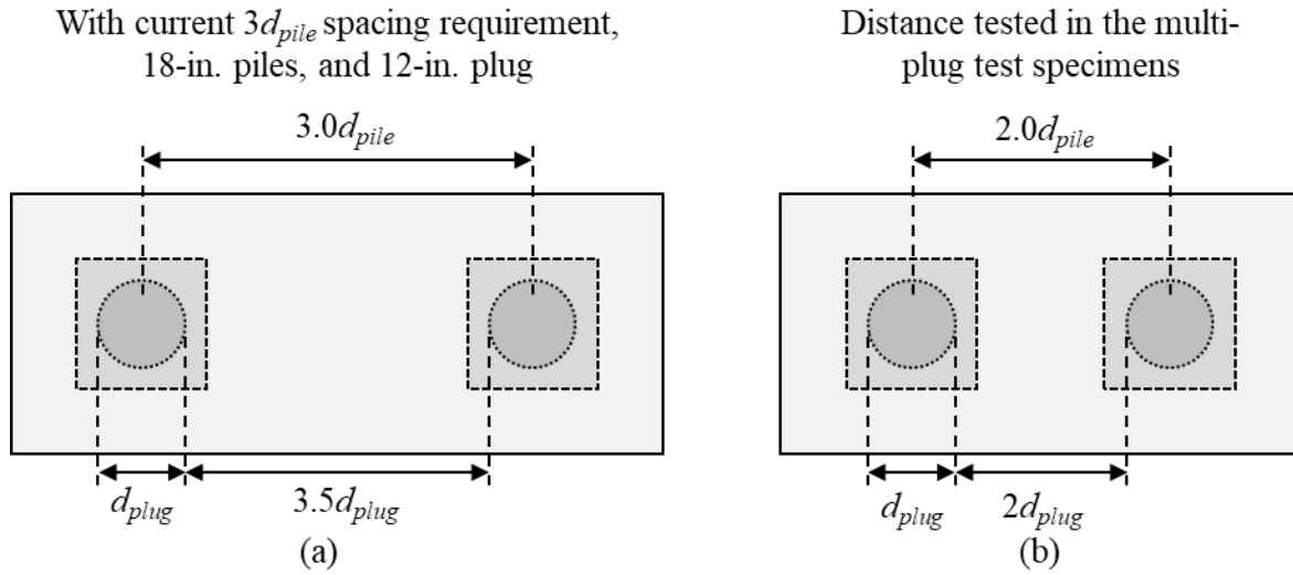
Figure 6.4: Spacing between piles and plugs (a) as specified in FDOT SDG and (b) minimum tested A cap reinforcement detail like that provided in the FDOT SDM, shown in Figure 6.5, was used in the test specimens. Confinement reinforcement around the pocket was provided in most specimens but was also omitted in several specimens.
