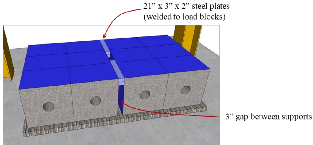
Figure 4.8: Schematic of supports with 3-inch space between load blocks
