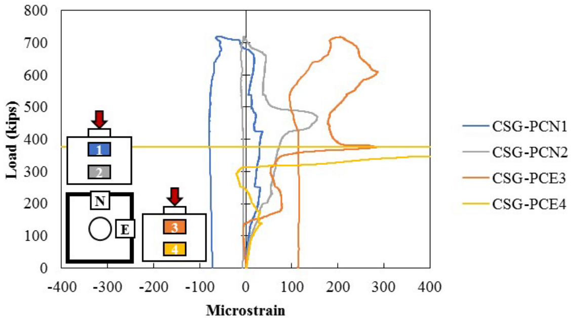
Figure A.65: Concrete strain gauges in the surface of Specimen S2-7
