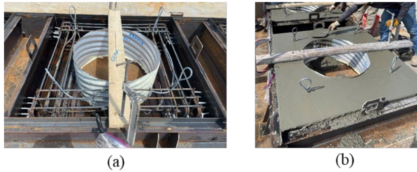
Figure 4.18: (a) Construction of the socket connection specimen and (b) casting of the cap.
