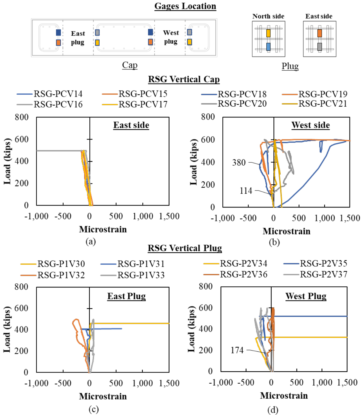
Figure B.34: Rebar strain gauges in vertical reinforcement on (a) cap around east plug, (b) cap around west plug, (c) east plug, and (d) west plug
