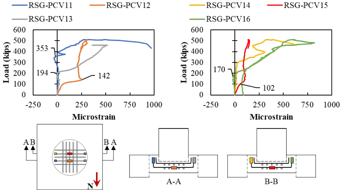
Figure 6.7: Sample load versus microstrain plots for socket reinforcement in SC-1
