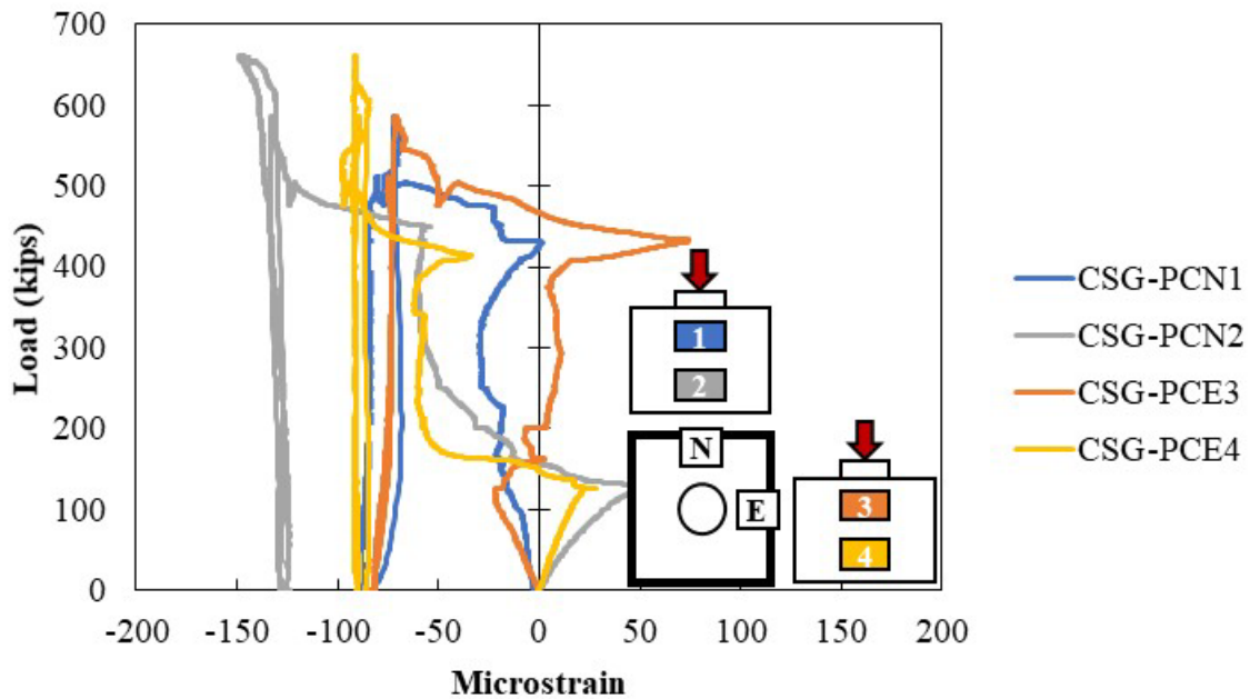
Figure A.79: Concrete strain gauges in the surface of Specimen S2-9
