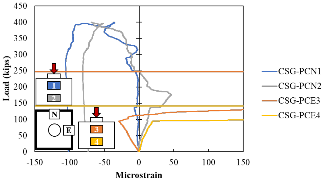
Figure A.94: Concrete strain gauges in the surface of the cap of Specimen S2-11
