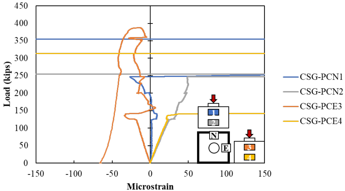
Figure A.223: Concrete strain gauges in the surface of the cap of Specimen S3-13
