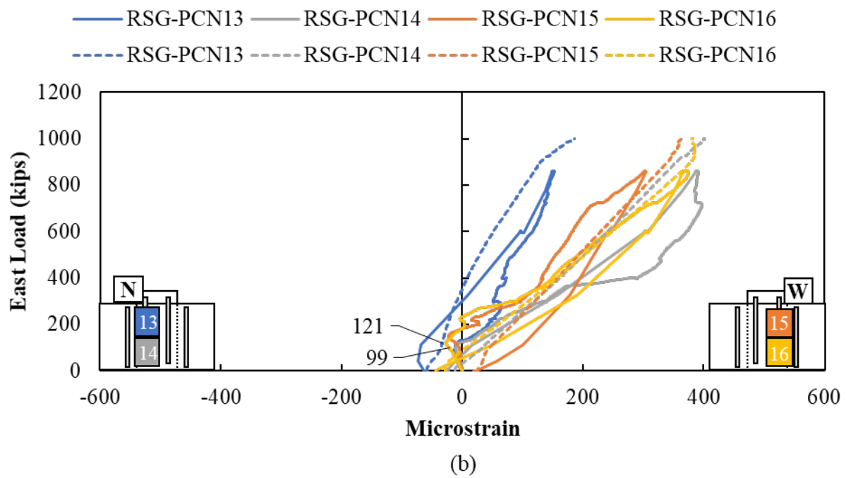
Figure B.20: Rebar strain gauges in vertical reinforcement on (a) cap and (b) plug of Specimen LP-3
