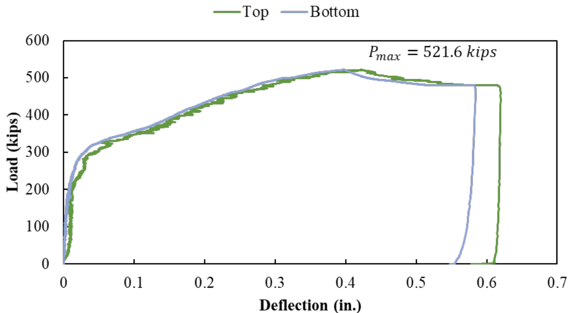
Figure A.99: Load versus deflection curve for Specimen S2-12
