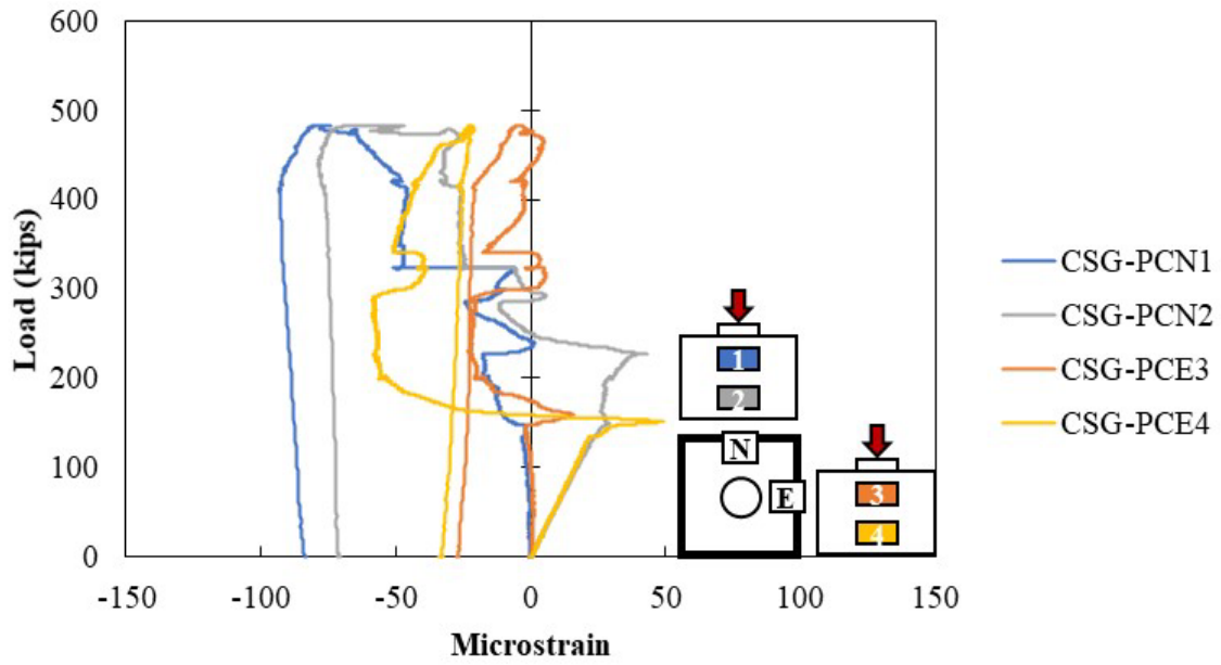
Figure A.133: Concrete strain gauges on the concrete surface of Specimen S2-19
