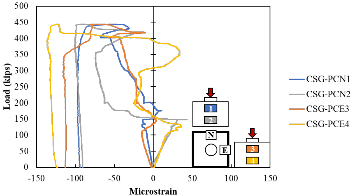
Figure A.149: Concrete strain gauges in the surface of Specimen S3-2
