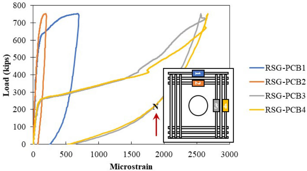
Figure A.29: Rebar strain in longitudinal bars on bottom of Specimen S2-2
