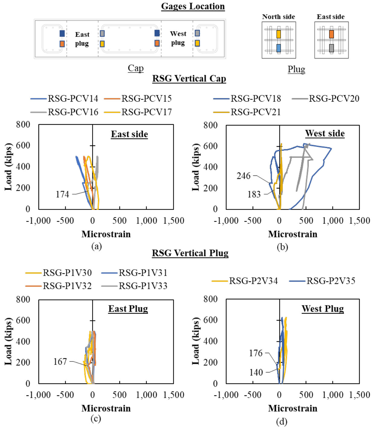
Figure B.40: Rebar strain gauges in vertical reinforcement on (a) cap around east plug, (b) cap around west plug, (c) east plug, and (d) west plug for Specimen MP-2
