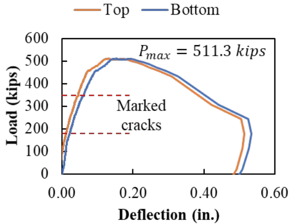
Figure 4.23: (a) Sample load versus deflection plot with stops and (b) crack pattern at 350 kips for Specimen SC-1
