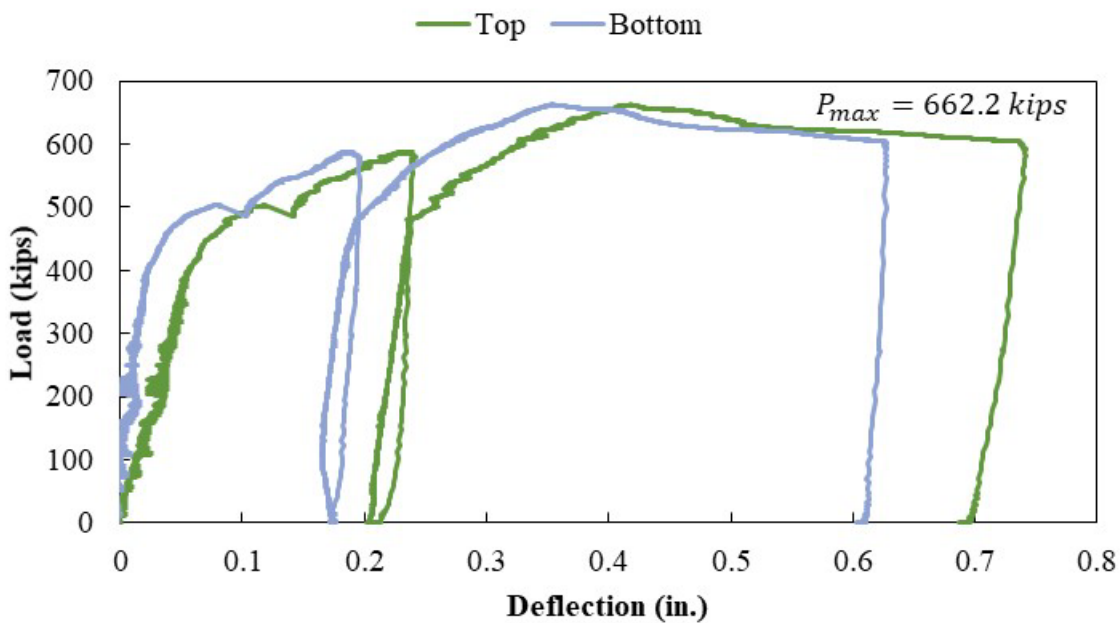
Figure A.77: Load versus deflection curve for Specimen S2-9
