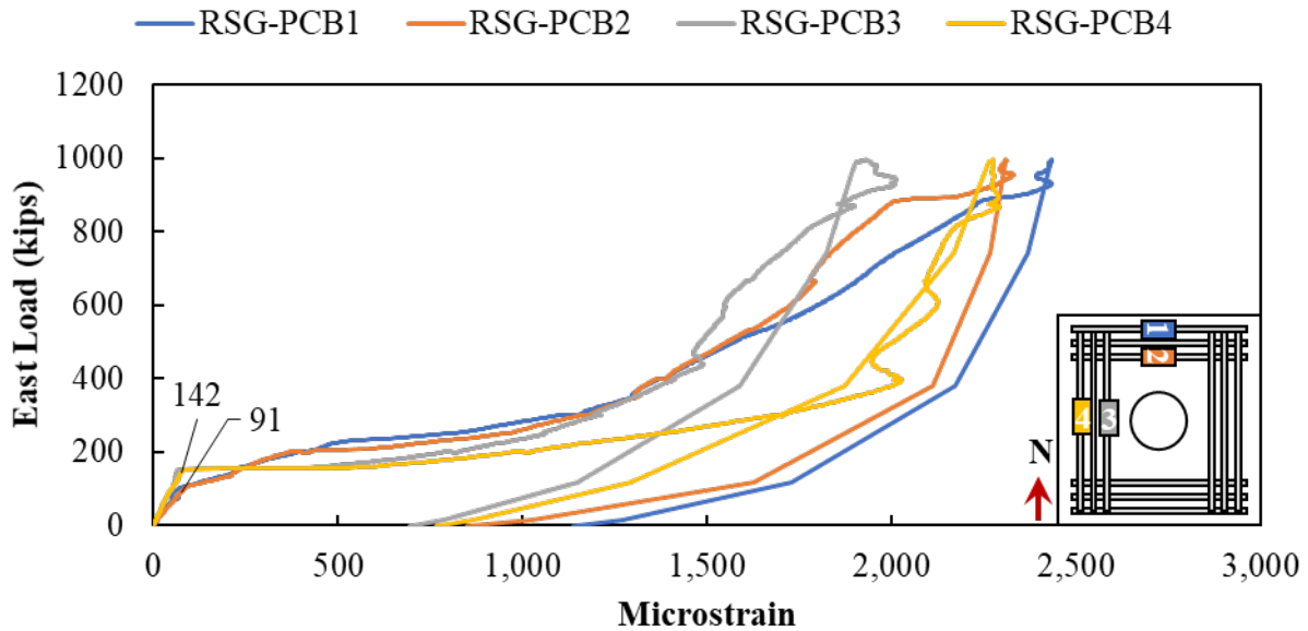
Figure B.23: Rebar strain gauges in the longitudinal reinforcement on bottom Specimen LP-4
