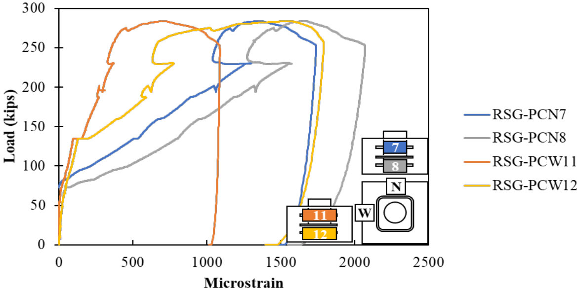
Figure A.177: Confining reinforcement around pocket of Specimen S3-6
