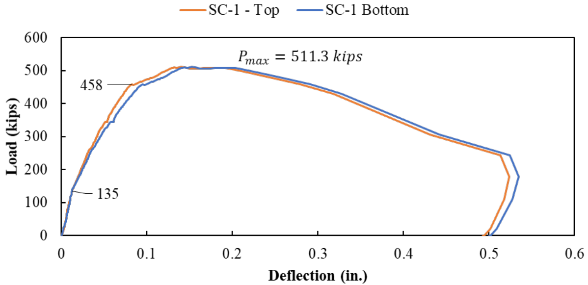
Figure B.43: Load versus deflection curve for Specimen SC-1
