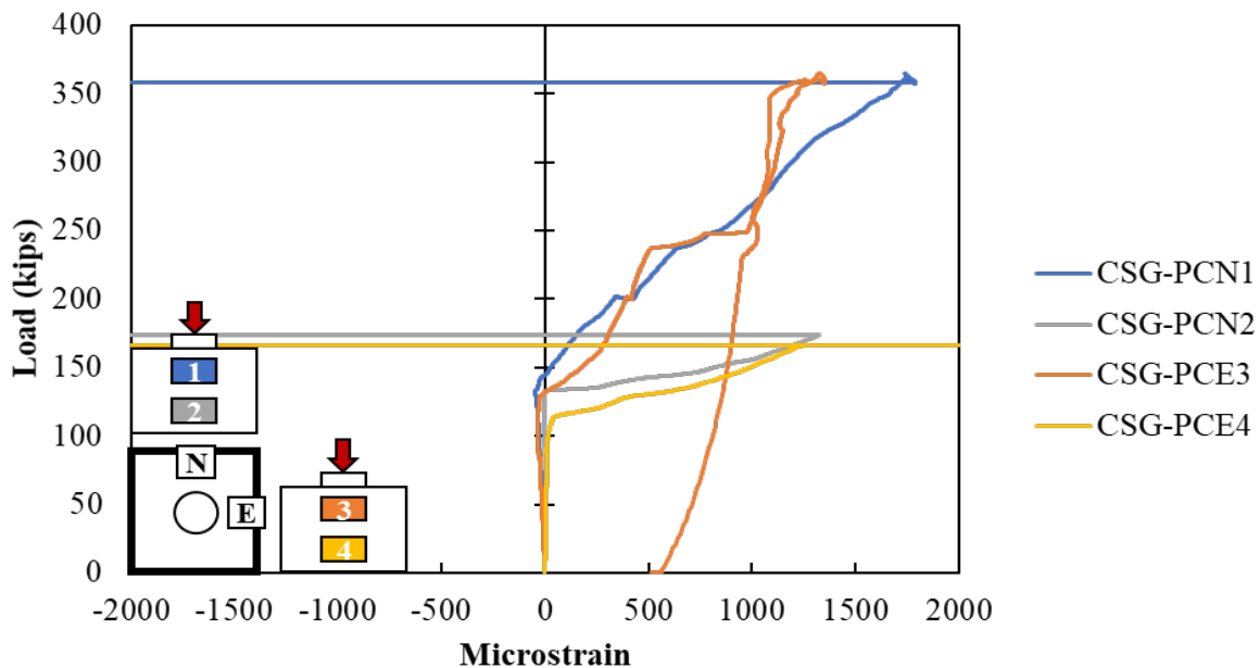
Figure A.196: Concrete strain gauges in the surface of the cap of Specimen S3-9
