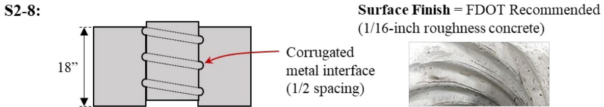
Figure A.69: Details for S2-8
