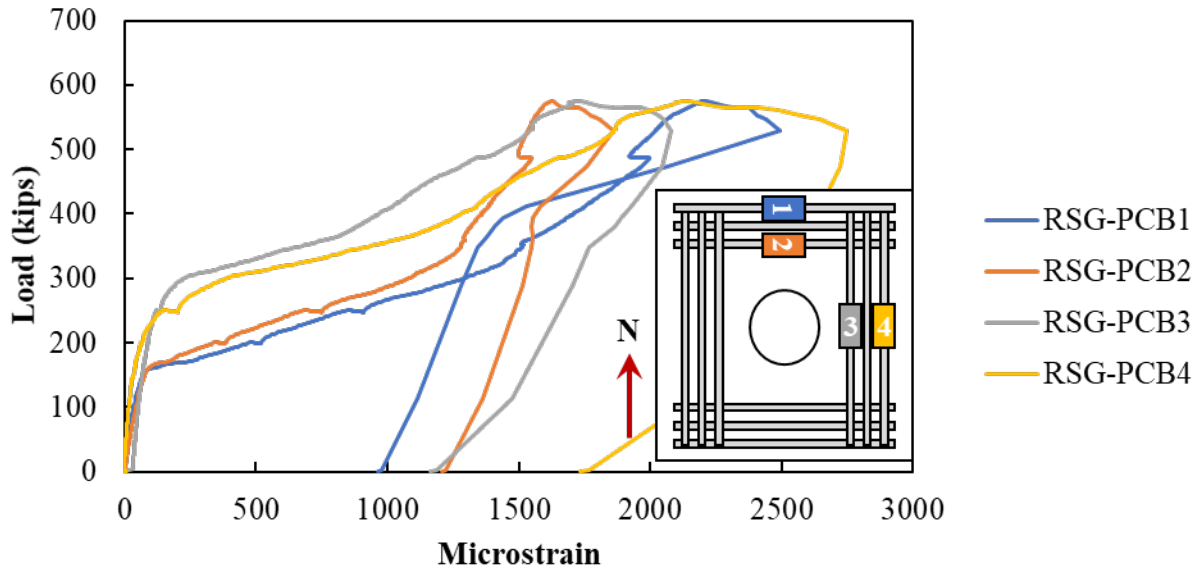
Figure 3.17: Rebar strain gauges in the longitudinal reinforcement on bottom of Specimen S2-10
