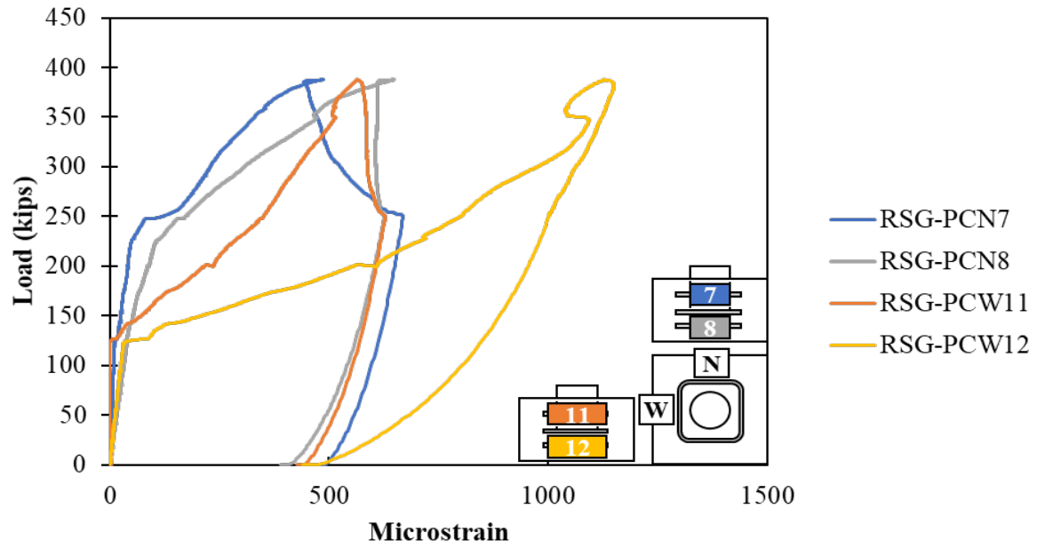
Figure A.225: Confining reinforcement around the pocket of Specimen S3-13
