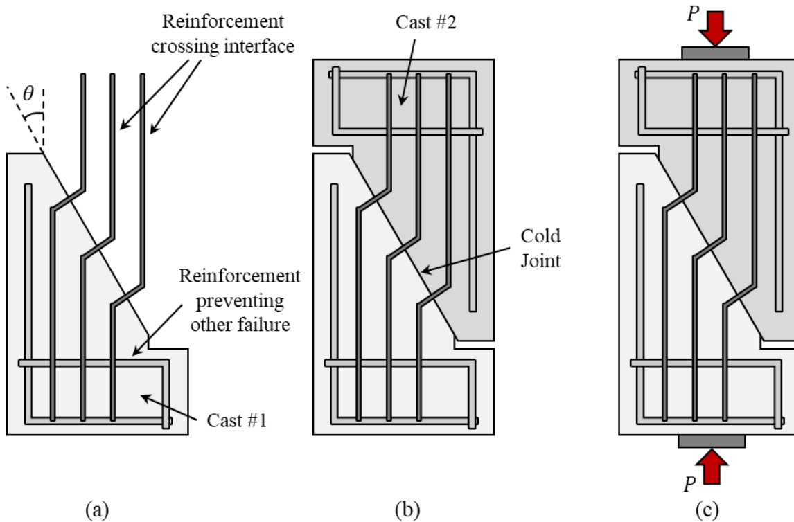
Figure 2.14: Typical casting and testing procedure for modified push-off tests: (a) casting of first component, (b) casting of second component, and (c) testing of modified push-off specimen
