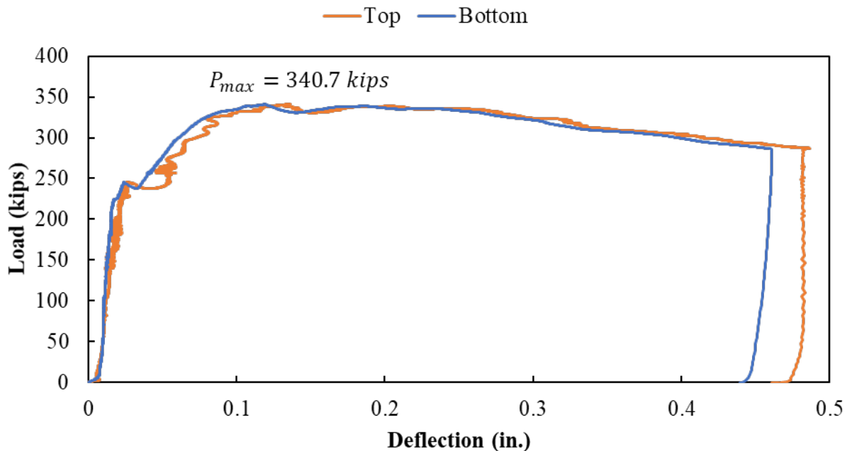
Figure A.167: Load versus deflection curve for Specimen S3-5
