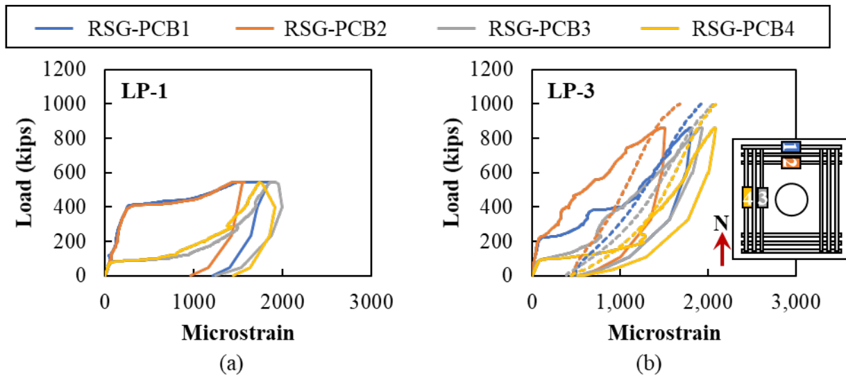
Figure 4.37: Rebar strain in longitudinal bars on bottom of (a) LP-1 (smooth with 1/16-inch roughness) and (b) LP-3 (corrugated with 1/16-inch roughness)
