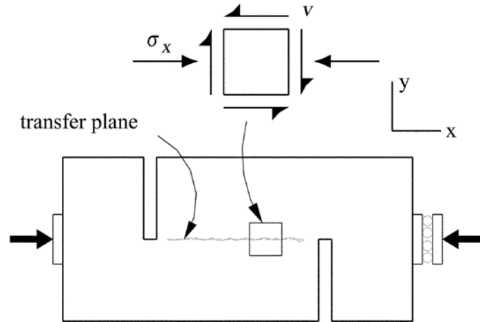
Figure 2.2: Typical push-off specimen and state of stress along shear transfer plane [1]
