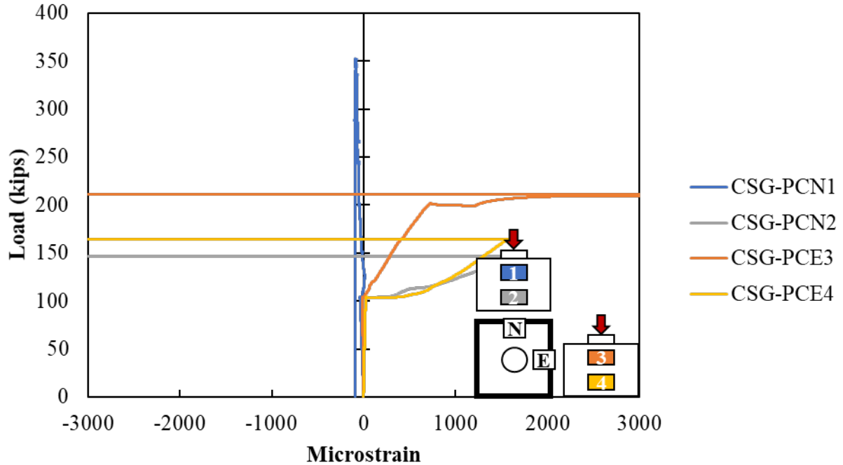
Figure A.210: Concrete strain gauges in the surface of the cap of Specimen S3-11
