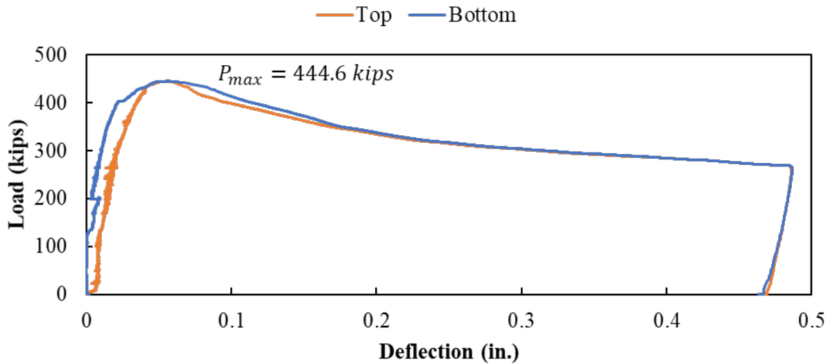
Figure A.147: Load versus deflection curve for Specimen S3-2
