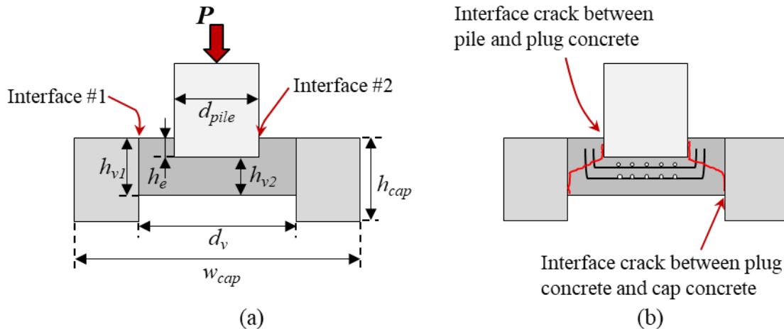
Figure 6.9: Socket specimen: (a) interface detail and (b) failure characteristics
