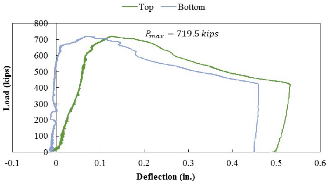
Figure A.63: Load versus deflection curve for Specimen S2-7
