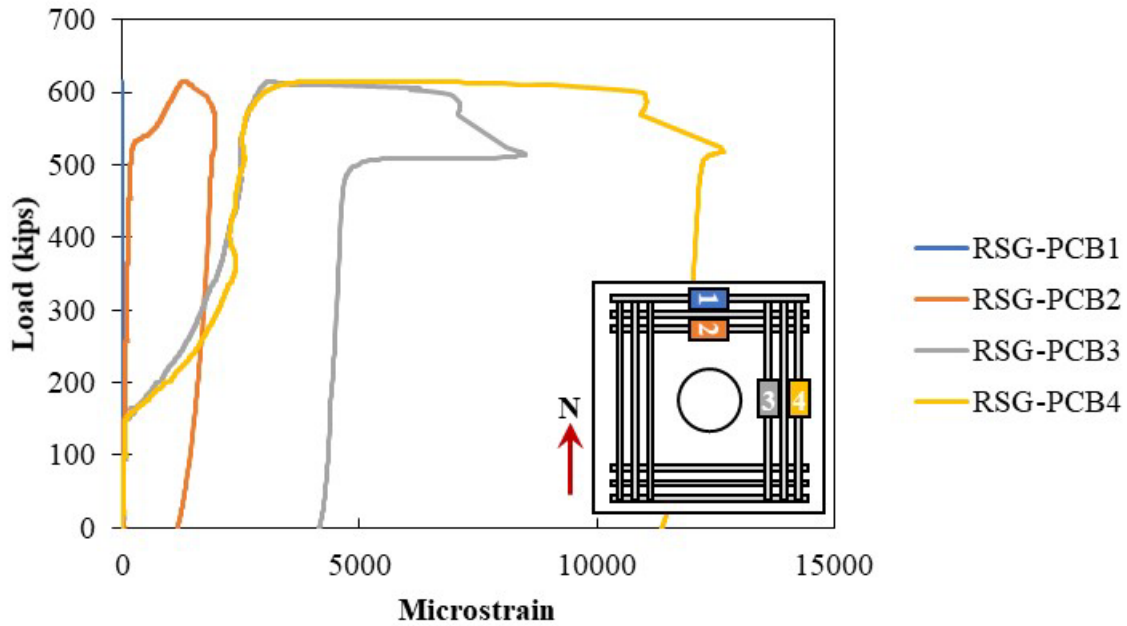
Figure A.43: Rebar strain gauges in longitudinal reinforcement in the bottom of Specimen S2-4
