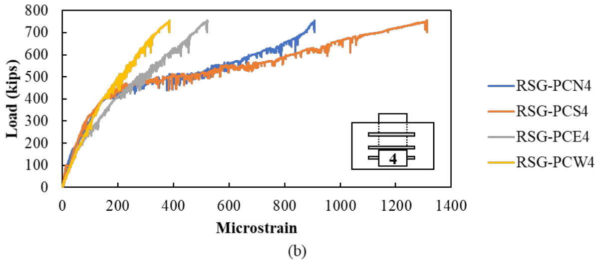
Figure A.8: Rebar strain gauges on confining reinforcement at (a) top and (b) bottom of the plug of Specimen SI-2
