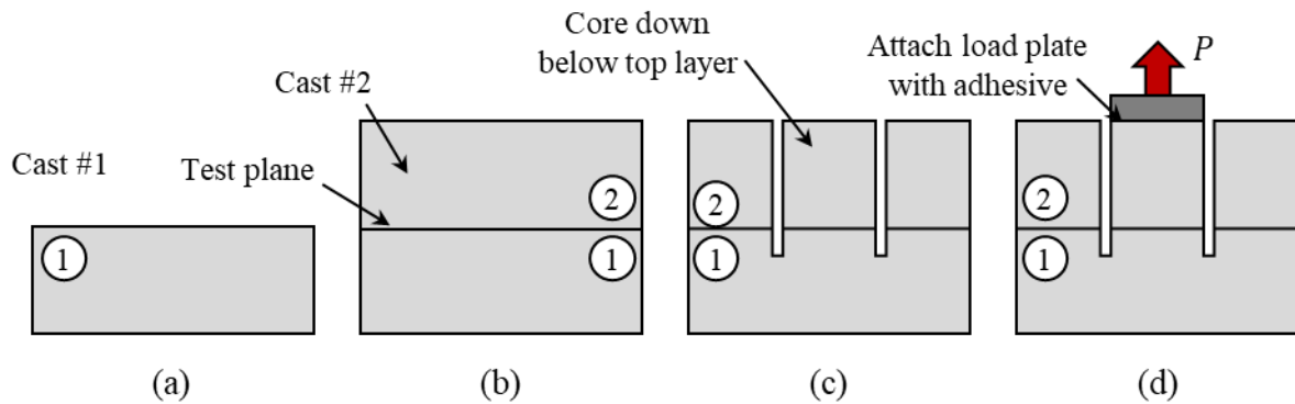
Figure 2.13: Casting and testing procedure for alternate pull-off test: (a) casting of first layer, (b) casting of second layer, (c) core through top layer into bottom layer, and (d) attach load plate and apply tensile force to failure
