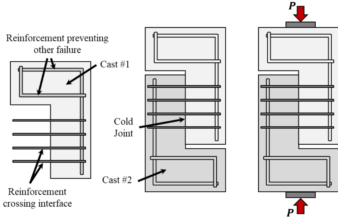
Figure 2.7: Typical casting and testing procedure for push-off tests: (a) casting of first L-shaped component, (b) casting of second L-shaped component, and (c) testing of push-off specimen
