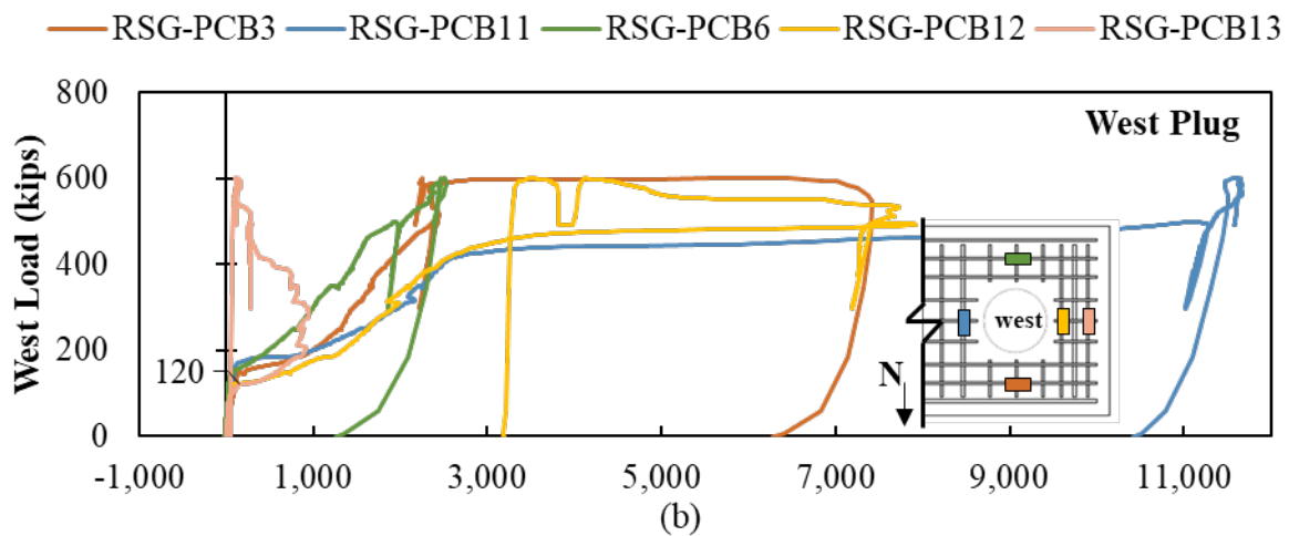
Figure B.31: Rebar strain gauges in the longitudinal reinforcement on bottom of Specimen MP-1
