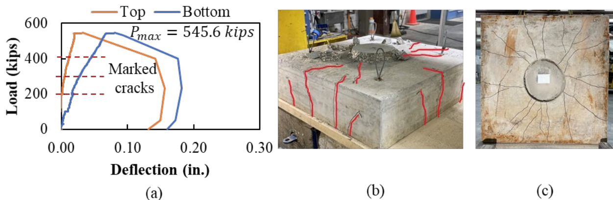
Figure 4.9: (a) Sample load versus deflection plot with stops, (b) crack pattern after failure, and (c) crack pattern on bottom specimen after failure for Specimen LP-1
