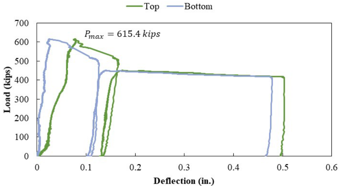
Figure A.42: Load versus deflection curve for Specimen S2-4
