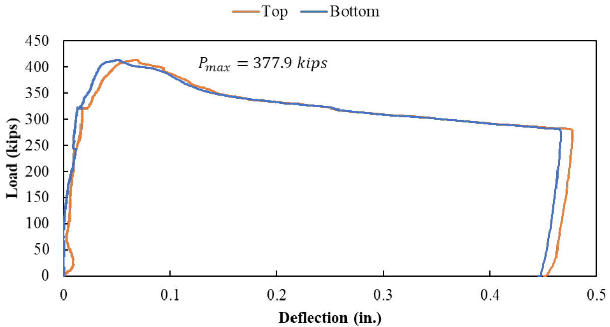
Figure A.180: Load versus deflection curve for Specimen S3-7
