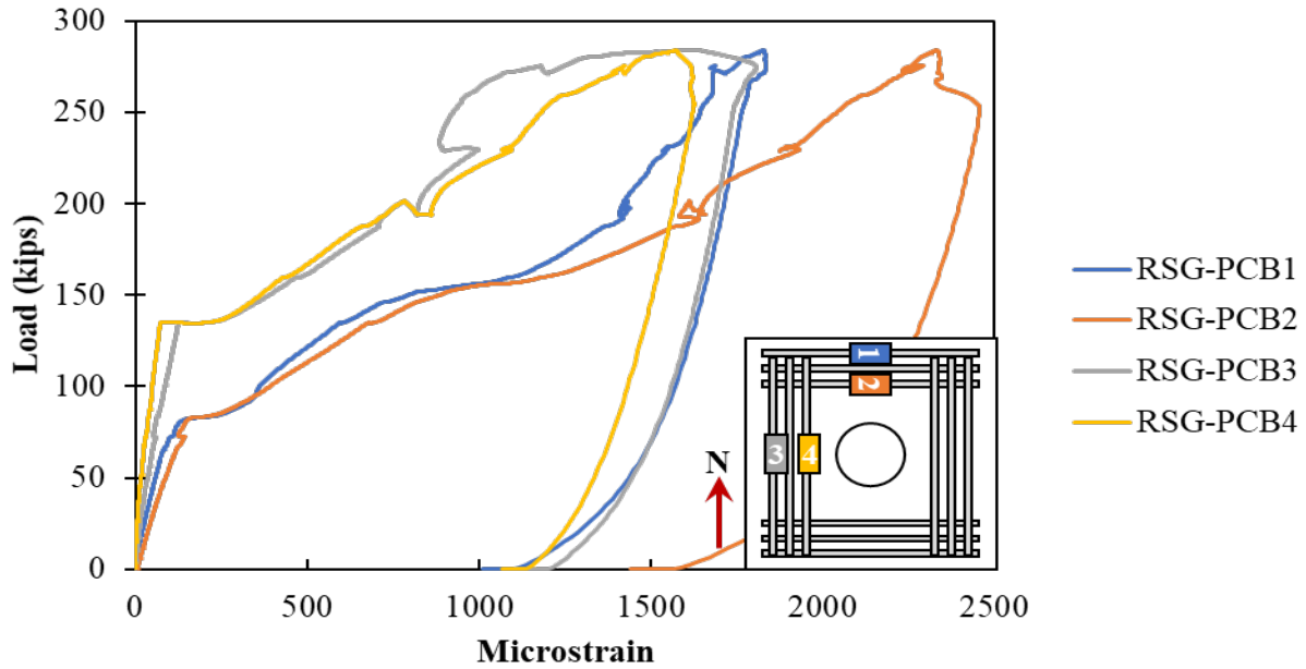
Figure A.174: Rebar strain gauges in the longitudinal reinforcement on the bottom of Specimen S3-6
