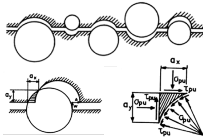
Figure 2.17: Transmission of forces between crack faces (mechanical interlocking) [10]
