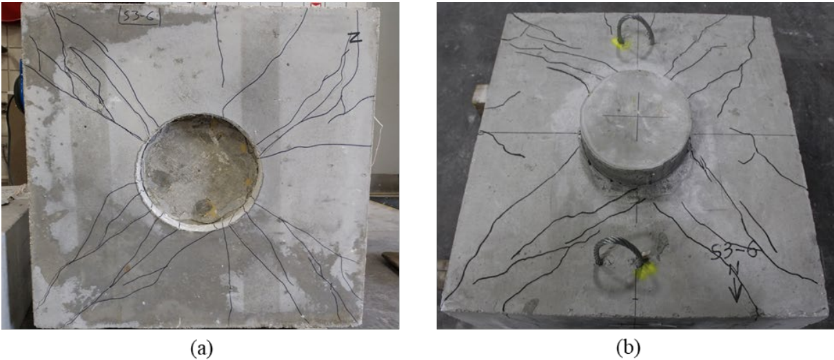
Figure A.176: Cracking after testing on (a) bottom and (b) top of Specimen S3-6
