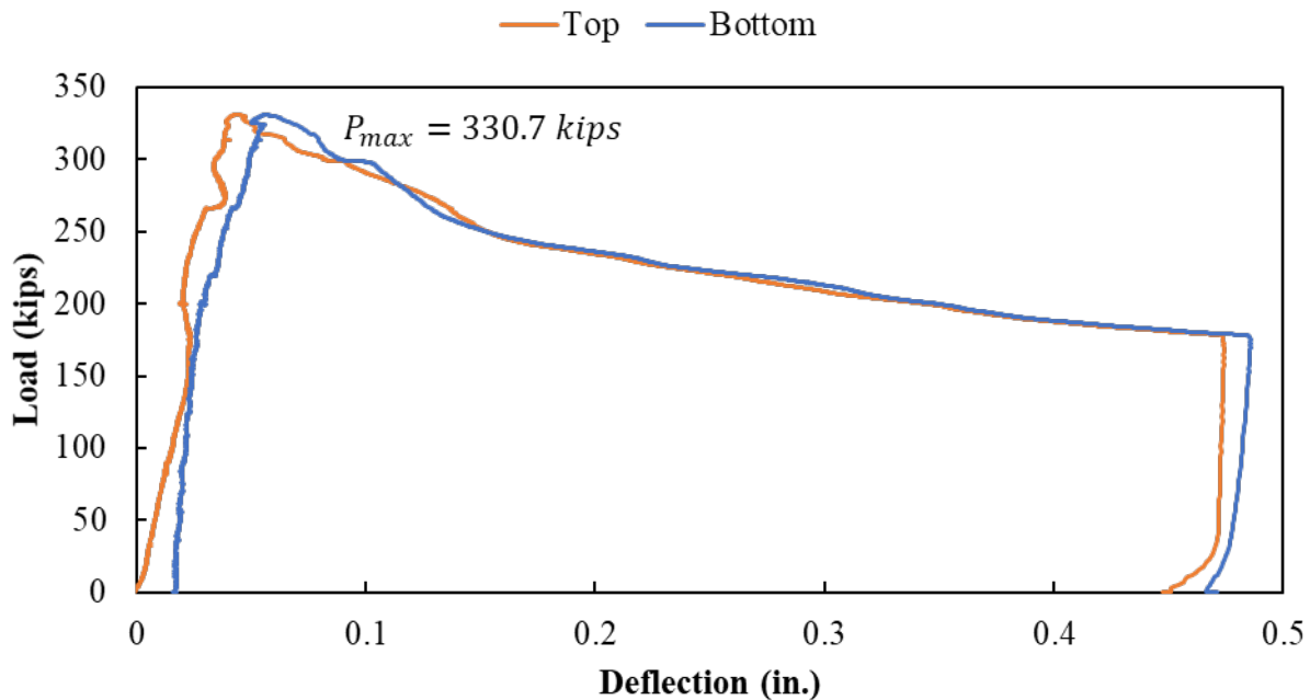
Figure A.201: Load versus deflection curve for Specimen S3-10
