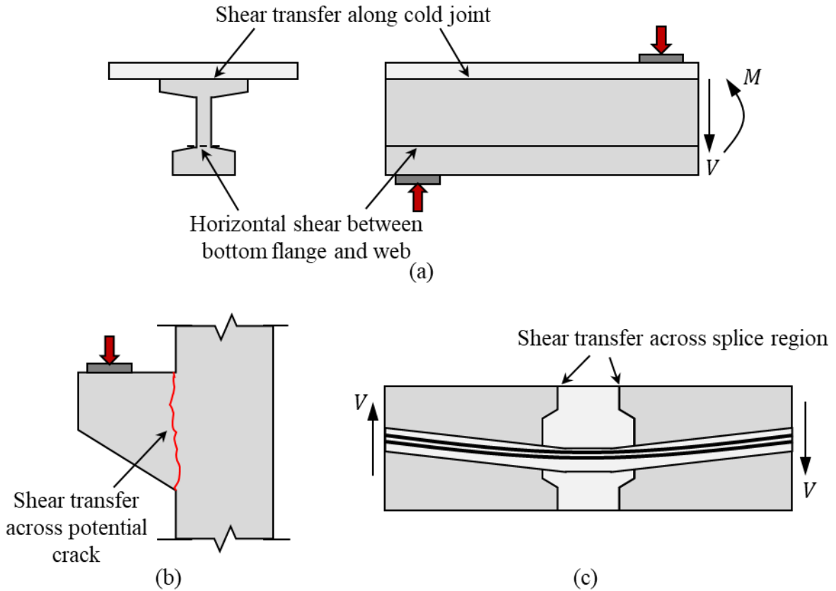
Figure 2.1: Examples of shear friction in (a) composite girder, (b) corbel, and (c) splice region (or other joint between precast members)
