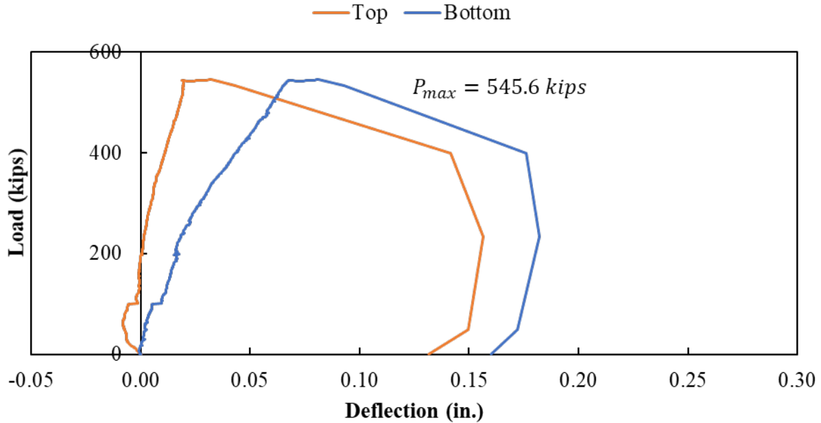
Figure B.1: Load versus displacement curve for Specimen LP-1
