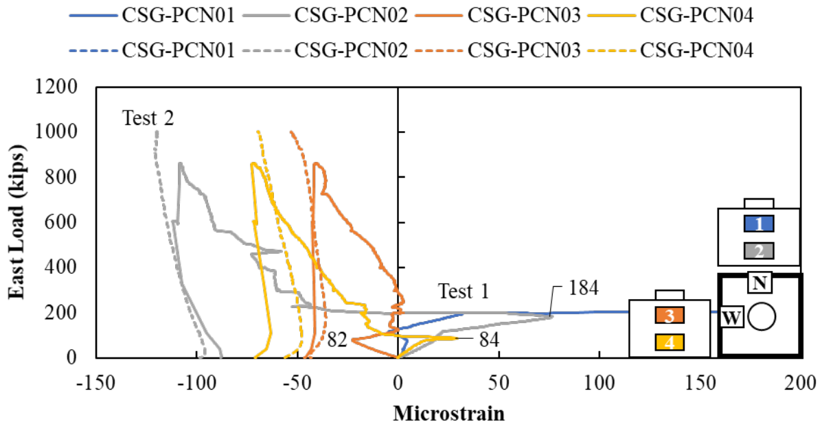
Figure B.18: Concrete strain gauges in the surface of Specimen LP-3
