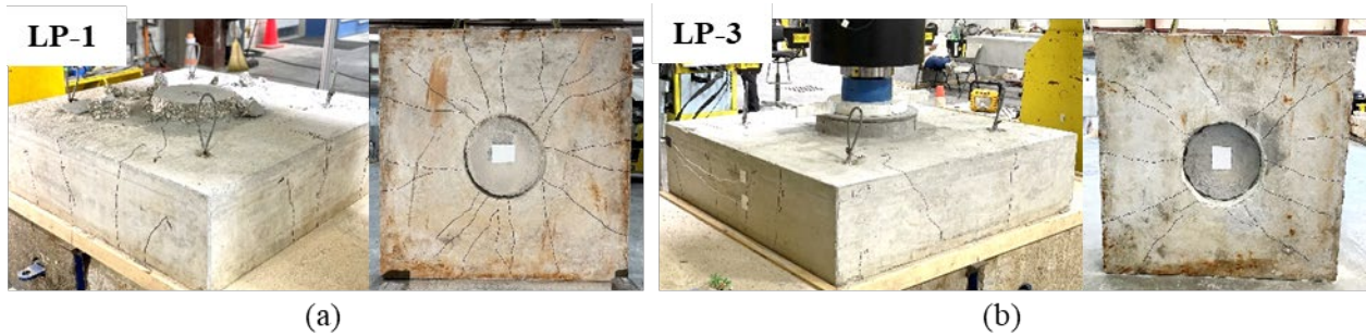
Figure 4.35: Crack patterns at failure for (a) LP-1 (smooth with 1/16-inch roughness) and (b) LP-3 (corrugated with 1/16-inch roughness)
