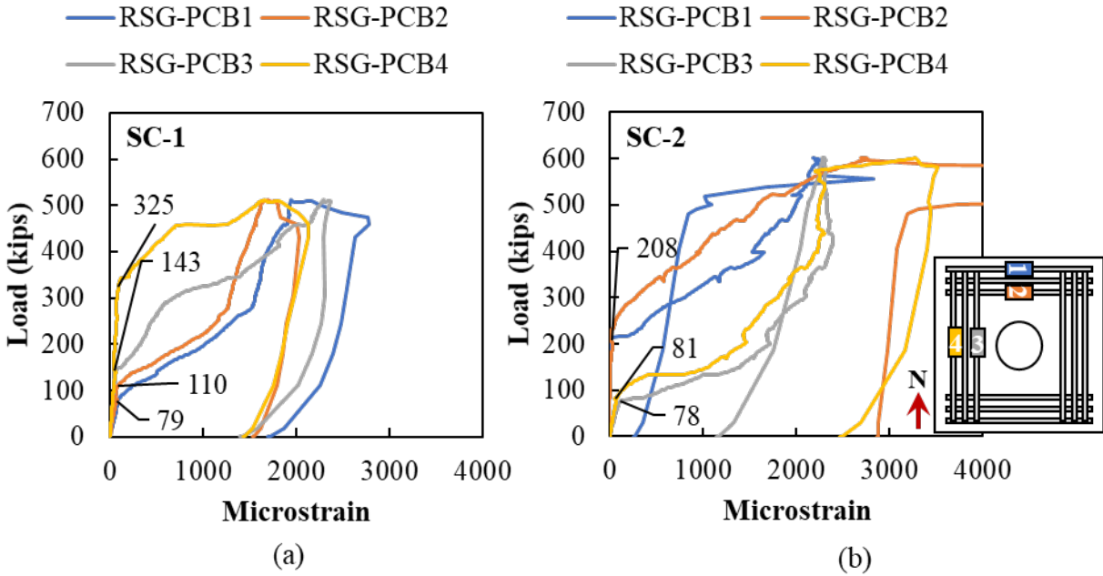
Figure 4.31: Load versus strain in longitudinal reinforcement for (a) SC-1 and (b) SC-2
