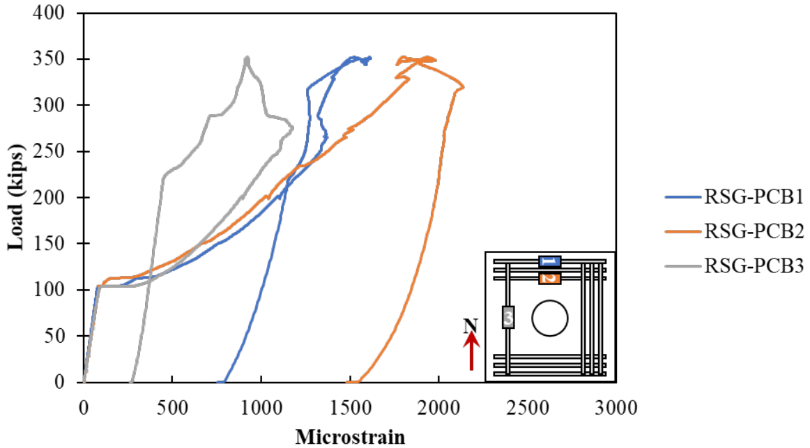
Figure A.209: Rebar strain gauges in the longitudinal reinforcement on the bottom of Specimen S3-11
