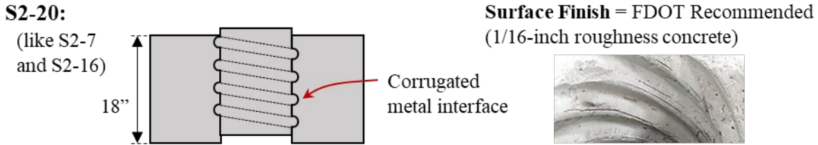
Figure A.135: Details for S2-20
