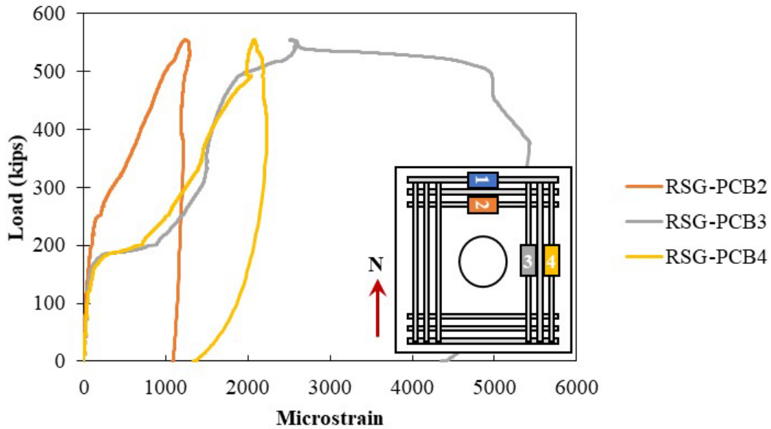
Figure A.71: Rebar strain gauges in the longitudinal reinforcement on the bottom of Specimen S2-8
