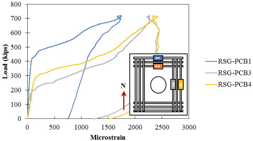
Figure A.64: Rebar strain gauges in the longitudinal reinforcement on bottom of Specimen S2-7
