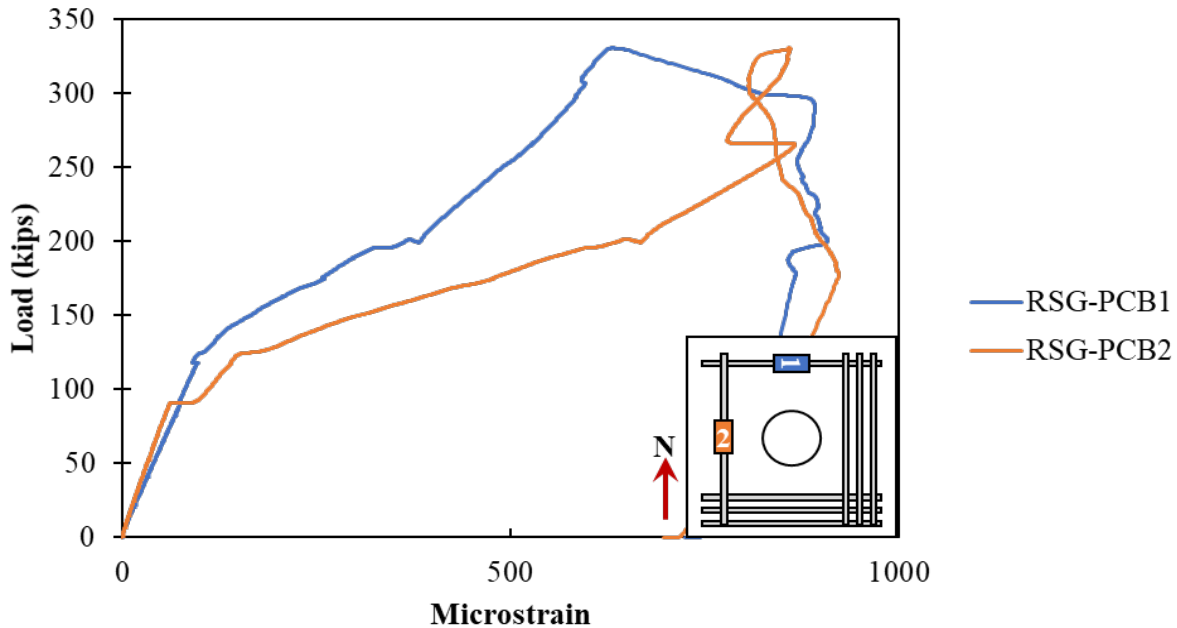
Figure A.202: Rebar strain gauges in the longitudinal reinforcement on the bottom of Specimen S3-10
