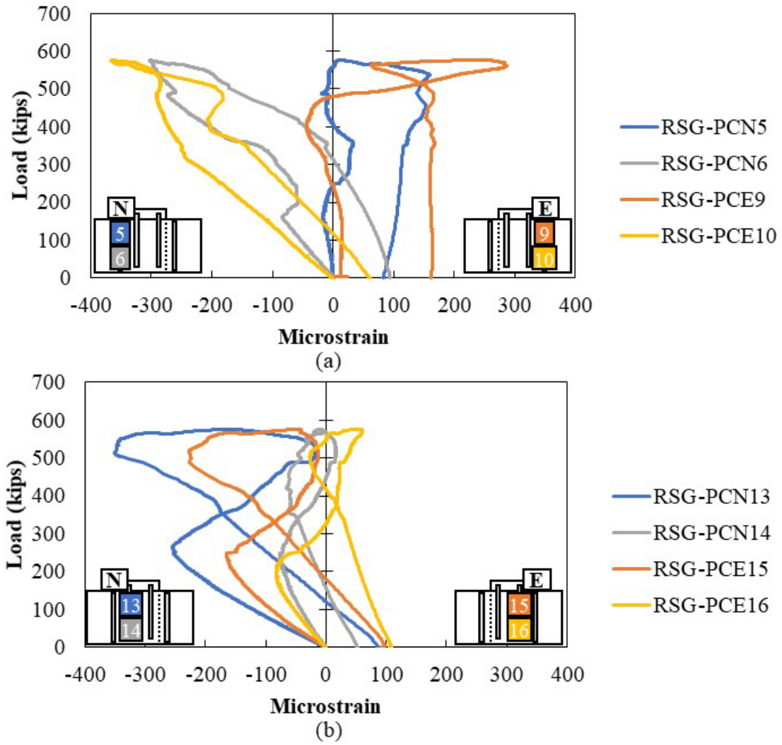
Figure A.90: Rebar strain gauges in vertical reinforcement on (a) cap and (b) plug of Specimen S2-10
