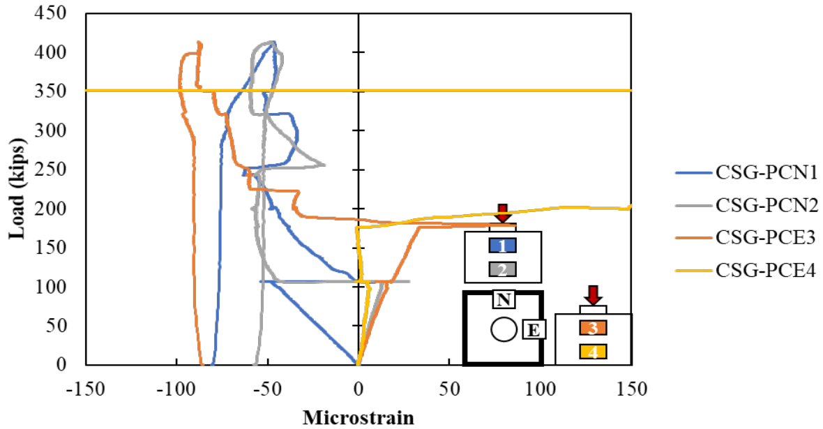
Figure A.182: Concrete strain gauges in the surface of the cap of Specimen S3-7
