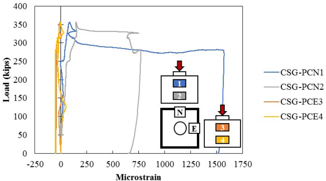
Figure A.51: Concrete strain gauges in the surface of Specimen S2-5
