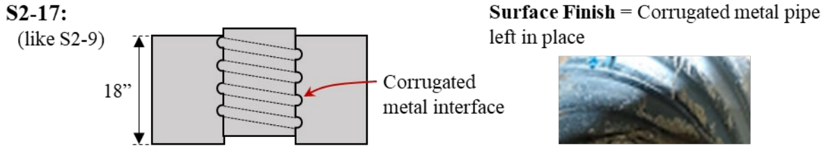
Figure A.123: Details for S2-17
