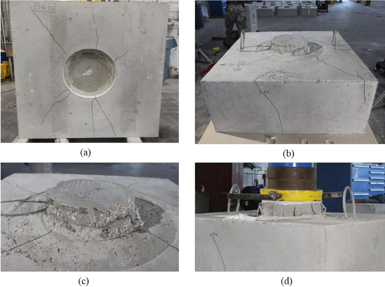
Figure A.224: Failure details on (a) bottom, (b) cap, (c) top of plug and (d) plug detail during testing of the Specimen S3-13
