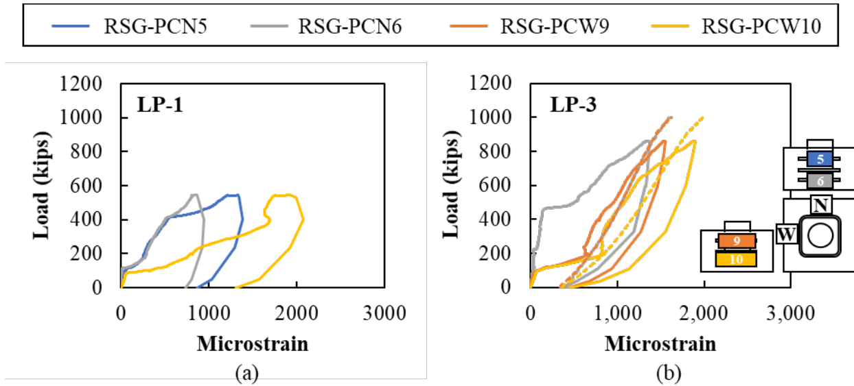
Figure 4.36: Rebar strain in confinement reinforcement around the pocket of (a) LP-1 (smooth with 1/16-inch roughness) and (b) LP-3 (corrugated with 1/16-inch roughness)
