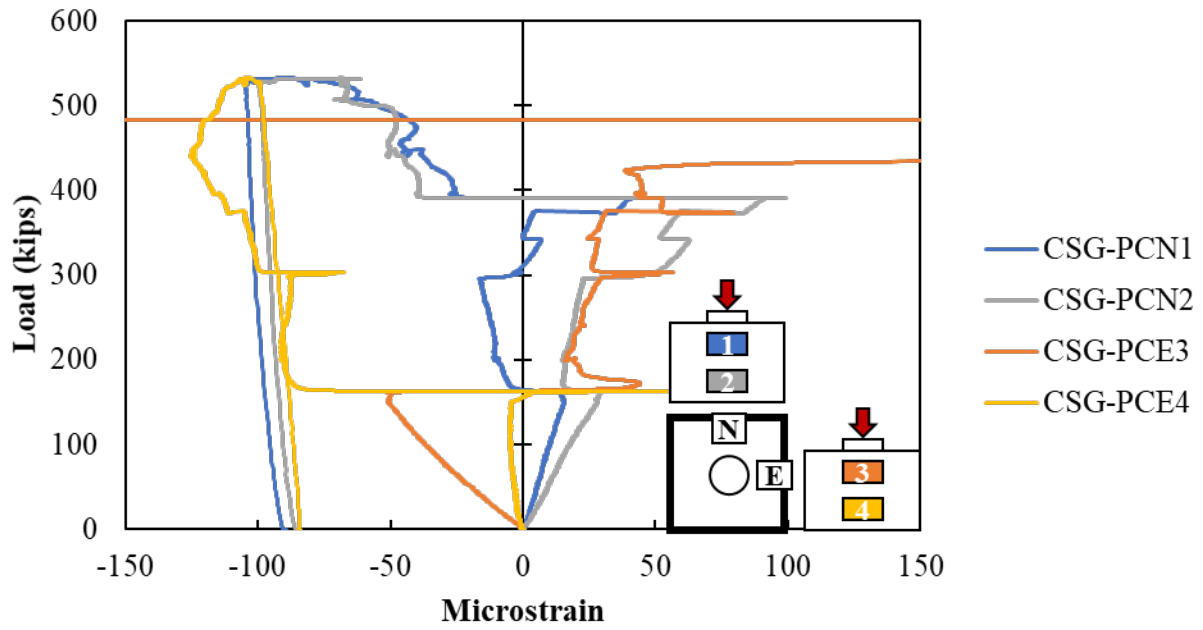
Figure A.125: Concrete strain gauges on the concrete surface of Specimen S2-17
