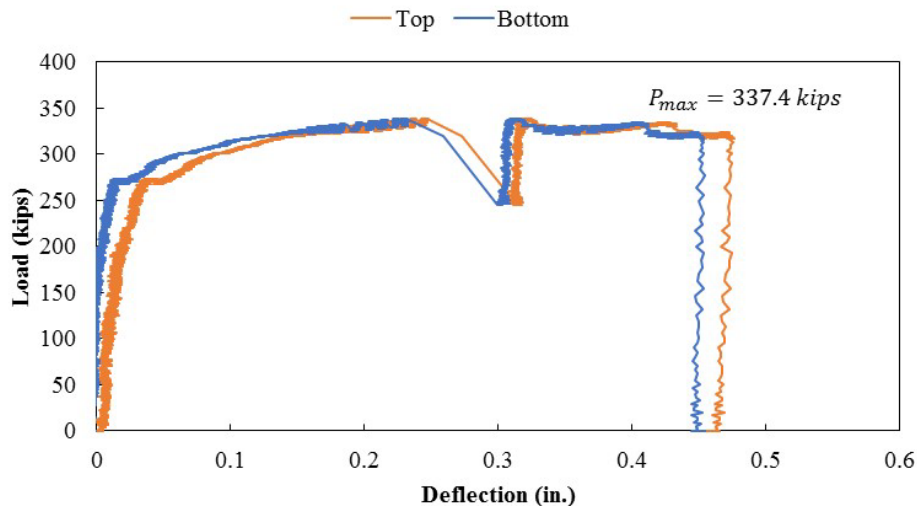
Figure A.21: Load-displacement curve for Specimen S2-1
