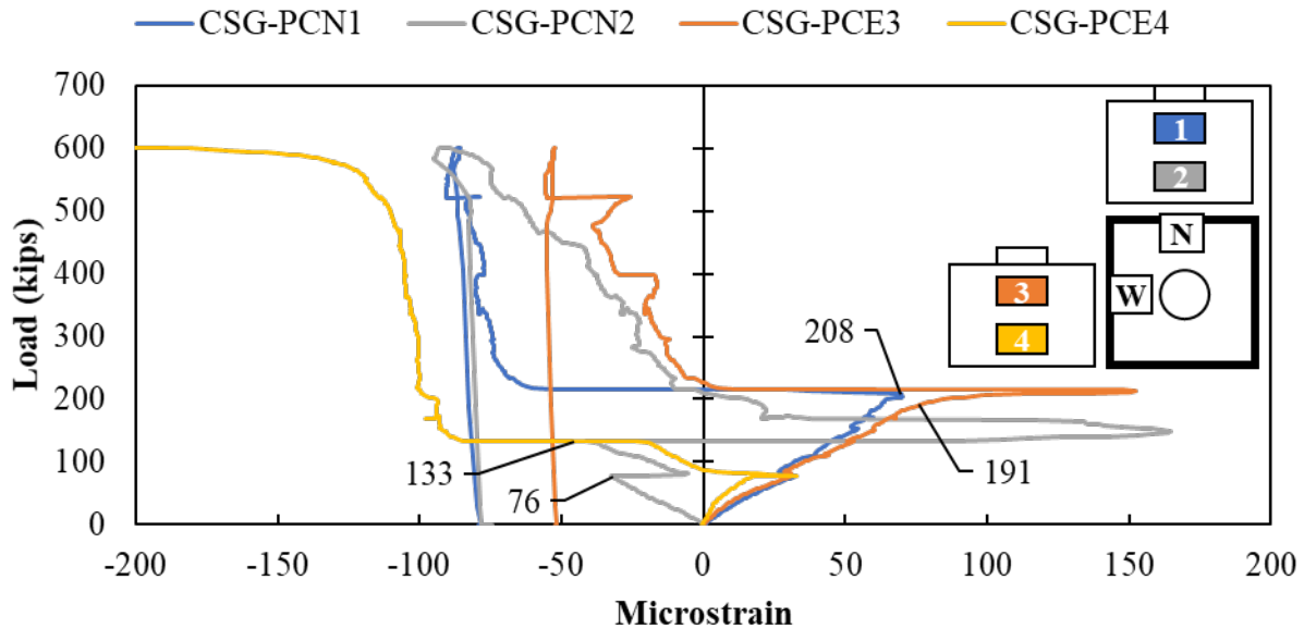
Figure B.55: Concrete strain gauges in the concrete surface of Specimen SC-2
