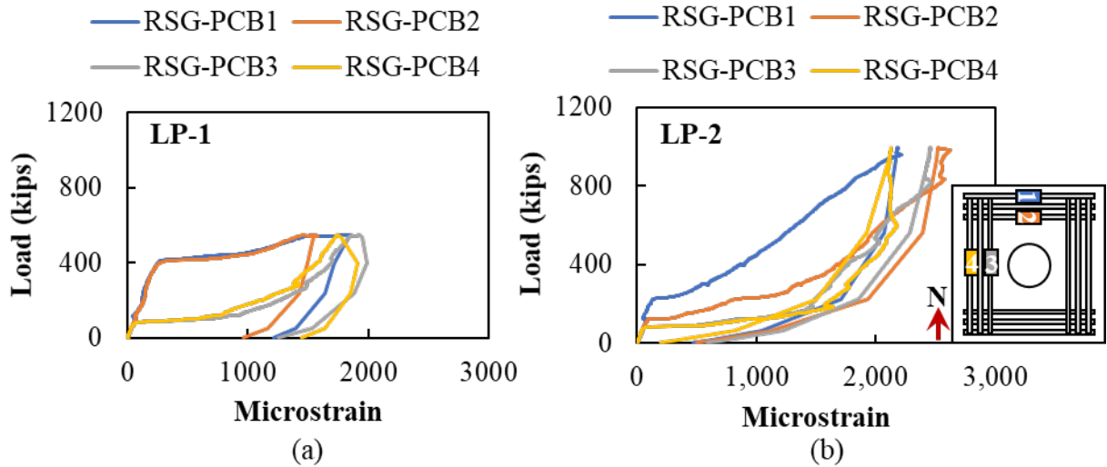
Figure 4.28: Rebar strain in longitudinal bars on bottom of (a) LP-1 (1/16-inch roughness) and (b) LP-2 (1/4-inch roughness) without corrugations
