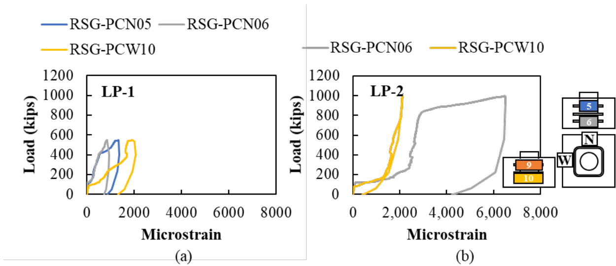
Figure 4.27: Rebar strain in confinement reinforcement around the pocket of (a) LP-1 (1/16-inch roughness) and (b) LP-2 (1/4-inch roughness) without corrugations
