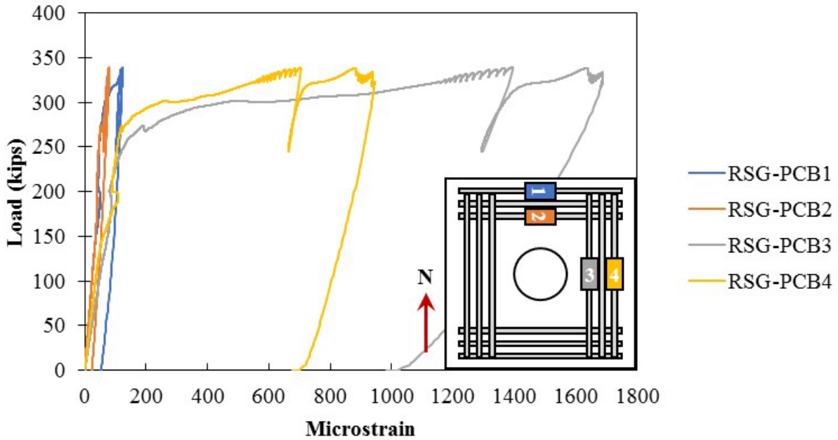
Figure A.22: Rebar strain in the longitudinal bars on bottom of the Specimen S2-1
