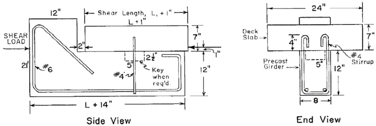
Figure 2.8: Push-off specimen in casting position for looking at interface between beam and composite deck [26].
