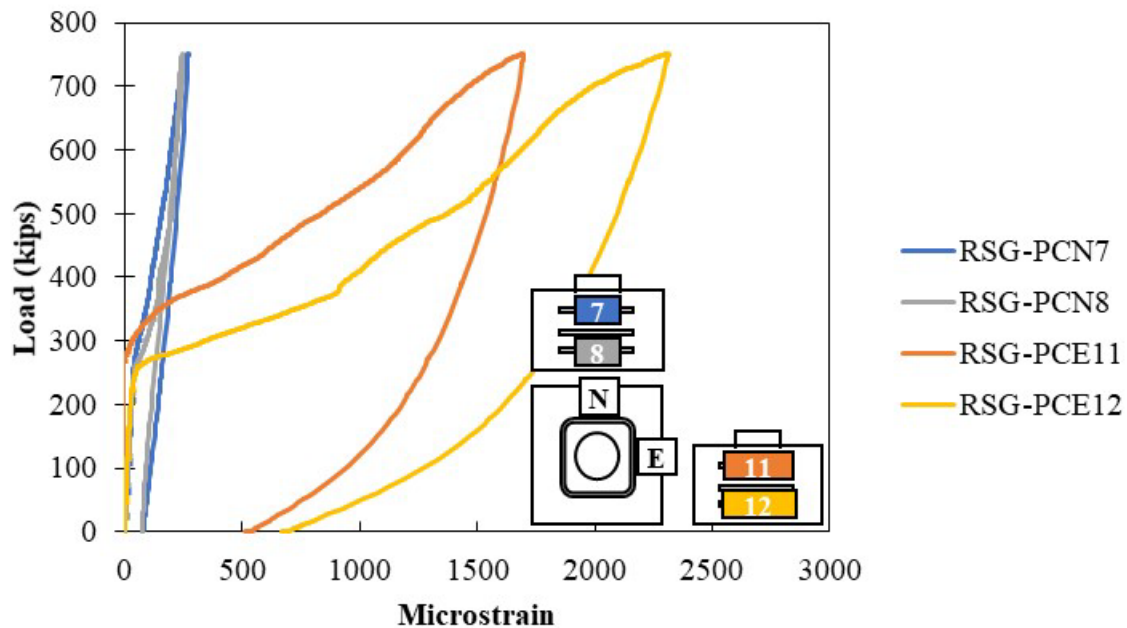
Figure A.32: Rebar strain gauges on confining reinforcement around the pocket of Specimen S2-2
