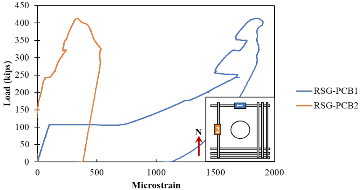
Figure A.181: Rebar strain gauges in the longitudinal reinforcement on the bottom of Specimen S3-7
