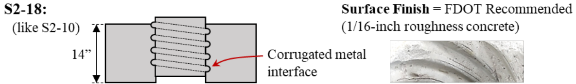
Figure A.127: Details for S2-18
