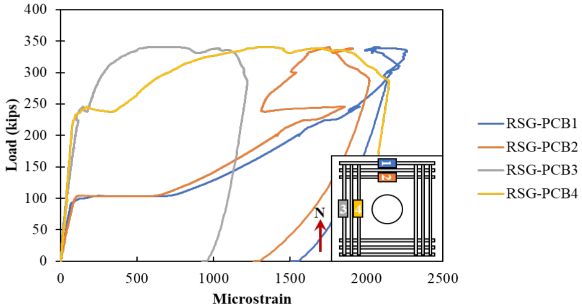
Figure A.168: Rebar strain gauges in the longitudinal reinforcement on bottom of Specimen S3-5
