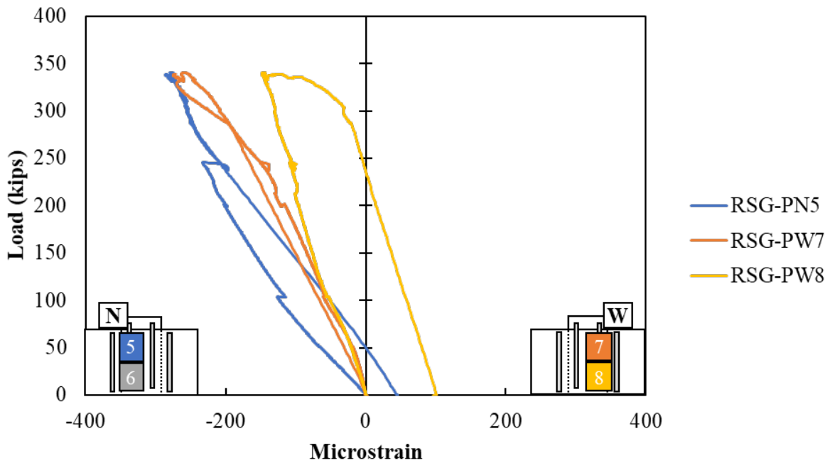
Figure A.171: Rebar strain gauges in vertical reinforcement on plug of Specimen S3-5
