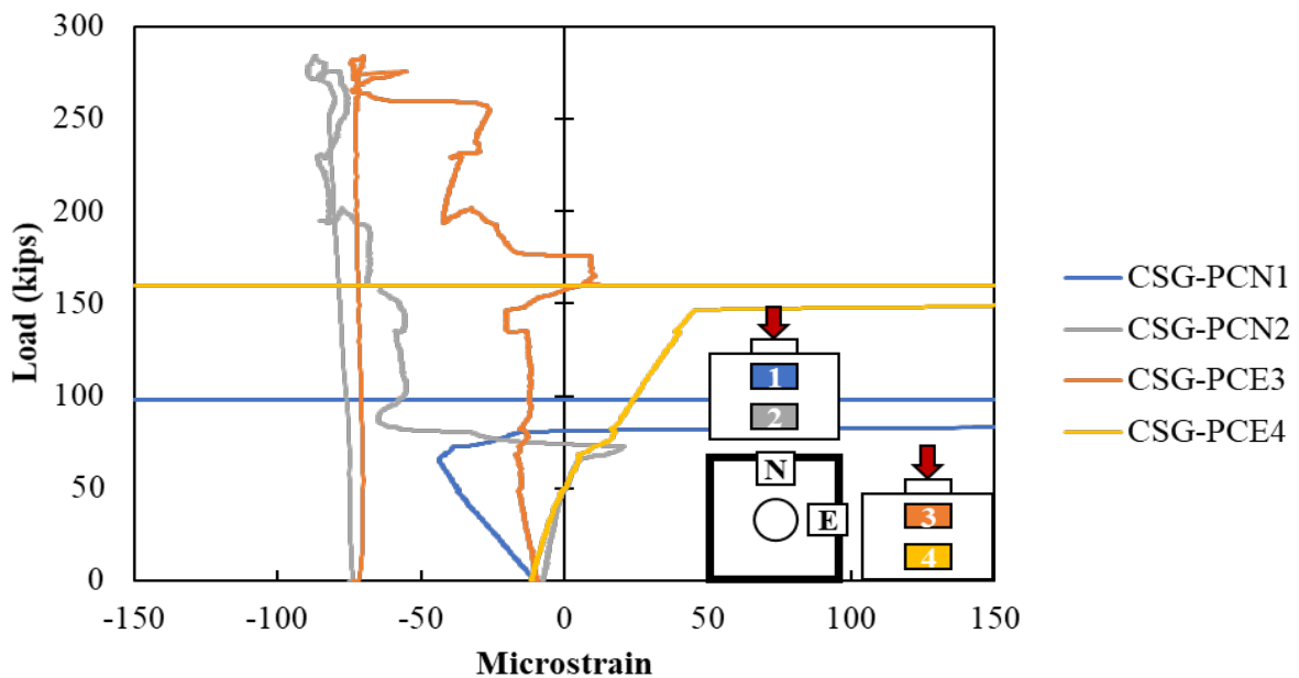
Figure A.175: Concrete strain gauges in the surface of the cap of Specimen S3-6
