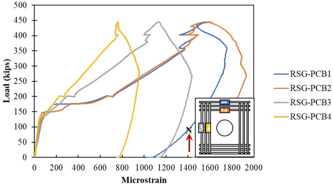
Figure A.148: Rebar strain gauges in the longitudinal reinforcement on bottom of Specimen S3-2
