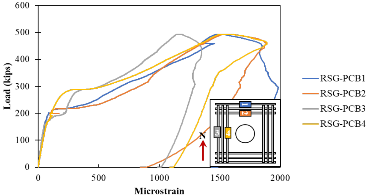
Figure A.161: Rebar strain gauges in the longitudinal reinforcement on the bottom of Specimen S3-4 Cracking was also observed in the surface concrete at a load of around 200 kips on the north and east side of the specimen according to CSG-PCN2 and CSG-PCE4, as shown in Figure A.162.
