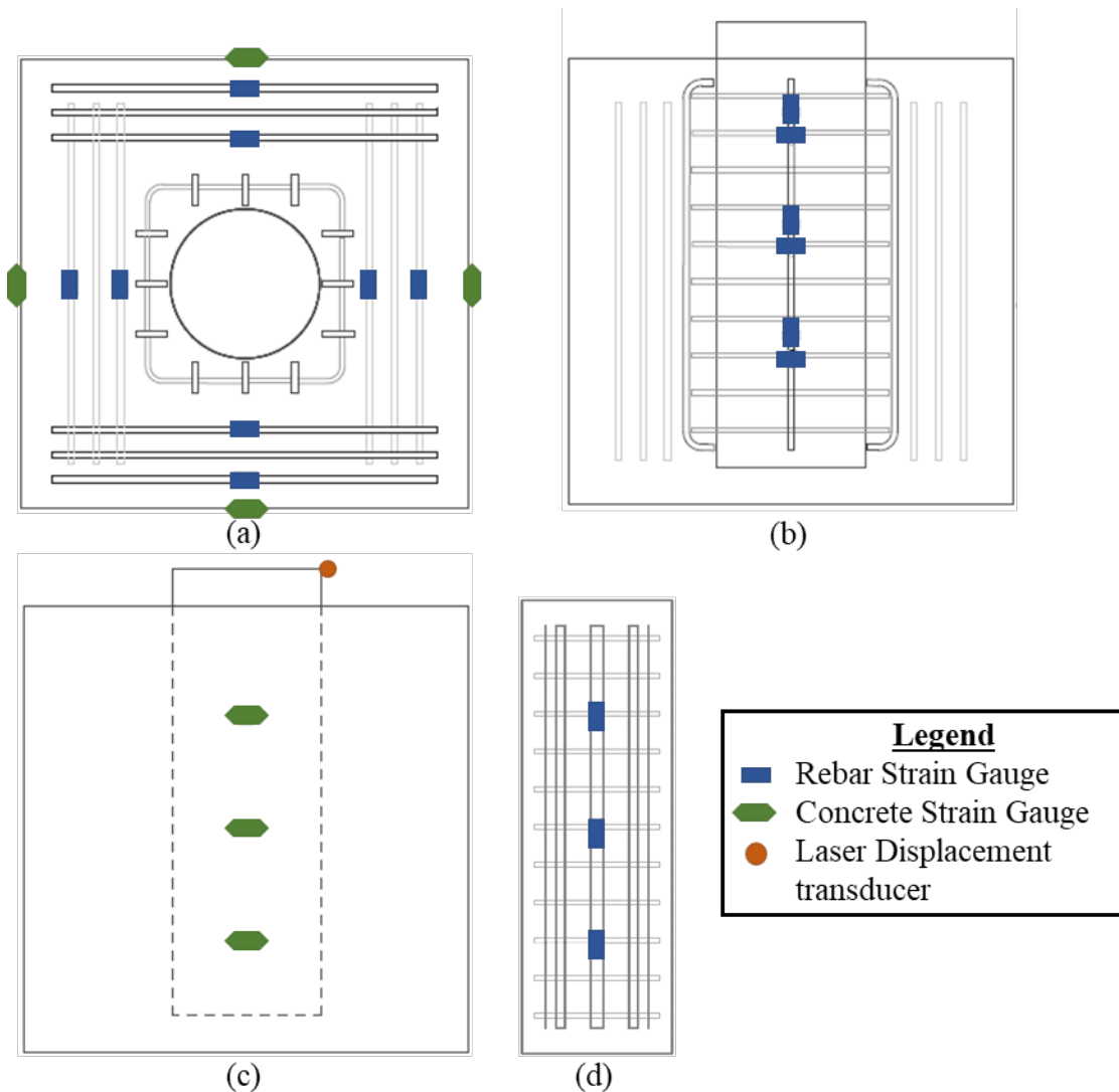
Figure 3.12: Instrumentation plan for Series I specimens: (a) pile cap bottom view (b) cap-elevation (c) pile cap, and (d) plug elevation.
