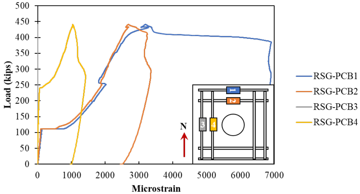
Figure A.154: Rebar strain gauges in the longitudinal reinforcement on bottom of Specimen S3-3
