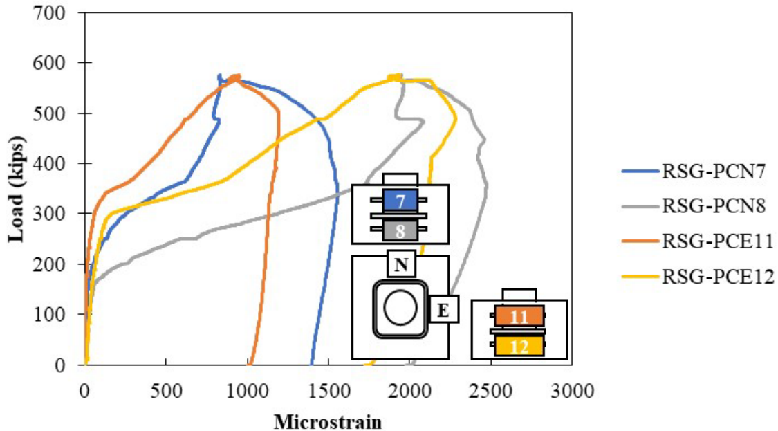
Figure A.89: Confining reinforcement around the pocket of Specimen S2-10
