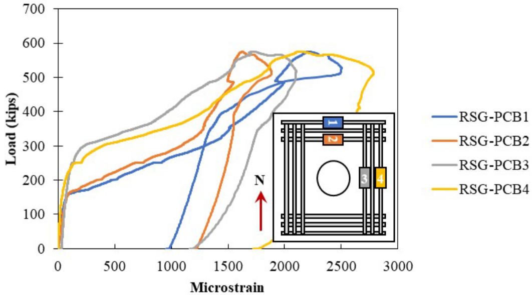
Figure A.86: Rebar strain gauges in the longitudinal reinforcement on bottom of Specimen S2-10
