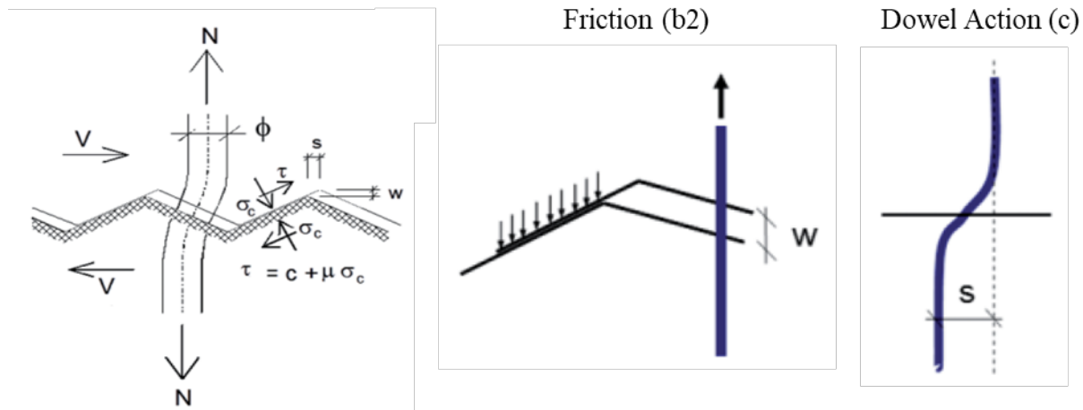
Figure 2.18: Shear resistance mechanisms when reinforcement is crossing interface [10]
