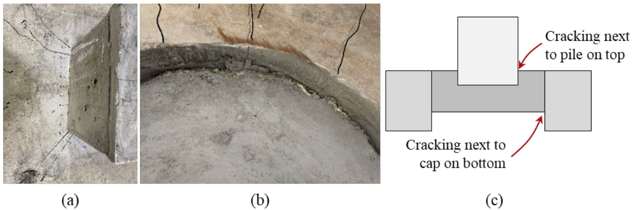
Figure 6.8: Location of cracking in socket specimens, SC-1 shown, (a) on top next to the pile, (b) on bottom next to the cap, and (c) schematic highlighting location of cracking
