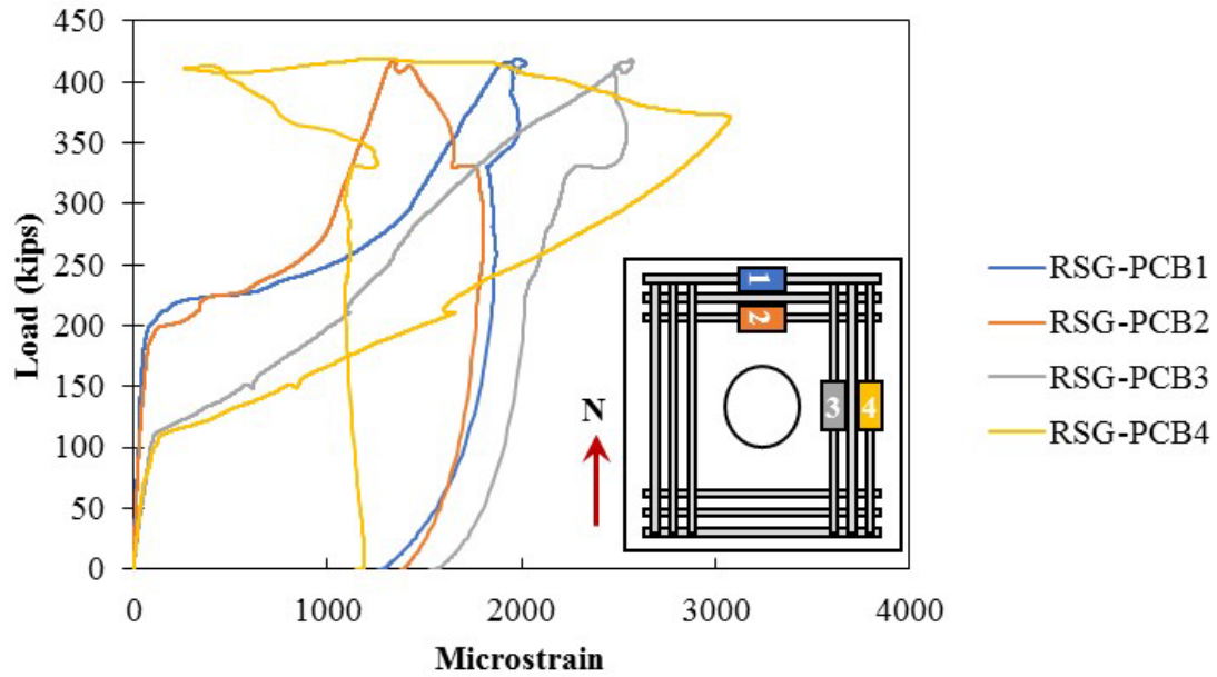
Figure A.57: Rebar strain gauges in the longitudinal reinforcement on bottom of Specimen S2-6
