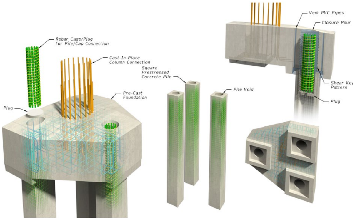
Figure 6.5: Sample detail for precast footings provided in FDOT Structures Detailing Manual [52]
