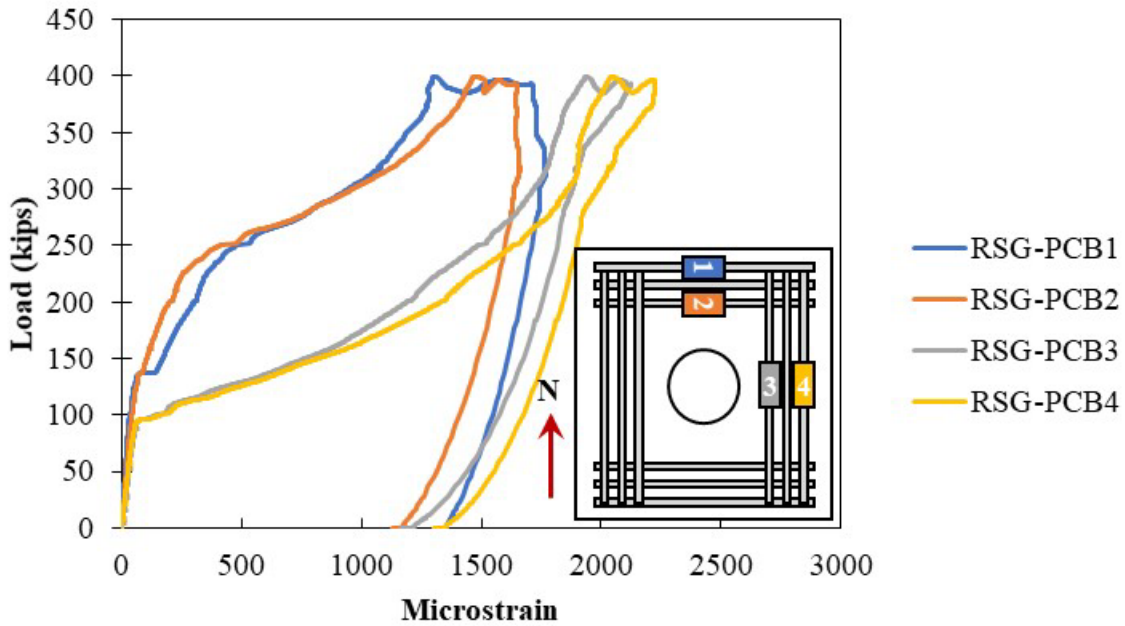
Figure A.93: Rebar strain gauges in the longitudinal reinforcement on the bottom of Specimen S2-11
