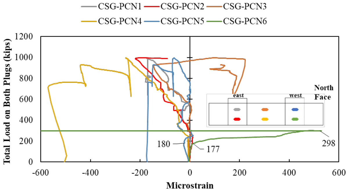
Figure B.33: Concrete strain gauges on the concrete surface of Specimen MP-1
