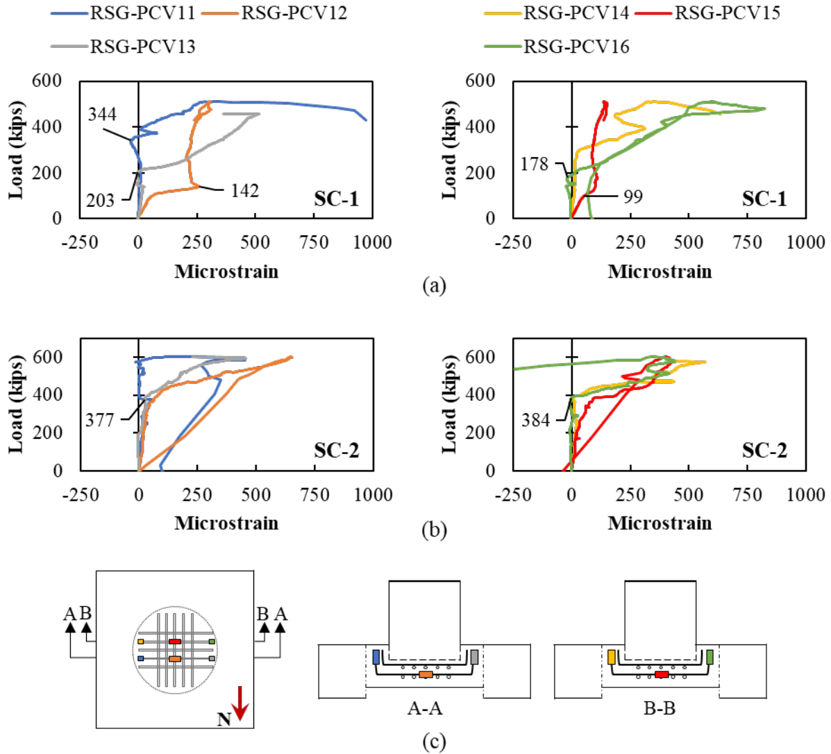
Figure 4.33: Load versus strain in socket reinforcement below pile in E-W direction for (a) SC-1 and (b) SC-2 and (c) location of RSGs
