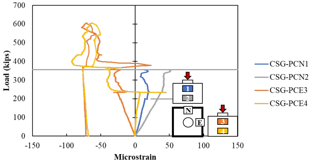
Figure A.109: Concrete strain gauge on the concrete surface of Specimen S2-13
