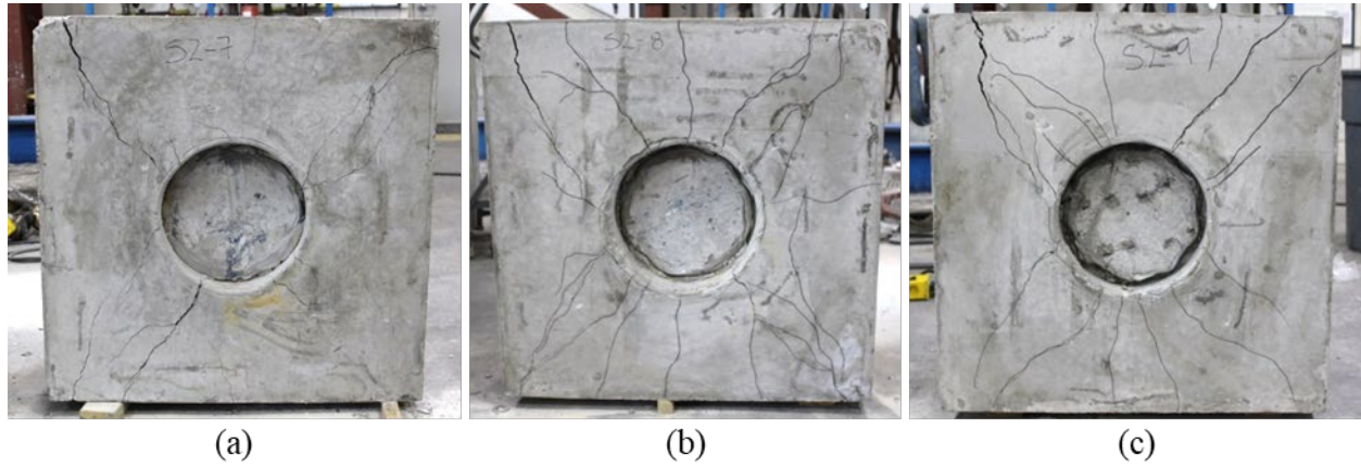
Figure 3.19: Sample crack patterns on the bottom of specimens (a) S2-7, (b) S2-8, and (c) S2-9
