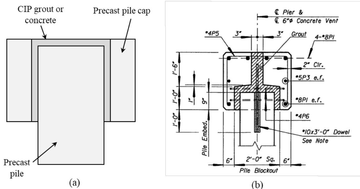
Figure 2.20: Examples of socket connections between pile cap and pile: (a) connection between two precast elements; (b) connection used in Parker River bridge (2007)[50].
