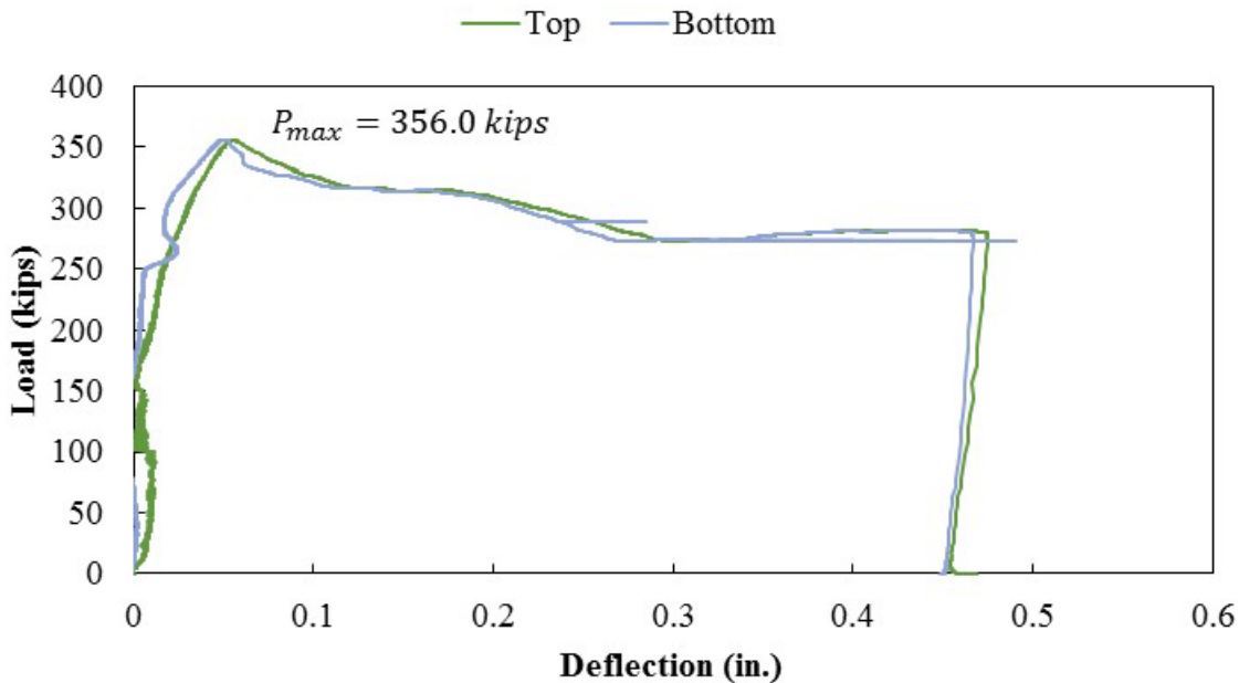
Figure A.49: Load versus deflection curve for Specimen S2-5
