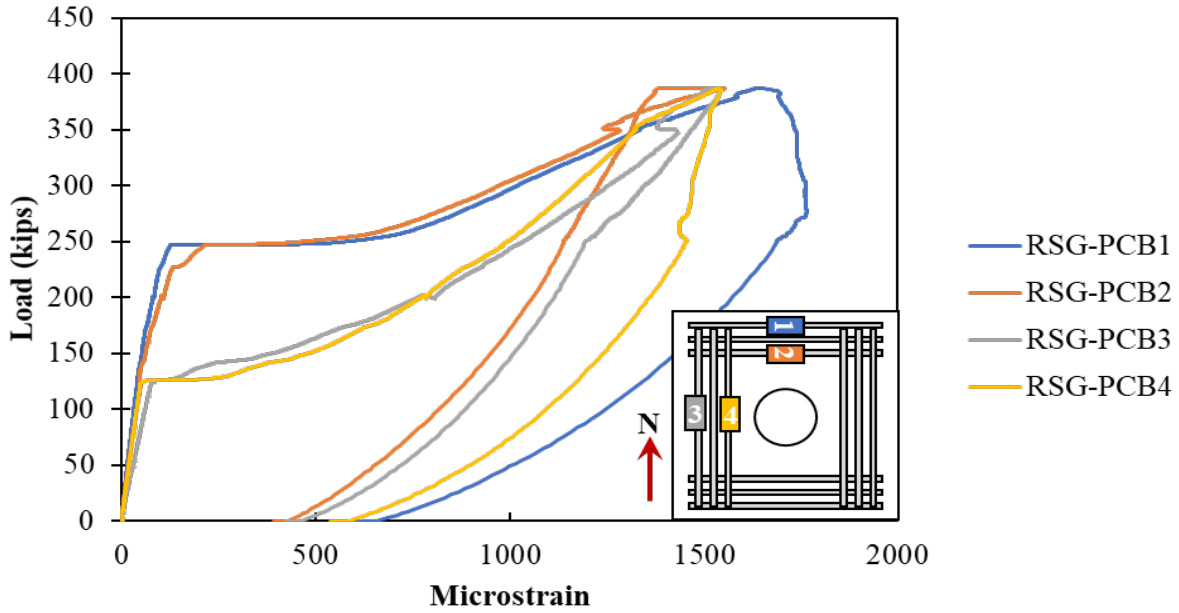
Figure A.222: Rebar strain gauges in the longitudinal reinforcement on the bottom of Specimen S3-13 Cracking was also observed in the surface concrete at a load of around 130 kips on the east side of the specimen (CSG-PCE3 and CSG-PCE4), as shown in Figure A.223. Cracking was seen in the north side of the specimen at a load around 250 kips.
