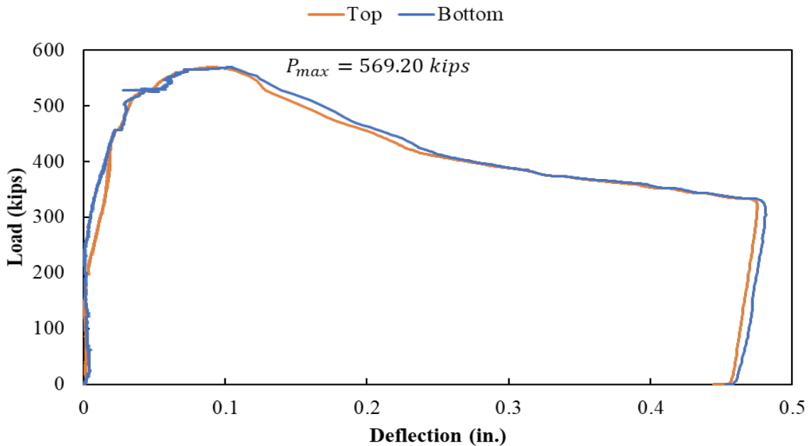
Figure A.128: Load versus displacement curve for Specimen S2-18
