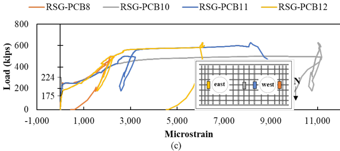
Figure B.38: Rebar strain gauges in the longitudinal reinforcement on bottom of Specimen MP-2
