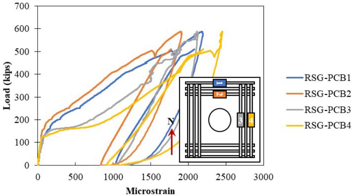
Figure A.78: Rebar strain gauges in the longitudinal reinforcement on bottom of Specimen S2-9
