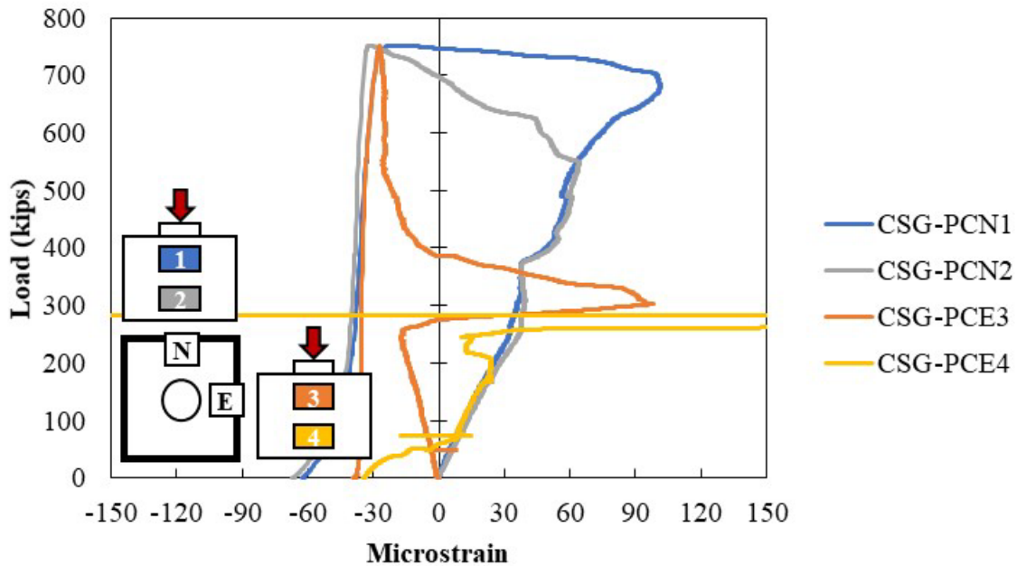
Figure A.30: Concrete surface gauges on the cap of Specimen S2-2
