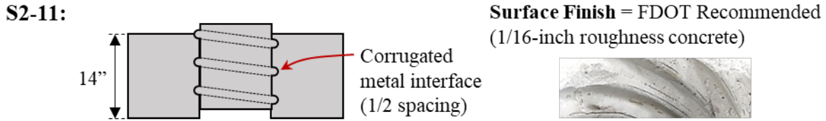
Figure A.91: Details for S2-11
