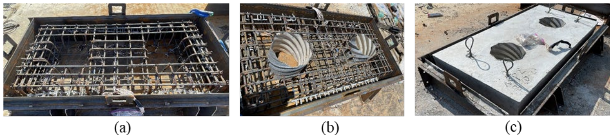
Figure 4.11: Construction and casting of multi-plug specimens: (a) reinforcement layout, (b) corrugated pipes placed, and (c) after concrete had hardened.
