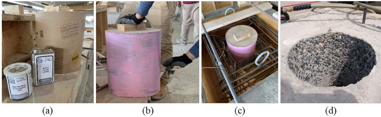
Figure 3.7: Procedure for achieving exposed aggregate finish: (a) application of polyurethane clear coat, (b) application of set retarding agent, (c) placement of void in cap, and (d) finish after pressure washing surface
