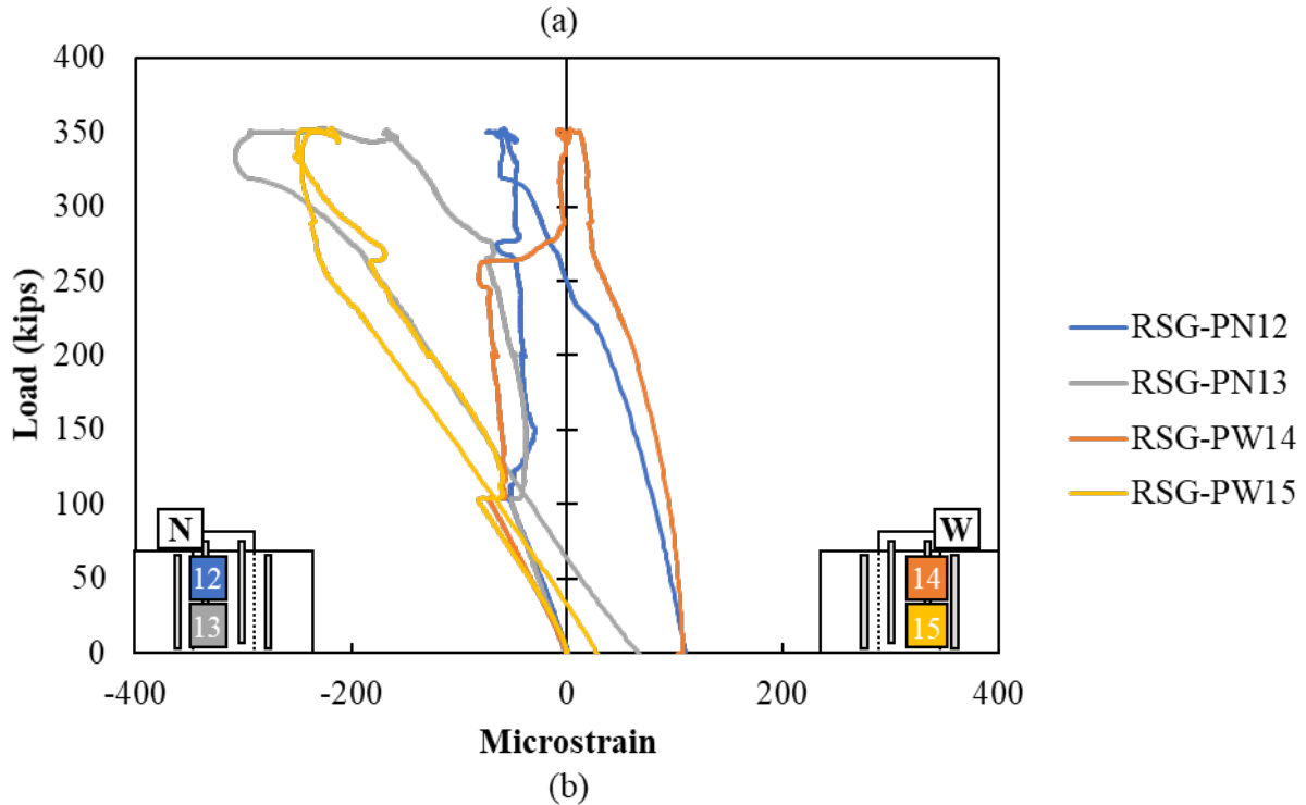
Figure A.213: Rebar strain gauges in vertical reinforcement (a) cap and (b) plug of Specimen S3-11
