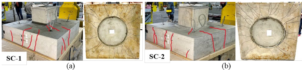
Figure 4.29: Cracking at failure for (a) SC-1 (sandblasted, 1/16-inch finish) and (b) SC-2 (metal pipe left in place)
