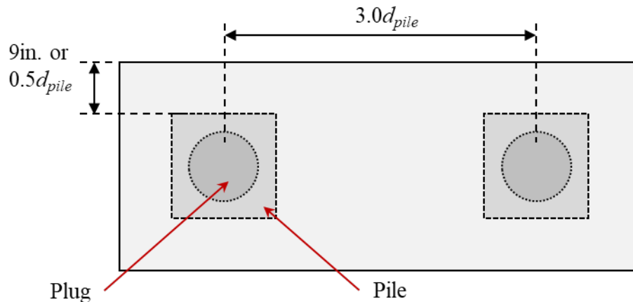
Figure 6.2: Current edge distance and spacing requirements for piles and pile caps in AASHTO LRFD BDS and FDOT SDG
