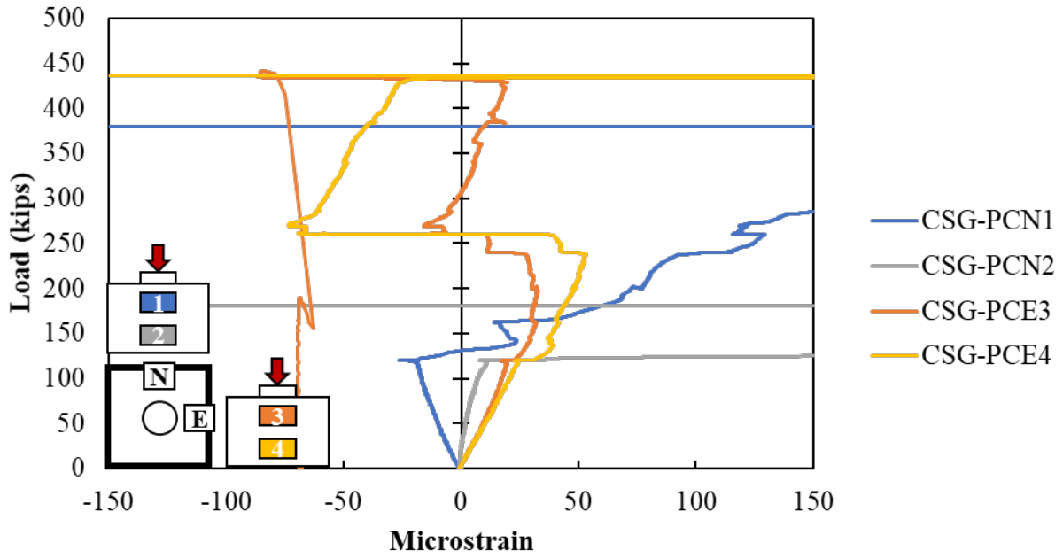
Figure A.113: Concrete strain gauge on the concrete surface of Specimen S2-14
