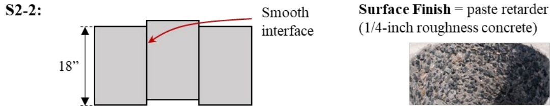
Figure A.27: Details for S2-2
