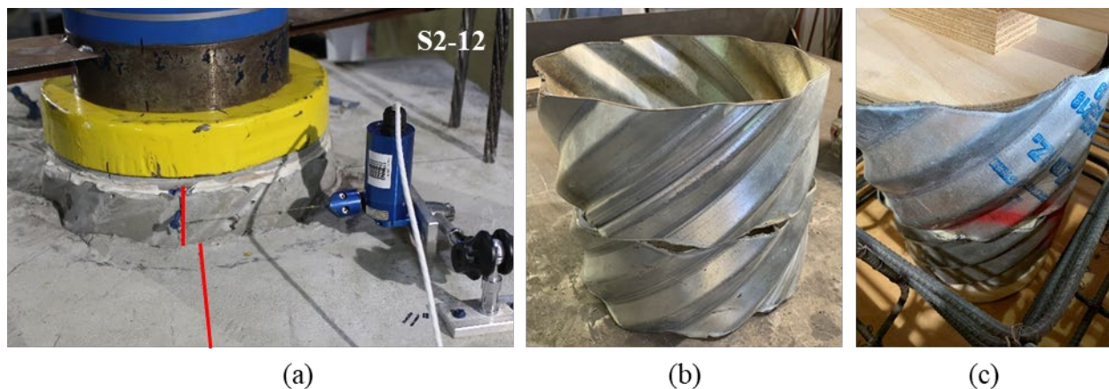
Figure 3.8: (a) Rotation observed in S2-12, (b) detail of the corrugated metal pipe when the pipe was left in place in later specimens, and (c) installed metal pipe with tape inside blocking voids
