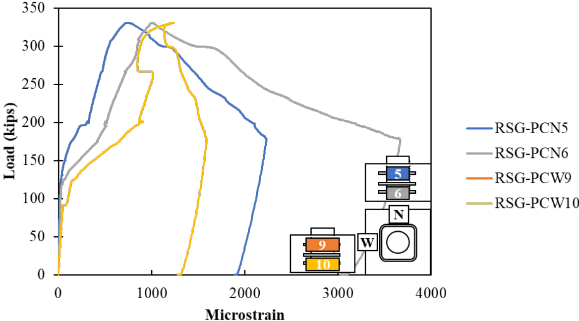
Figure A.205: Confining reinforcement around pocket of Specimen S3-10
