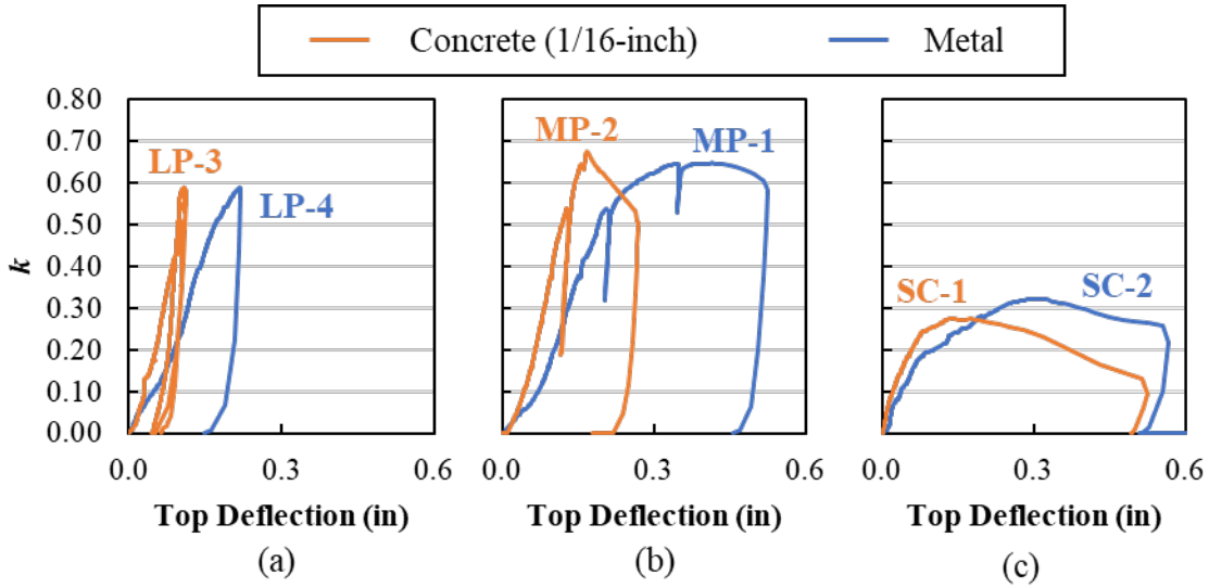
Figure 4.30: Normalized load versus top deflection plots for specimens with corrugation, (a) large-plug specimens, (b) multi-plug specimens, and (c) socket connection specimens
