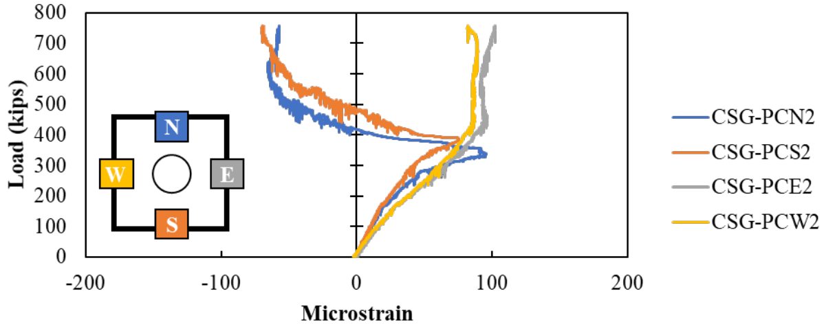
Figure A.7: Concrete surface gauges on the sides of cap closest to bottom of Specimen S1-2
