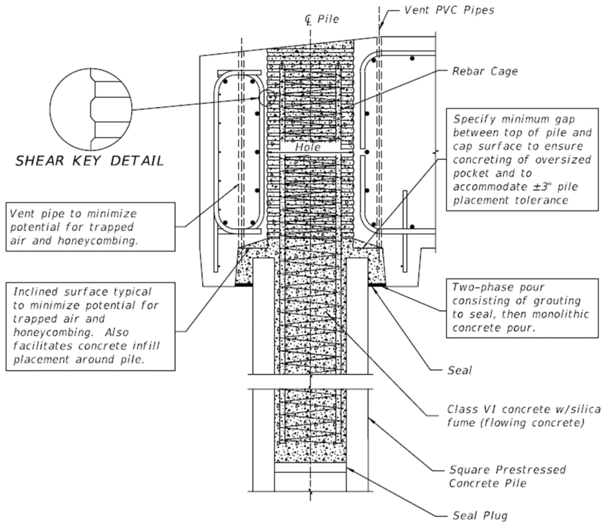
Figure 2.23: Precast footing details [52]
