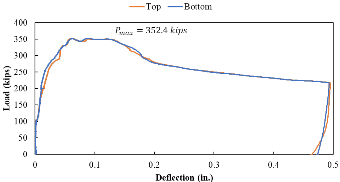
Figure A.208: Load versus deflection curve for Specimen S3-11
