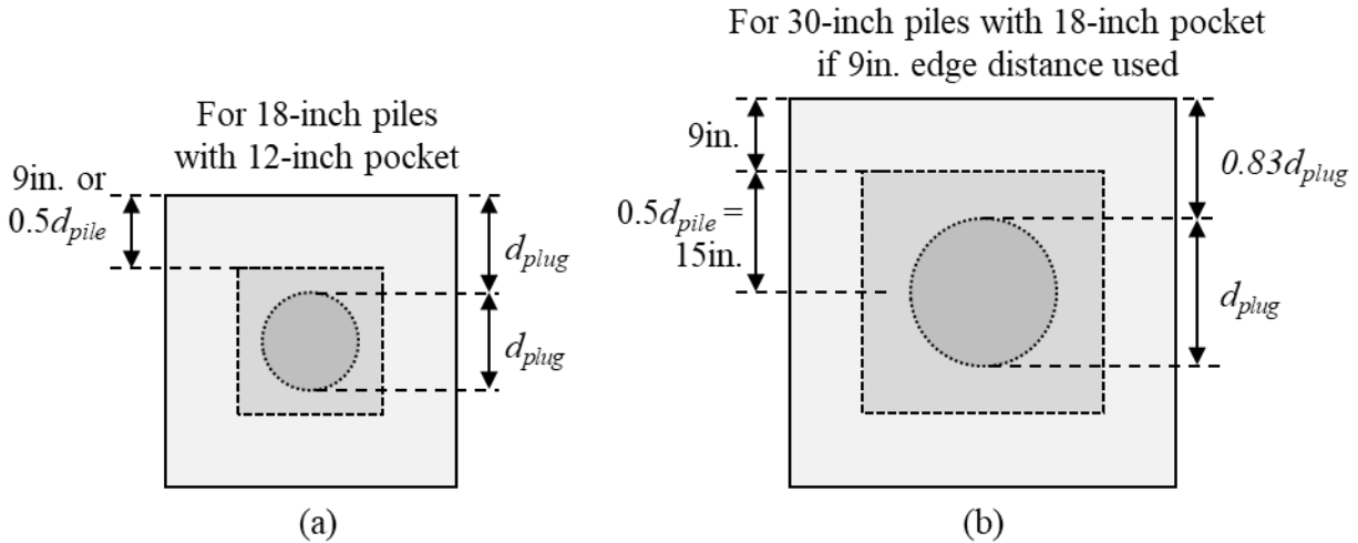
Figure 6.3: Distance between the edge of the pocket or plug and the edge of the cap for (a) 18-inch piles with 12-inch pockets and (b) 30-inch piles with 18-inch pockets when only 9-inch edge distance is provided
