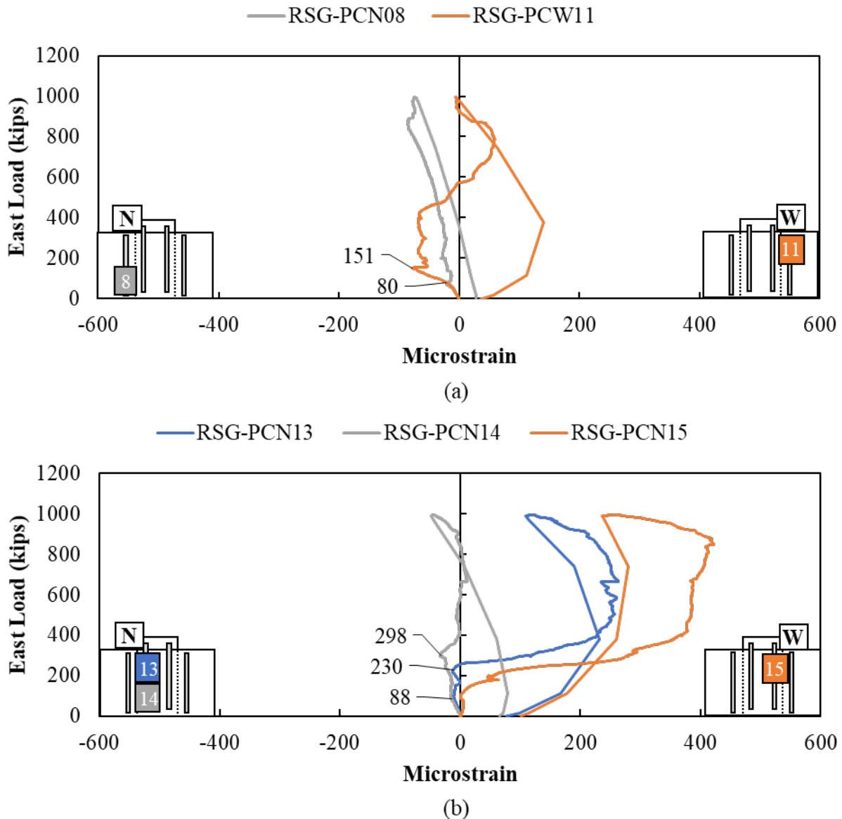
Figure B.27: Rebar strain gauges in vertical reinforcement on (a) the cap and (b) plug of Specimen LP-4
