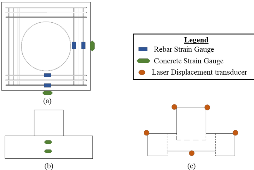
Figure 4.24: Instrumentation scheme for socket connection: (a) pile cap bottom view, (b) cap elevation, and (c) specimen elevation through centerline.
