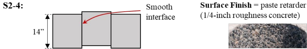
Figure A.41: Details for S2-4
