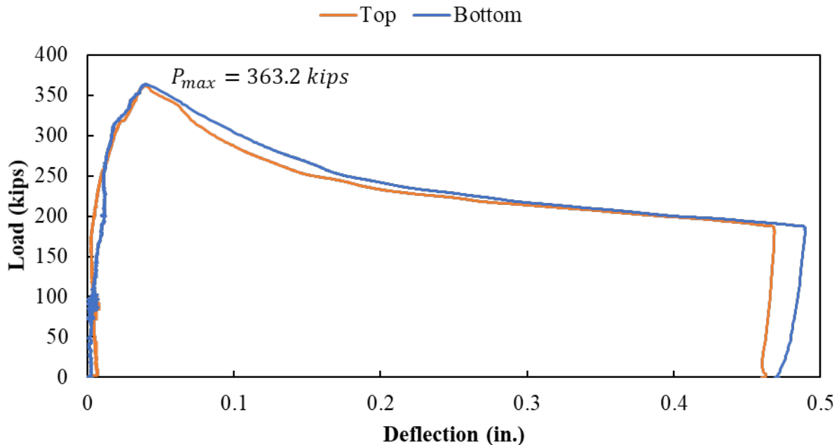
Figure A.215: Load versus deflection curve for Specimen S3-12
