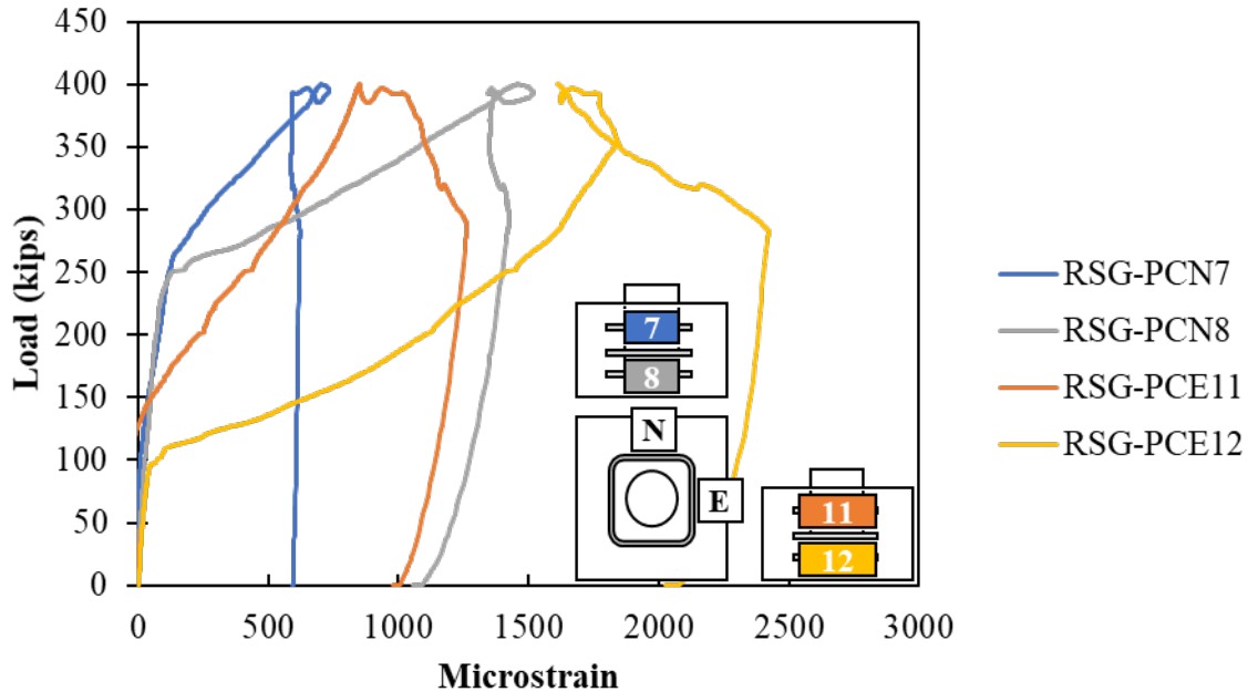
Figure A.96: Confining reinforcement around the pocket of Specimen S2-11
