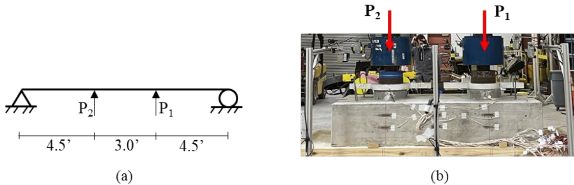
Figure 4.16: (a) Assumed loading and boundary conditions for load frame and (b) side view of specimen during testing for the multi-plug test specimens
