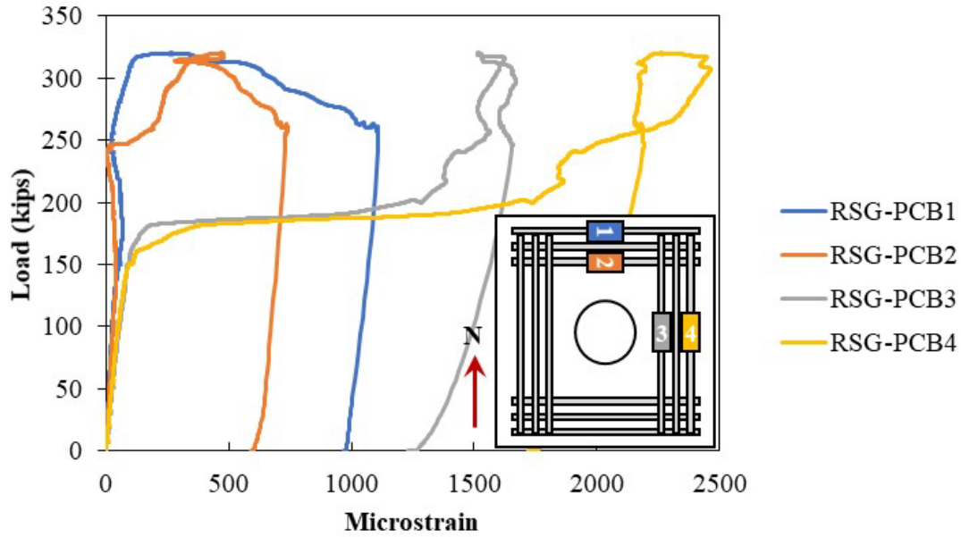
Figure A.36: Rebar strain gauges in the longitudinal reinforcement on the bottom of Specimen S2-3
