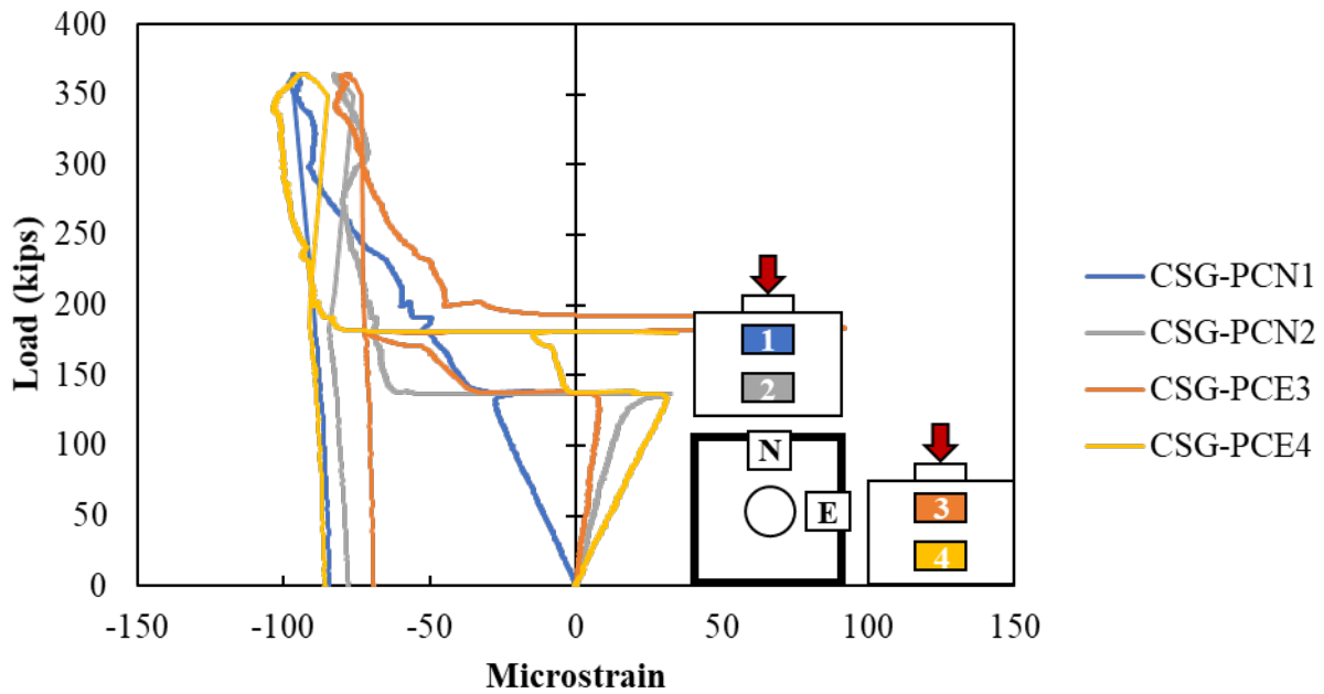
Figure A.143: Concrete strain gauges in the surface of the cap of Specimen S3-1
