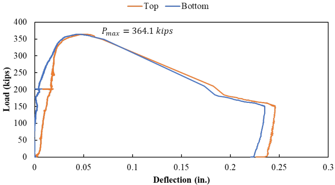
Figure A.141: Load-deflection curve for Specimen S3-1
