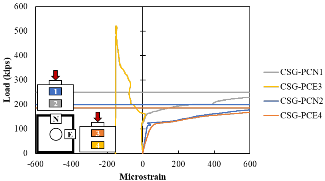
Figure A.101: Concrete strain gauges in the surface of Specimen S2-9
