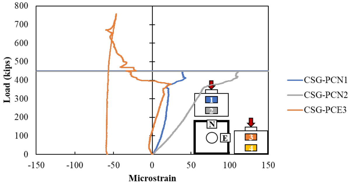
Figure A.121: Concrete strain gauges on the surface of Specimen S2-16
