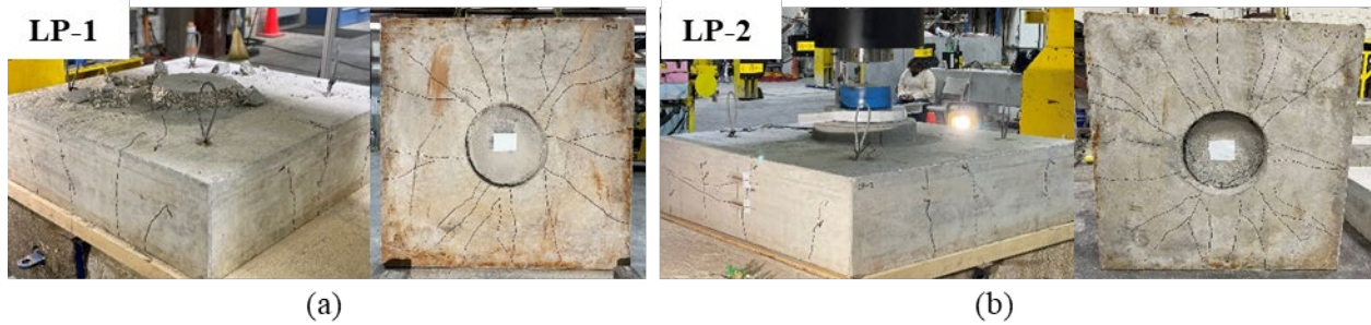
Figure 4.26: Crack patterns at failure for (a) LP-1 (1/16-inch roughness) and (b) LP-2 (1/4-inch roughness) without corrugations
