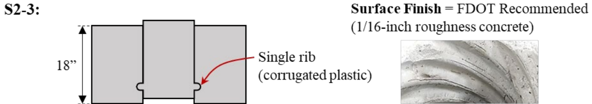
Figure A.34: Details for S2-3
