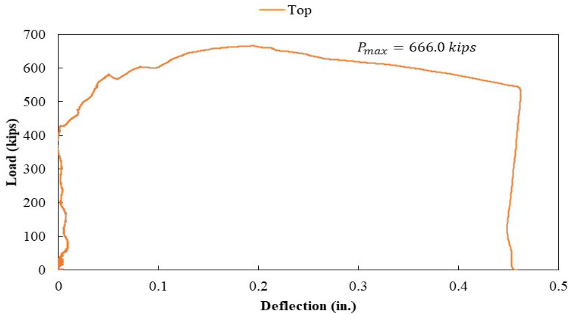
Figure A.136: Load versus displacement curve for Specimen S2-20
