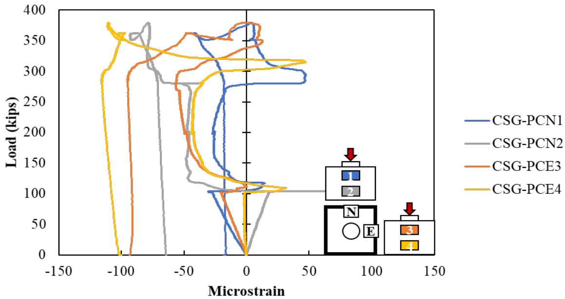
Figure A.189: Concrete strain gauges in the surface of Specimen S3-8
