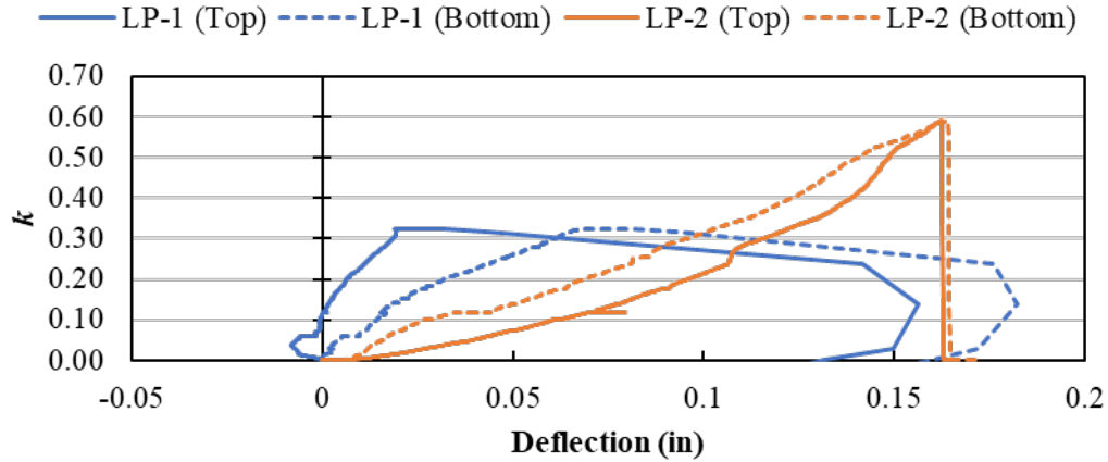
Figure 4.25: Normalized load ( k ) versus top and bottom deflection for (a) LP-1 (1/16-inch roughness) and (b) LP-2 (1/4-inch roughness) without corrugations
