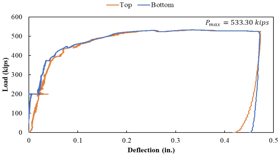
Figure A.124: Load versus displacement curve for specimen S2-17
