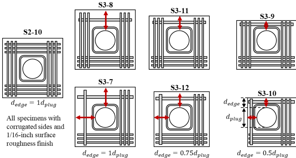
Figure 3.34: Specimens details for edge distance comparisons
