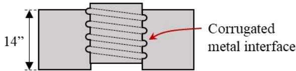
Figure A.139: Details for Series III specimens
