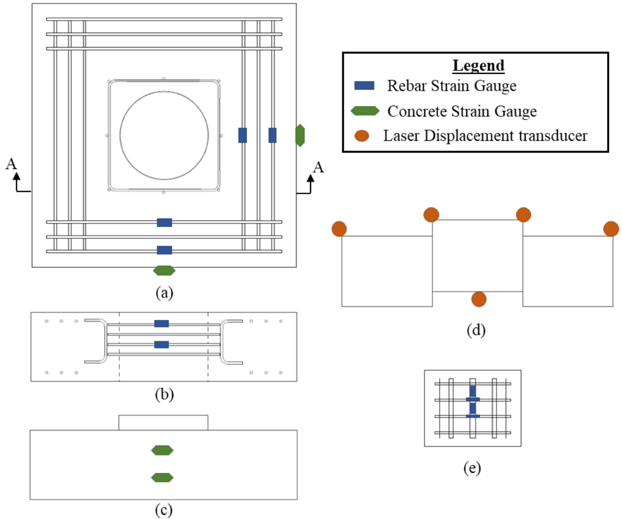
Figure 4.10: Instrumentation scheme for larger plug specimens: (a) pile cap bottom view, (b) section A-A, (c) cap elevation, (d) specimen elevation through centerline, and (e) plug reinforcement detail.
