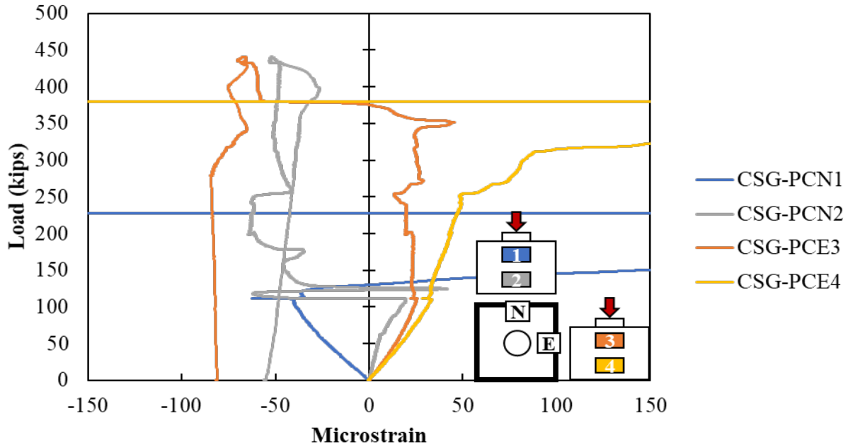
Figure A.155: Concrete strain gauges in the surface of Specimen S3-3
