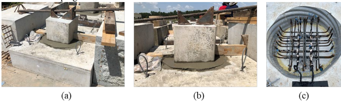
Figure 4.19: Construction of socket connection: (a) and (b) details of 18-inch pile and (c) reinforcement in the plug.
