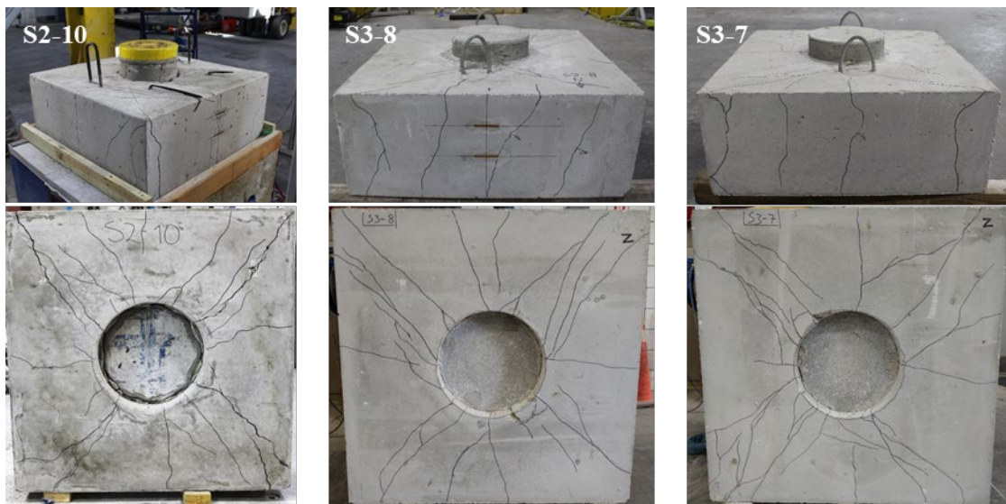
Figure 3.37: Cracking at failure for (a) S2-10, (b) S3-8, and (c) S3-7
