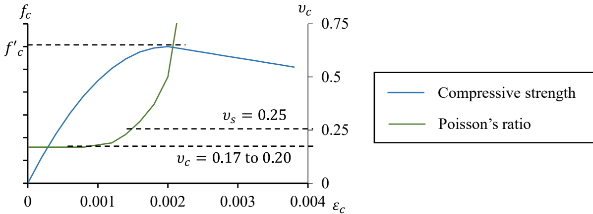
Figure 5.4: Relationship between concrete stress, concrete strain, and Poisson's ratio, based on Harries and Kharel [56]
