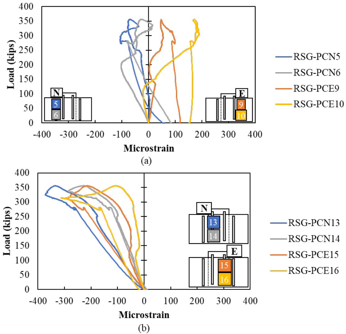
Figure A.54: Rebar strain gauges in vertical reinforcement on (a) cap and (b) plug of Specimen S2-5
