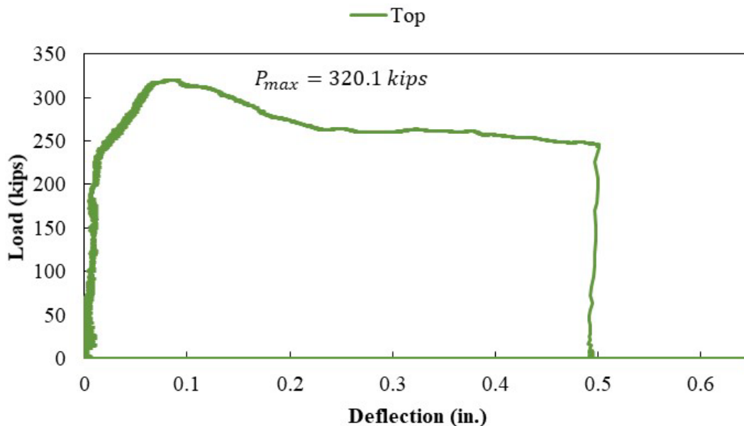
Figure A.35: Load versus deflection curve for Specimen S2-3
