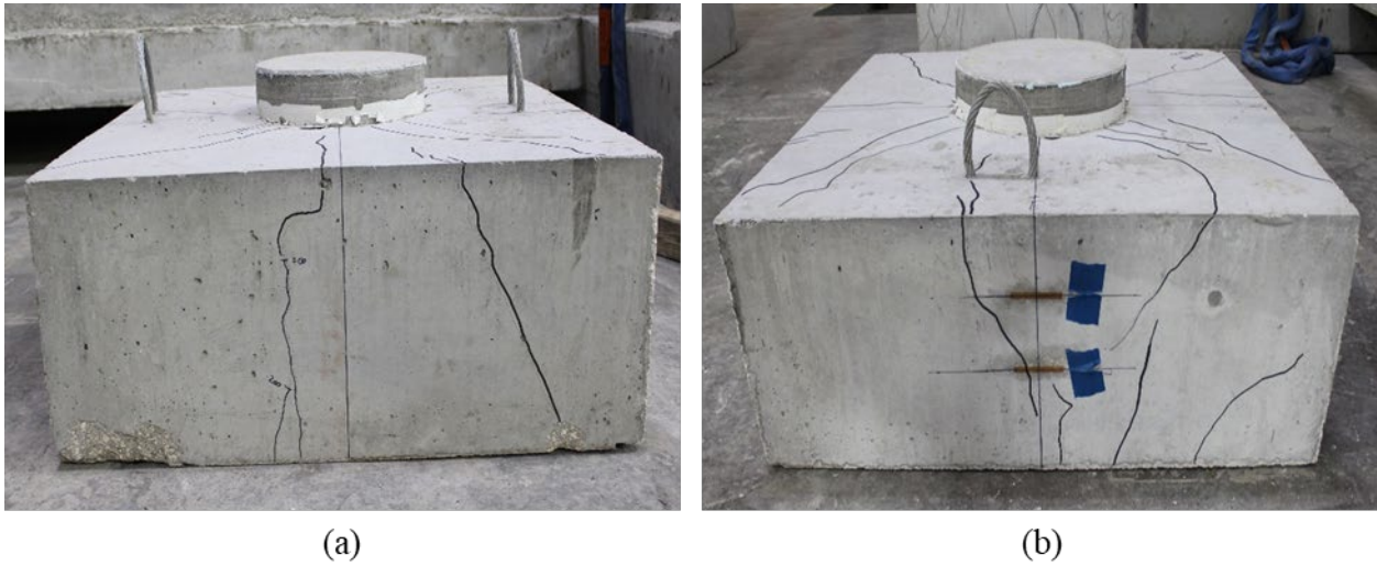
Figure A.114: Cracking on the (a) south side and (b) east side on specimen S2-14
