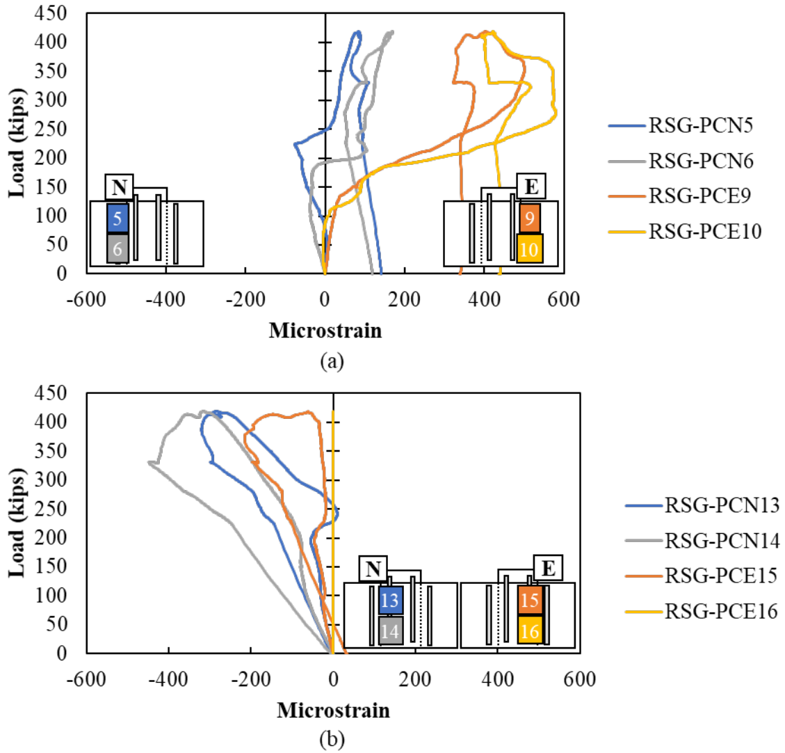
Figure A.61: Rebar strain gauges in vertical reinforcement on (a) cap and (b) plug of Specimen S2-6
