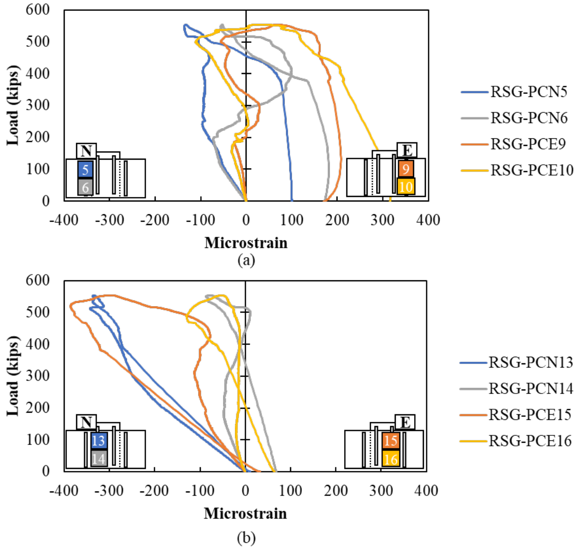
Figure A.75: Rebar strain gauges in vertical reinforcement on (a) the cap and (b) plug of Specimen S2-8
