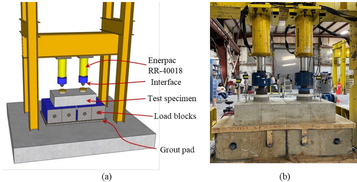
Figure 4.13: (a) Schematic and (b) photograph of test setup for multi-plug specimens.
