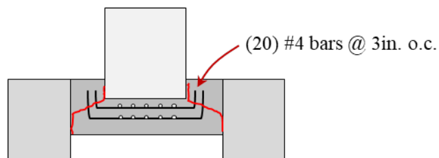
Figure 6.6: Reinforcement layout in the pocket of the specimen
