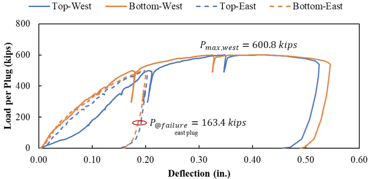
Figure B.30: Load versus deflection curve for Specimen MP-1
