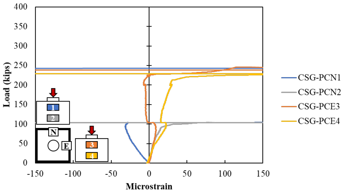
Figure A.169: Concrete strain gauges in the surface of Specimen S3-5
