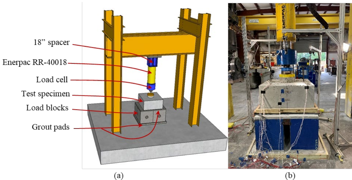
Figure 3.9: (a) Schematic and (b) photograph of test setup
