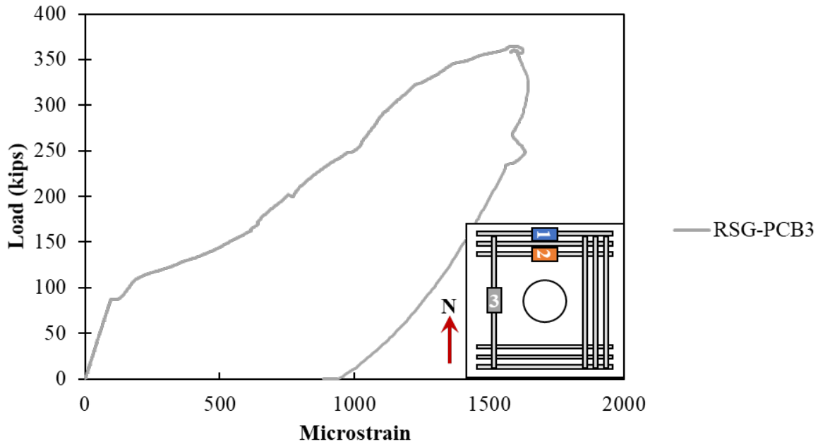
Figure A.195: Rebar strain gauges in the longitudinal reinforcement on the bottom of Specimen S3-9
