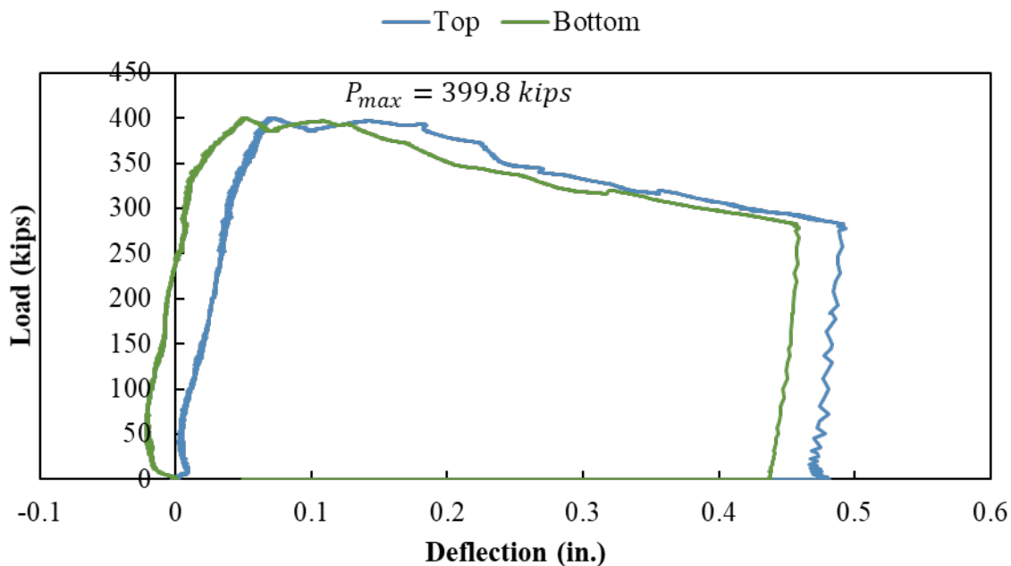
Figure A.92: Load versus deflection curve for Specimen S2-11
