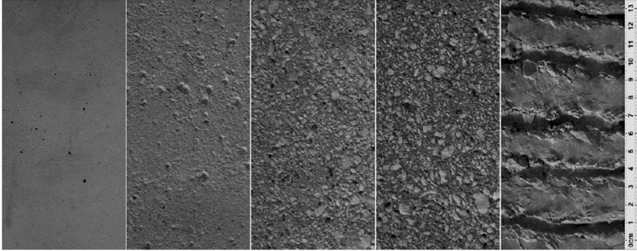
Figure 2.4: Surface preparations for specimens from Santos and Julio [22]
