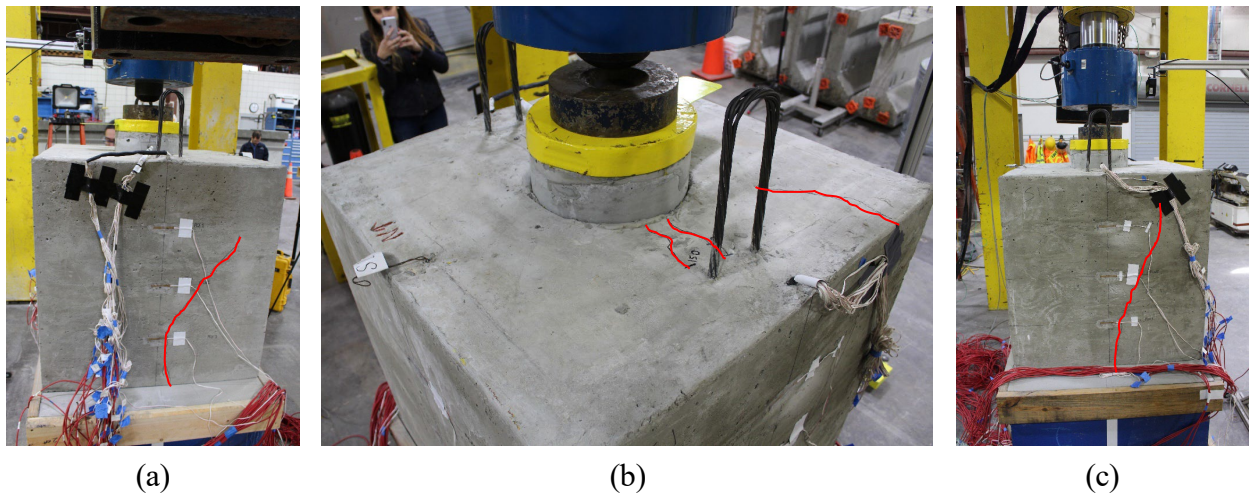
Figure A.17: Cracking on the (a) east, (b) top, and (c) west faces of Specimen S1-4 after failure
