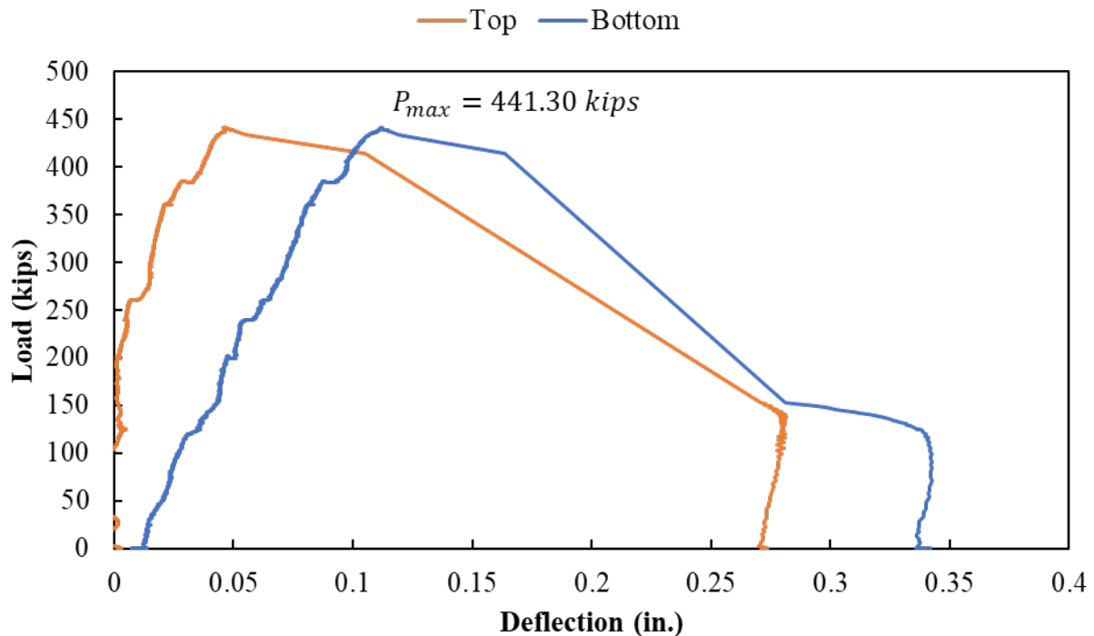
Figure A.112: Load versus displacement curve for Specimen S2-14
