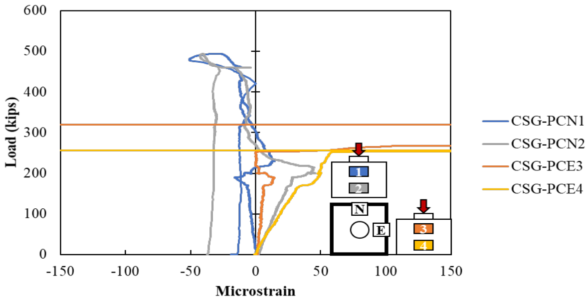
Figure A.162: Concrete strain gauges in the surface of the cap of Specimen S3-4
