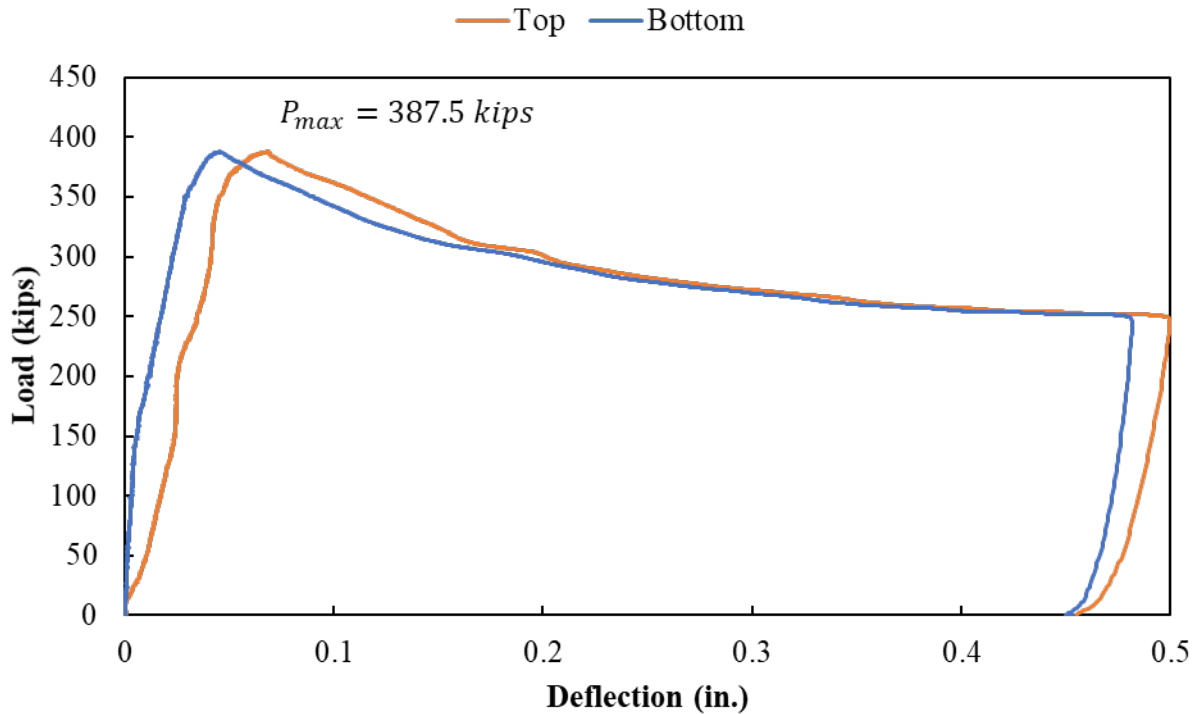
Figure A.221: Load versus deflection curve for Specimen S3-13
