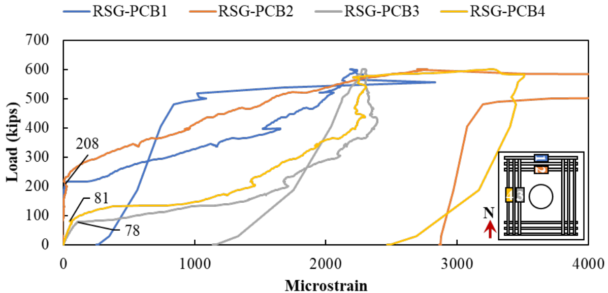
Figure B.53: Rebar strain gauges in the longitudinal reinforcement on bottom of Specimen SC-2
