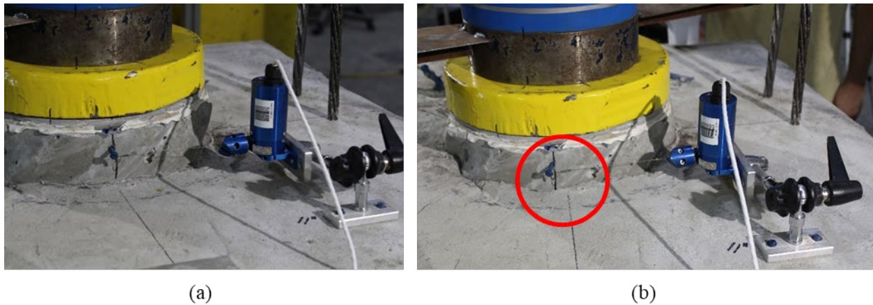
Figure A.105: Details of plug rotation (a) before testing (b) after testing of specimen S2-12
