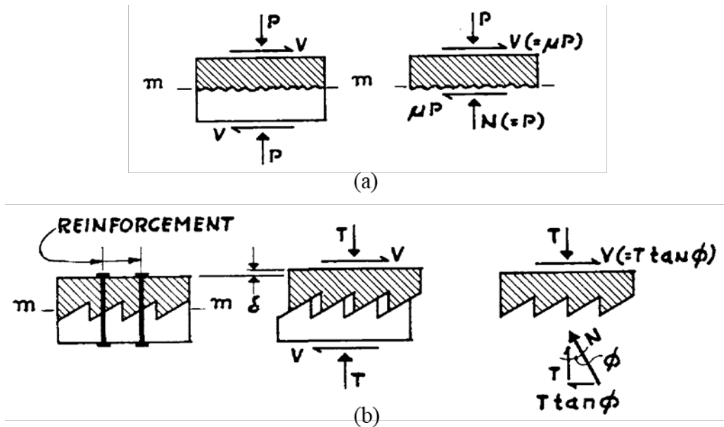
Figure 2.3: Shear friction models for (a) smoother and (b) rougher surfaces [12]
