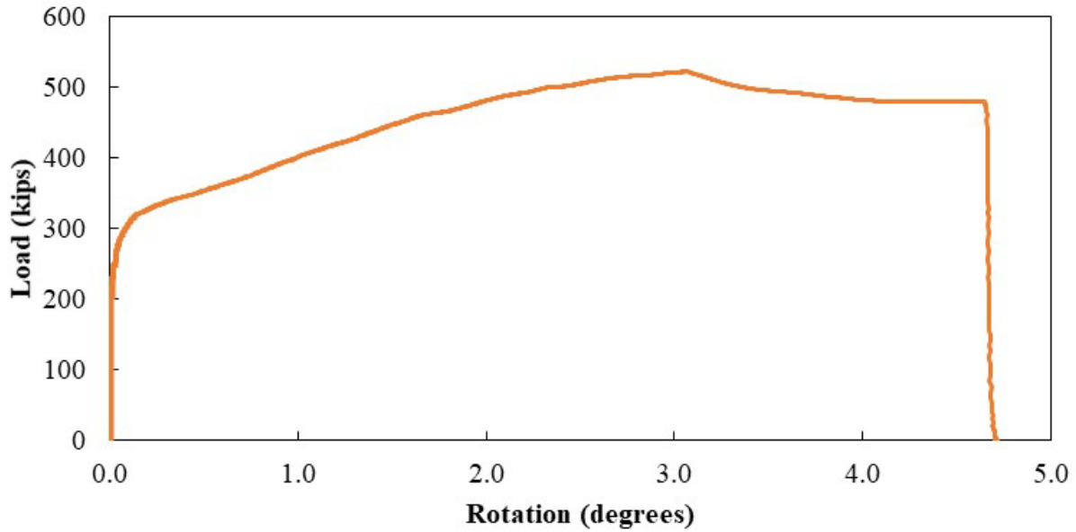
Figure A.104: Load versus rotation (degrees) of the plug of Specimen S2-12
