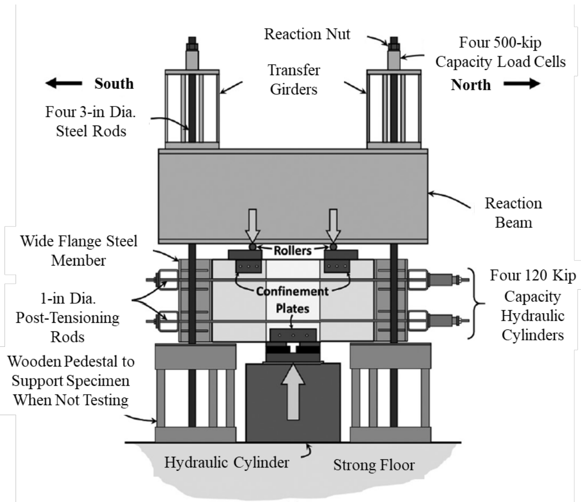
Figure 2.16: Test setup – elevation view [35]
