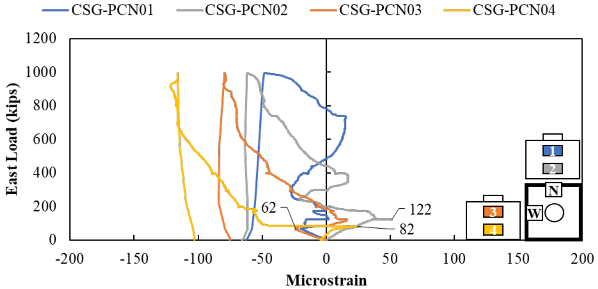
Figure B.11: Concrete surface gauges on the cap of Specimen LP-2
