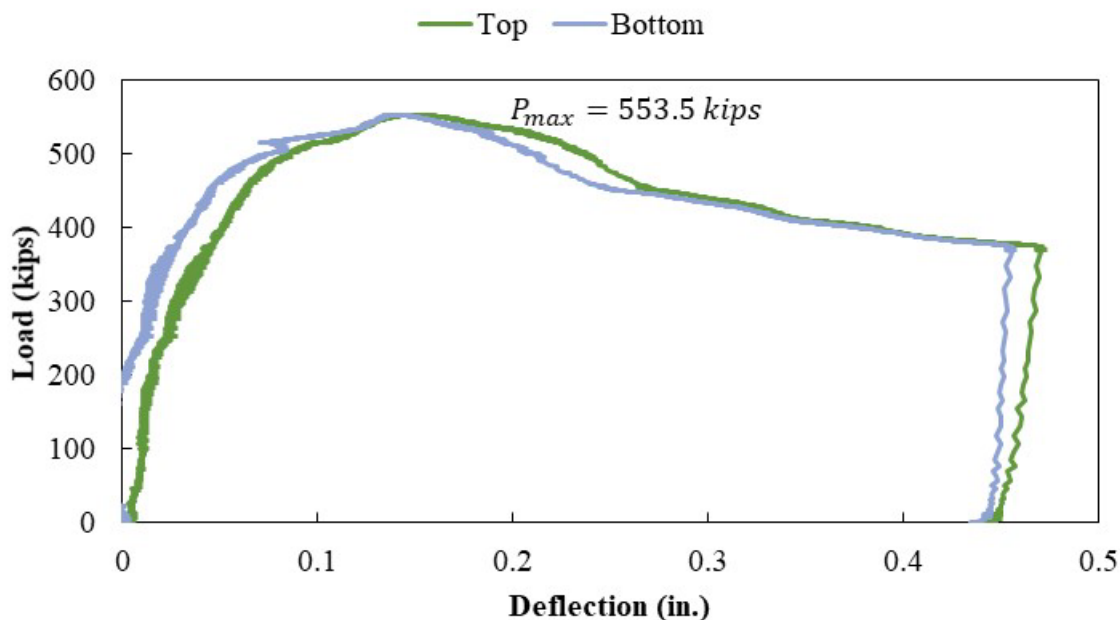
Figure A.70: Load versus deflection curve for Specimen S2-8
