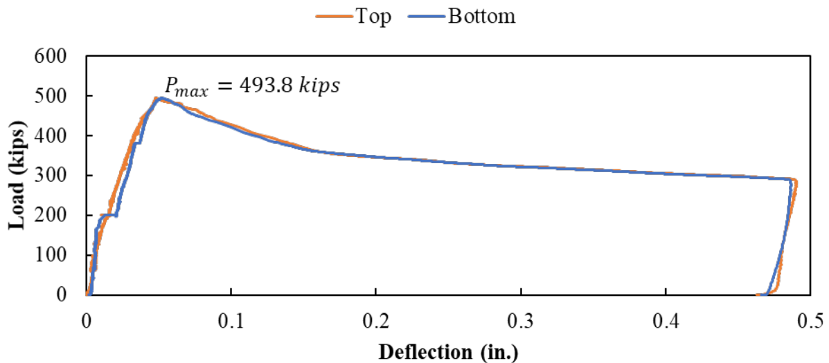
Figure A.160: Load versus deflection curve for Specimen S3-4
