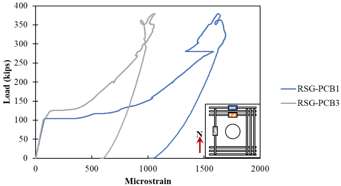
Figure A.188: Rebar strain gauges in the longitudinal reinforcement on the bottom of Specimen S3-8 Cracking was also observed in the surface concrete at a load of around 100 kips in both faces, as shown in Figure A.189.
