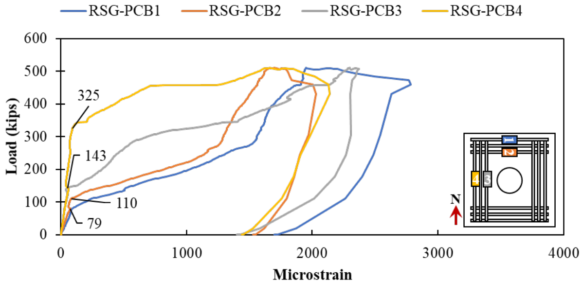
Figure B.44: Rebar strain gauges in the longitudinal reinforcement on bottom of Specimen SC-1
