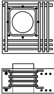
Figure A.200: Details for S3-10
