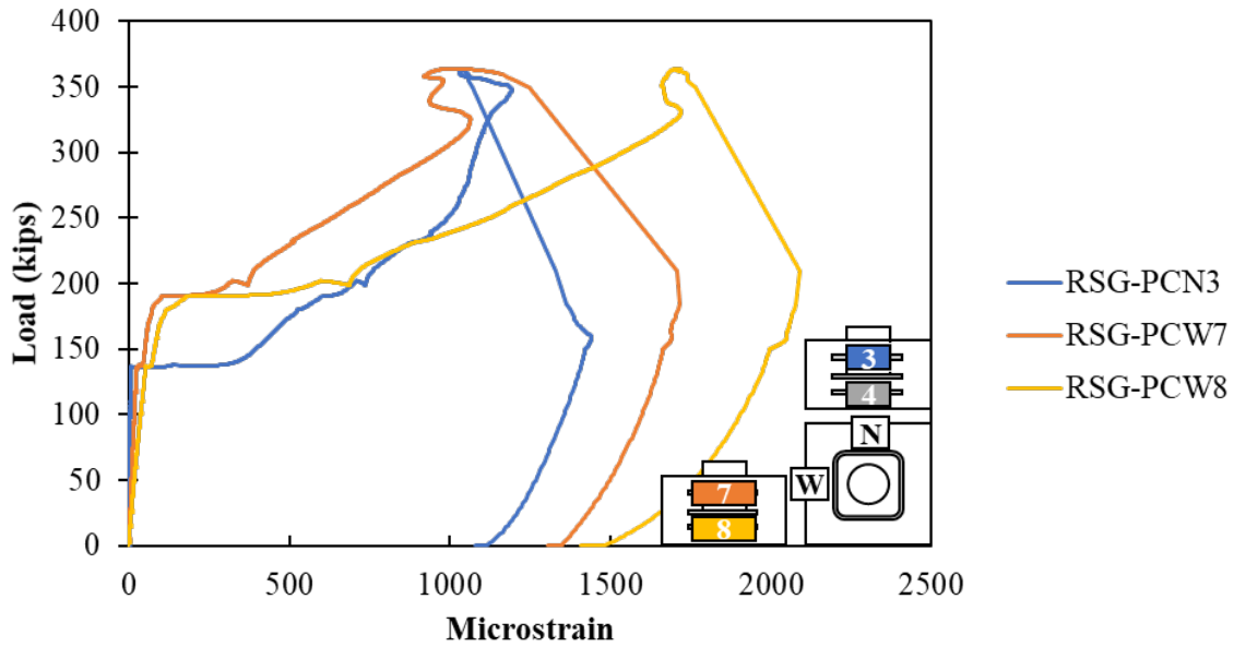
Figure A.142: Confinement reinforcement around pocket for Specimen S3-1
