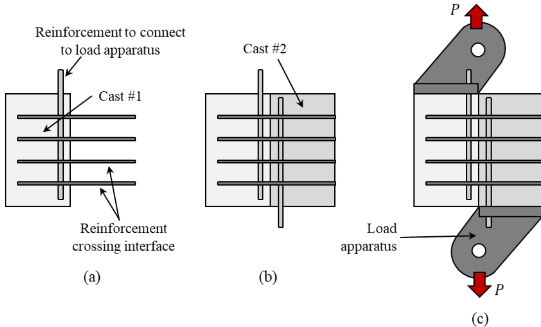
Figure 2.12: Typical casting and testing procedure for pull-off tests: (a) casting of first component, (b) casting of section component, and (c) attaching load apparatus and testing of pull-off specimen.
