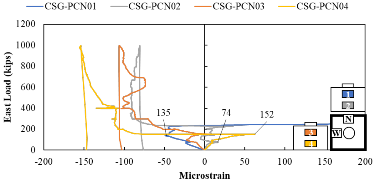
Figure B.25: Concrete strain gauges on the concrete surface of Specimen LP-4
