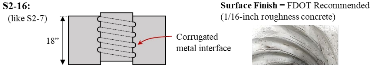
Figure A.119: Details for S2-16
