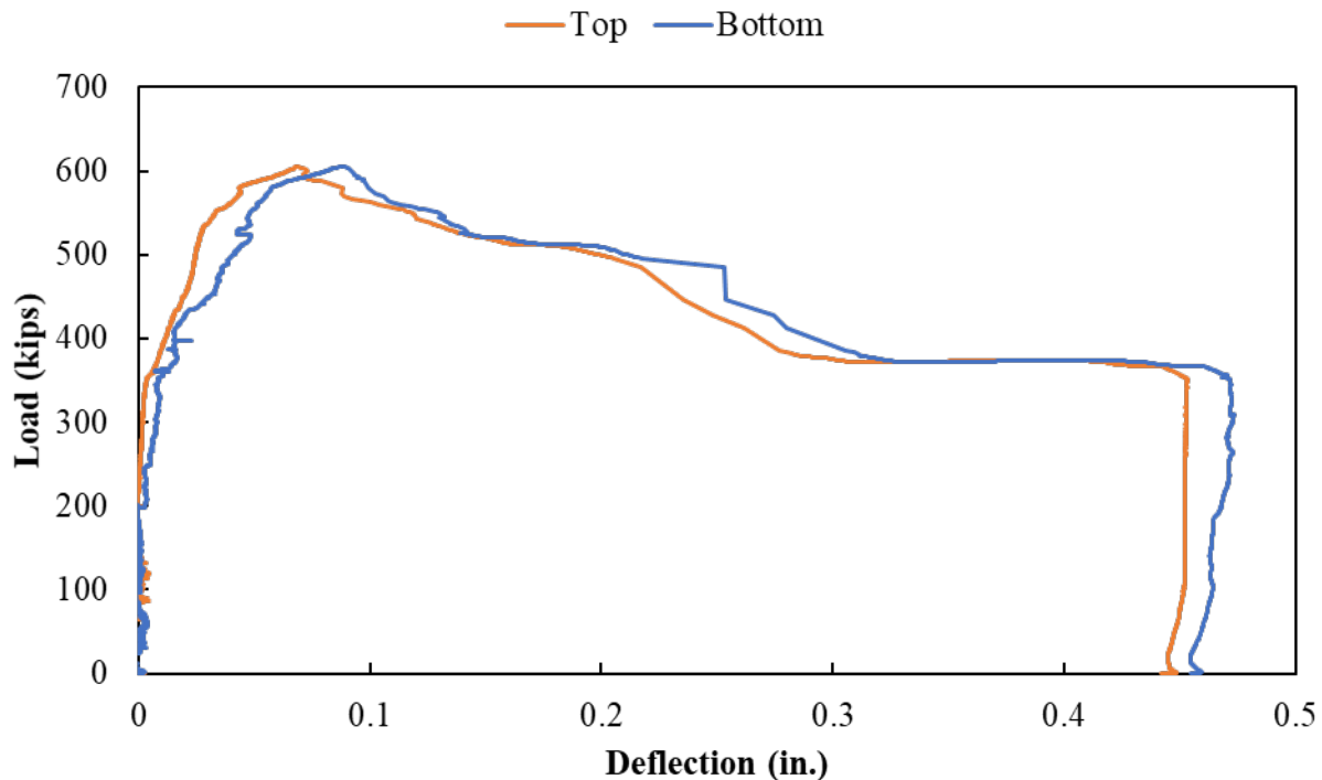
Figure A.108: Load-displacement curve for Specimen S2-13
