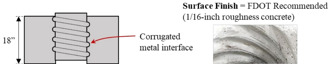
Figure A.62: Details for S2-7
