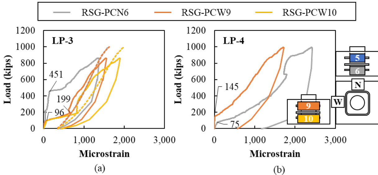
Figure 4.32: Load versus strain in confinement reinforcement around plug for (a) LP-3 and (b) LP-4
