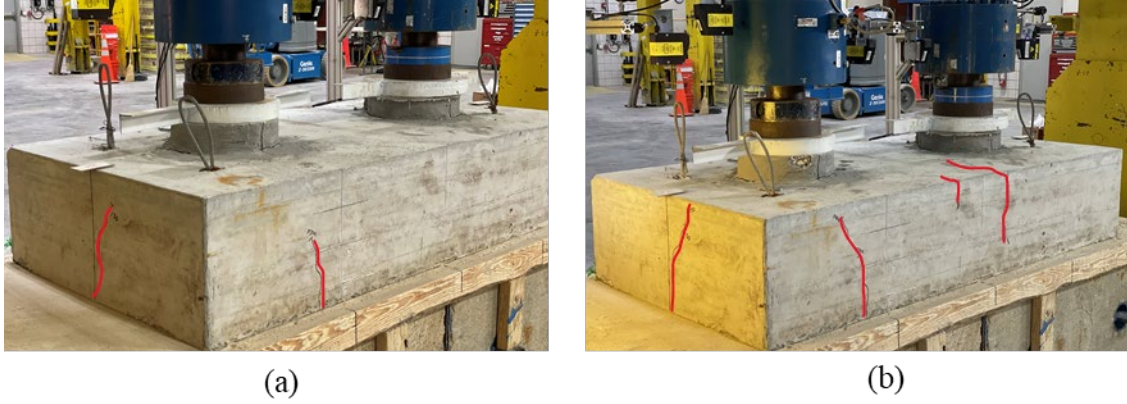
Figure B.32: Crack propagation during testing at (a) 150 kips and (b) 250 kips on MP-1
