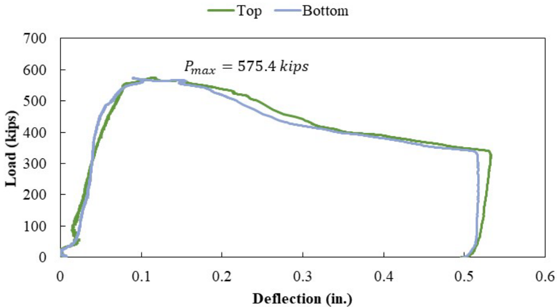
Figure A.85: Load versus deflection curve for Specimen S2-10
