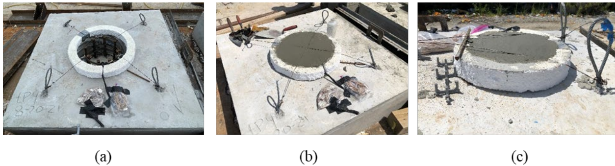
Figure 4.3: Plug construction: (a) 3-inch cylindrical form on top of cap before casting, (b) after casting the plug and (c) close up of the 3-inch cylindrical form.
