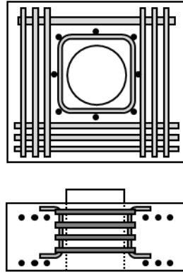
Figure A.207: Details for S3-11
