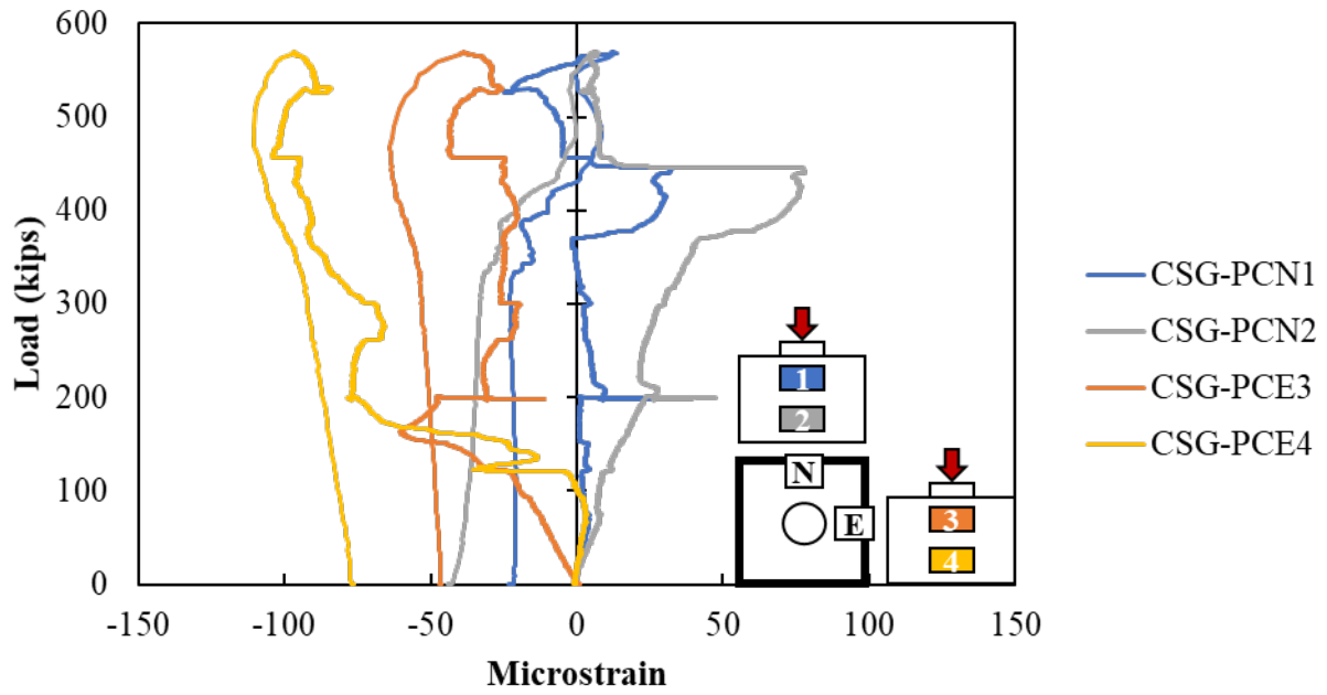
Figure A.129: Concrete strain gauges on the concrete surface of Specimen S2-18
