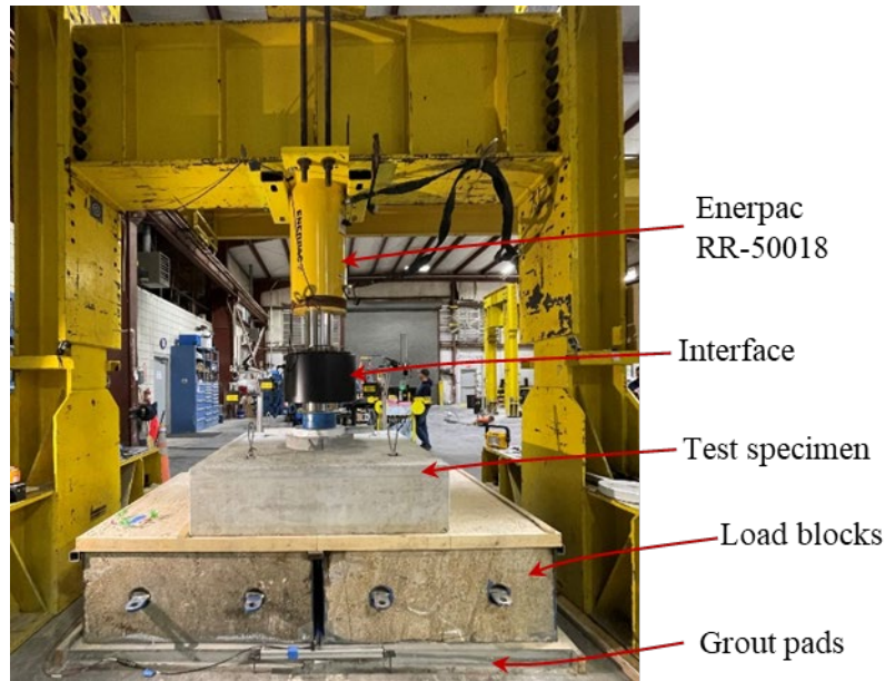
Figure 4.7: Photograph of test setup for larger plug specimens.
