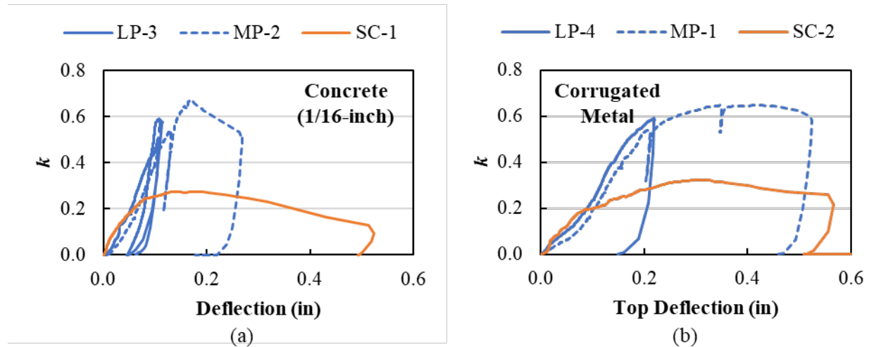
Figure 4.38: Normalized load ( k ) versus top and bottom deflection for LP, MP, and SC specimens with corrugated interface with (a) 1/16-inch concrete and (b) corrugated metal finish
