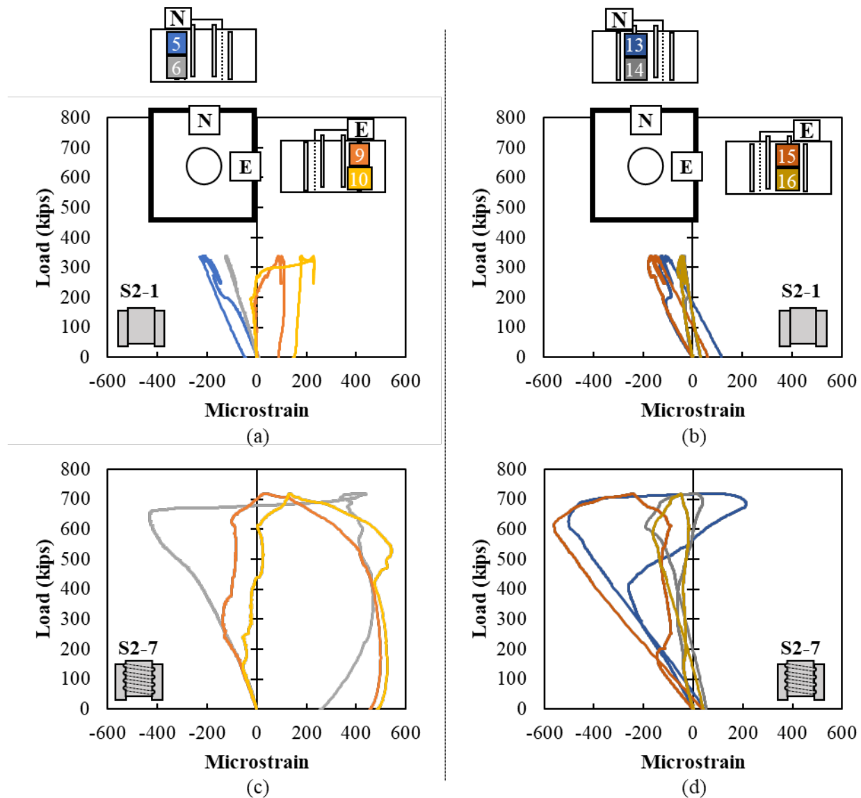
Figure 3.33: Load versus strain in (a) vertical reinforcement in pile cap for S2-1, (b) vertical reinforcement in plug for S2-1, (c) vertical reinforcement in plug for S2-7, and (d) vertical reinforcement in plug for S2-7
