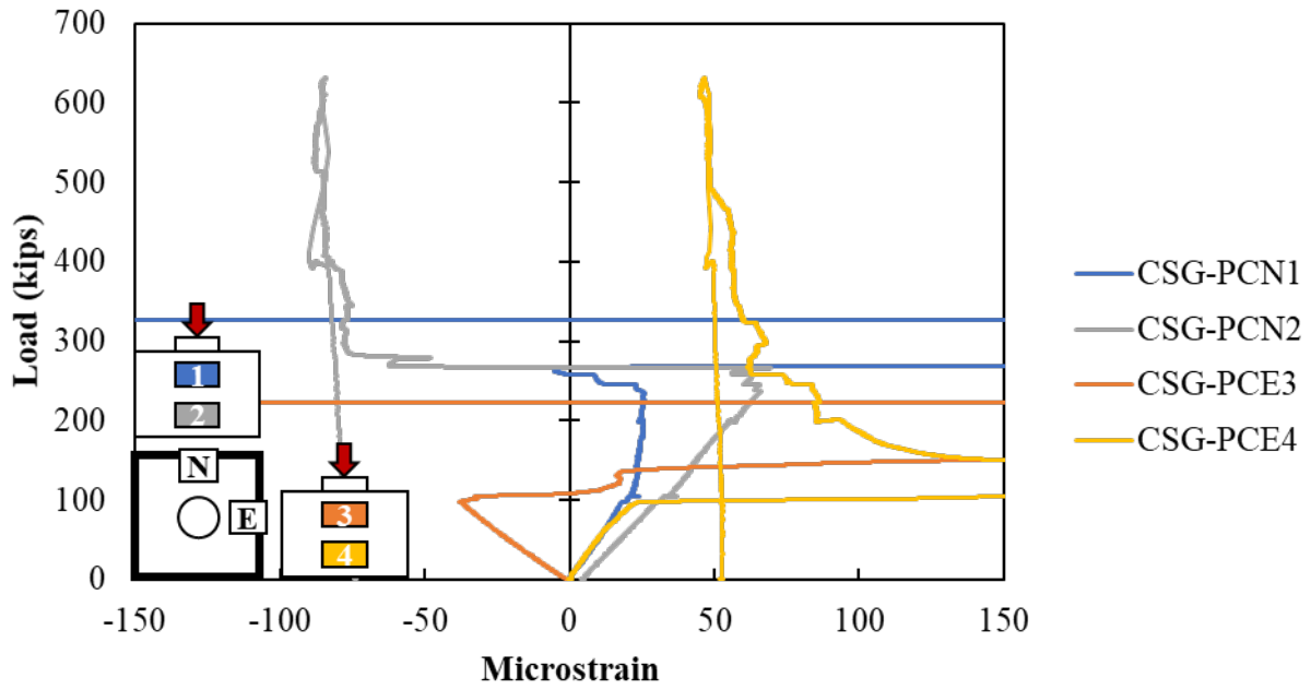
Figure A.117: Concrete surface gauges on the cap on specimen S2-15
