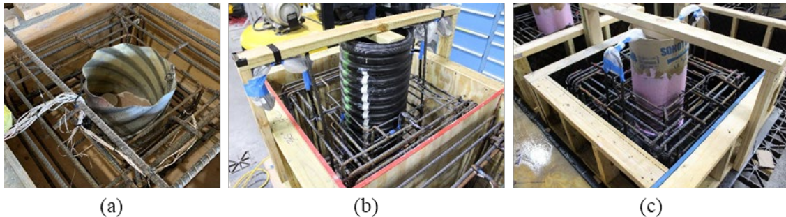
Figure 3.2: Construction of cap and installation of blockout for void with (a) corrugated metal pipe, (b) corrugated plastic pipe, and (c) Sonotube
