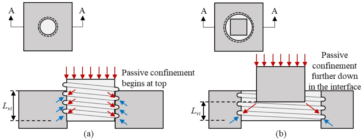
Figure 4.39: Cross section A-A of (a) LP and (b) SC specimens with sketch of confining stresses in pocket and socket from applied loads
