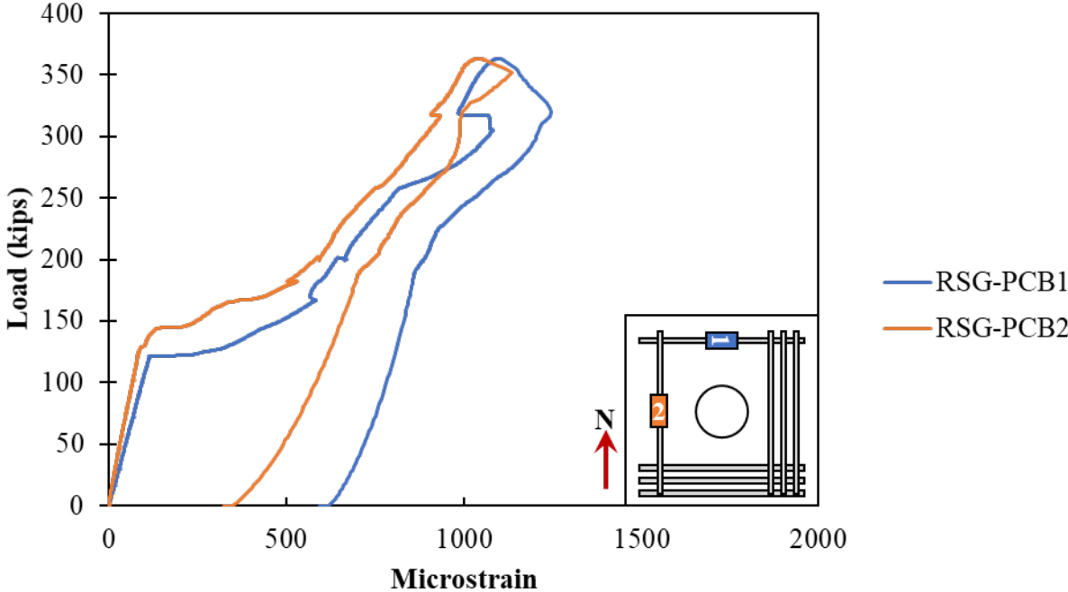
Figure A.216: Rebar strain gauges in the longitudinal reinforcement on the bottom of Specimen S3-12 Cracking was also observed in the surface concrete at a load of around 120 kips in the north side of the specimen, as shown in Figure A.217.
