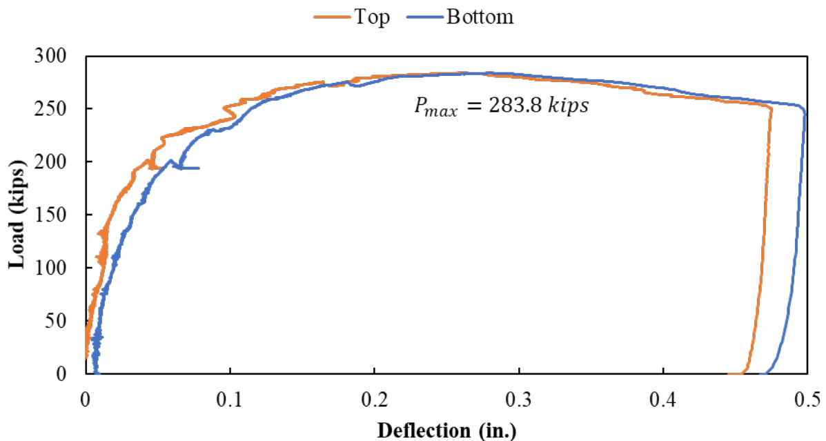
Figure A.173: Load versus deflection curve for Specimen S3-6
