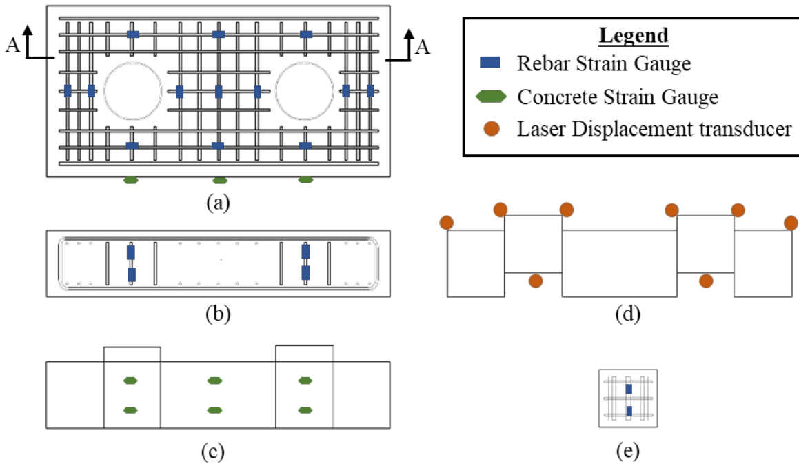
Figure 4.17: Instrumentation scheme for multi plug specimens: (a) pile cap bottom view, (b) section A-A, (c) cap elevation, (d) specimen elevation through centerline, and (e) plug reinforcement detail.
