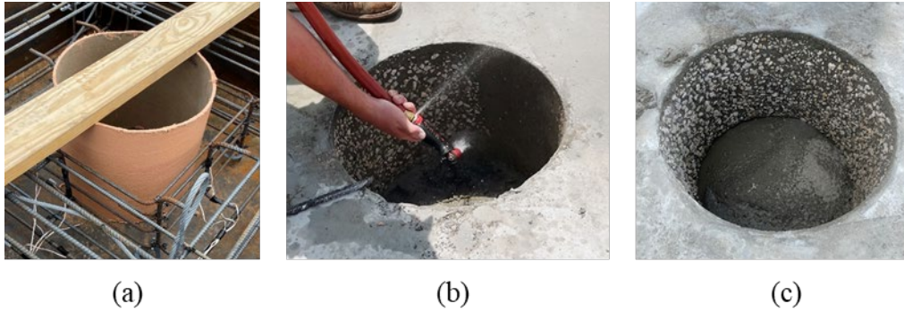
Figure 4.6: Exposed aggregate finish: (a) pipe with the set retarding agent, (b) pressure washing the surface, and (c) surface finish.
