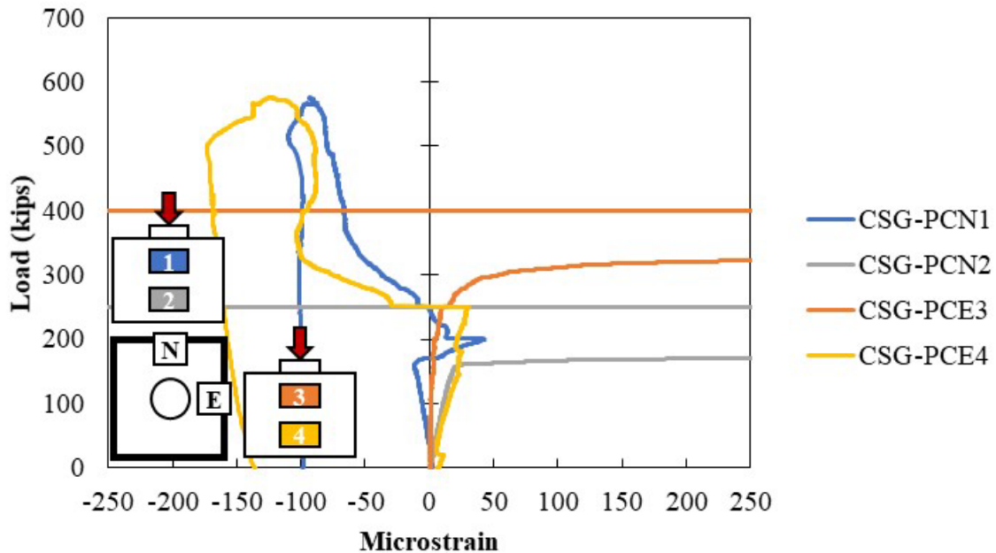
Figure A.87: Concrete strain gauges in the surface of Specimen S2-10
