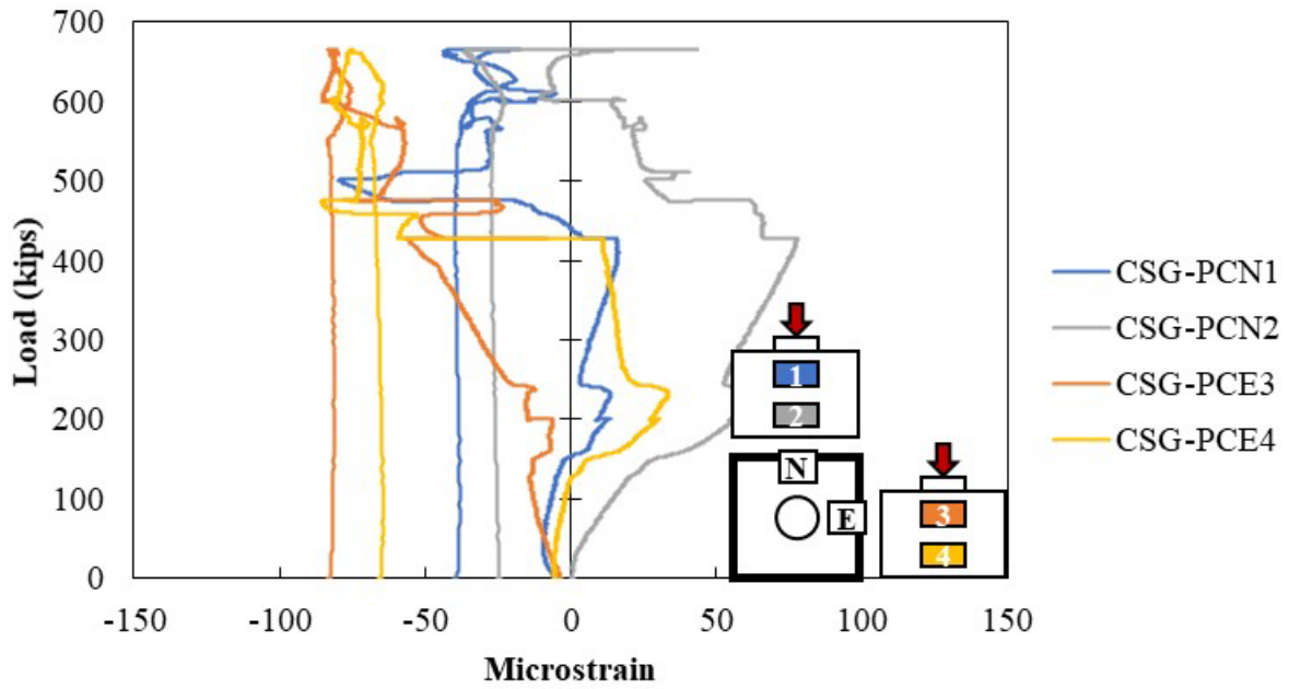
Figure A.137: Concrete strain gauges on the concrete surface of Specimen S2-20
