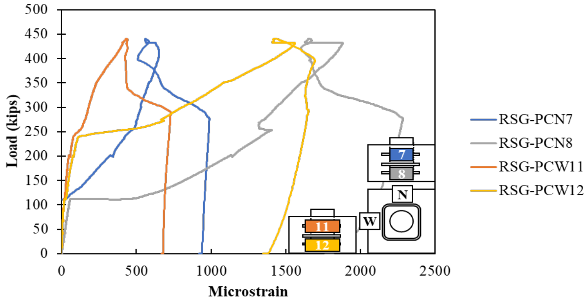
Figure A.157: Confining reinforcement around pocket of Specimen S3-3
