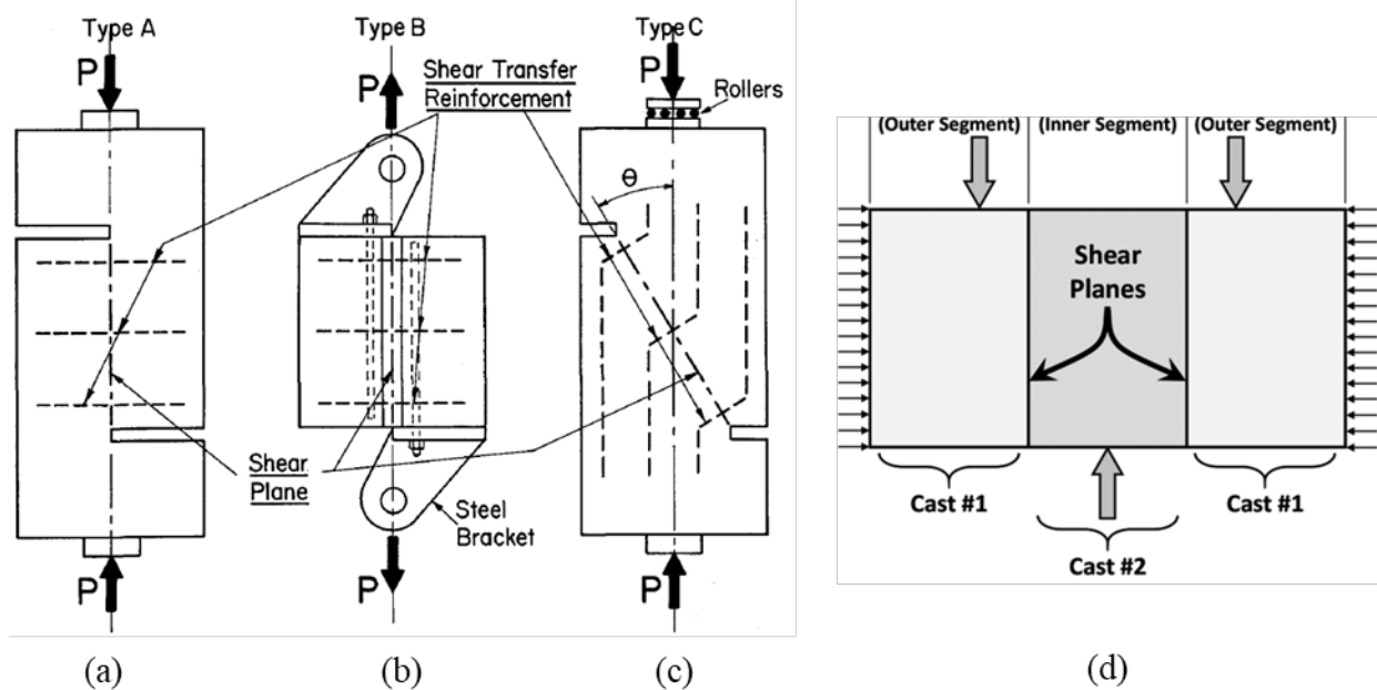
Figure 2.6: Typical test specimens used for (a) push-off tests, (b) pull-off tests, and (c) modified push-off tests [7] and (d) push-through tests [35]
