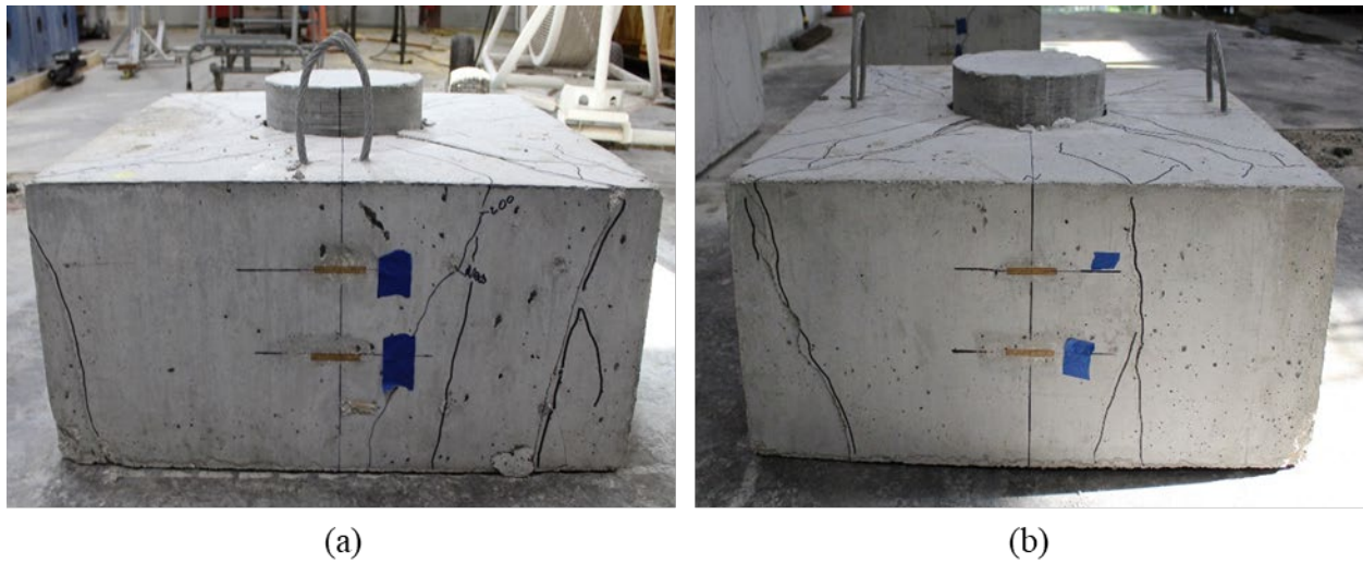
Figure A.134: Cracking on the (a) east side and (b) north side of specimen S2-19
