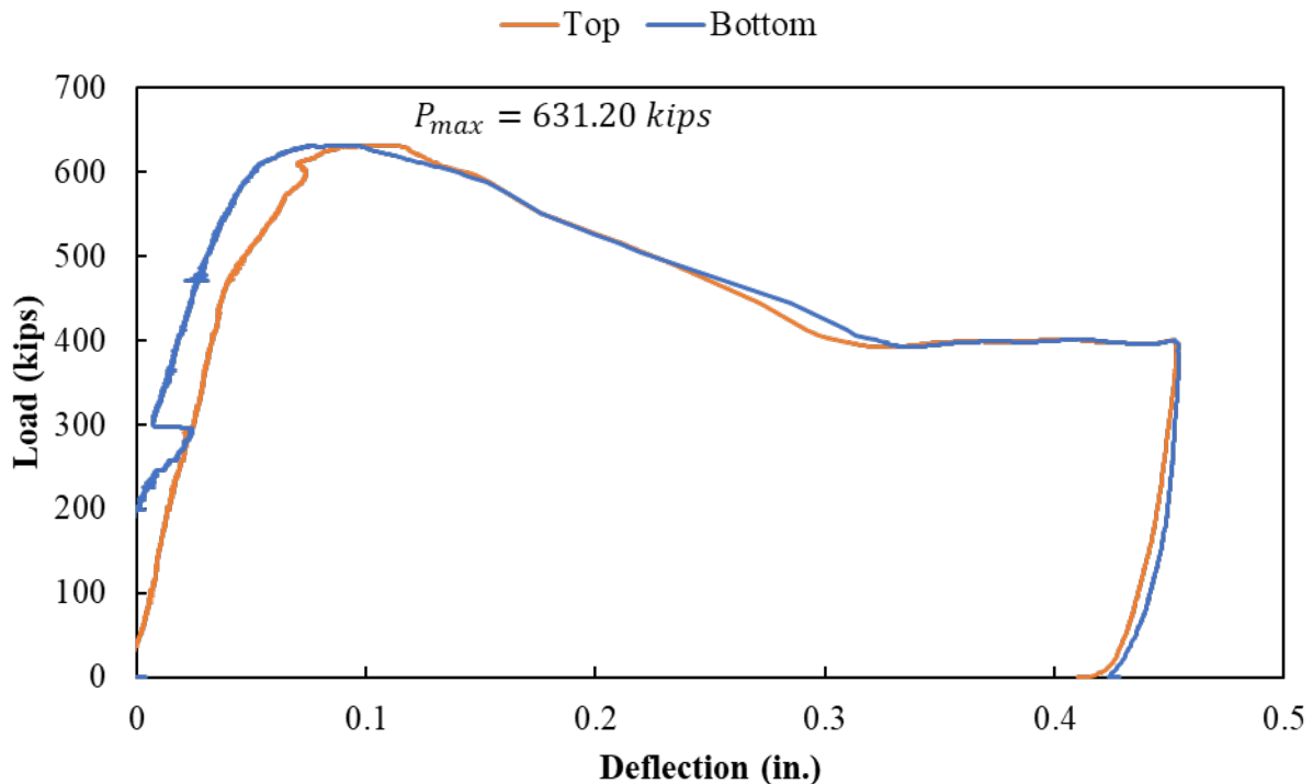
Figure A.116: Load versus displacement curve for specimen S2-15
