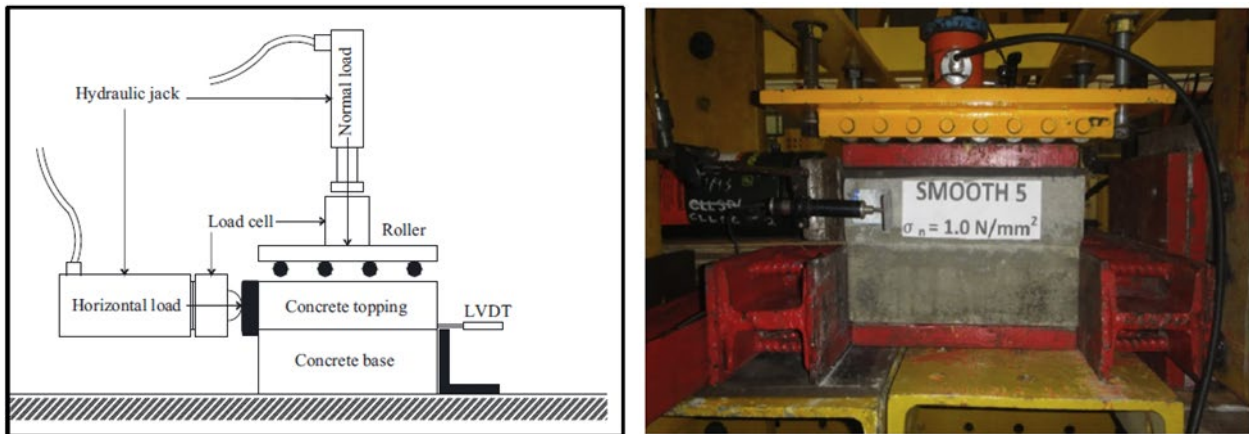
Figure 2.9: Push-off test setup [8]
