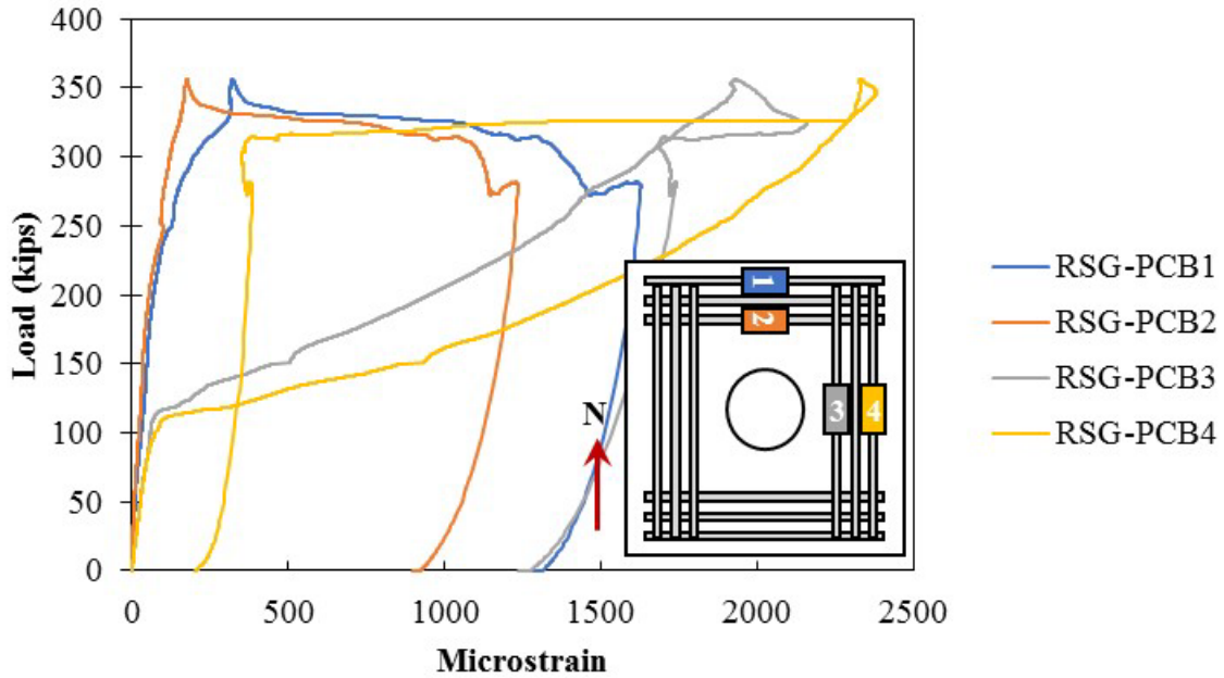
Figure A.50: Rebar strain gauges in the longitudinal reinforcement on bottom of Specimen S2-5
