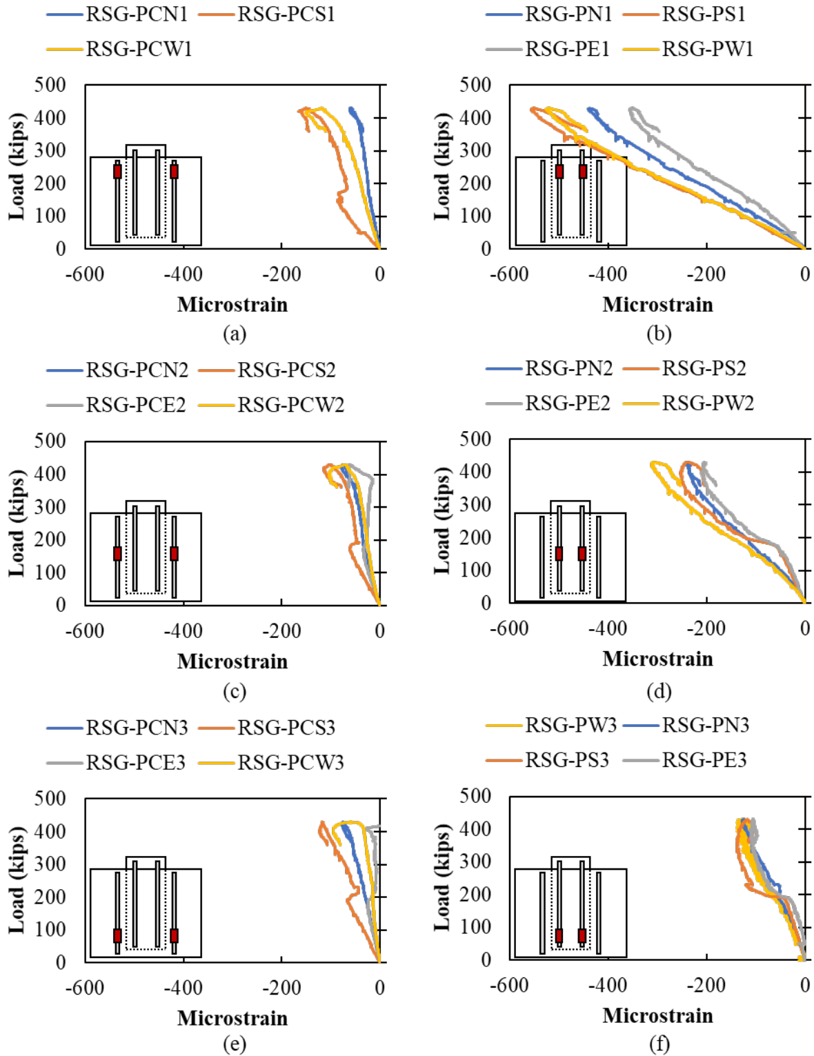
Figure A.19: Rebar strain gauges in vertical reinforcement in plug and cap of Specimen S1-4
