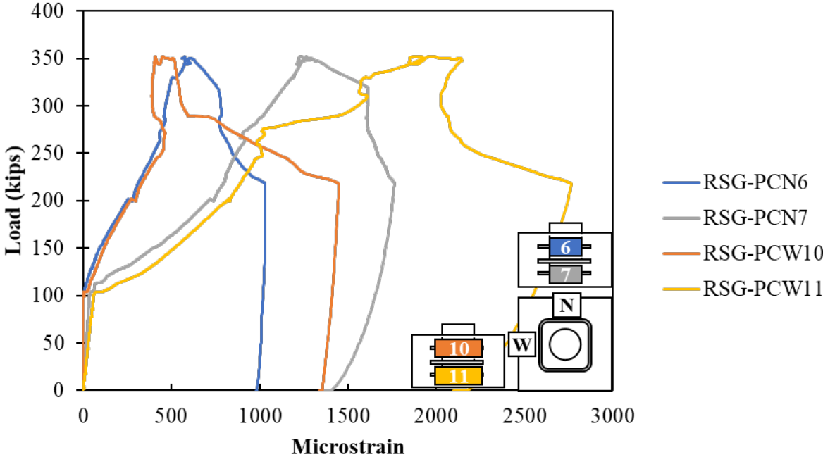
Figure A.212: Confining reinforcement around pocket of Specimen S3-11
