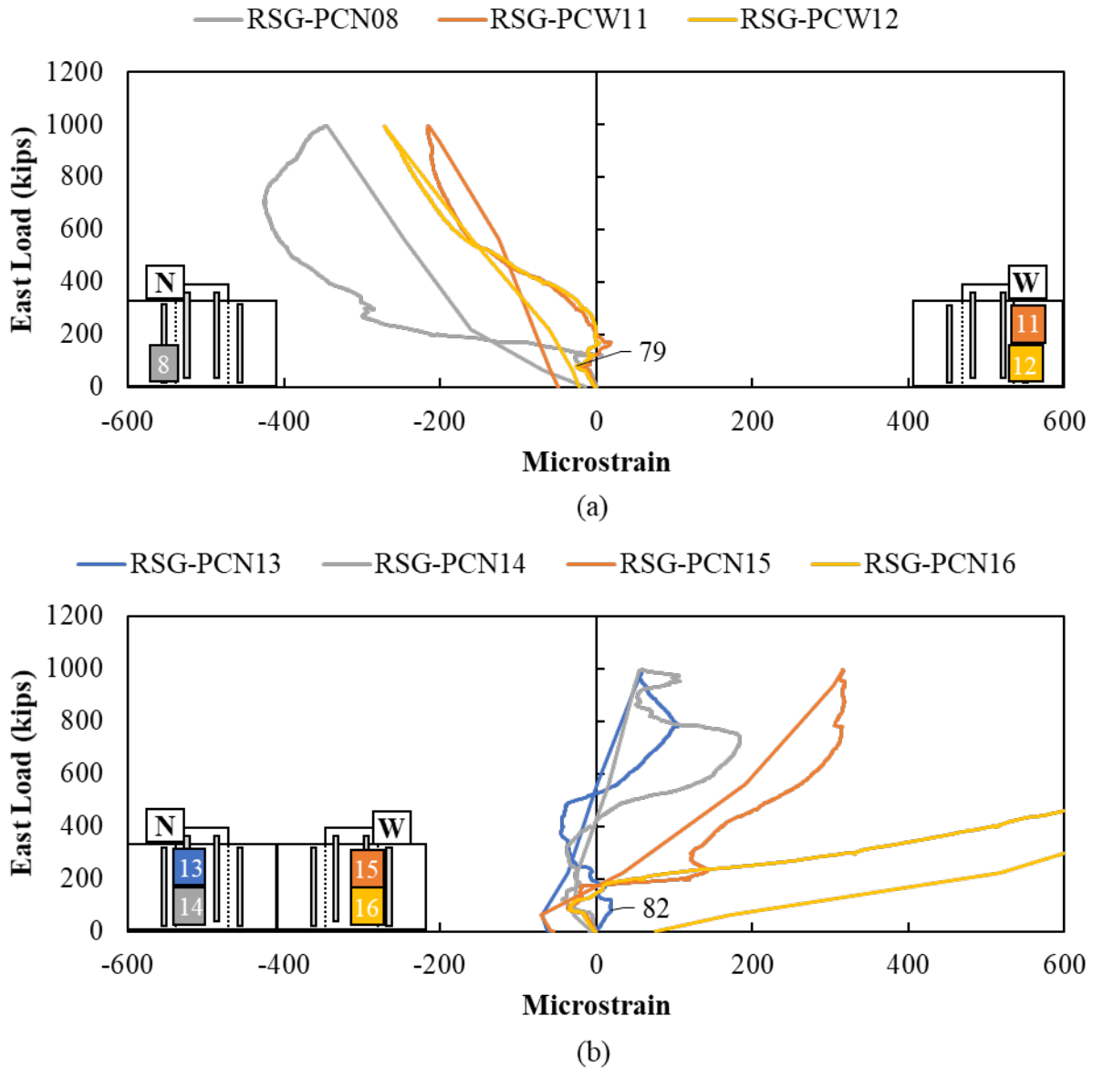
Figure B.13: Rebar strain gauge in vertical reinforcement on (a) cap and (b) plug of Specimen LP-2
