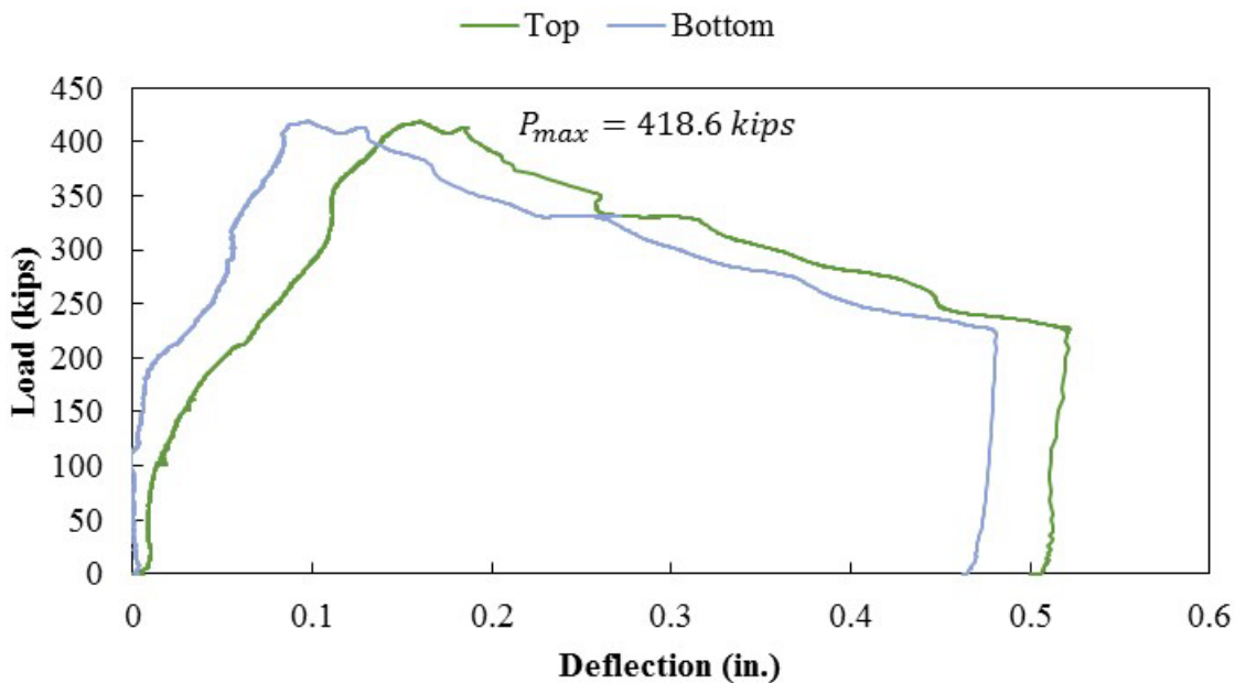
Figure A.56: Load versus deflection curve for Specimen S2-6
