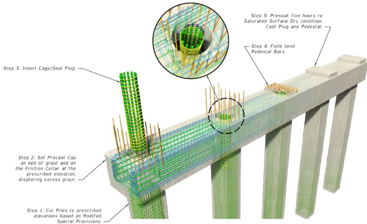
Figure 2.22: Pile cap erection process [52]
