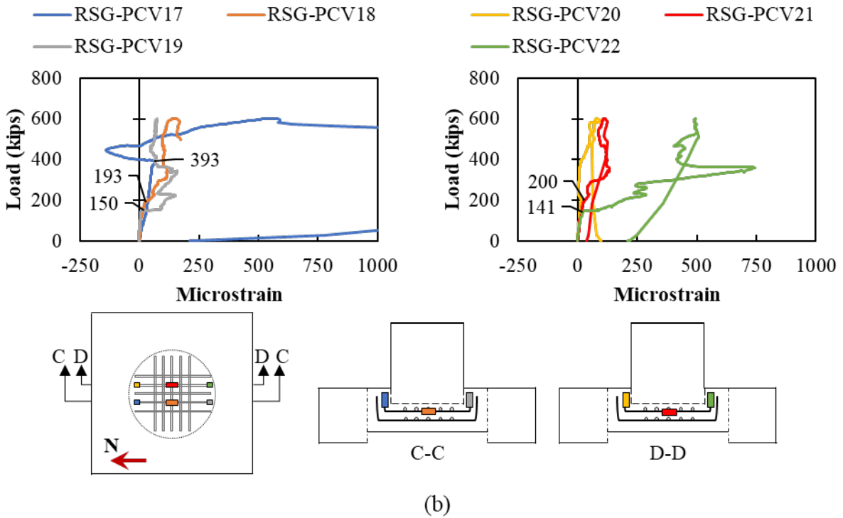
Figure B.57: Load versus strain measured using RSG for (a) bottom layer and (b) top layer of void reinforcement in Specimen SC-2 in the north-south direction.
