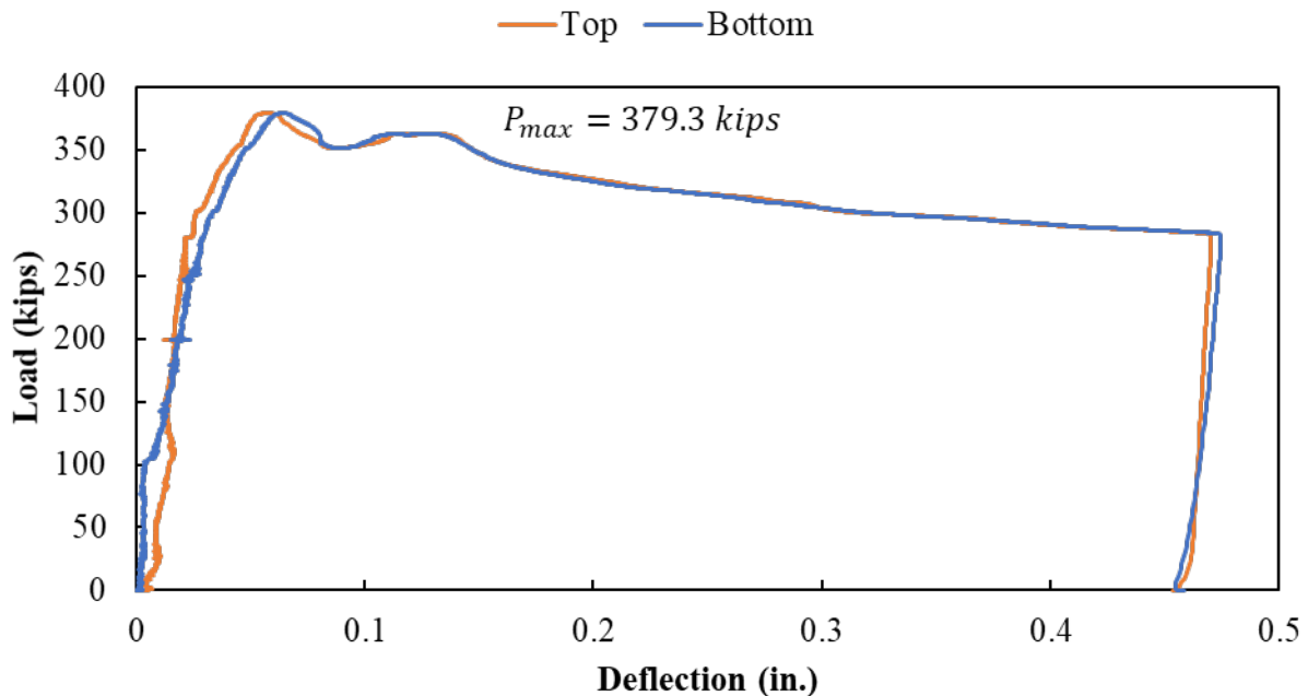
Figure A.187: Load versus deflection curve for Specimen S3-8
