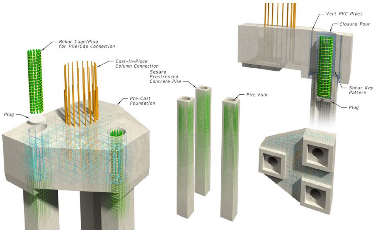
Figure 2.21: Precast footing connection recommended by FDOT [52].
