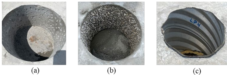
Figure 4.5: Surface finishes for larger-plug specimens: (a) electrical hammer with chisel attachment, (b) exposed aggregate finish, and (c) metal pipe left in place.
