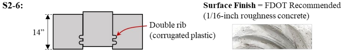
Figure A.55: Details for S2-6
