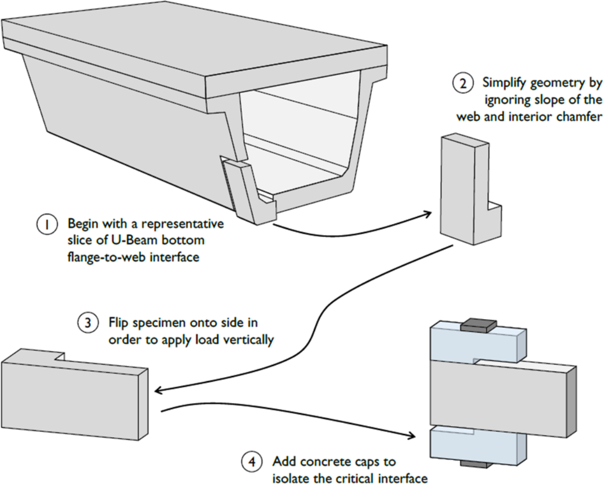
Figure 2.10: Location of shear friction specimen in actual U-beam [36]
