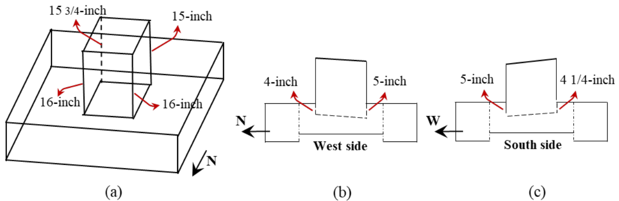
Figure 4.21: Pile embedment details in specimen SC-2: (a) measurements taken at site, (b) west side view and embedment of the pile, and (c) south view and embedment of the pile.
