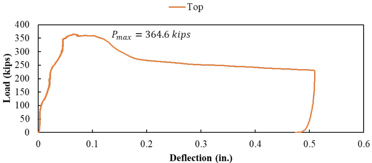
Figure A.194: Load versus deflection curve for Specimen S3-9
