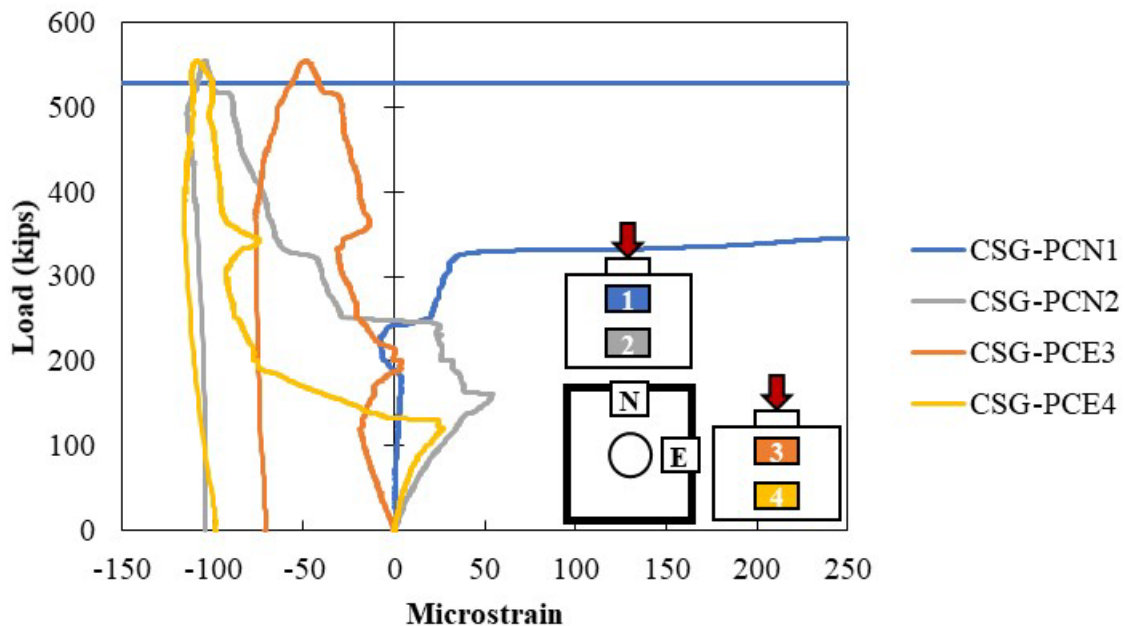
Figure A.72: Concrete strain gauges in the surface of the cap of Specimen S2-8
