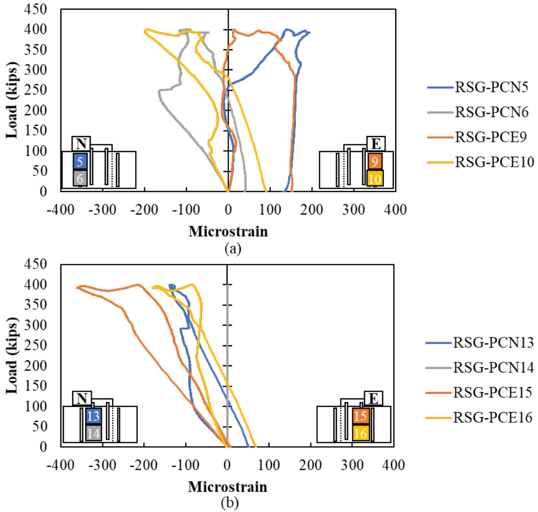
Figure A.97: Rebar strain gauges in vertical reinforcement on (a) the cap and (b) plug of Specimen S2-11
