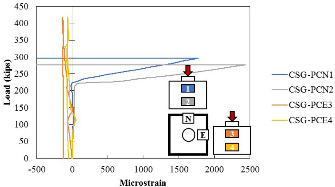
Figure A.58: Concrete strain gauges in the surface of Specimen S2-6
