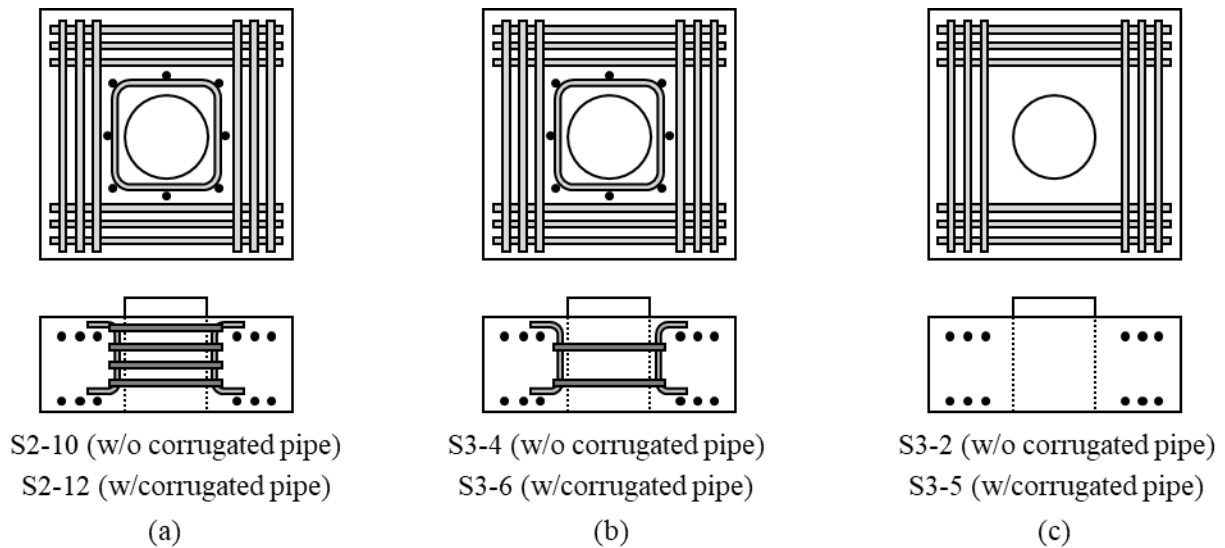
Figure 3.46: Reinforcement details for confinement reinforcement specimens, (a) full longitudinal reinforcement, (b) 2/3 longitudinal reinforcement, and (c) no longitudinal reinforcement
