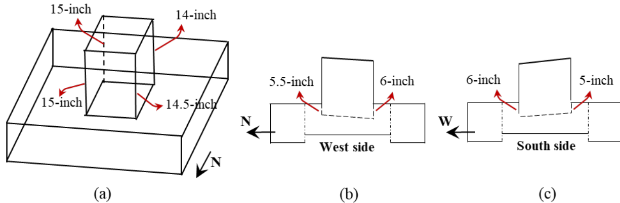
Figure 4.20: Pile embedment details in specimen SC-1: (a) measurements taken at site, (b) west side view and embedment of the pile, and (c) south view and embedment of the pile.
