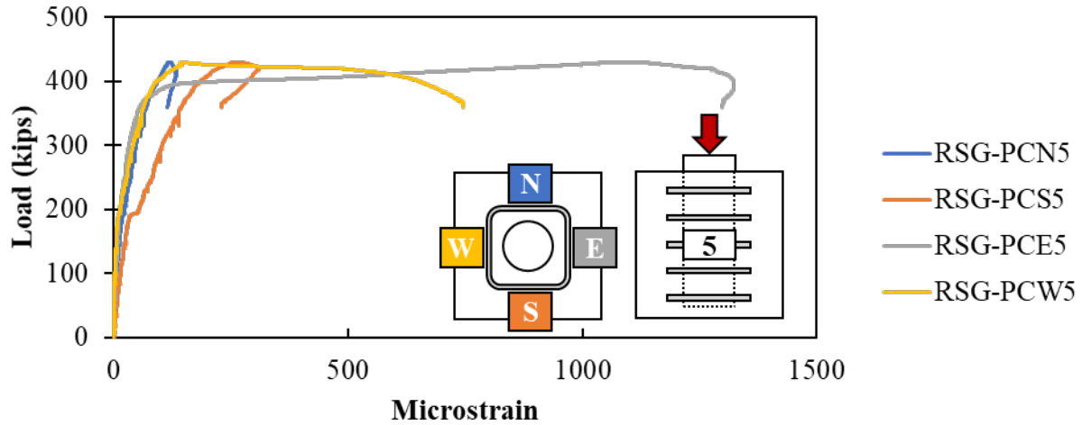
Figure A.18: Rebar strain gauges on confining reinforcement at mid-depth of the plug of Specimen S1-4. Specimen S1-4 had a smooth interface between the plug and cap, so it was initially assumed that only the cohesion component of the shear friction capacity should be considered. It appears that there were some stresses perpendicular to the friction plane though, evident from the cracking stresses, so there would have also likely also been a friction component to the shear friction resistance.
