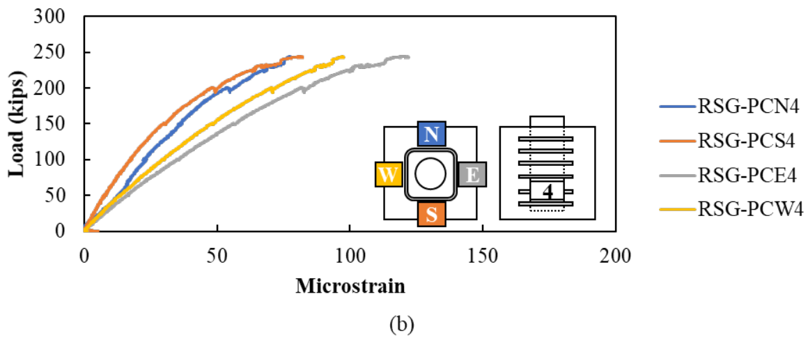
Figure A.12: Rebar strain gauges on confining reinforcement at (a) top and (b) bottom of the plug of Specimen SI-3
