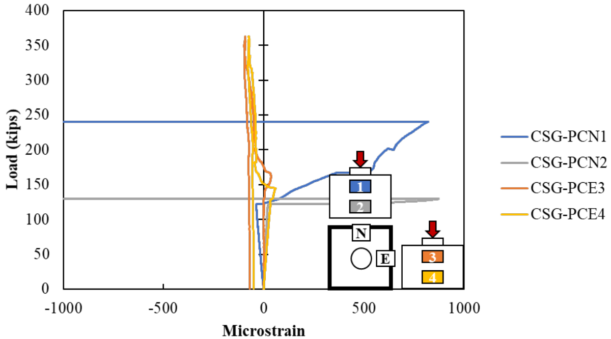
Figure A.217: Concrete strain gauges in the surface of Specimen S3-12
