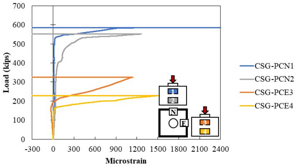
Figure A.44: Concrete strain gauges in the surface of the cap of Specimen S2-4
