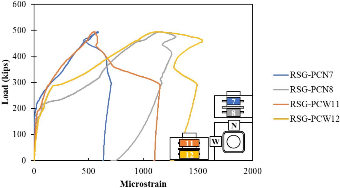
Figure A.164: Confining reinforcement around pocket of Specimen S3-4
