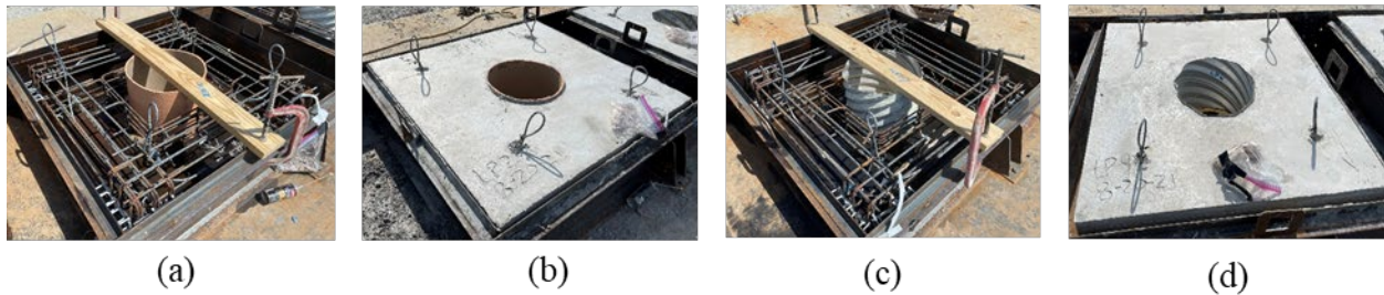
Figure 4.1: Construction and casting of cap: (a) placement of reinforcement and (b) casting of cap concrete for specimen with Sonotube and (c) placement of reinforcement and (d) casting of cap concrete for specimen with corrugated metal pipe.
