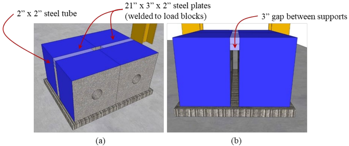
Figure 3.10: Load blocks with 3-inch of separation (a) overview and (b) lateral view of gap.
