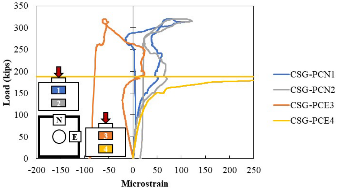
Figure A.37: Concrete strain gauges in the surface of the cap of Specimen S2-3
