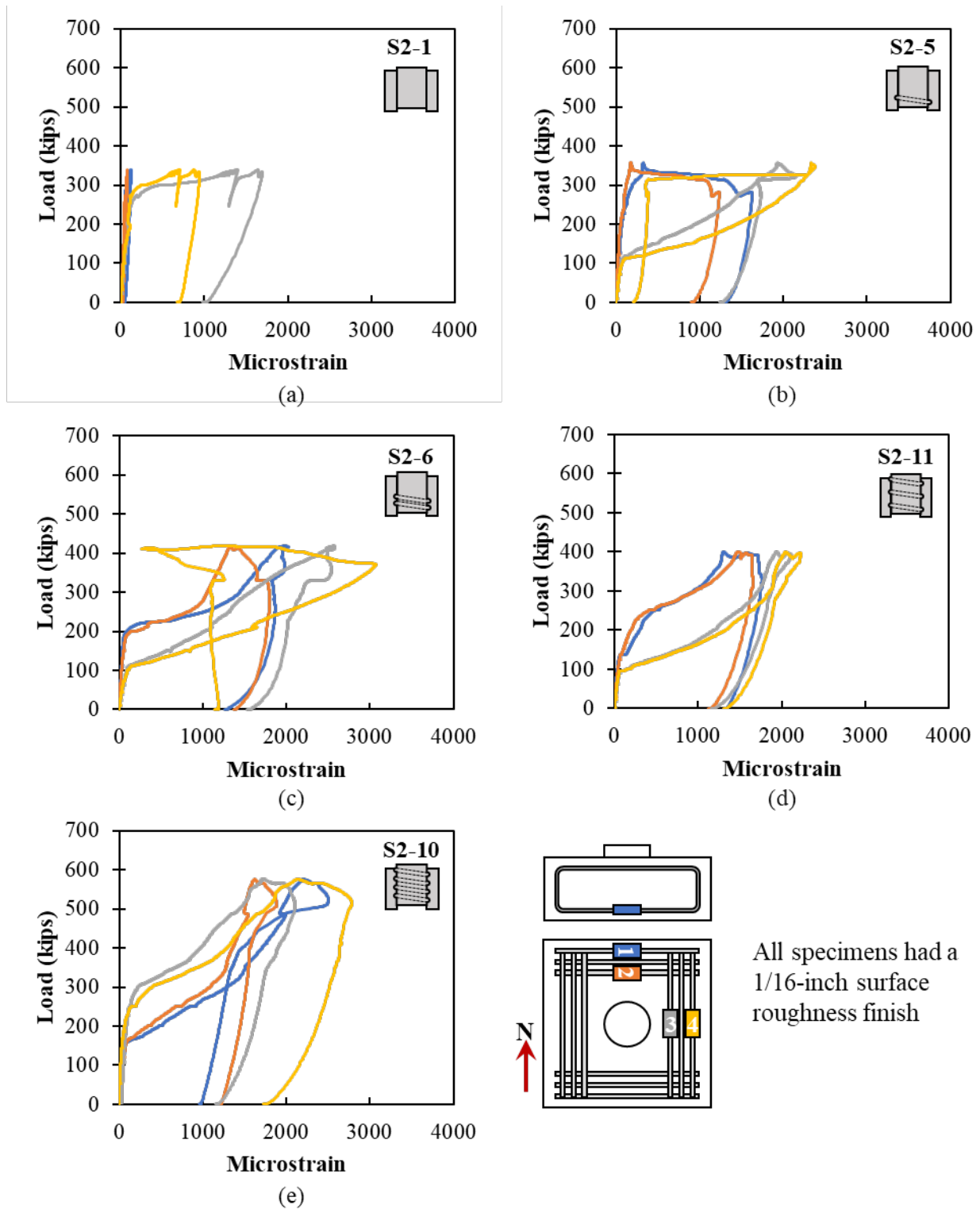
Figure 3.31: Load versus strain in longitudinal reinforcement for (a) S2-1, (b) S2-5, (c) S2-6, (d) S2-11, and (e) S2-10
