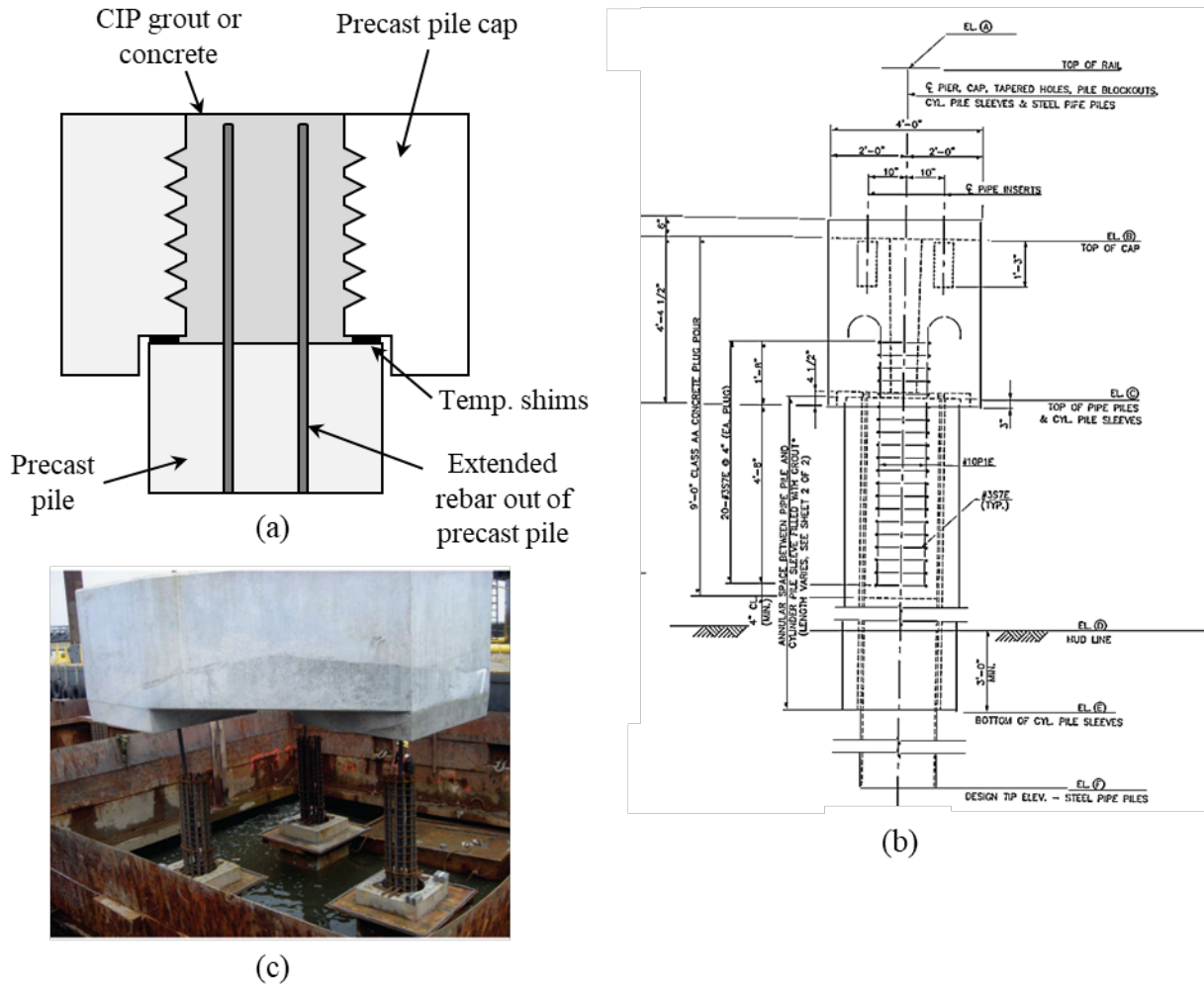
Figure 2.19: Examples of pocket connection between pile cap and pile: (a) connection between two precast elements; (b) connection use in Beaufort and Morehead Railroad Trestle Bridge[48]; (c) connection use in I-10 Bridge over Escambia Bay[49].
