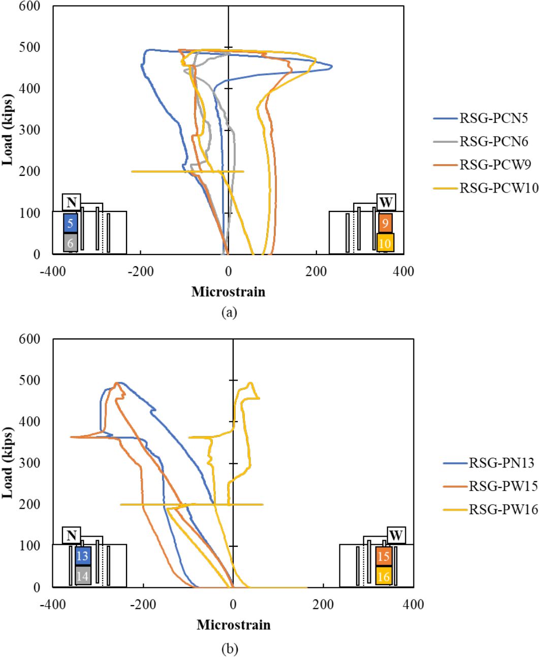
Figure A.165: Rebar strain gauges in vertical reinforcement on (a) cap and (b) plug of Specimen S3-4
