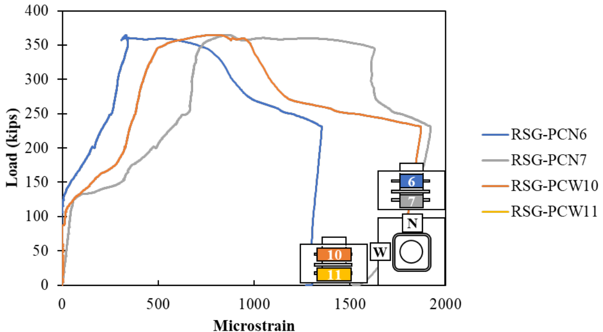
Figure A.198: Confining reinforcement around pocket of Specimen S3-9
