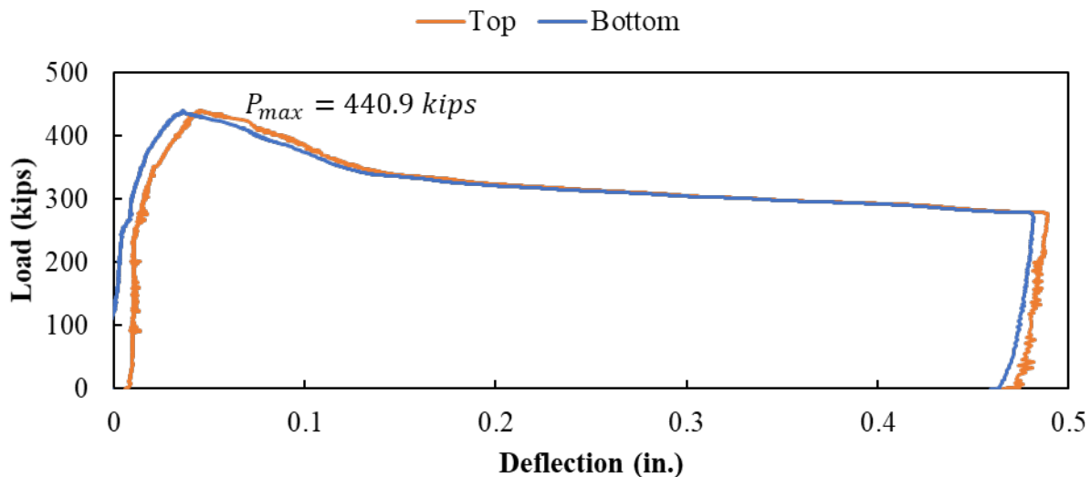
Figure A.153: Load versus deflection curve for Specimen S3-3
