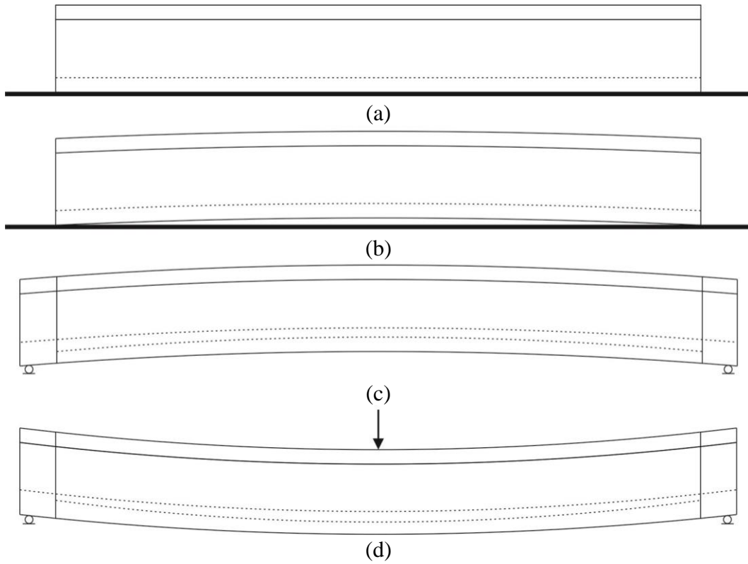
Figure 8.106 Constructions stages for simply-supported beams: (a) application of gravity to girder placed over prestressing bed, (b) pretensioning, (c) addition of end blocks and post-tensioning, (d) external loads
