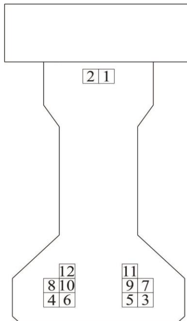
Figure 5.15 Detensioning pattern for SS specimens
