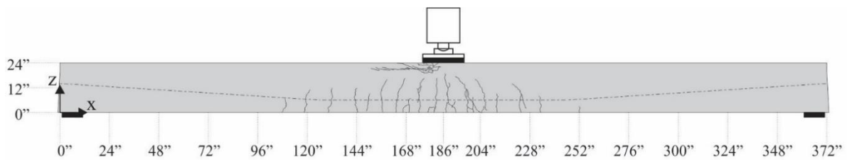
Figure D.2 Beam specimen SS-5 crack pattern: east side
