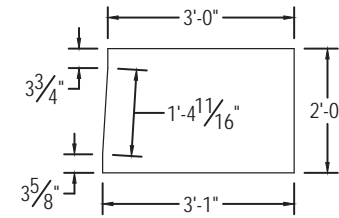
Endblock Dimensions
