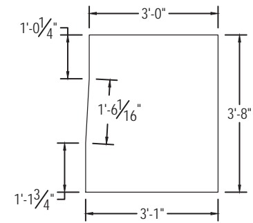
Endblock Dimensions
