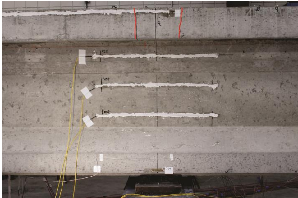
Figure E.8 Specimen NB-1: first observed cracks (marked in red) at P = 120 kip on east side
