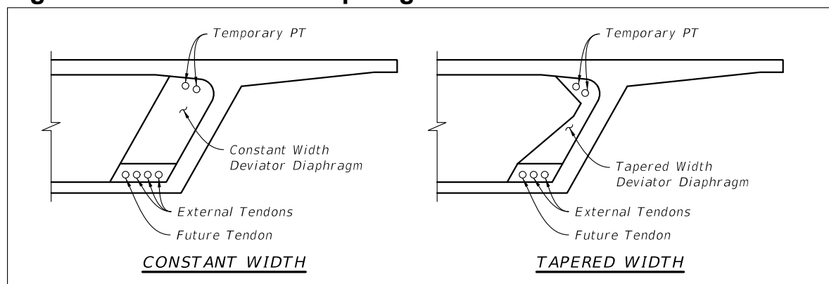
Figure 4.6.4-1 Deviator Diaphragm Detail
