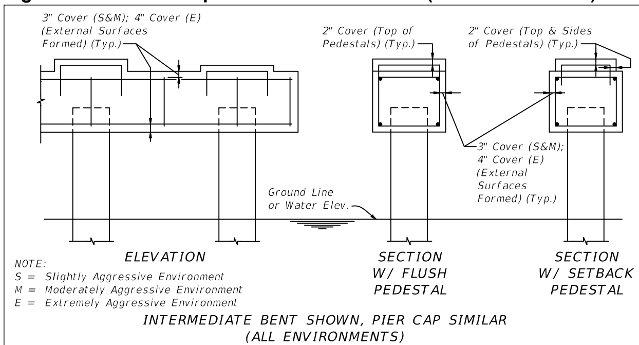
Figure 1.4.2-5 Pier Cap and Intermediate Bent (All Environments)
