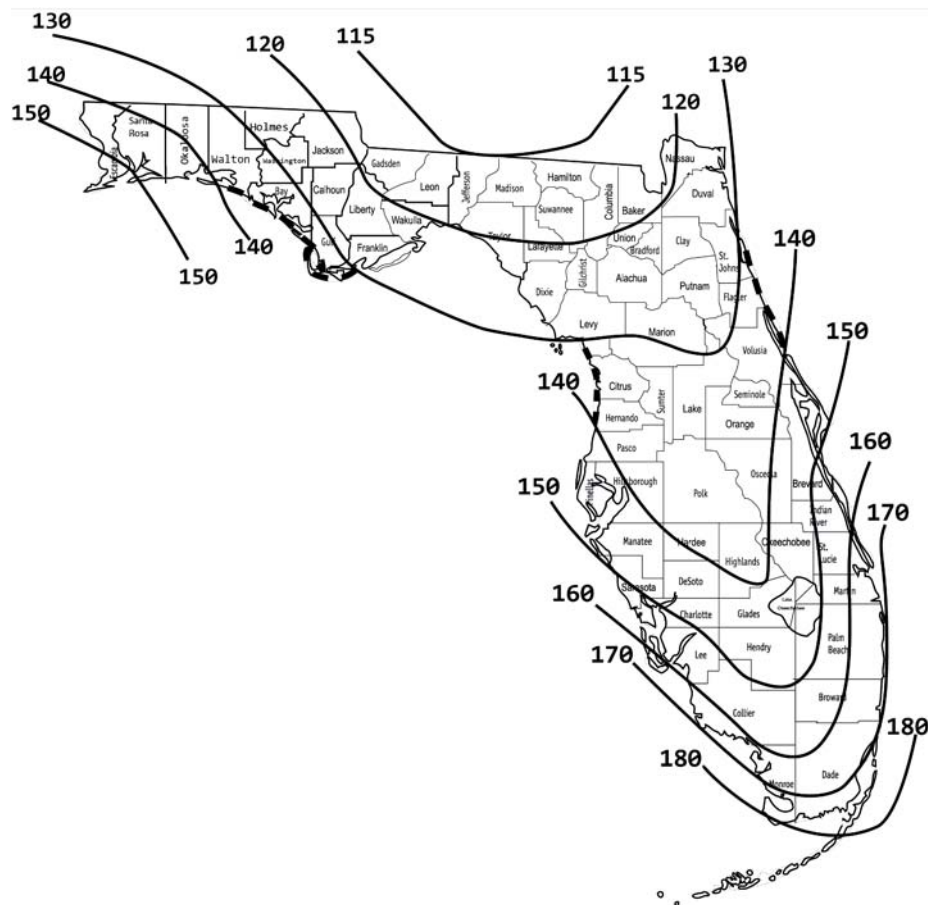
FDOT Figure 18.1-1 700-year MRI Florida Wind Speed Map
