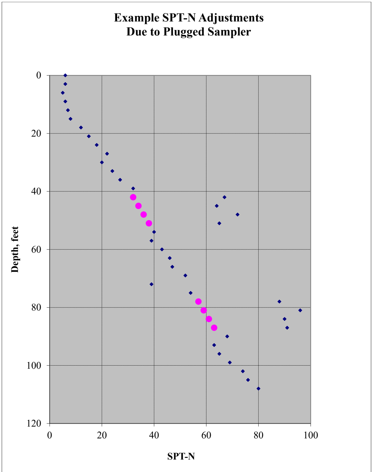
Figure 5, Example SPT-N Adjustments Due to Plugged Sampler
