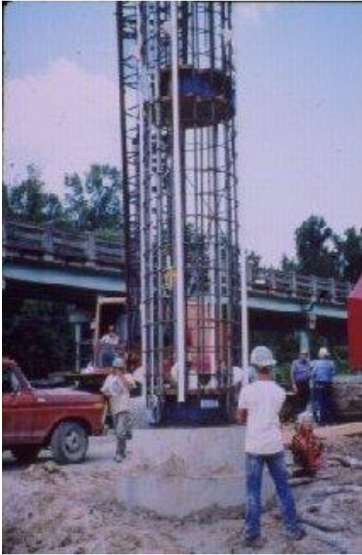
Figure 39, Osterberg Load Cells
