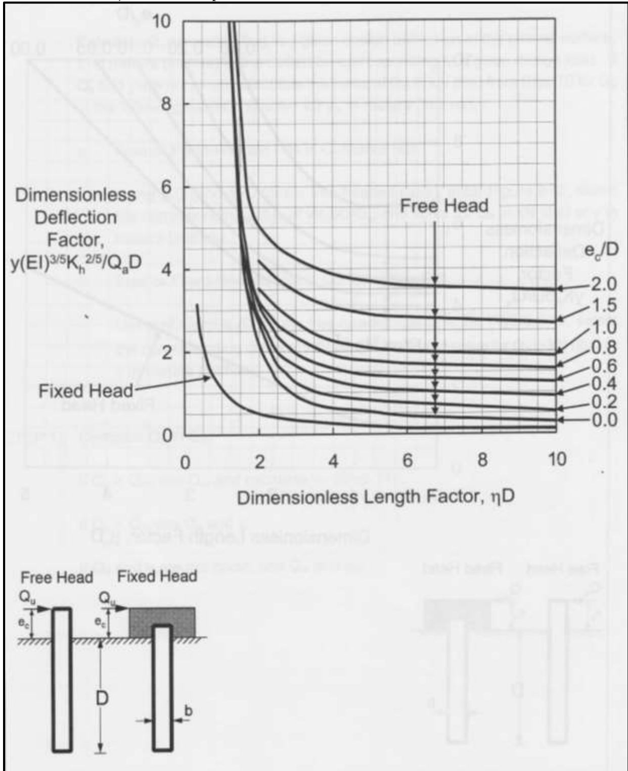
Figure 44, Broms' Deflection Factor vs. Length Factor (after FHWA-NHI-05-042) ( K_h = k_h )
