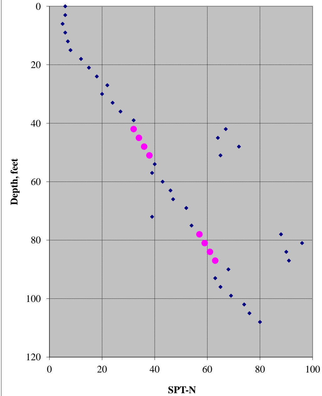
Figure 6 Example SPT-N Adjustments Due to Plugged Sampler
