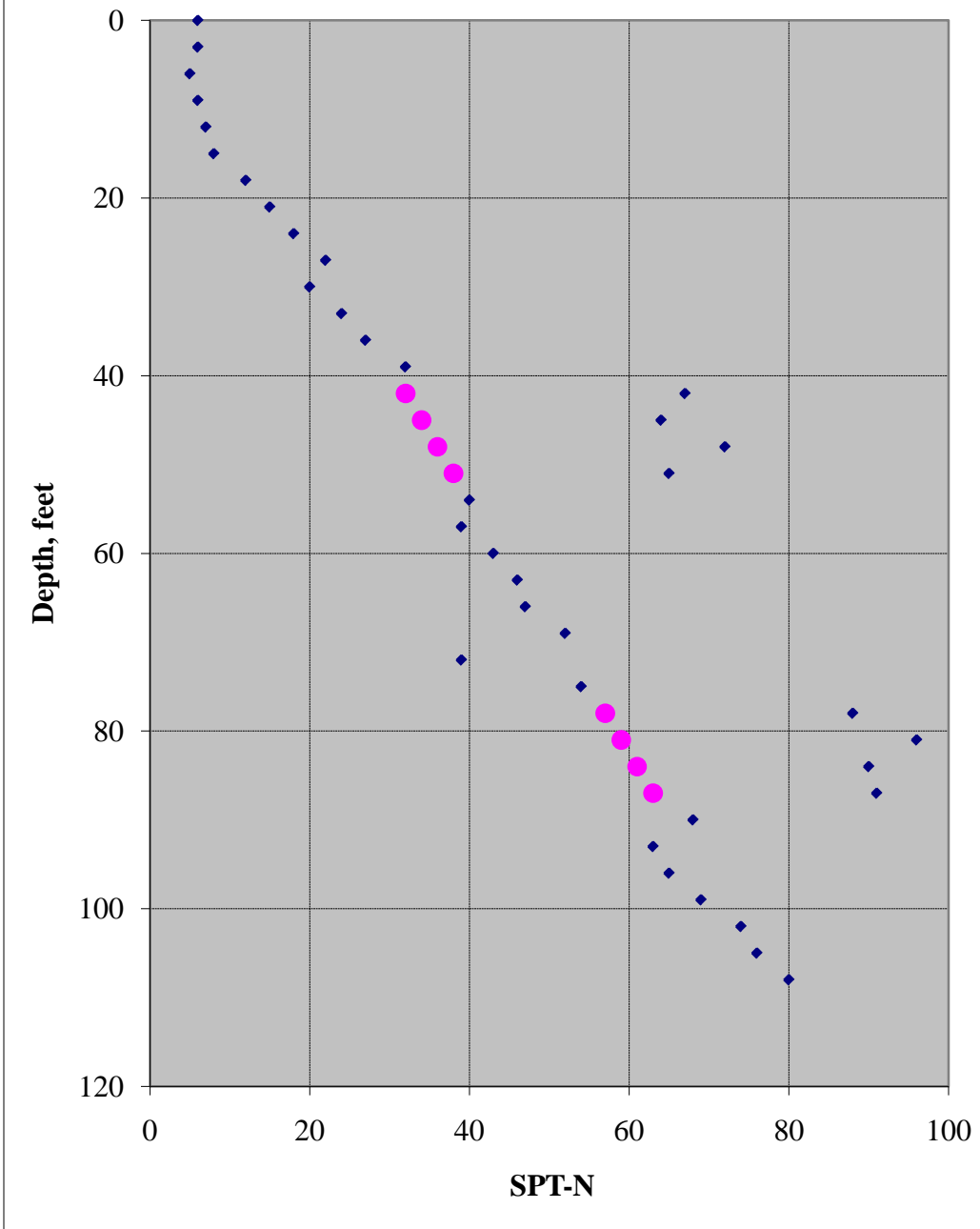
Figure 6 Example SPT-N Adjustments Due to Plugged Sampler
