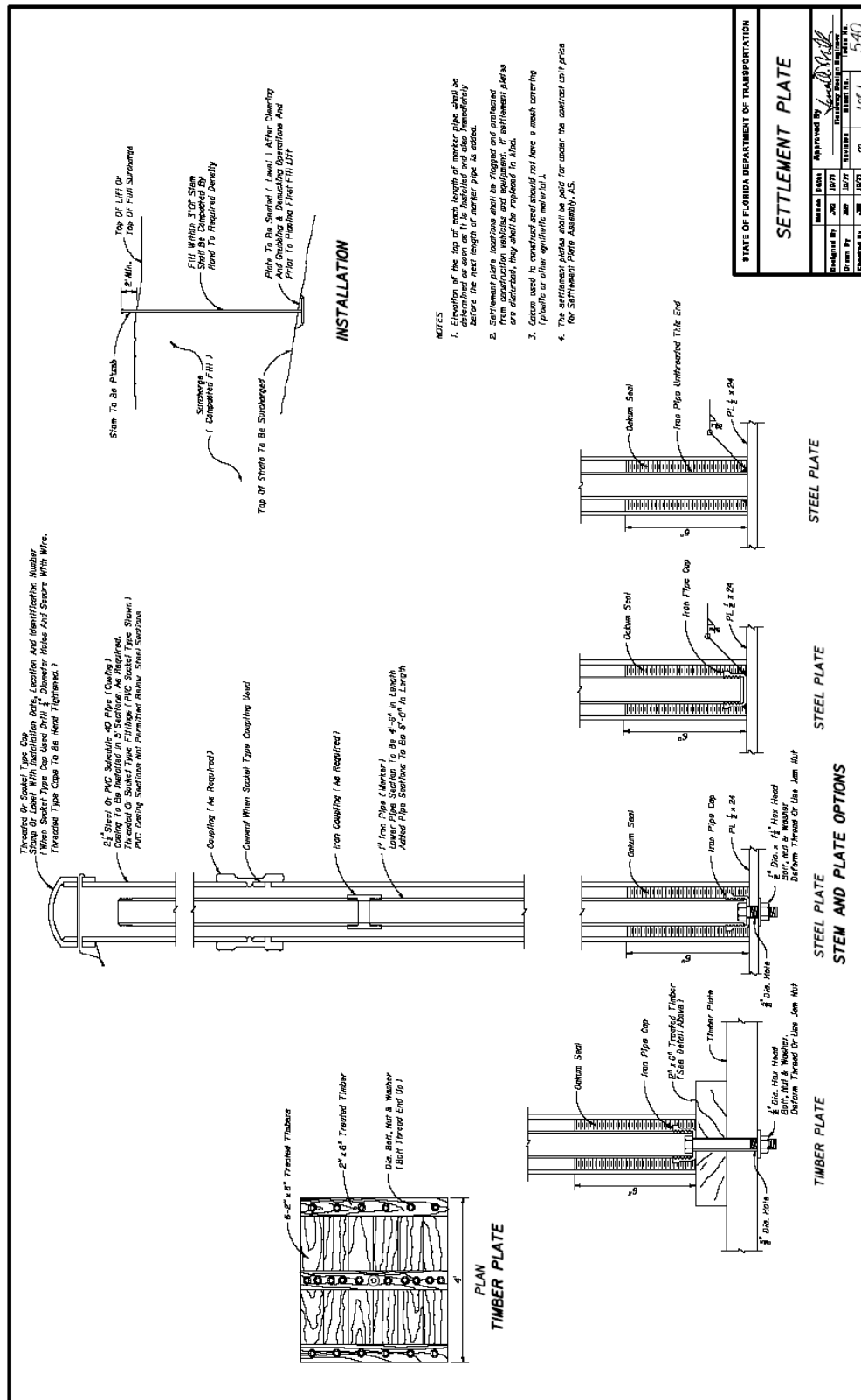
Figure 28, Typical Settlement Platform Design (FDOT Standard Index 540)
