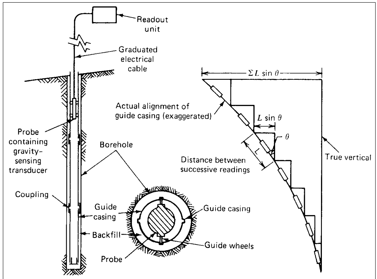
Figure 27, Principle of Inclinometer Operation (After Dunncliff, 1988)
