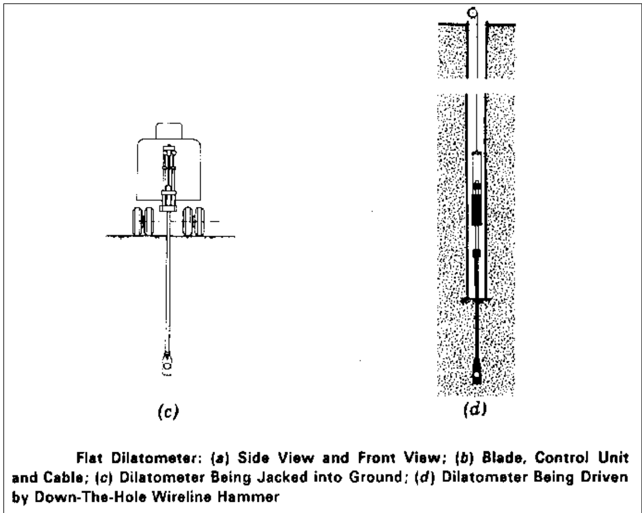
Figure 11, Dilatometer (Continued)
