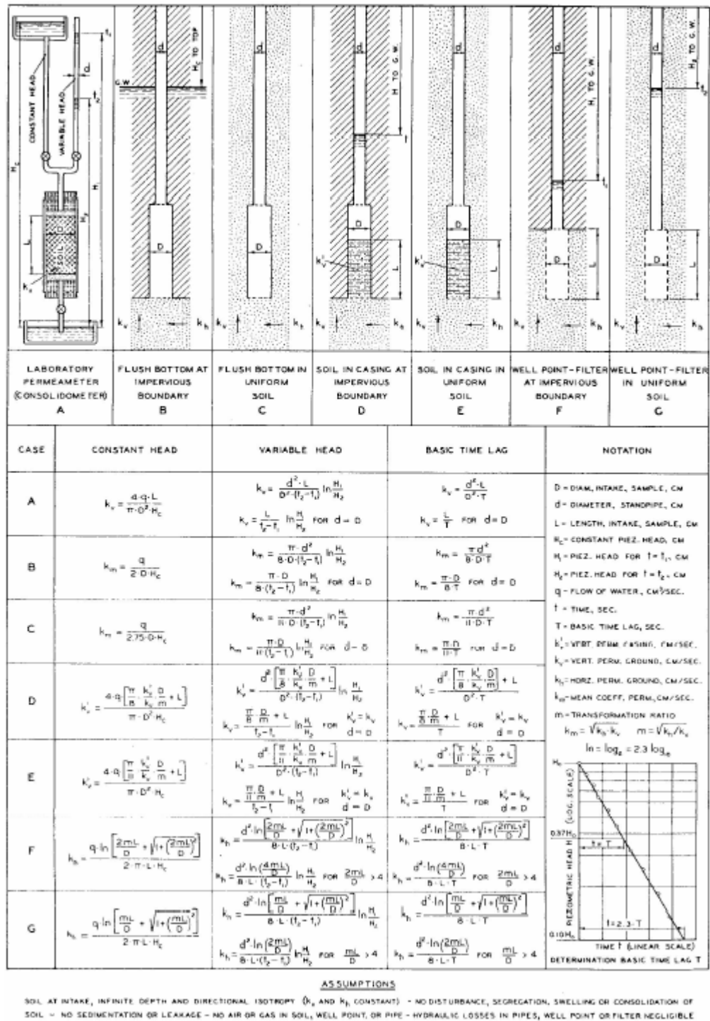
Figure 16, Formulas for Determination of Permeability (Hvorslev, 1951)
