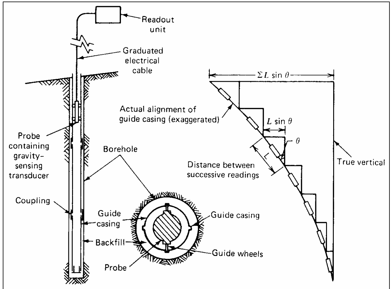
Figure 27, Principle of Inclinometer Operation (After Dunnicliff, 1988)
