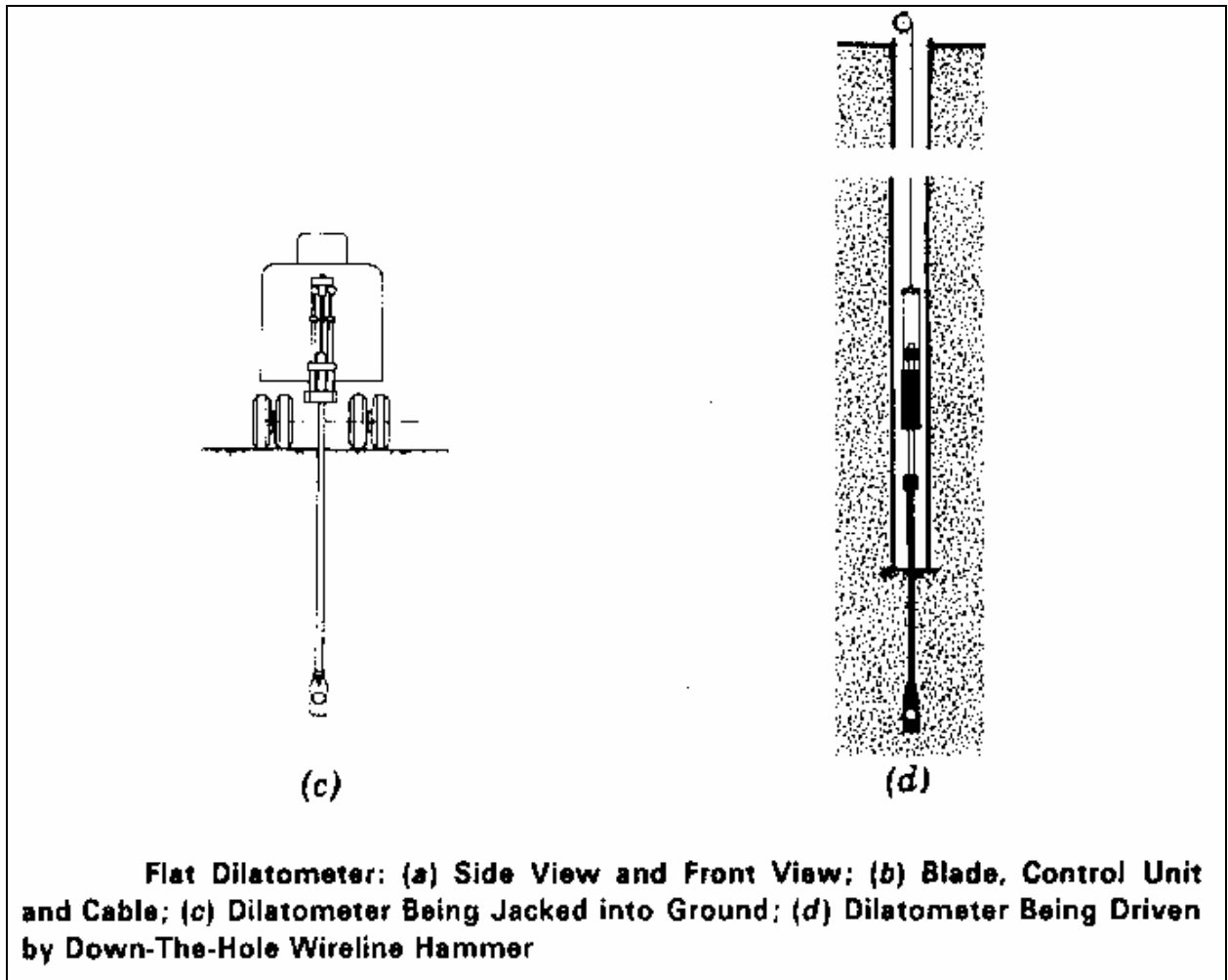
Figure 12, Dilatometer (Continued)
