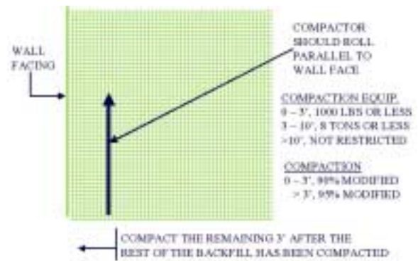
Figure 43, Final Compaction
