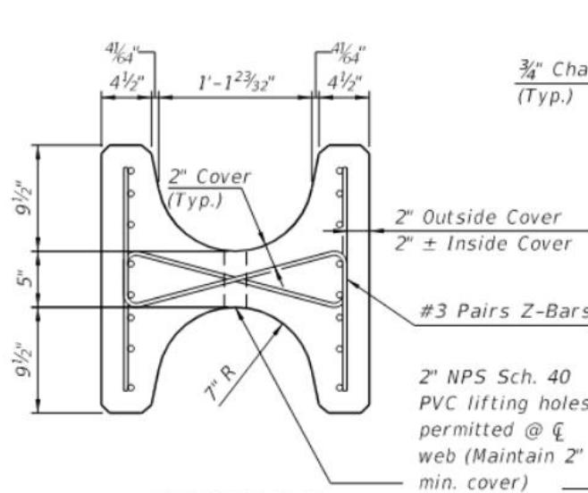
SECTION B-B (H-Shape - Option 1)
