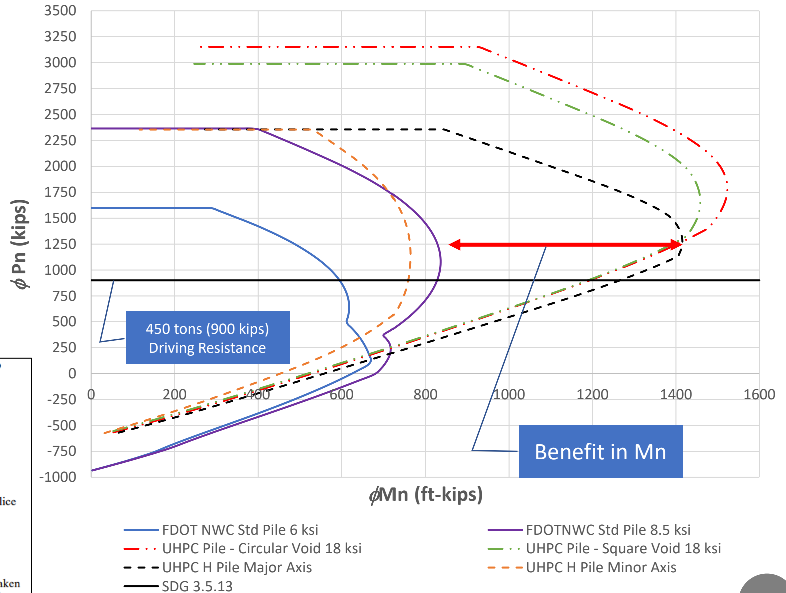
Example: 24" Pile Interaction Diagram
