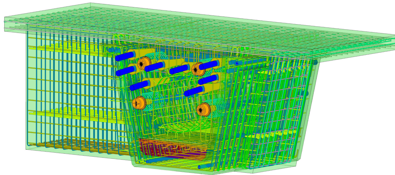
ROTATED VIEW LACED OPTION ILLUSTRATED
