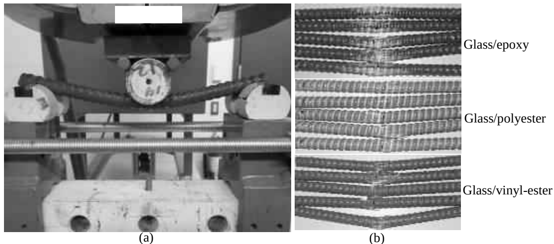
Figure 4.29: Setup for flexural testing and typical failure mode: (a) test setup; (b) failure mode
