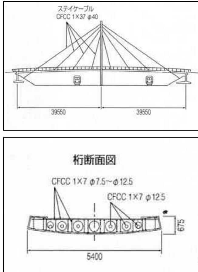
Figure 2.27: Herning footbridge
