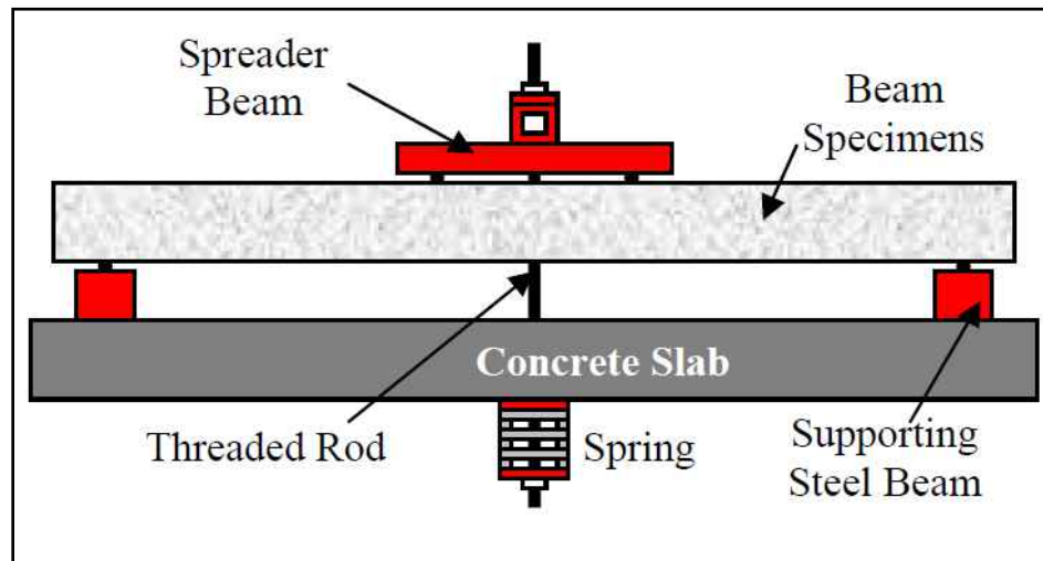
Figure 2.19: Test set-up for sustained loading (environmental exposure) (Mertol et al. 2007)
