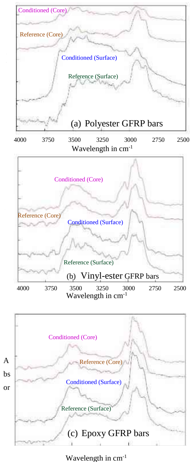
Figure 4.22: FTIR spectra of reference and specimens conditioned for 5,000 hr
