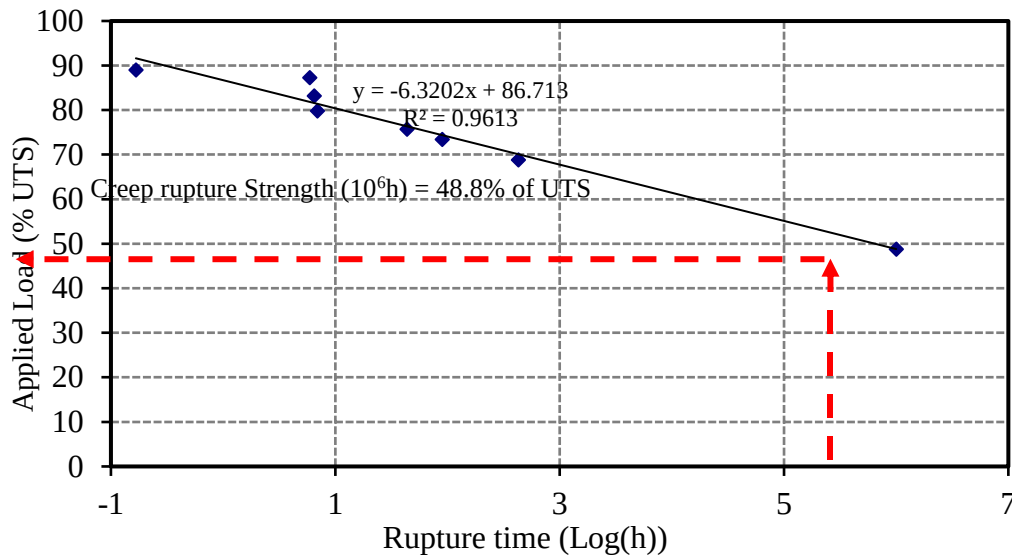
Figure 2.10: Logarithmic Time to Failure (Stress Rupture) Curve for GFRP bars (Robert et al. 2013).
