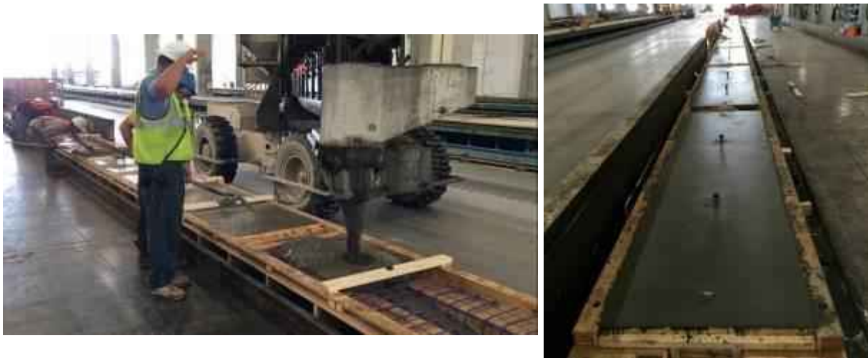
Figure 6.7: Casting of Concrete
