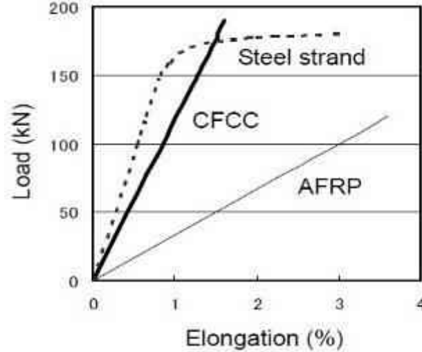
Figure 2.4: Load-Elongation curve (Enomoto and Ushijima 2012)
