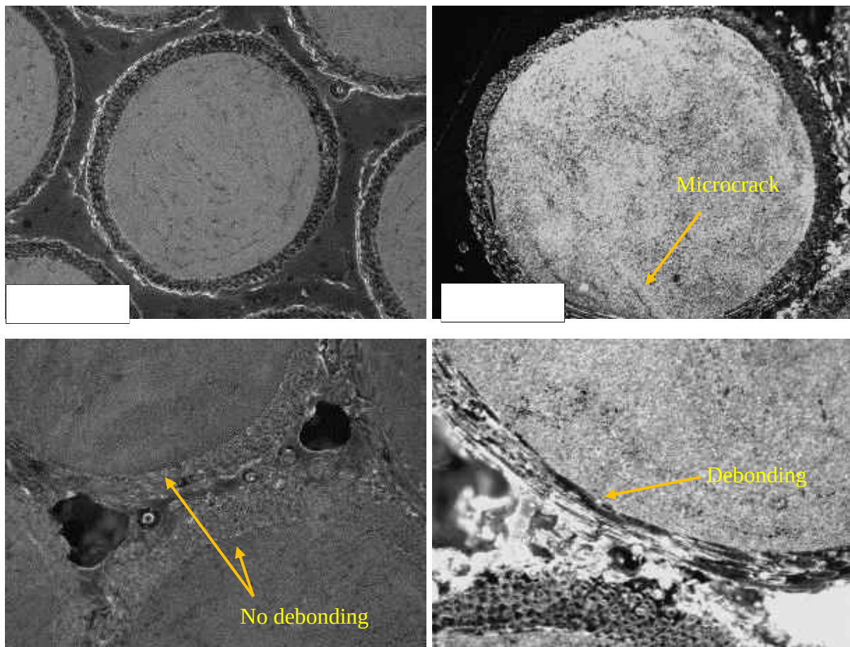
Figure 3.27: View of strand and Intersection between two strands
