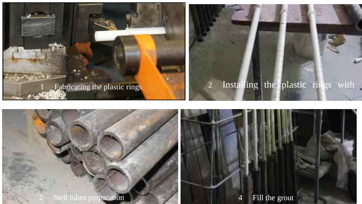
Figure 4.4: Preparation of the test GFRP bar specimens
