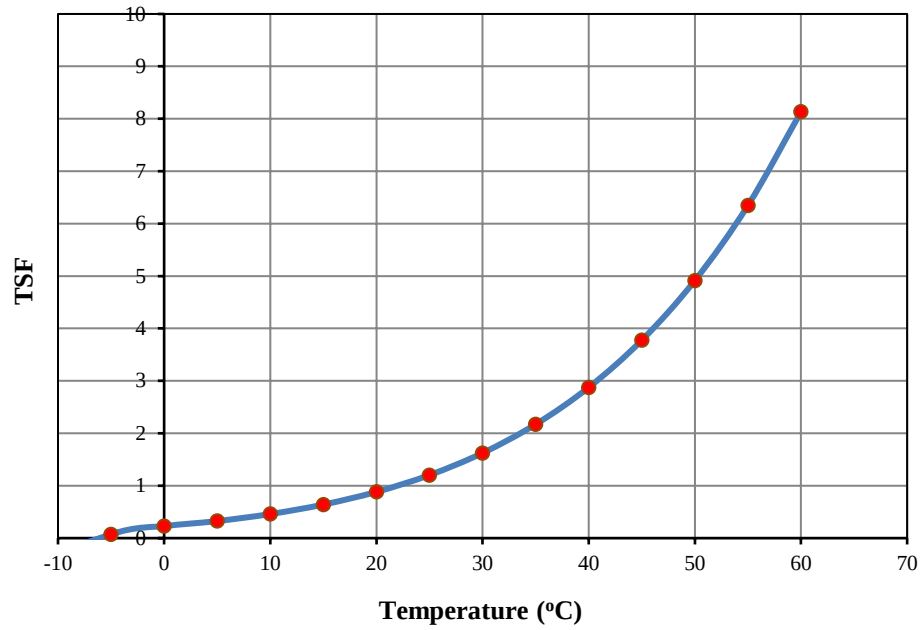
Figure 4.60: TSF versus temperature
