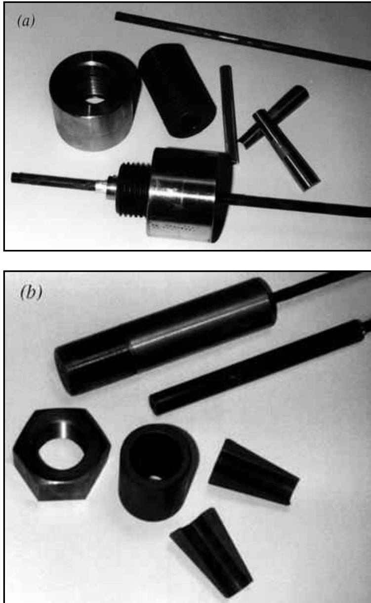
Figure 2.16: (a) Leadline PC-D8 tendon; (b) 1 x 7 CFRP and their respective grips (Saadatmanesh and Tannous 1999).
