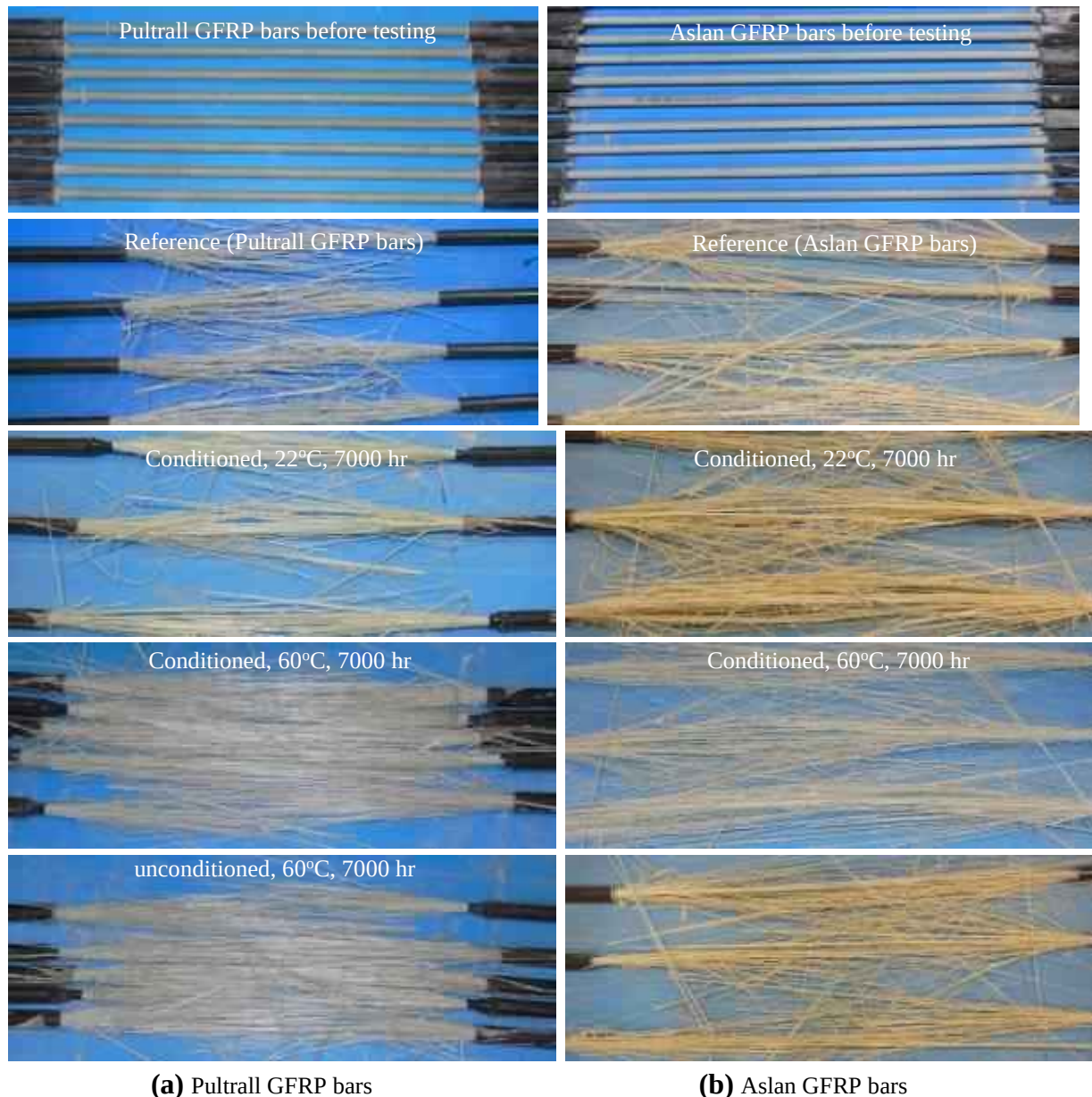
Figure 4.13: Typical mode of failure for Pultrall and Aslan GFRP bars
