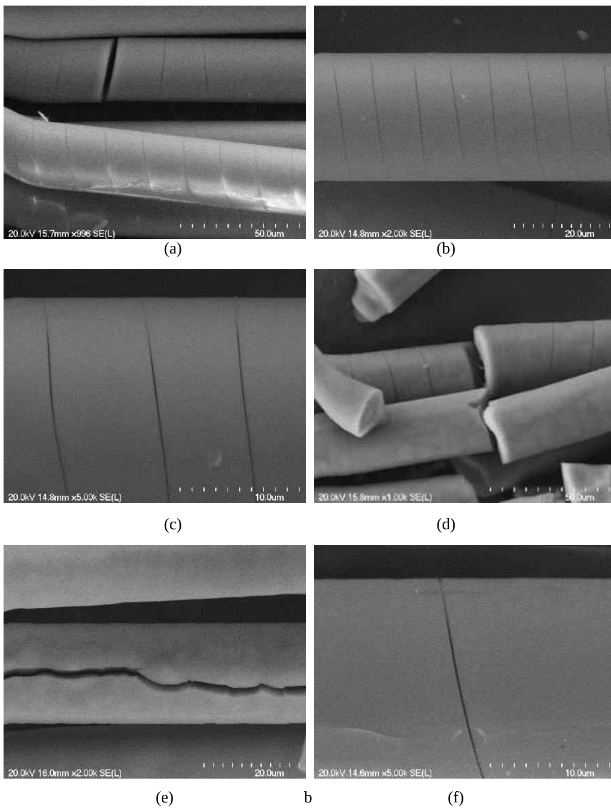
Figure 4.41: SEM analysis at of glass fiber submerged in HCl for 168 hr, a)V1 at 1000X, b)V1 at 2000X, c)V1 at 5000 d)V4 at 1000X, e)V4 at 2000X and f)V4 at 5000X
