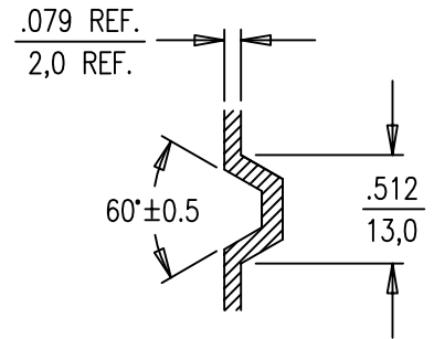
DETAIL SCALE 1:1
