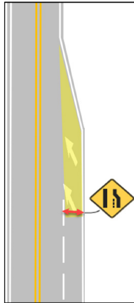
7: Merging Outside Lane
