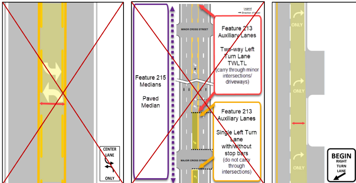
1: Two-way Left Turn Lane ( Obsolete September 2019)
