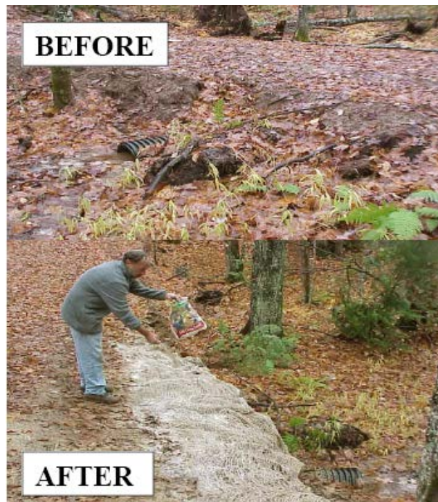
Figure AIII-10: Stream Crossing or Culvert Stabilization.
