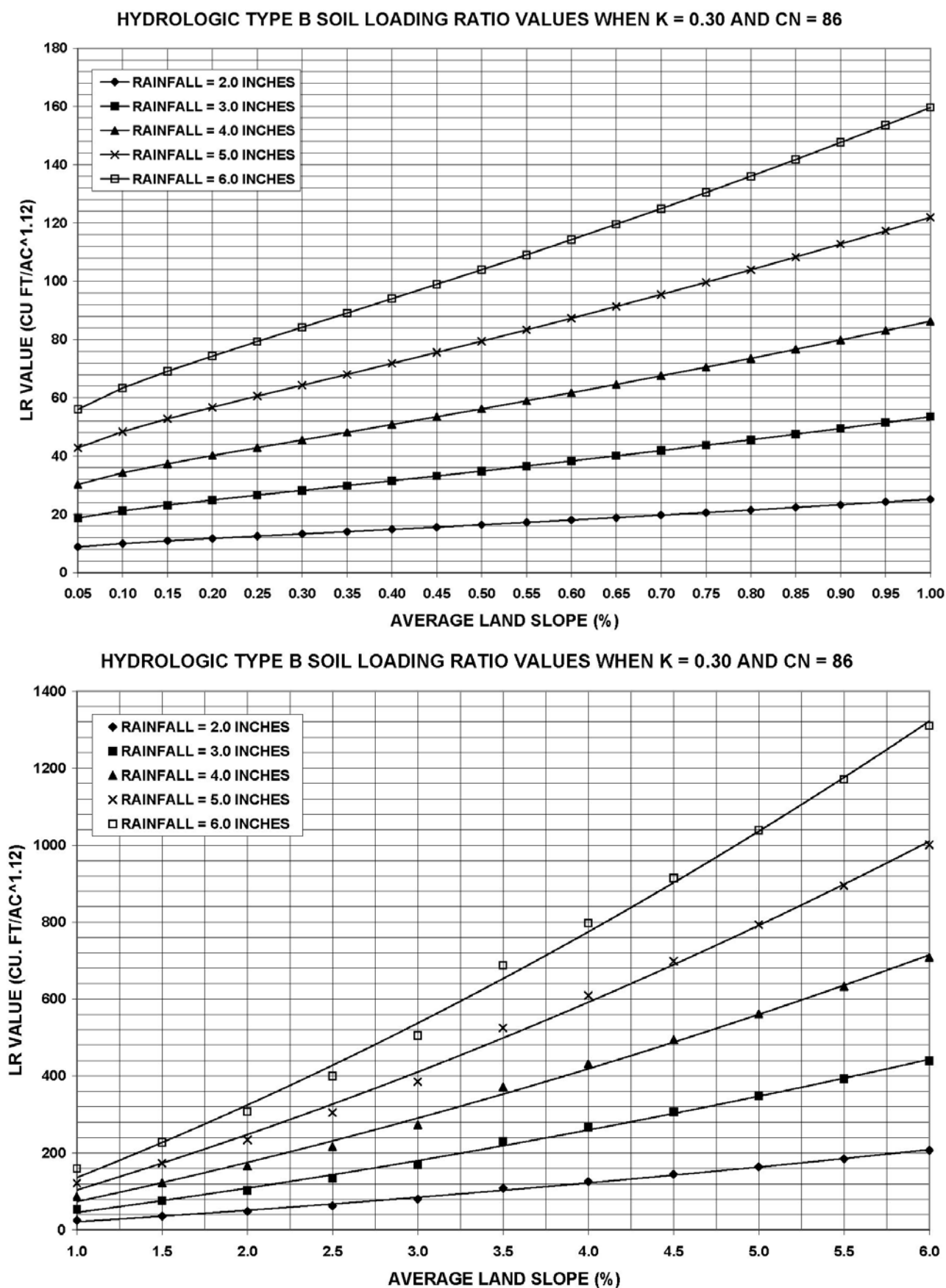
Figure IV-9: Hydrologic Type B Soils Loading Ratio Graph
