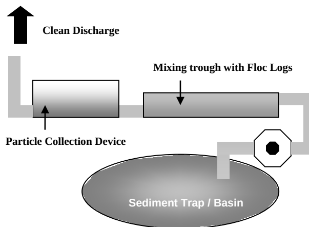
Using in-line mixing with a Floc Log
