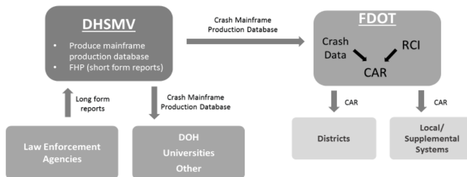
Figure 9. Crash data processing workflow.
