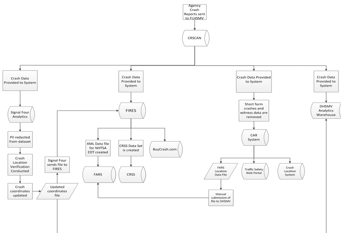
Figure 10. High-level crash systems relationship map.
