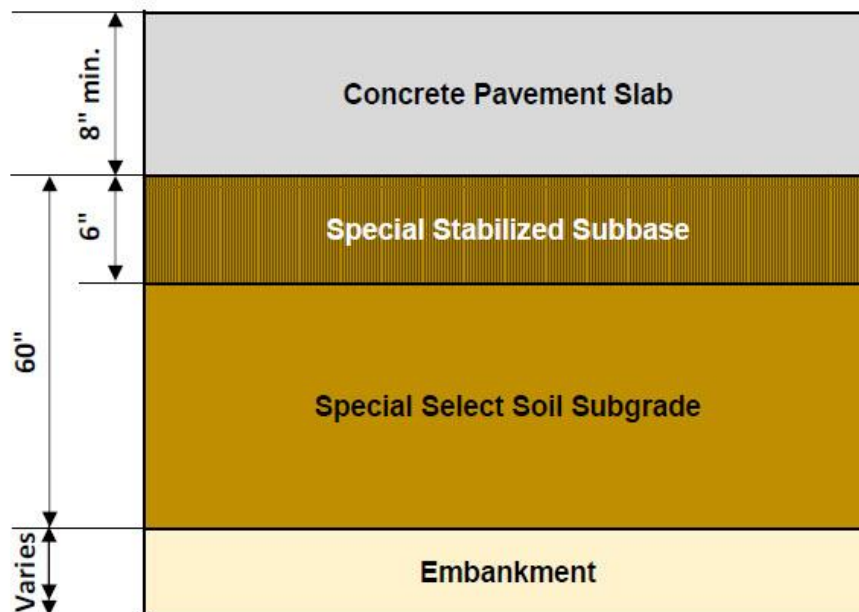
FIGURE 2.2 SPECIAL SELECT SOIL BASE OPTION
