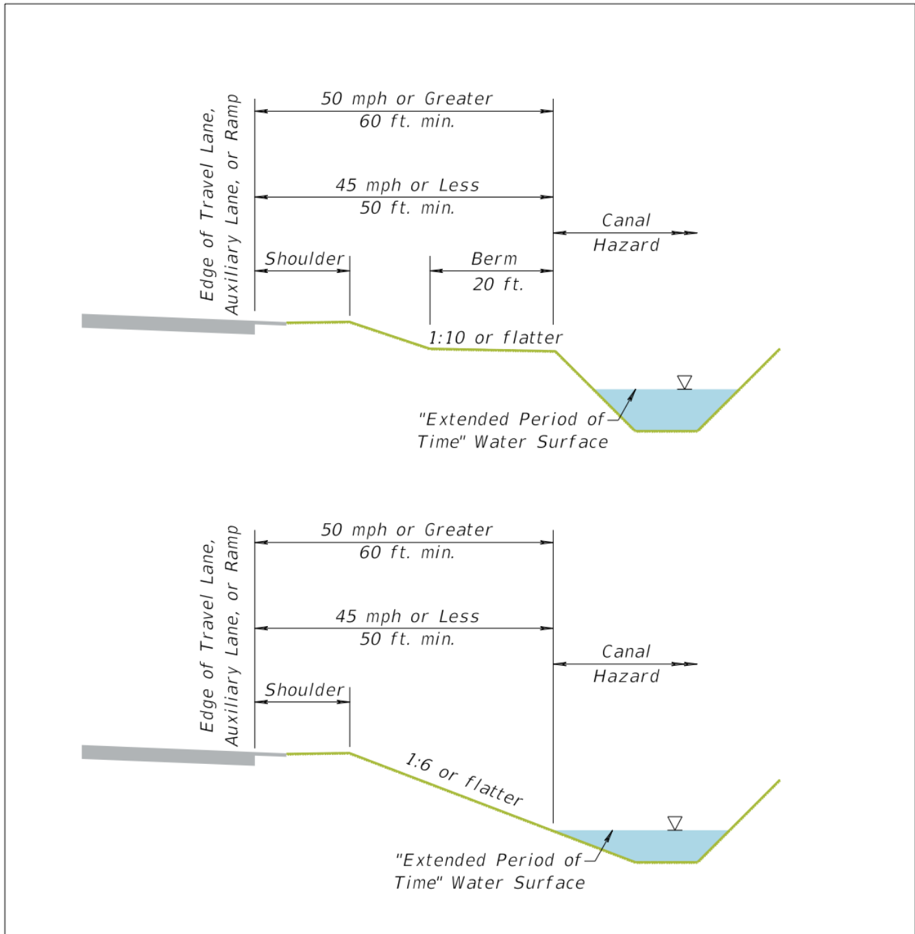
Figure 4-7. Minimum Offsets for Canal Hazards (Flush Shoulders)
