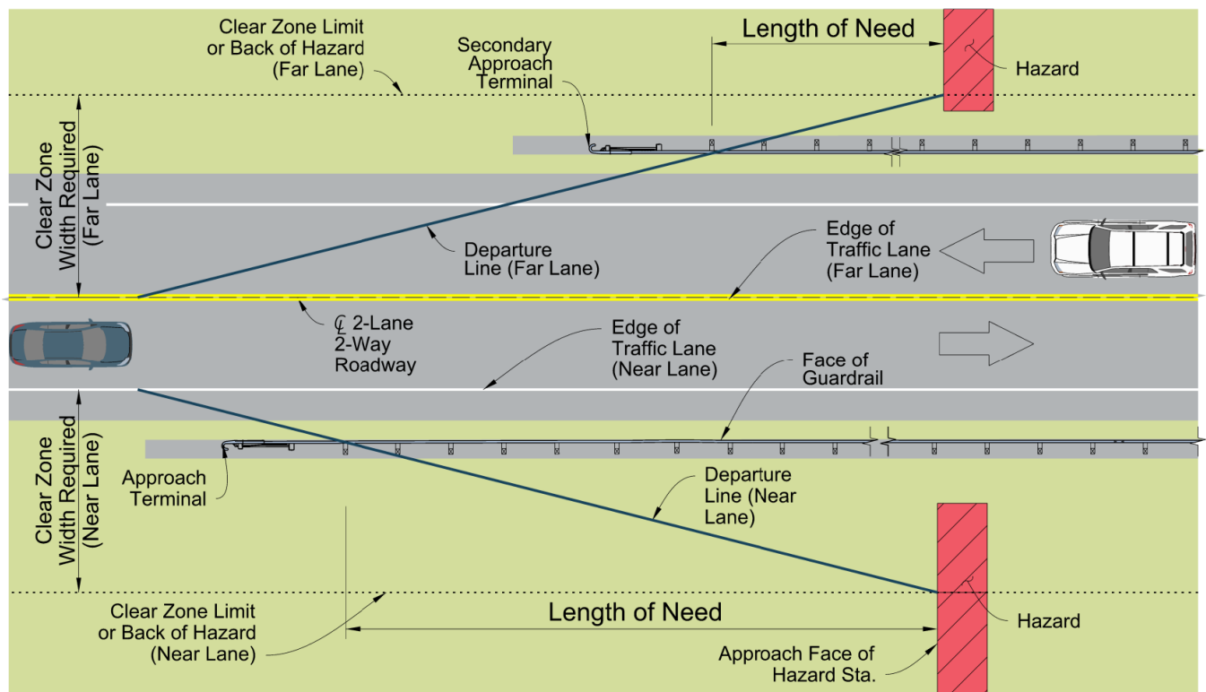
Figure 4-11. Approach Terminal Usage When End of Guardrail Is Within Clear Zone of Approaching Near and Far Lanes (Two-Lane, Two-Way Road)
