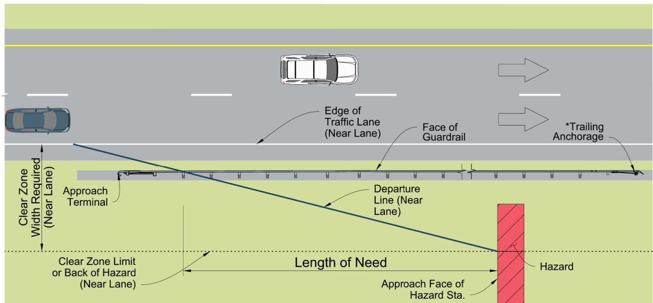
Figure 4-12. Approach Terminal and Trailing Anchorage Usage When End of Guardrail Is Within Clear Zone of Approaching Near Lane (Two-Lane, One-Way Road)
