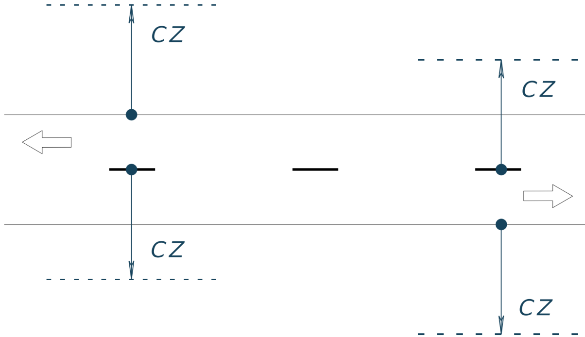
Figure 4-1. Clear Zone Plan View (Two-Lane, Two-Way Roadway)
