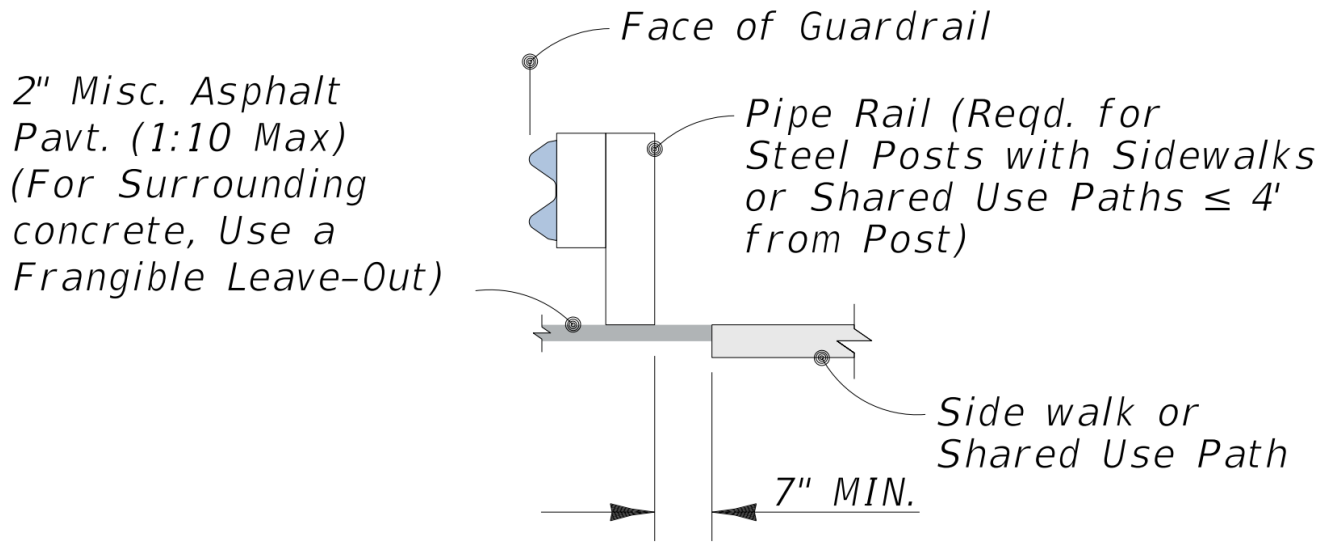
Figure 4-10. Guardrail with Pipe Rail Detail
