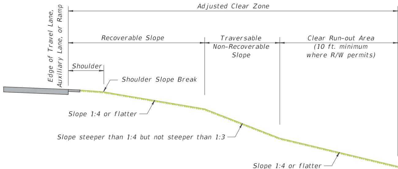
Figure 4-4. Adjusted Clear Zone Concept
