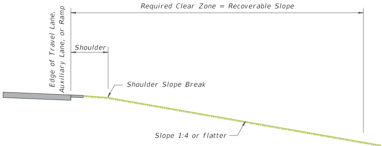
Figure 4-3. Basic Clear Zone Concept
