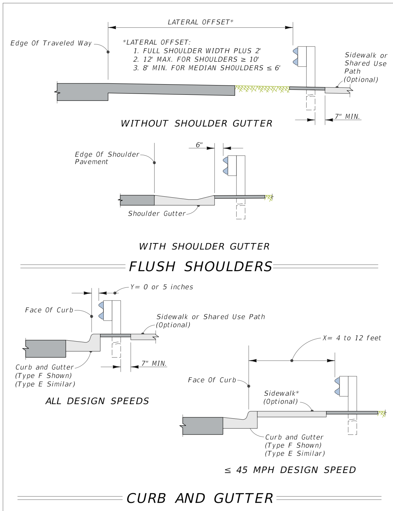
Figure 4-9. Location of Guardrail
