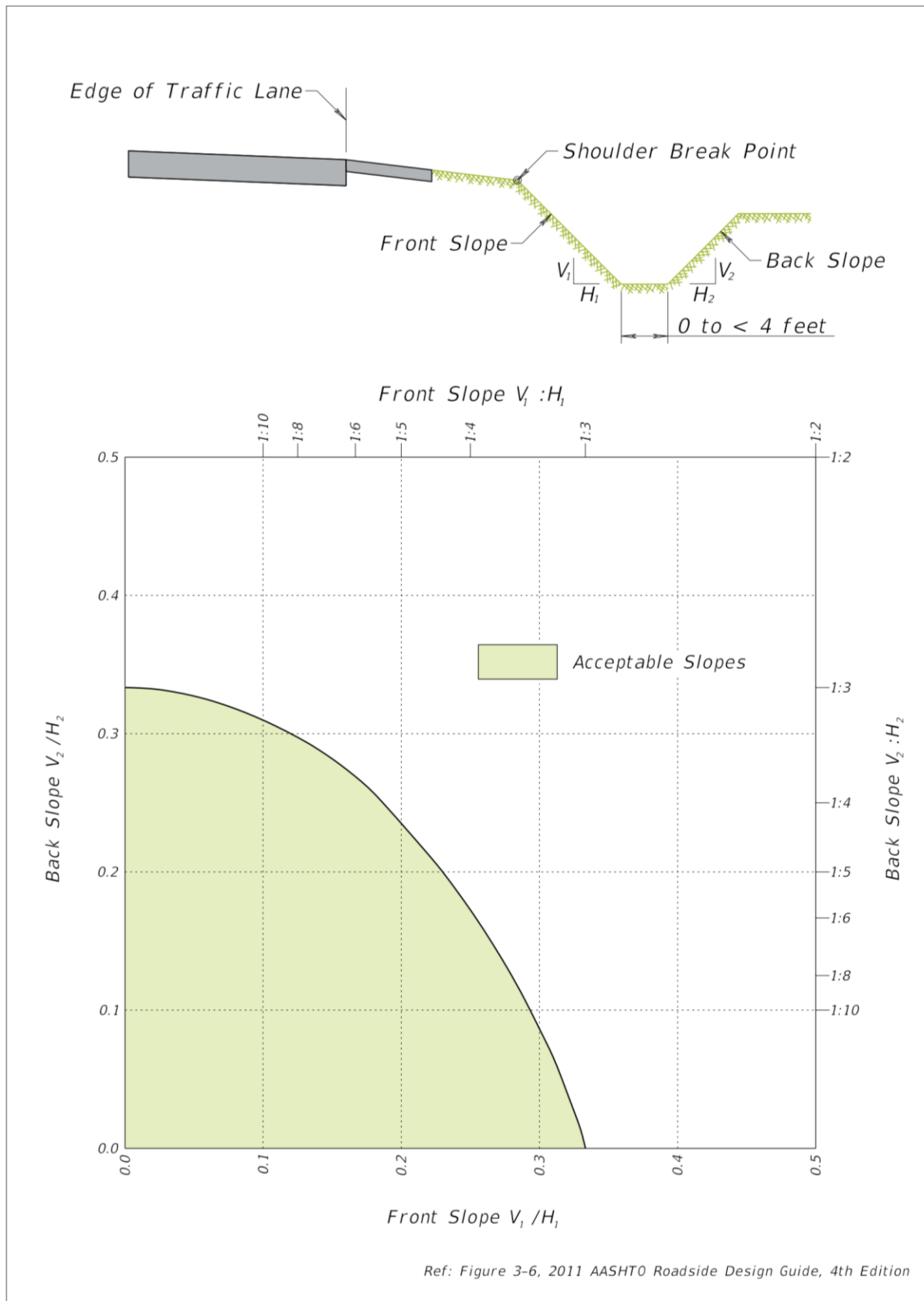
Figure 4-5. Roadside Ditches—Bottom Width 0 to < 4 ft (Source: Figure 3-6, AASHTO Roadside Design Guide 4th Edition [2011])
