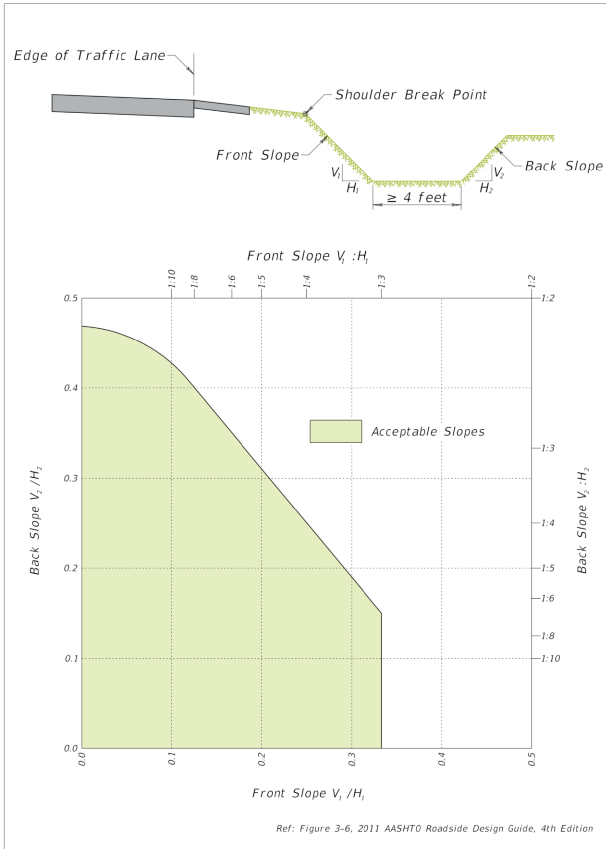
Figure 4-6. Roadside Ditches—Bottom Width \geq 4 ft (Source: Figure 3-6, AASHTO Roadside Design Guide 4th Edition [2011])
