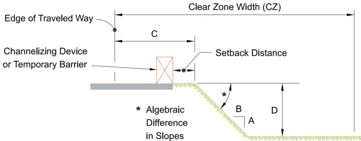
Figure 4-12. Drop-Off Condition Detail (Use with Table 4-6)
