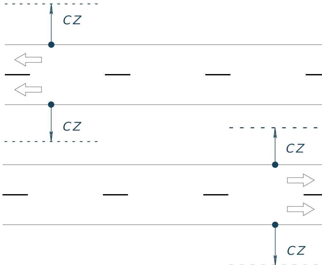
Figure 4-2. Clear Zone Plan View (Multilane, Two-Way Roadway)
